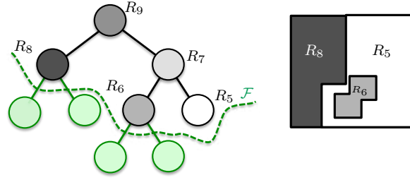
Figure 1.5: BPT pruning example
