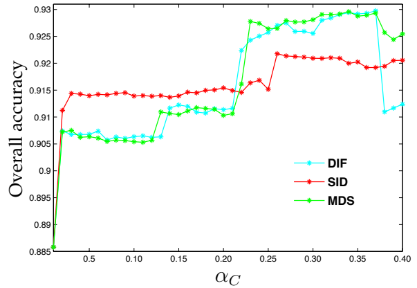
(b) Overall Accuracy versus \alpha_C
