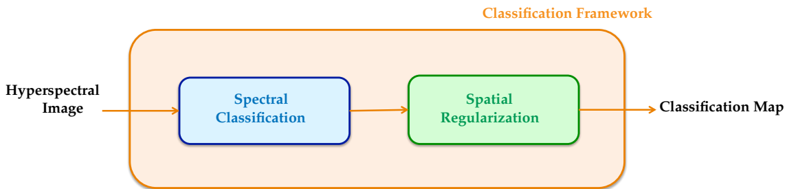
Figure 2.4: Spatial information as a post-processing stage
