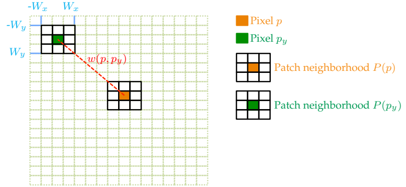
Figure 3.8: Two-dimensional illustration of the pixel probability distribution estimation. The probability of pixel value p is formed by the contributions to the histogram which depend on some weights. The weight w(p, p_j) is based on the similarity of the intensities in square neighborhoods P(p) and P(p_j) around p and p_j .
