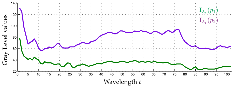
Figure 3.18: Shadow effect
