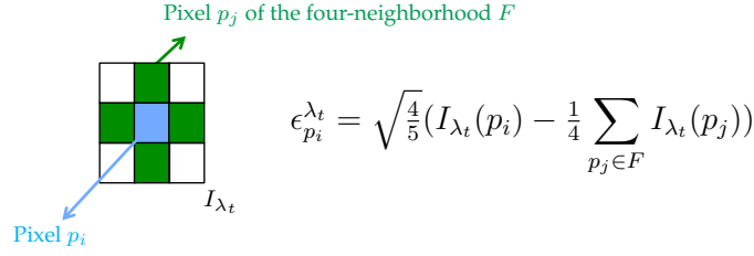
Figure 3.9: Pseudo-residual \epsilon_{p_i}^{\lambda_t} for the pixel p_i by using a four-neighborhood F
