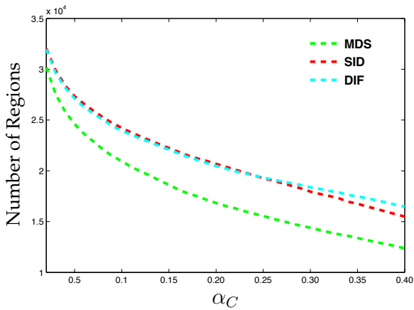
(a) Number of Regions versus \alpha_C
