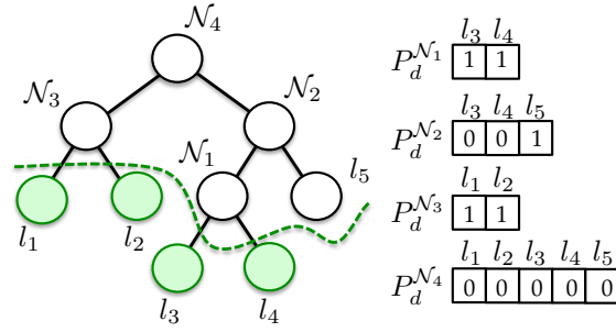
Figure 4.21: Example of BPT pruning
