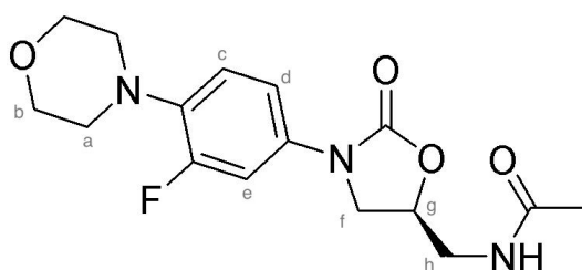
Figure 2.1 – Linezolid molecule ( \text{C}_{16}\text{H}_{20}\text{FN}_3\text{O}_4 ), with each proton-wielding carbon labelled arbitrarily.
