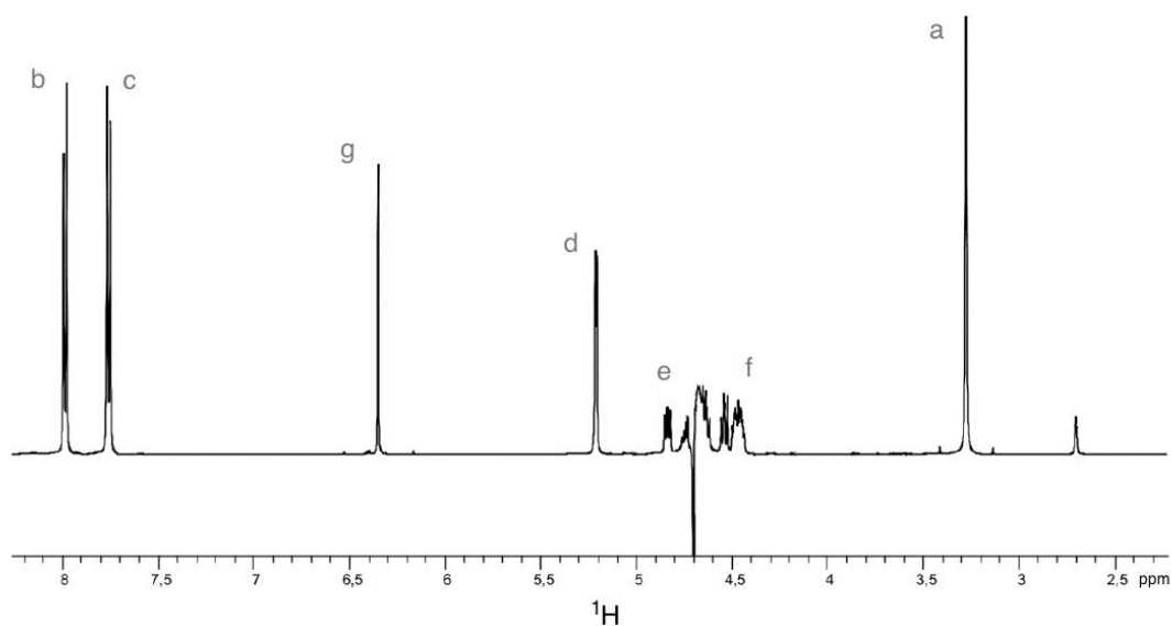
Figure 2.7 – 1D proton spectrum of florfenicol, no decoupling of ^{19}\text{F} . The proton peak around 2.8 ppm is due to the residual non-deuterated DMSO.
