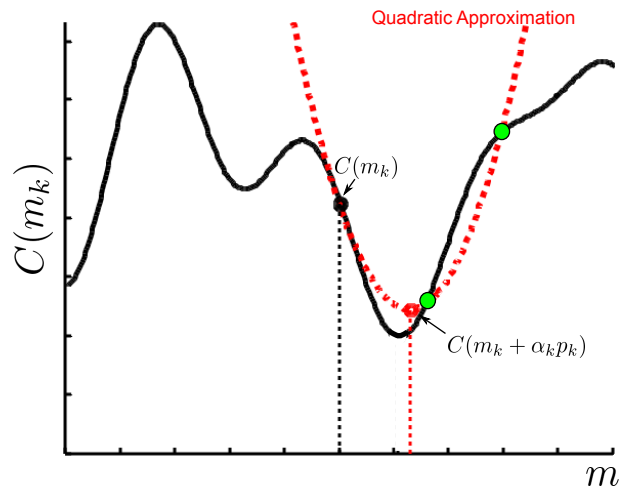
Figure 1.5: Illustration of the iterative decrease of the objective function by indirect local optimization. From the starting point m_k two additional forward modelling steps are applied for to calculate the cost function at two more positions (shown in green) along the current descent direction p_k . The updated model m_{k+1} = m_k + \alpha_k p_k comes from the minimum of the quadratic function (red dot) that joins C(m_k) and the two green points. This location must satisfy Wolfe's conditions (Reproduced from Menke, 1984; Vigh et al., 2009)
