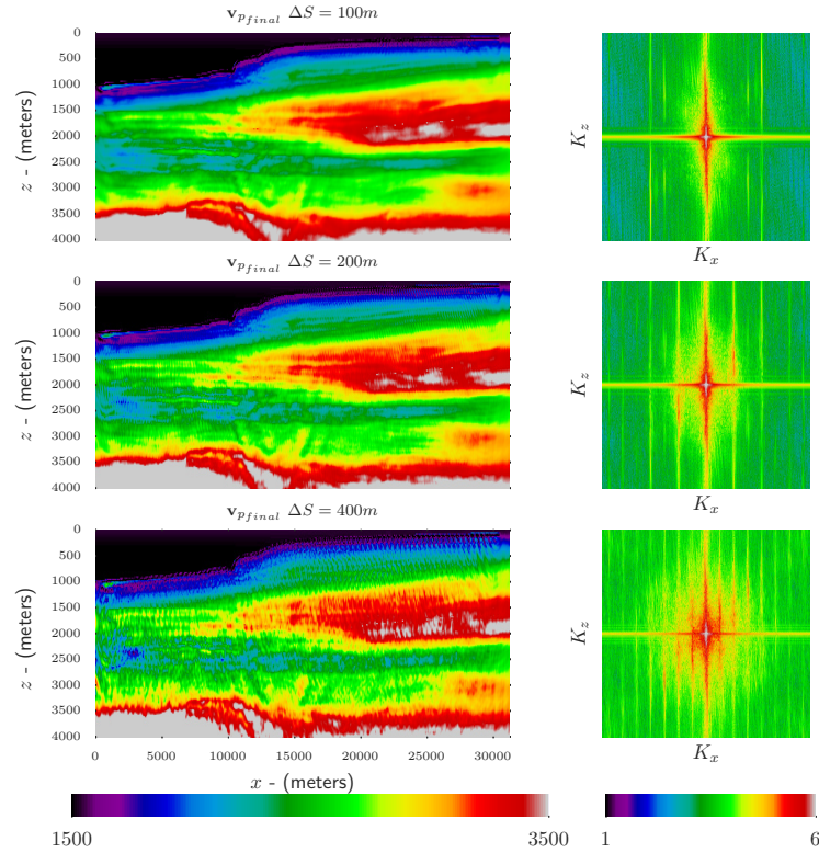
Figure 4.25: The final inversion results when FWI is performed with every 5 th (TOP), 10 th (CENTRE) or 20 th (BOTTOM) shot. The increased shot spacing results in aliased artifacts in the final inversion results.
