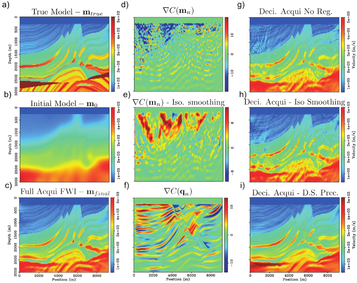
Figure 1.7: FWI applied to the Marmousi 2 model with a surface acquisition. a) True model, b) Initial Model, c) Final inversion result using \Delta S = 50 m, d) Gradient achieved using decimated shots \Delta S = 2,500 m e) \Delta S = 2,500 m gradient with isotropic smoothing f), \Delta S = 2,500 m gradient using data-space preconditioning. g,h,i and correspond to inversion results obtained from the gradients d,e,f respectively ( Reproduced from Guitton et al., 2012 ).
