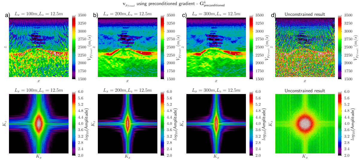
Figure 3.17: The final inversion result for the case with \mathbf{d}_{obs} contaminated with white noise. The inversion is constrained by the additive inverse Laplacian preconditioned gradient ( \mathbf{G}_{preconditioned}^0 ) using a) L_x = 100 m, b) L_x = 200 m and c) L_x = 300 m compared to the d) unconstrained gradient \mathbf{G}_{data}^0 . The top row is the final inversion results in the x - z domain while the bottom row shows the the wavenumber domain.
