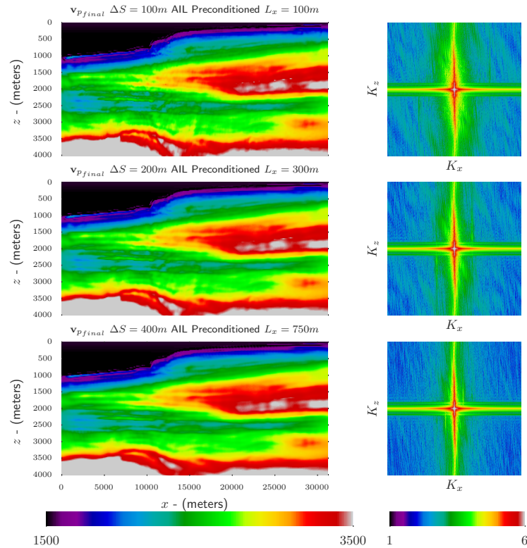
Figure 4.29: The final inversion results from FWI when it is performed with every 5 th (TOP), 10 th (CENTRE) or 20 th (BOTTOM) shot. The aliasing artifacts related to increased shot spacing are mitigated using horizontal correlation lengths of 100 m, 300 m and 750 m respectively.
