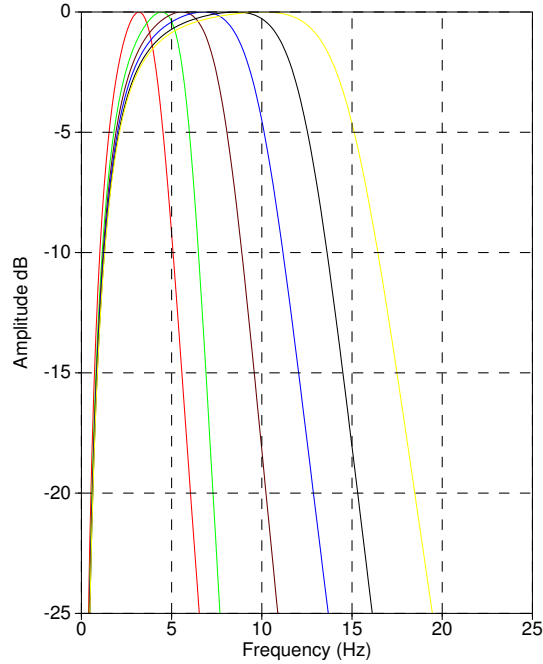
Figure 4.15: The six butterworth second order frequency bands used as part for FWI. The four frequencies describe the band pass filter being applied and correspond to those shown in Figure 4.1.
