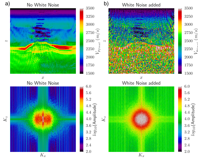
Figure 3.9: The inversion results for the case with no white noise a) and with white noise added b). The upper row shows the inversion results in the space domain ( x - z ) while the lower row shows the wavenumber domain K_x - K_z
