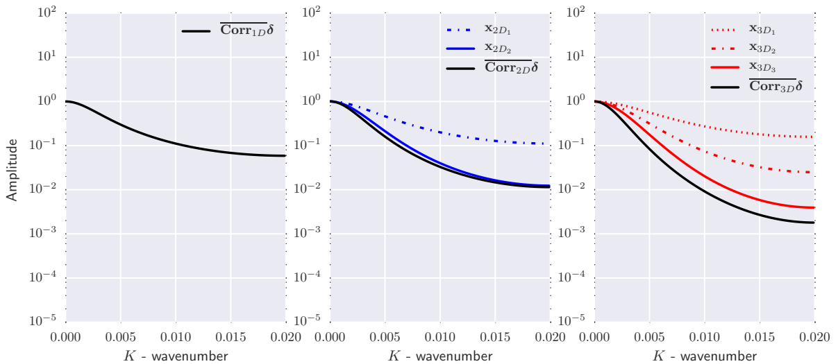
Figure 2.48: The vertical wavenumber of spike tests of operators in 1D ( LEFT ), 2D ( CENTRE ) and 3D ( RIGHT ). All examples have the same L value ( L = 50 m and h = 25 m) in 2D and 3D these represent the vertical wavenumber component calculate from 2D FFT (where K_x = 0 ) and a 3D FFT ( K_x = K_y = 0 ).
