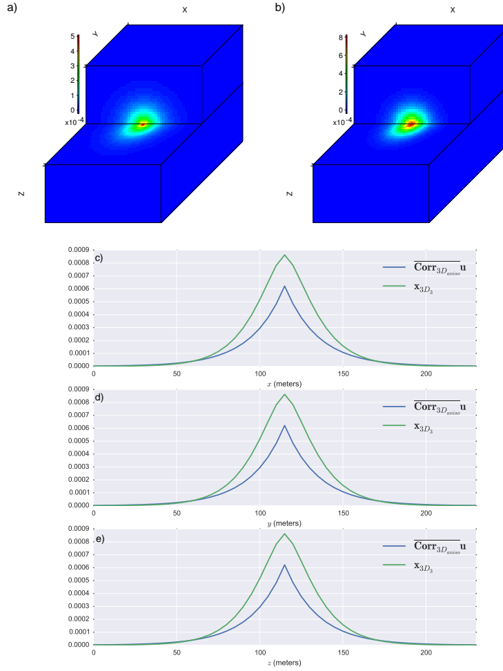
Figure 2.43: 3D vector spike test ( \mathbf{u} = \boldsymbol{\delta} ). a) \overline{\text{Corr}}_{3D_{aniso}} \mathbf{u} and b) \mathbf{x}_{3D_3} . Traces extracted from the middle of the model in the x c) y d) and z directions. e) The operators are not exactly the same but another test is used to compare their wavenumber filtering, properties on a more complex vector (Figure 2.44).
