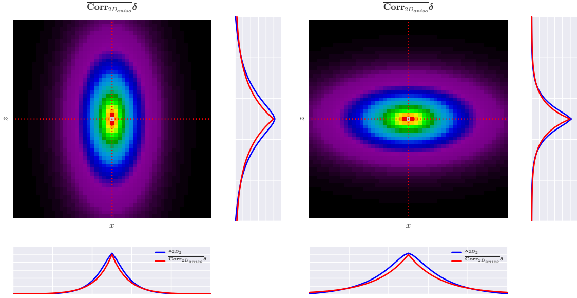
Figure 2.36: Comparison of \mathbf{x}_{2D_2} (blue) obtained from solving 2.44 twice as per Algorithm 1 vs the application of the normalized 2D Laplacian correlation function (red). a) L_x = 20 m and L_z = 40 m b) L_x = 40 m and L_z = 20 m. The sparse approach can handle anisotropic operators.
