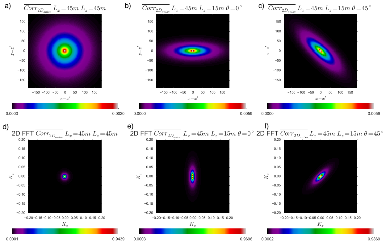
Figure 2.18: The impulse response of the 2D normalized anisotropic Laplacian correlation function (a,b,c) and the associated 2D FFT (d,e,f). When L_x = L_z we have an isotropic filter (a,d), however we may want to have an anisotropic filter where L_x \neq L_z (b,e) and if there is dip we may wish this to not be aligned with the geological dip (c,f)
