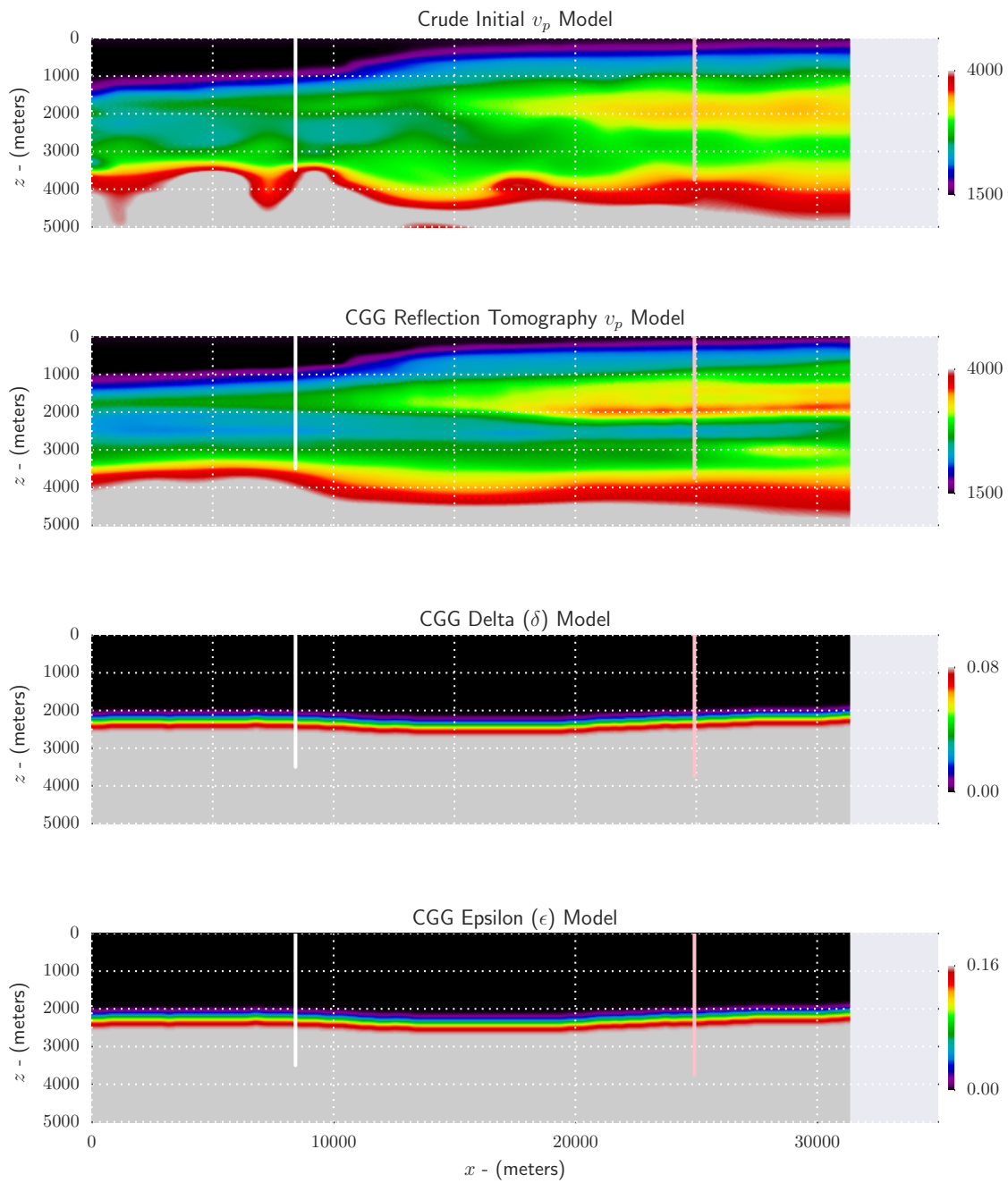
Figure 4.9: a) Crude initial velocity model built from stacking velocities, b) The reflection tomography FWI initial model built from a global velocity only tomographic update with the anisotropic parameters c) \delta and d) \epsilon set prior to the update. The location of the Chrysaor-1 (white) and WTR-4 (pink) wells are also annotated.
