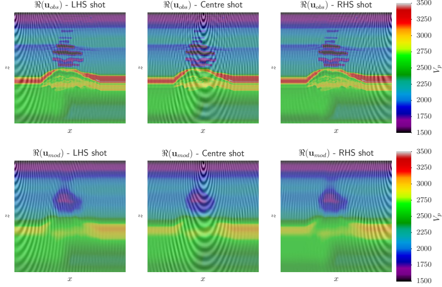
Figure 3.2: The real component of observed \mathbf{u}_{obs} ( TOP ) and modelled ( BOTTOM ) \mathbf{u}_{mod}(\mathbf{m}) monochromatic wavefields at 6Hz . Underlying the wavefields is the velocity model used for their respective calculation.
