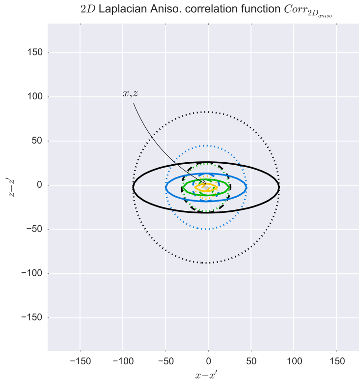
Figure 2.16: The 2D correlation function controls how nearby points (x', z') influence (x, z) . The anisotropic correlation function (solid contours) allows different correlation lengths in orthogonal directions. In this case horizontal correlation length ( L_x ) is 3 times larger than the vertical correlation length. The dotted circle shows the isotropic correlation function for function for L = 45 m while the dashed shows the correlation function for L = 15 m. Note that the solid lines contours intersect the dotted contours in the x-direction and the dashed contours in the y-direction.
