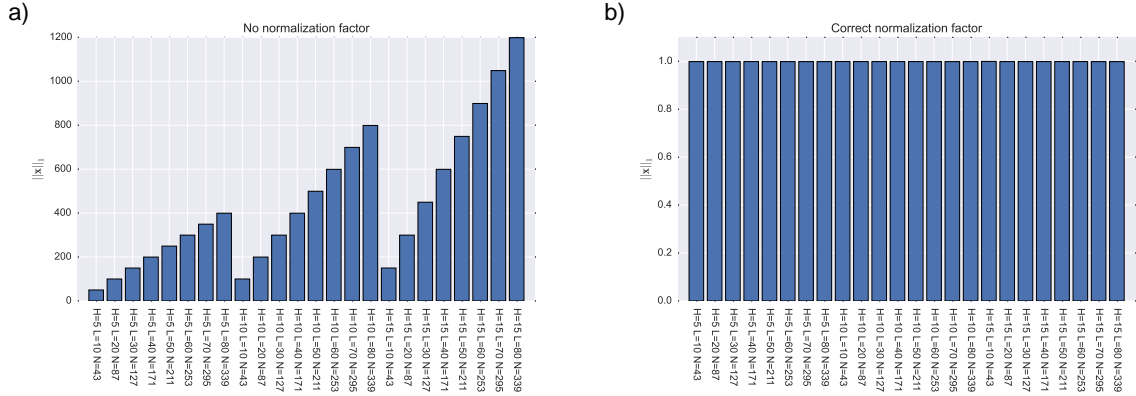
Figure 2.30: Comparison of the \ell_1 norm from what is obtained from solving the linear system involving \mathbf{Corr}_{1D}^{-1} a) as opposed to the one involving \overline{\mathbf{Corr}}_{1D}^{-1} b). The application of the normalization factor a = hL to \mathbf{Corr}_{1D}^{-1} ensures that \mathbf{x} is equivalent to \overline{\mathbf{Corr}}_{1D}^{-1}\mathbf{u} .
