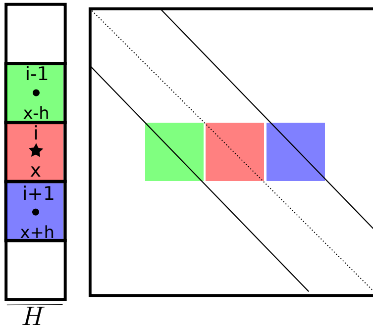
Figure 2.28: The inverse correlation stencil for a 1D vector of length 5. For each element in vector we only need to consider a given point (represented by the diagonal where x = x' represented in pink) and its neighbouring points x = x' \pm h .
