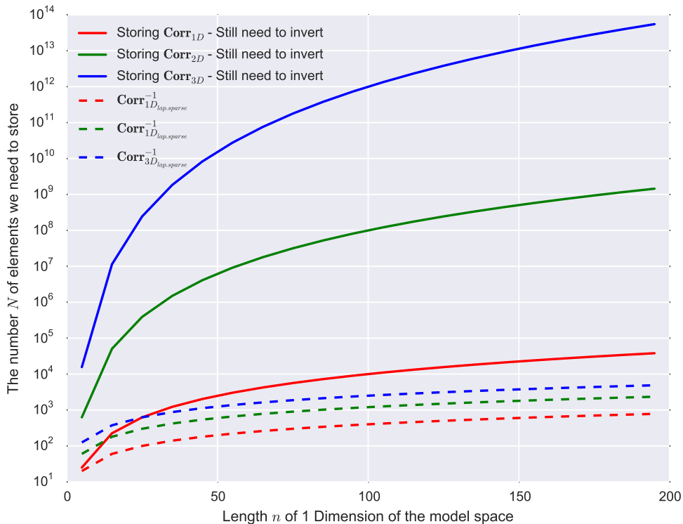
Figure 2.2: The memory required to store the correlation matrix \mathbf{Corr} . We consider a spatial vector \mathbf{u} of length n in 1D, length n \times n in 2D and n \times n \times n in 3D. If we want to store the correlation matrix (perhaps to calculate \mathbf{Corr}^{-1} ), we see that as n increases the memory requirements increases N = n^2 for \mathbf{Corr}_{1D} , N = n^4 for \mathbf{Corr}_{2D} and N = n^6 for \mathbf{Corr}_{3D} . This increasing memory complexity is shown by the solid lines. Our sparse inverse Laplacian memory requirements (dashed lines) require significantly less memory. Moreover, they do not need to be inverted for estimating the effect of the operator \mathbf{Corr}^{-1} .
