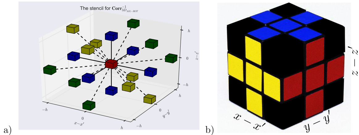
Figure 2.46: a) The stencil for the rotated inverse correlation operator \mathbf{Corr}_{3D_{AIL-ROT}}^{-1} b) The stencil can be visualized if one considers a rubix cube. We have 19 non-zero elements with the middle square being the diagonal. The 8 extreme corners are not involved in the stencil and are blacked out. NOTE: The colours on the rubix cube are of no significance and are not related to those in a).
