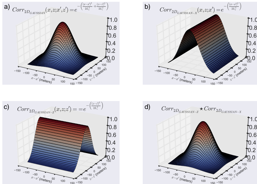
Figure 2.23: The Gaussian function a) is a multi-dimension function that can be applied in a tensorial fashion (Equation 2.26). The correlation function for the X only b) and Z only c) can be used to yield a function d) that is equivalent to the more expensive to apply operator a).
