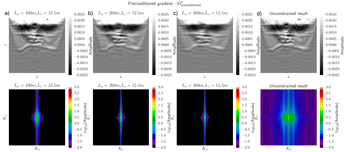
Figure 3.16: The additive inverse Gaussian preconditioned gradient \mathbf{G}_{\text{preconditioned}}^0 from the first iteration of FWI in the case where \mathbf{d}_{\text{obs}} contains white noise. The gradient preconditioning results for a) L_x = 100 m b) L_x = 200 m and c) L_x = 300 m are shown compared to the d) unconstrained gradient \mathbf{G}_{\text{data}}^0 . The top row is the gradient in the space domain while the bottom row is in the wavenumber domain.
