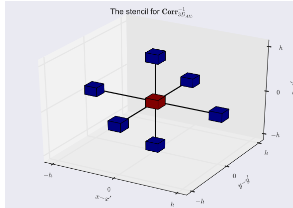
Figure 2.42: The stencil used to build \mathbf{Corr}_{3DAIL}^{-1} . The red point represents the diagonal of the \mathbf{Corr}_{3DAIL}^{-1} while the blue points are the cells at a space lag of \pm h away.
