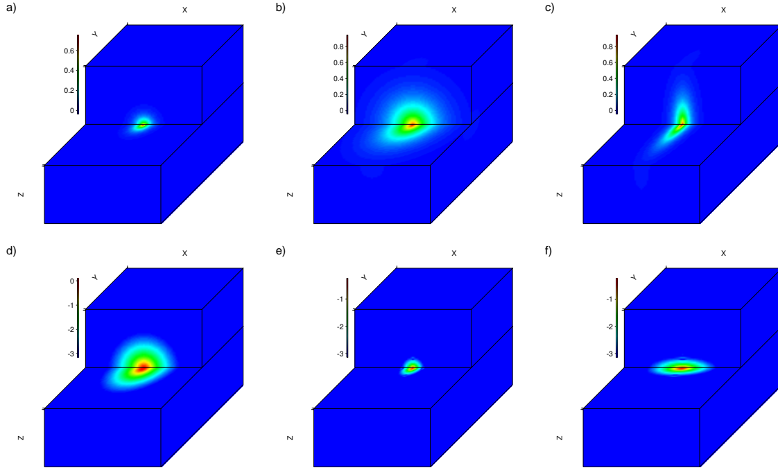
Figure 2.19: The correlation function for a 3D volume 75 \times 75 \times 75 . The top row (a,b,c) shows the 3D anisotropic correlation function Corr_{3D_{aniso}} a) L_x = L_y = L_z = 15 m b) L_x = L_y = L_z = 45 m c) L_x = 15 m, L_y = L_z = 45 m. The bottom row (d,e,f) shows the 3D wavenumber spectrum of \overline{Corr_{3D_{aniso}}} for the same L values as above. The display of Corr_{3D_{aniso}} for the top row and \overline{Corr_{3D_{aniso}}} for the bottom row is to make it easier the colourbar limits easier to choose. The bottom plot display the logarithm of the amplitude of the FFT).
