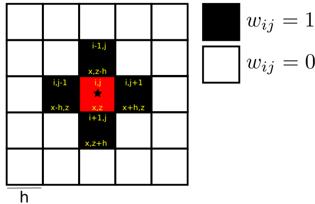
Figure 2.5: The weighting function w_{i,j} used in Figure 2.6. When calculating the Moran’s I function, we look at how similar the attributes surrounding the red cell are. It is important to note that, in our case, we only consider the 4 neighbouring cells as all other cells have a weighting value of zero.
