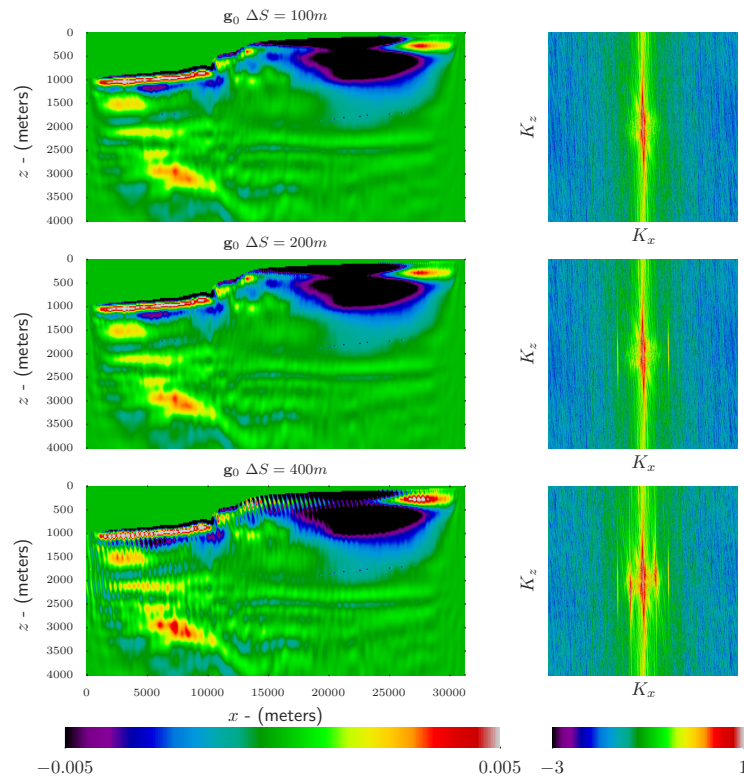
Figure 4.26: The gradient at the first iteration of FWI when it is performed with every 5 th (TOP), 10 th (CENTRE) or 20 th (BOTTOM) shot. The increased shot spacing results in aliased artifacts in the gradient.
