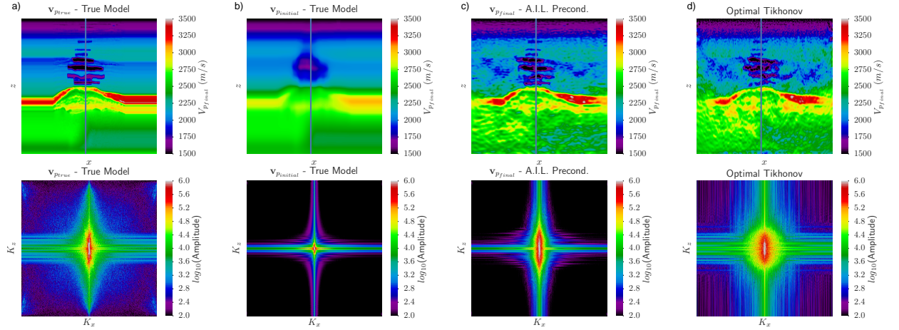
Figure 3.18: Composite of final inversion results and their spectrum. Note the blue vertical line represents the vertical extracted trace displayed in Figure 3.19 a) True Model, b) Starting model c) \mathbf{v}_{pfinal} -Additive inverse Laplacian and d) \mathbf{v}_{pfinal} -Optimal Tikhonov
