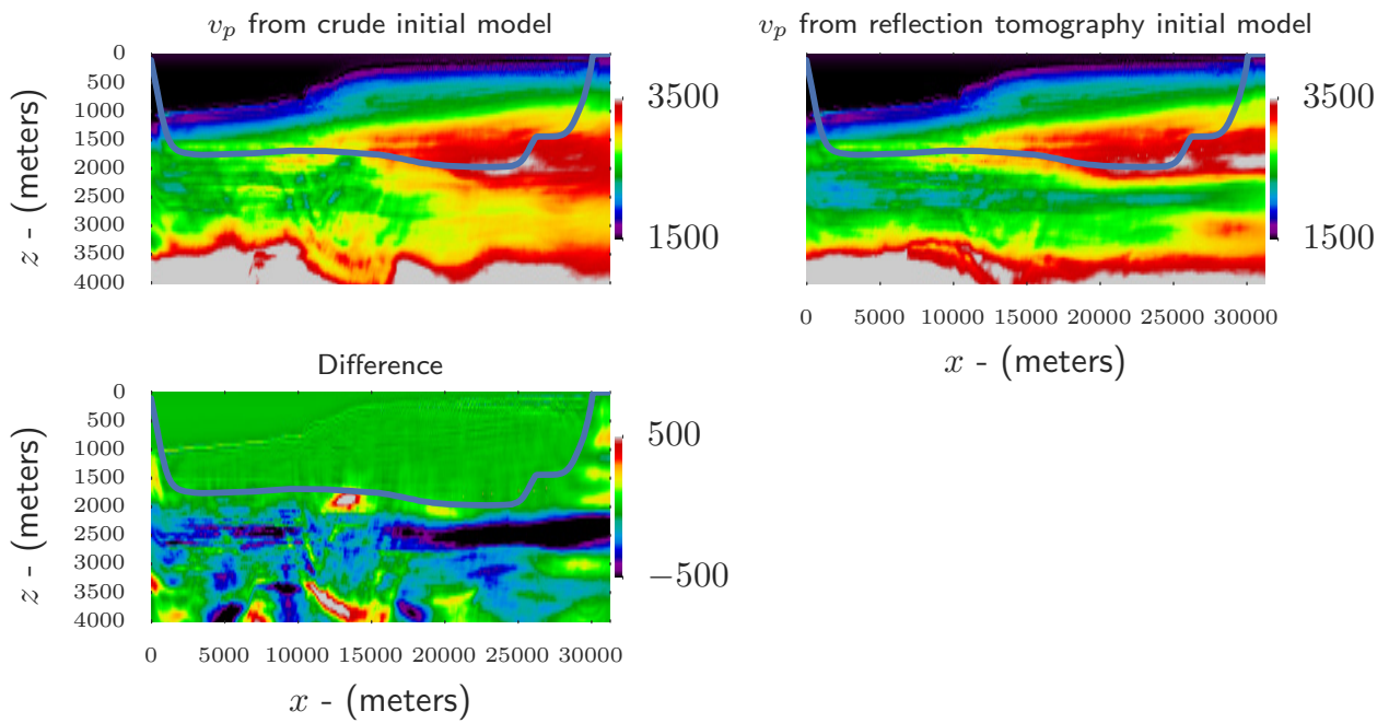
Figure 4.22: The final inversion result obtained using the ( TOP ) crude initial model ( CENTRE ) CGG reflection tomography initial model ( BOTTOM ) The difference between the two results, with the blue line highlighting the penetration of diving waves calculated using a back-ray-tracing algorithm.
