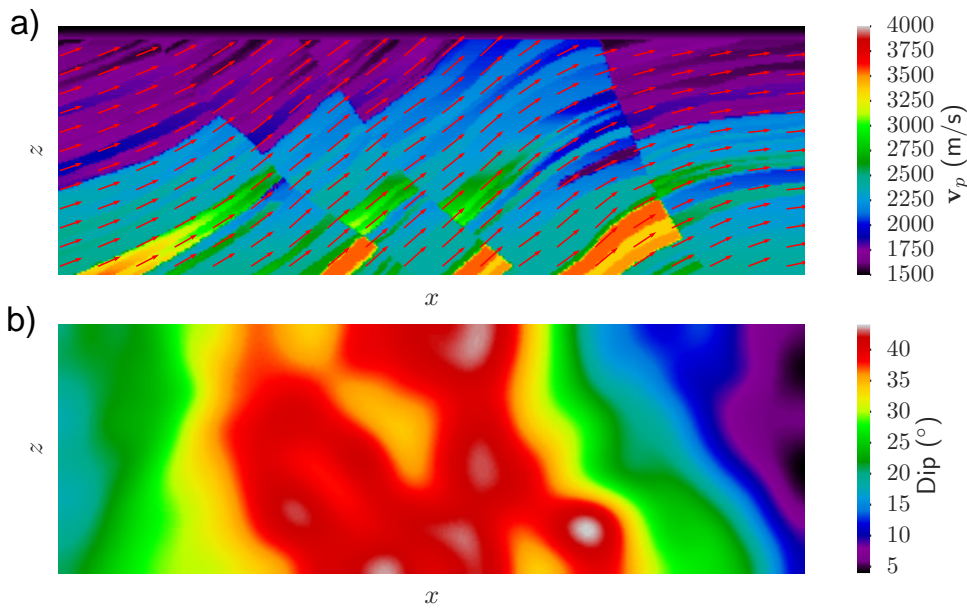
Figure 3.20: The Marmousi synthetic model. a) The true Marmousi velocity model. The red arrows show a vector field representation of the geological dip of the stratigraphy in the model. The scalar value of the dip is shown in the dip vector b). Note the dip values range from 5^\circ to 45^\circ .
