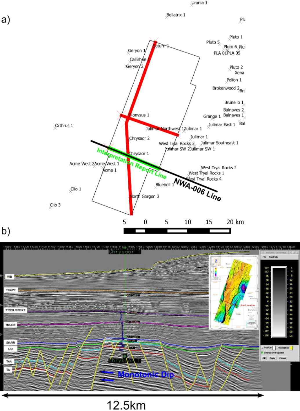
Figure 4.8: a) The Chrysaor-East Anisotropic PreSDM project is highlighted by the polygon. Three 2D lines are displayed in the report (Red and green). b) The green line was coincident with a portion of the NWA-006 line and showed the expected structure in the shallow part and at depth. Note the relatively homogeneous dip in the Chrysaor-1 structure.
