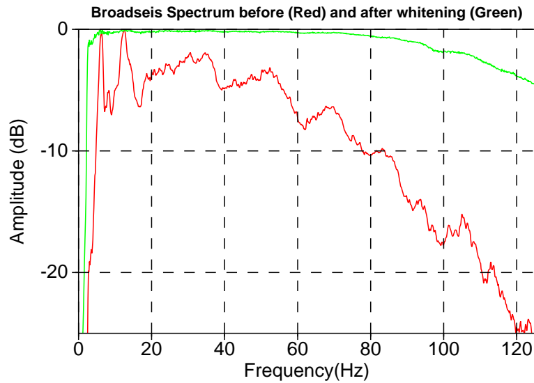
Figure 4.13: The Broadseis spectrum before (red) and after (green) minimum phase spectral whitening.
