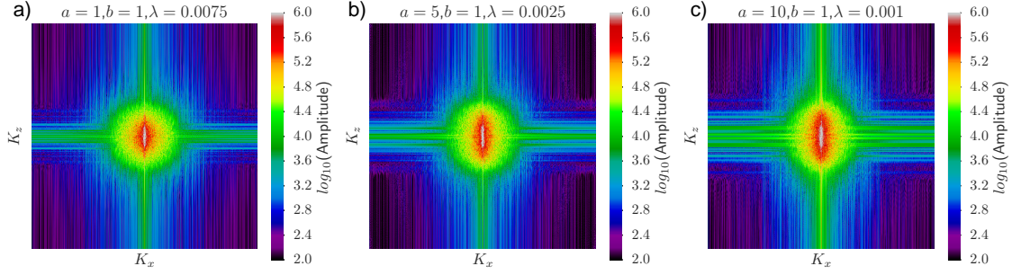
Figure 3.12: Frequency spectrum of Tikhonov results with optimal value of \lambda . a) \frac{a}{b} = 1 b) \frac{a}{b} = 5 c) \frac{a}{b} = 10 . As we increase the penalty on high wavenumber variations in the horizontal direction we add in more stable vertical wavenumbers
