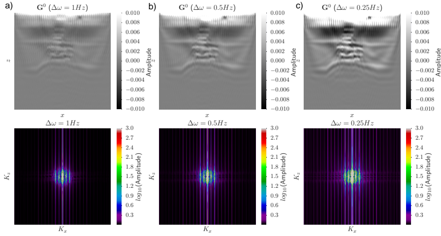
Figure 3.6: The impact of the frequency increment \Delta\omega on the FWI gradient \mathbf{G} . We show the first gradient \mathbf{G}^0 computed in the first band for a): \Delta\omega = 1Hz , b): \Delta\omega = 0.5Hz and c): \Delta\omega = 0.25Hz . The top row shows the gradients where it can be seen that the geological features we want to add to our initial model become more dominant as \Delta\omega decreases. The wavenumber spectrum shows that we have strongly aliased sampling of the wavenumber spectrum in the horizontal direction.
