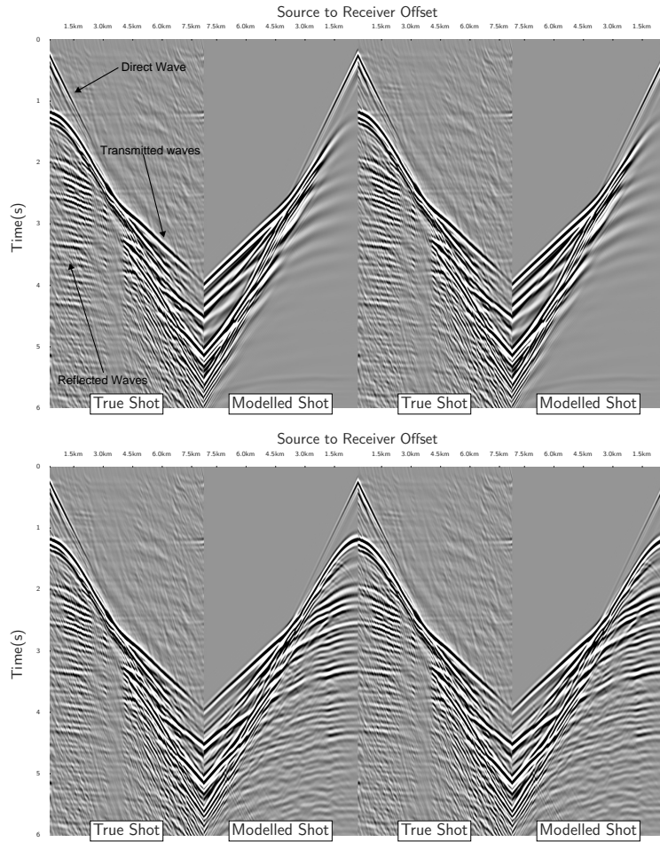
Figure 2: A true shot record prior to FWI compared to the modelled shot record TOP : Before FWI BOTTOM : After FWI. The shot records are mirrored so that the match between the near and far offsets can be observed. The key "families" of waves (direct, reflected and transmitted) are highlighted, all of which are involved in the fitting process in FWI.
