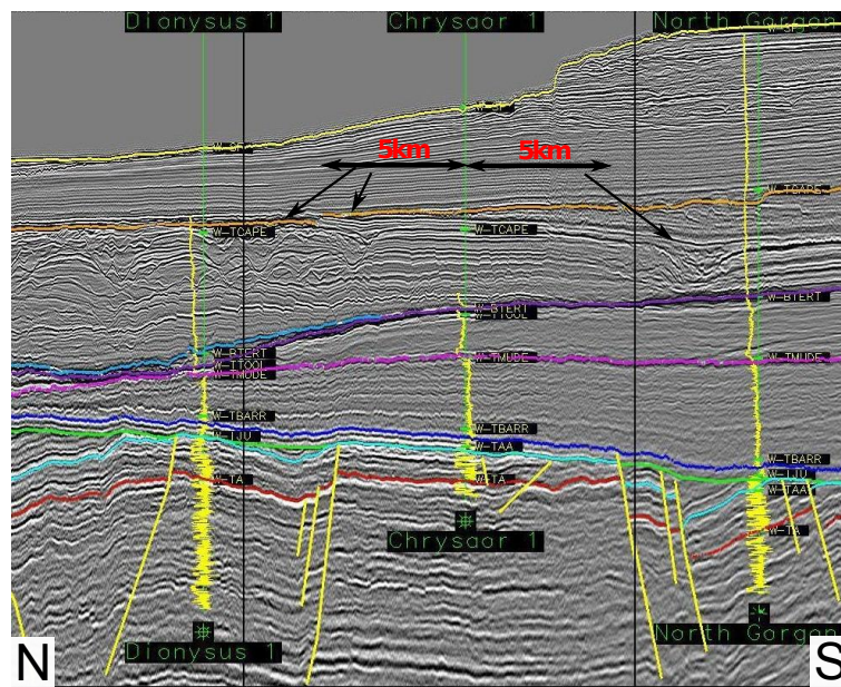
Figure 1.14: An image taken from Walton (2008) showing some of the chaotic seismic character that may cause "out of plane" effects on the NWA-006 line.
