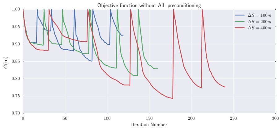
Figure 4.27: The evolution of the objective function for different levels of shot decimation
