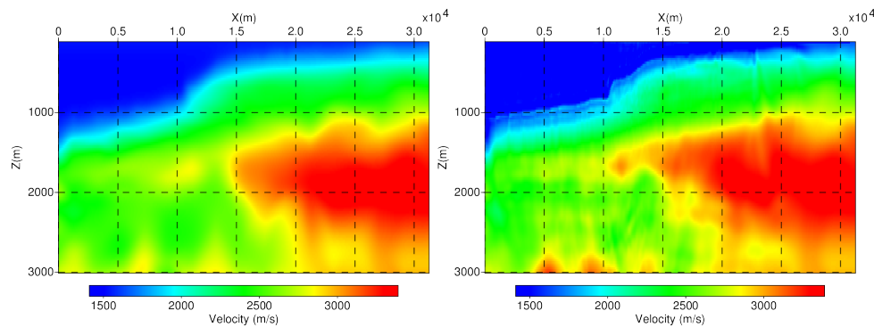
Figure 2 The initial velocity model is shown in the left panel and the final velocity model is shown on the right panel. Same color scale is used in both figures
