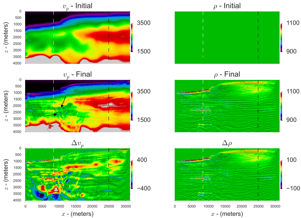
Figure 4.20: FWI using the crude initial model.
