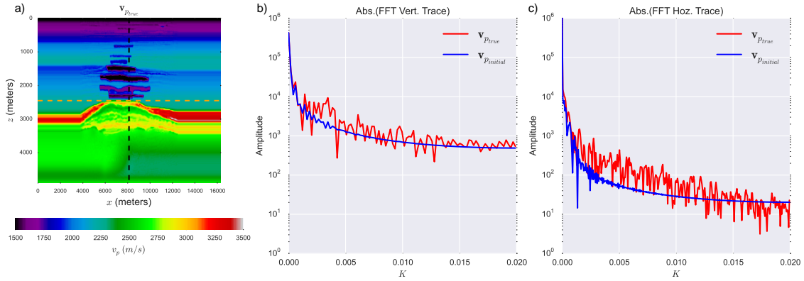
Figure 2.10: a) The Valhall synthetic model with a vertical b) and horizontal c) trace extracted. The plots in b) and c) show the wavenumber spectrum of the true (red) and initial model (blue).
