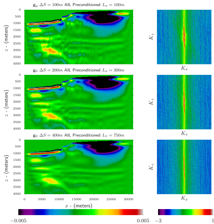
Figure 4.28: The gradient at the first iteration of FWI when it is performed with every 5 th (TOP), 10 th (CENTRE) or 20 th (BOTTOM) shot. The aliasing artifacts related to increased shot spacing are mitigated using horizontal correlation lengths of 100 m, 300 m and 750 m respectively.
