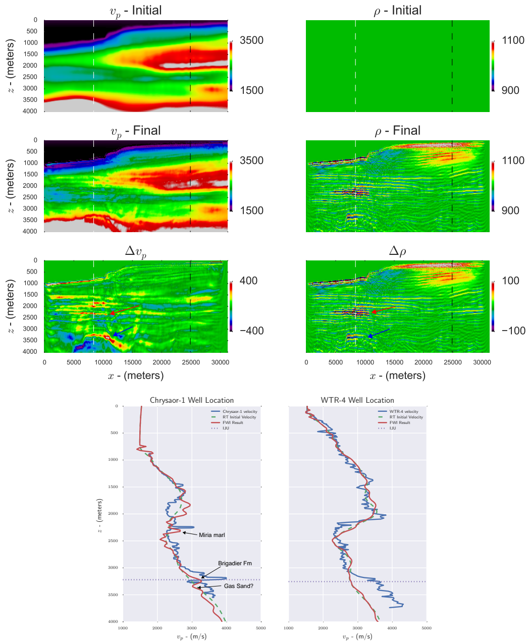
Figure 4.16: FWI using reflection tomography initial model. The arrows highlight the Miria Marl at H2 and the IJU (Brigadier Marl to Triassic gas sand).
