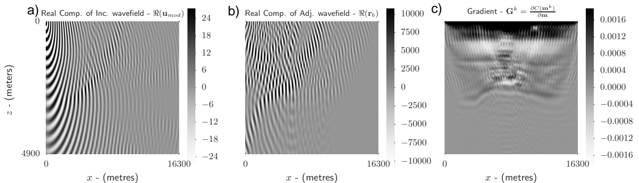
Figure 3.4: a): The incident wavefield \mathbf{u}_{mod}^k for a source at the LHS extreme of the model. The restriction operator \mathbf{R} is applied to allow calculation of the residual vector \Delta \mathbf{d}^k before these residuals are re-injected at the receiver locations (using \mathcal{P} ) to calculate the back-projected adjoint field \mathbf{r}_b b). The gradient is formed from the combination of these two wavefields 3.12. c). The gradient in this example is computed from summation over all of the 48 shots for the monochromatic frequency \omega = 6Hz
