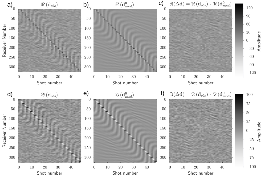
Figure 3.8: The effect of white noise contaminating \mathbf{d}_{obs} on our residual vector \Delta\mathbf{d}^k . We show the real (a,b,c) and imaginary (d,e,f) components for the 6Hz monochromatic frequency. A comparison of the residual without noise is shown in Figure 3.3
