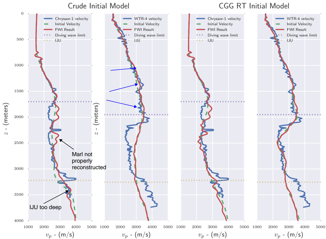
Figure 4.21: The FWI results from the crude initial model ( LEFT ) and the reflection tomography initial model ( RIGHT ). Blue arrows highlight apparent improvement of the velocity.
