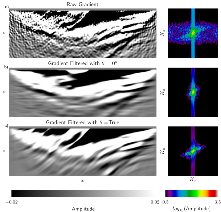
Figure 3.22: The FWI gradient from the first iteration of the inversion. a) The raw gradient with no preconditioning operator is contaminated by noise. If we perform preconditioning using L_x = 75\text{m} and L_z = 10\text{ m} (b) we see that we have decreased noise but suppressed much of the sharpness of the dipping reflectors. We are able to remove the noise and keep the reflectors by using the preconditioning with our variable dip vector (d). The wavenumber spectrums are also shown for each of the gradients is shown on the right.
