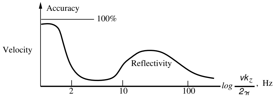
Figure 1: The different wave-number reconstruction of the subsurface from the velocity macro-model (low wavenumbers) vs reflectivity information (high wavenumbers). There is a gap in the intermediate wave-number region. Taken from (Claerbout, 1985).
