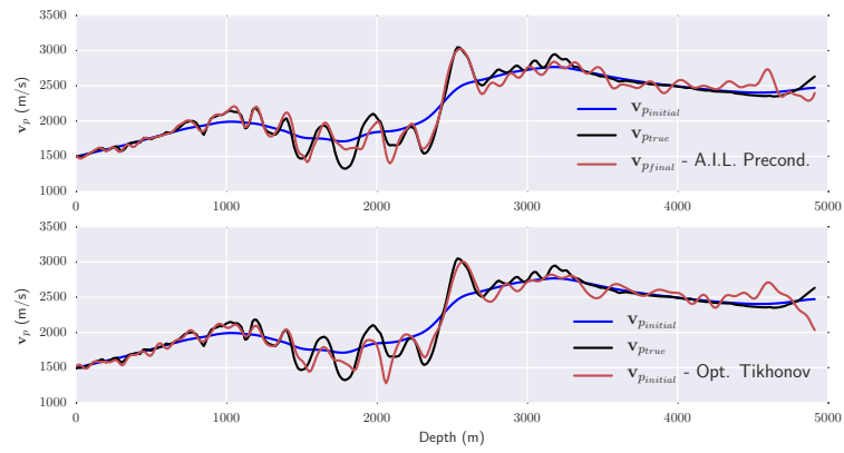
Figure 3.19: Extracted vertical trace from inversion results for the additive inverse Laplacian preconditioned ( TOP ), and the optimal Tikhonov ( BOTTOM ). The blue line represents the initial model while the black and red are the true and inversion result respectively.
