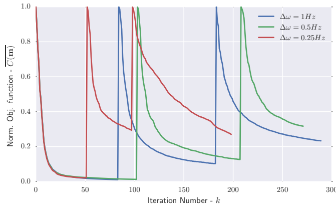
Figure 3.7: The objective function for the 3 bands involved in the test of the effect of frequency sampling on the FWI model. Note: The behaviour where the curve spikes back up to the value of 1.0 occurs when the previous frequency band has converged and the next frequency band is selected.
