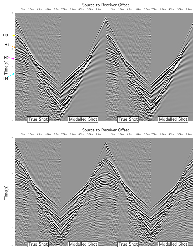
Figure 4.18: Shot taken from the approximate Chrysaor-1 location before ( TOP ) and after ( BOTTOM ) FWI using the reflection tomography initial model. The key stratigraphic horizons are highlighted in the shot record (H3 appears too weak to see on an individual shot record.)
