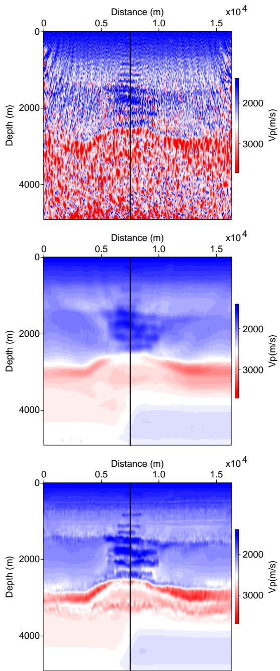
Figure 4: Comparison of Final Vp Inversion Results: No Preconditioning(TOP) Constant (200m) L Preconditioning Result(CENTER) Variable L Preconditioning Result (BOTTOM). The black line represents the extracted trace in Figure 5.
