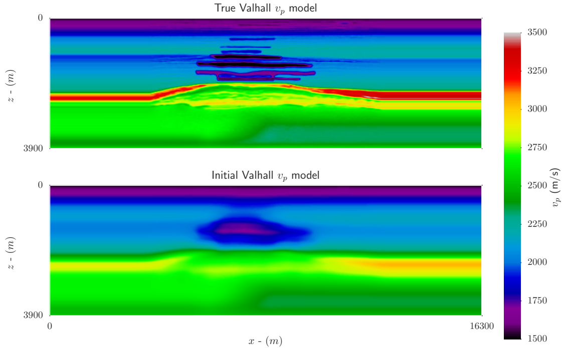
Figure 1.10: a) The true Valhall synthetic velocity model. b) 375 m Gaussian smoothed version of the true model that serves as the starting point for FWI.
