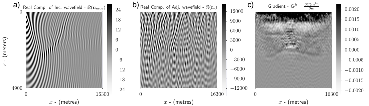
Figure 3.10: The real component of the incident a) and back propagated adjoint b) wave-fields for the case with white noise for a shot on the LHS of the model. We see that the adjoint wavefield contains much more noise than we noticed in Figure 3.4. When we sum over all the shots c) we can see the imprint of the geology we want to reconstruct but also significant amounts of noise.
