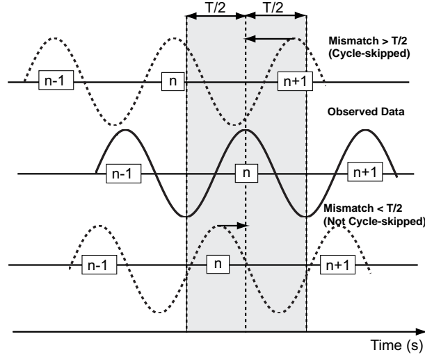
Figure 1.4: The "cycle skipping phenomena". Two cases for the modelled data, \mathbf{d}_{mod} are shown. The top trace shows the case where the distance between the n^{\text{th}} peak of the modelled data and the observed data \mathbf{d}_{obs} is greater than half a period ( \frac{T}{2} ). The data in this case is cycle skipped. The bottom trace shows a difference in timing of less than \frac{T}{2} . FWI will be able to account for this kinematic mismatch. Modified from (Virieux and Operto, 2009).
