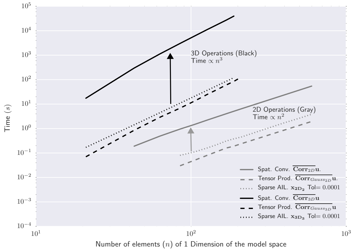
Figure 2.51: Computational cost sensitivity described by increasing the size of the model vector \mathbf{u} while keeping the value of L constant. The gray and black arrows highlight the large increase in computation time when comparing AIL and tensorized Gaussian to the spatial convolution approach.
