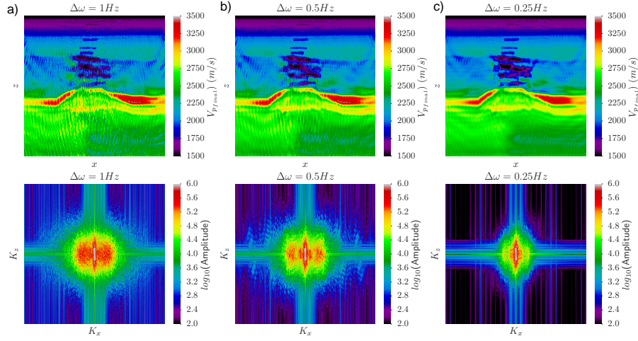
Figure 3.5: The impact of the frequency increment \Delta\omega on the final FWI result. a) \Delta\omega = 1Hz , b) \Delta\omega = 0.5Hz and c) \Delta\omega = 0.25Hz . The top row shows the final value of \mathbf{m} while the bottom row shows the wavenumber spectrum of these results. It can be seen that the contamination of high wavenumber noise increases as the value of \Delta\omega increases.
