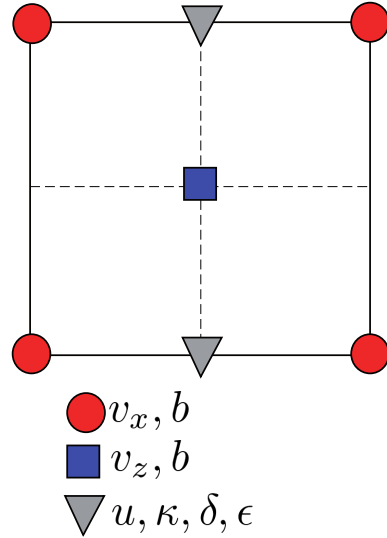
Figure 4.1: Staggered grid for Virieux-Lavander stencil adapted to the Acoustic VTI case
