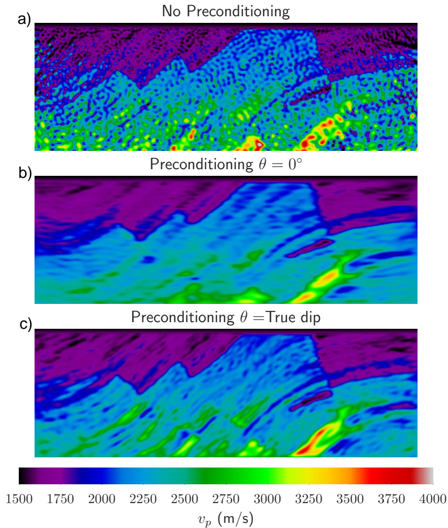
Figure 3.23: The inversion results obtained from the 3 preconditioning strategies: a) No preconditioning, b) Preconditioning zero dip, c) Preconditioning with variable dip. The best result occurs when we precondition with the correct dip field.
