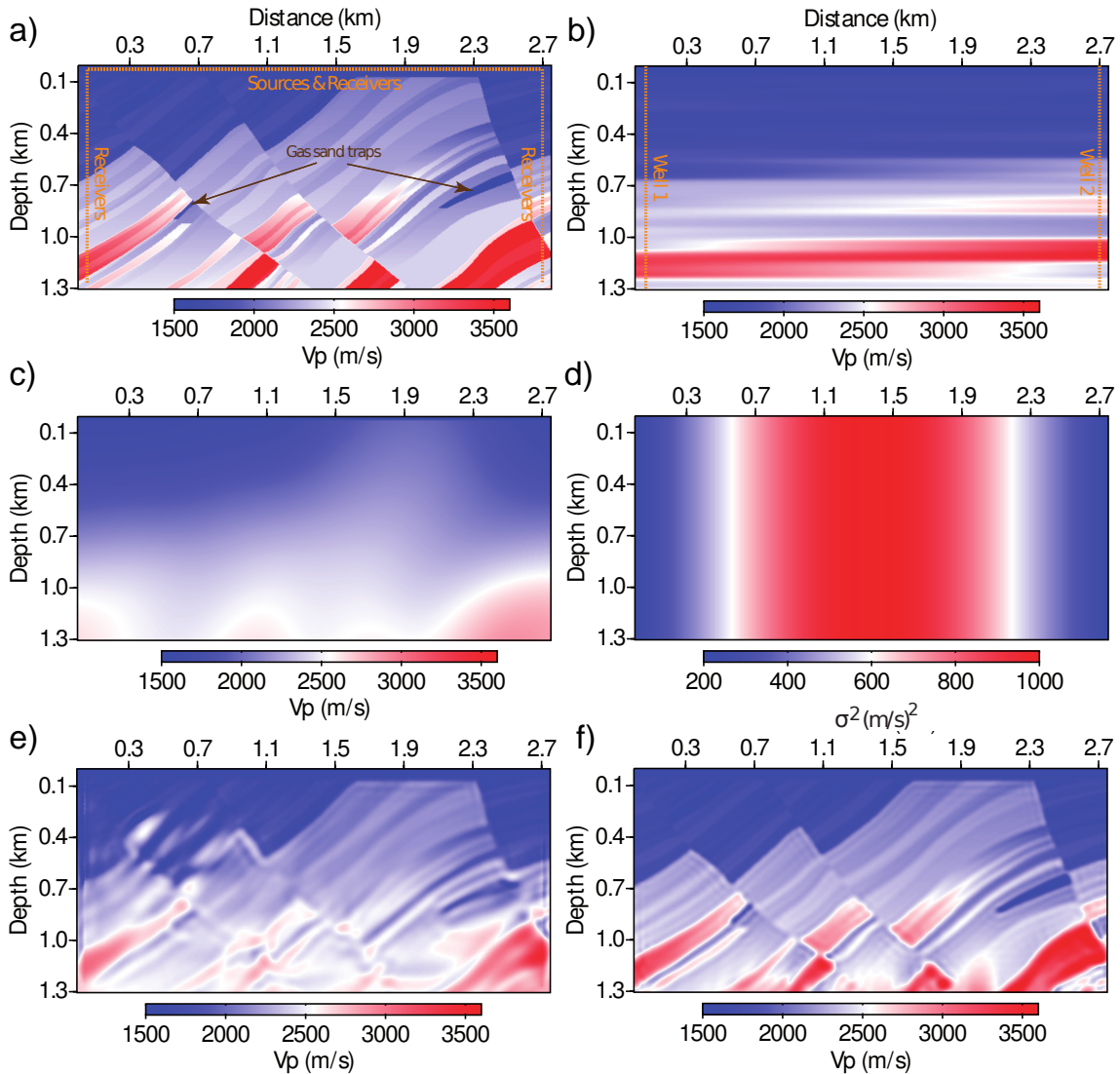
Figure 1.6: Application of prior-model regularization a) The true Marmousi velocity model, c) The initial model for FWI, b) The prior model vector \mathbf{m}_p built from interpolation of the two wells d) The uncertainty of \mathbf{m}_p e) The inversion result without using prior, f) the inversion result using prior model regularization ( Recreated from Asnaashari et al., 2013 ).
