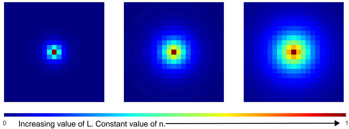
Figure 2.50: Computational cost sensitivity attained by increasing the correlation length, L while keeping the value of n constant.
