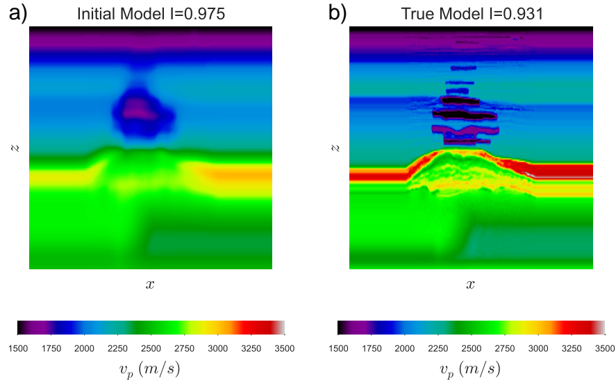
Figure 2.7: Moran's I classification applied to the Valhall model a) \mathbf{v}_{p_{initial}} b) \mathbf{v}_{p_{true}} . Note that both have a strong degree of clustering as can be identified from visual inspection.
