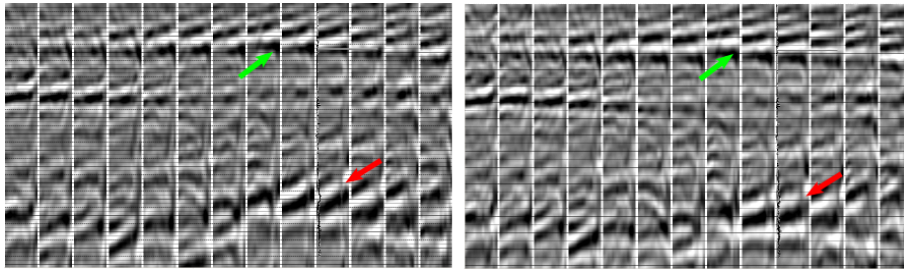
Figure 4.17: The common angle gathers computed using ( LEFT ) Reflection Tomography initial model ( RIGHT ) velocity model after FWI. The green arrow highlights the Miria marl while the red arrow highlights the IJU reflector at the Chrysaor structure.
