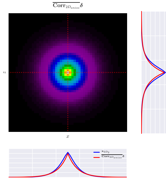
Figure 2.35: Comparison of \mathbf{x}_{2D_2} (blue) obtained from solving 2.44 twice using Algorithm 1 versus the application of the normalized 2D Laplacian correlation function (red). The extracted vertical and horizontal traces show the decay of the two results. Both results show similar decay characteristics and are both well normalized.
