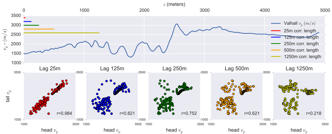
Figure 2.11: Calculation of correlation coefficients for head of the correlation vector compared to the tail. 5 lengths of correlation vector are shown (25 m, 125 m, 250 m, 500 m and 1250 m). The correlation vectors can be seen as a sliding window where the point on the LHS (head) of the vector is compared to the RHS (tail). As the length of this vector increases, the linear correlation coefficient r between the head and the tail decreases.
