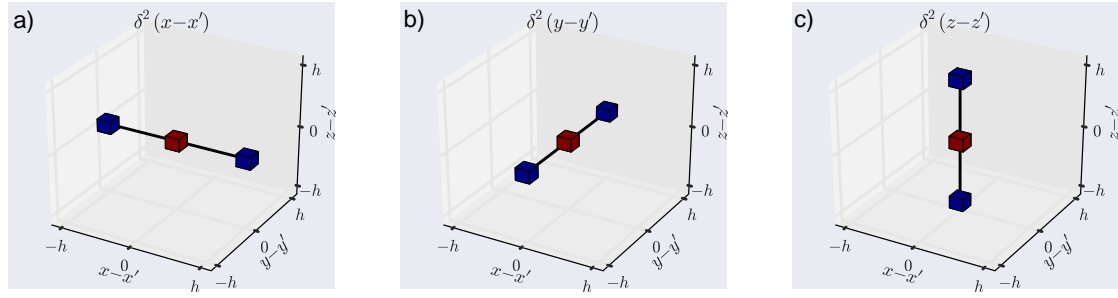
Figure 2.41: The discretization of the \delta^2 for the 3 orientations in 3D. The red cube is the diagonal which has a value of -\frac{2}{h^3} while the blue cubes are the off diagonal terms that exist at a space lag of h . These have the value \frac{1}{h^3} . The discretization of \delta only occurs on the diagonal of the matrix (shown in red) and has a value of \frac{1}{h}
