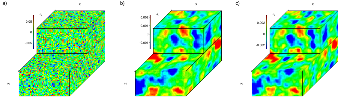
Figure 2.44: A white noise vector \mathbf{u} = \boldsymbol{\epsilon}_w a) is used to compare the application of the brute force approach b) \mathbf{Corr}_{3D_{aniso}} \mathbf{u} and the result from solving the sparse linear system b) \mathbf{x}_{3D_3}
