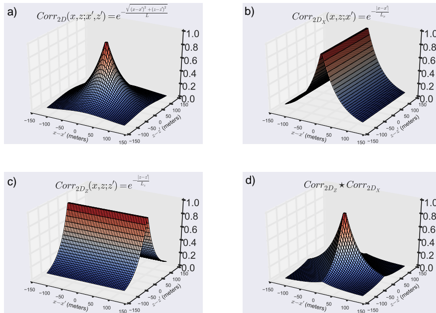
Figure 2.24: The Laplacian function a) is a multi-dimension function that cannot be applied in a tensorial fashion (Equation 2.26). The correlation function for the X only b) and Z only c) cannot be used to yield a function d) that is equivalent to the more expensive to apply operator a).
