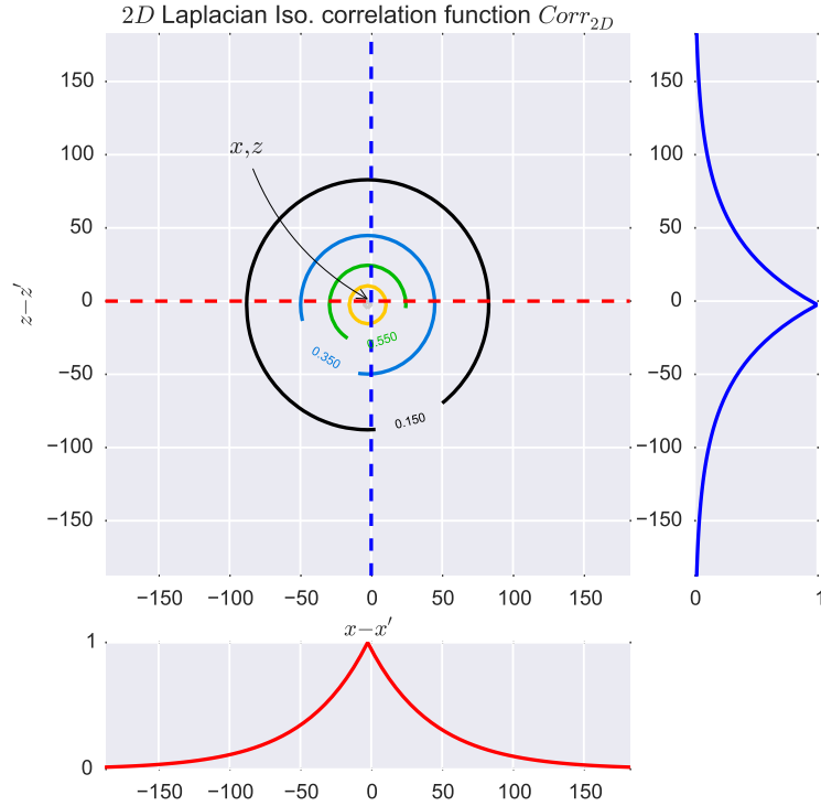
Figure 2.15: The 2D correlation function control how points that at some space-lag x', z' influence the points at x, z . When there is zero space lag ( x = x' and z = z' ) the correlation coefficient is equal to 1. As we increase the space-lag the correlation decreases.
