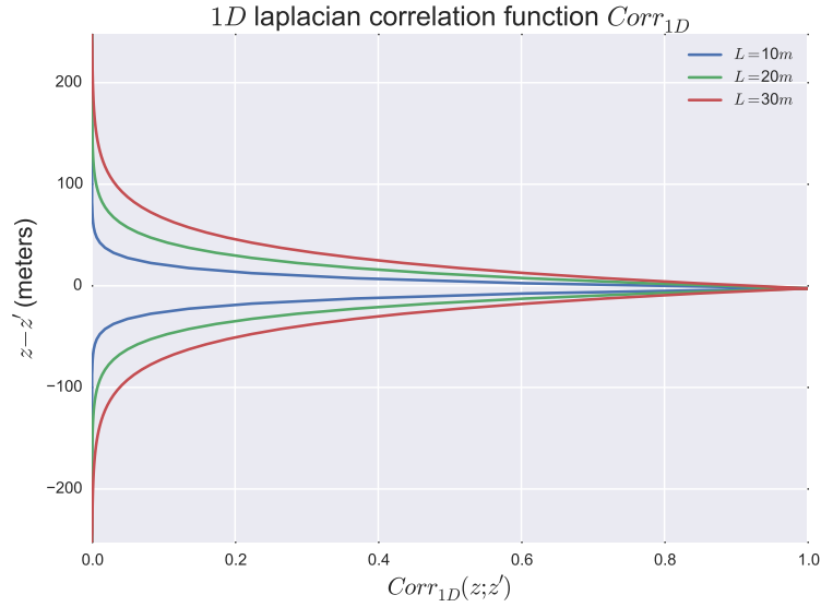
Figure 2.13: Correlation based on the Laplacian distribution described in equation 2.5. The correlation function can also be seen as a special case of the covariance function equation 2.4 when \sigma = 1
