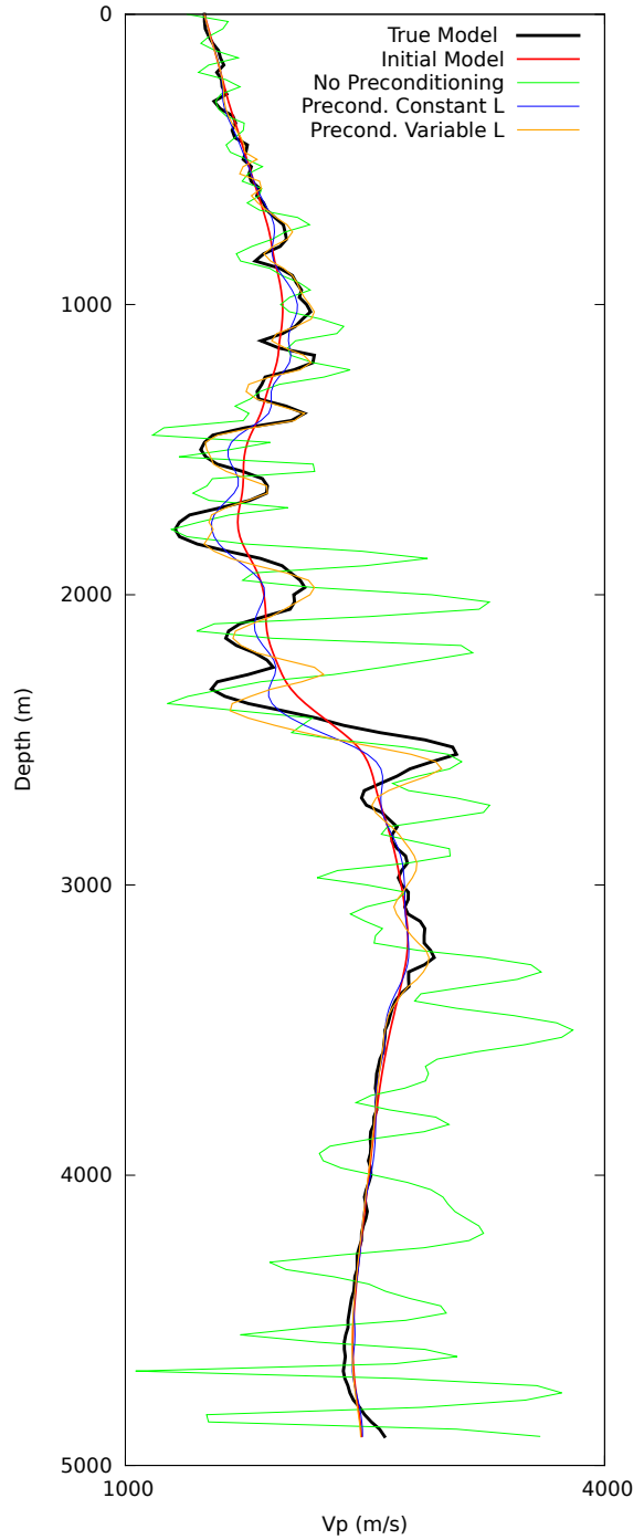
Figure 5: Inversion extracted trace comparison.
