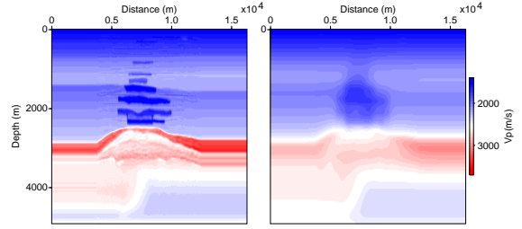
Figure 1: True Vp model(LEFT) and Initial Vp Model (RIGHT).
