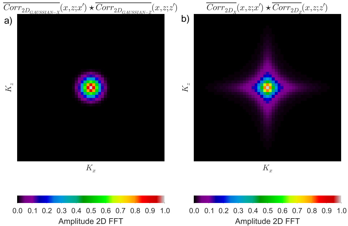
Figure 2.25: The wavenumber spectrum for the tensor application of Gaussian operator a) and tensor application of the Laplacian operator b). The tensorized Gaussian operator has a familiar circular wavenumber spectrum (elliptical if L_x \neq L_z ). The tensor application of the Laplacian has a strong effect coming from wavenumbers aligned with the Cartesian directions. This operator will cause undesired angle dependent effects when it is applied as a filter.
