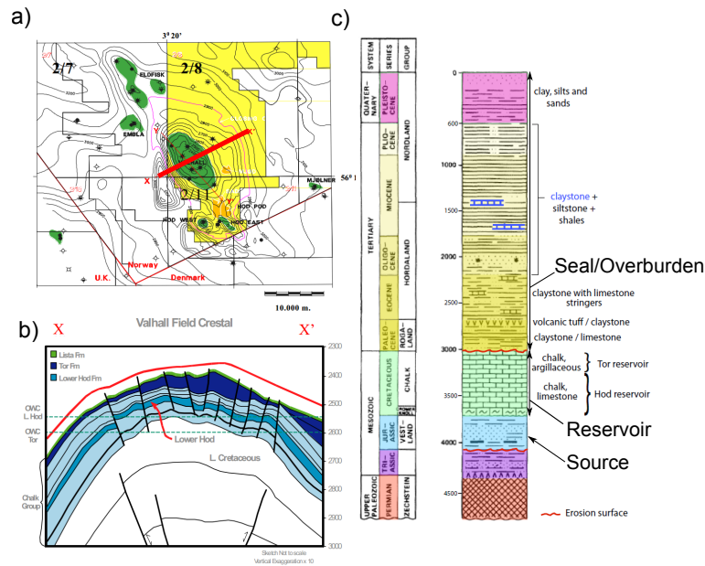
Figure 1.9: a) A contour map across the oil field with a WSW-ENE cross-section highlighted in red, b) The cross section shows the faulted structure of the Valhall oil field reservoir while the stratigraphy is described in the stratigraphic column c). Reproduced from Barkved et al. (2003).
