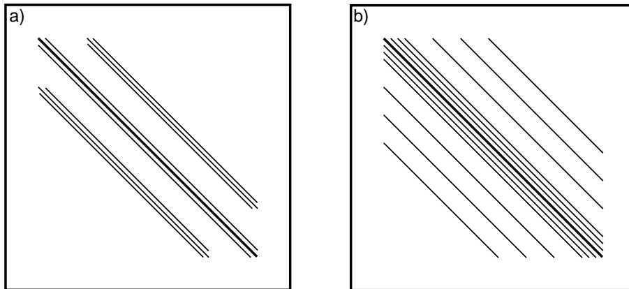
Figure 3.1: The sparsity of the real components of the complex impedance matrix \mathbf{B} (reproduced from Hustedt et al. (2004)). The impedance matrix is large with the dimension of (nx \times nz)^2 . The mixed stencil has only 9 \times nx \times nz non-zero entries a), while the fourth order staggered grid stencil b) requires 13 \times nx \times nz non-zero entries.
