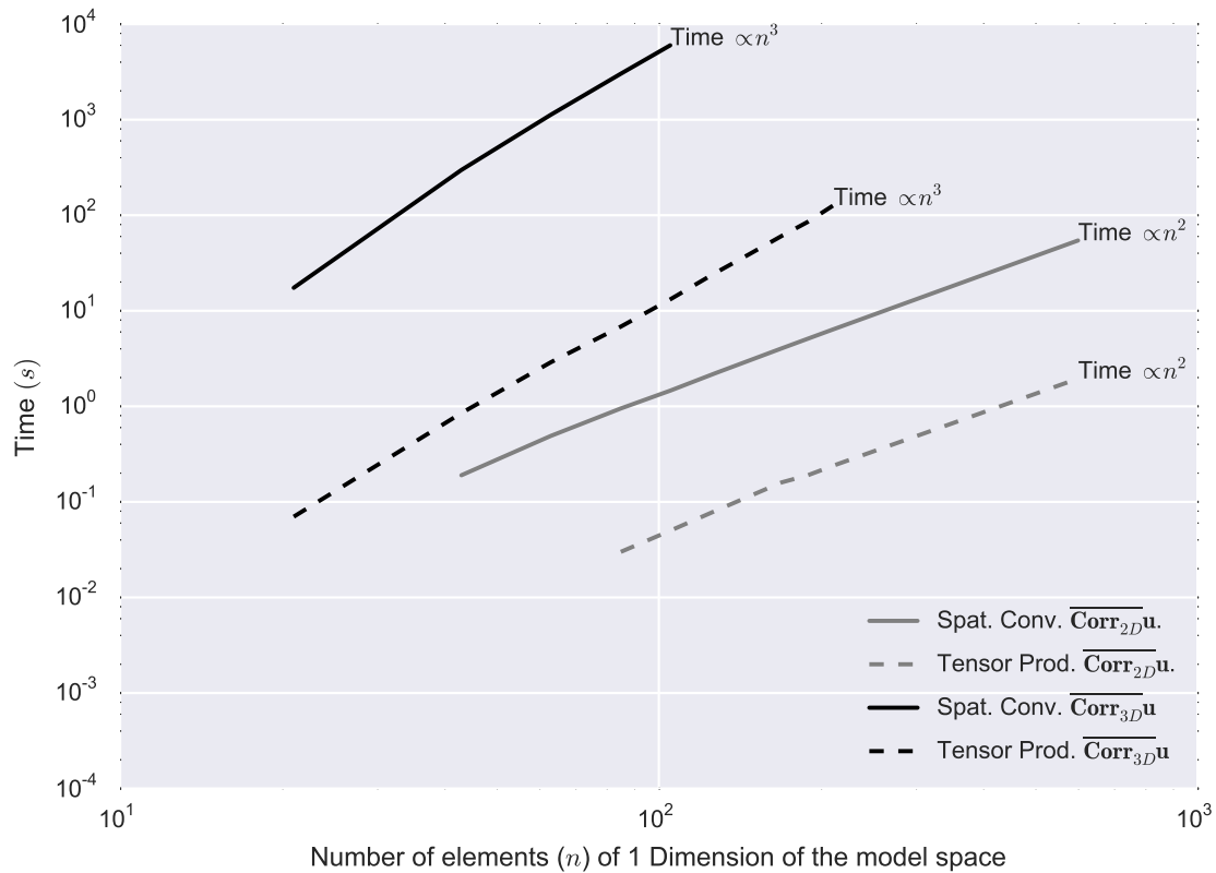
Figure 2.22: The time complexity for calculating \int_{\Omega_L} d\tau' \overline{\text{Corr}}(\mathbf{x}') \mathbf{u}(\mathbf{x}') in the 2D and 3D cases. The solid lines represents the cost for the spatial convolution approach. The dashed lines shows the equivalent cost for a tensorized operator.
