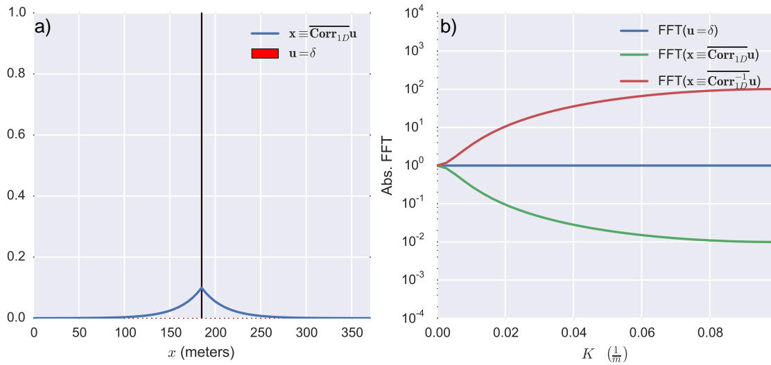
Figure 2.31: \overline{\mathbf{Corr}}_{1D}\mathbf{u} can be seen as a low-pass filter on the white unit-amplitude spectrum of \mathbf{u} . We can also calculate \overline{\mathbf{Corr}}_{1D}^{-1}\mathbf{u} . This operator can be seen to be the inverse low-pass filter. These filtering and inverse filtering operations are reversible, i.e. \overline{\mathbf{Corr}}_{1D}^{-1}(\overline{\mathbf{Corr}}_{1D}\mathbf{u}) = \mathbf{u} as well as \overline{\mathbf{Corr}}_{1D}(\overline{\mathbf{Corr}}_{1D}^{-1}\mathbf{u}) = \mathbf{u}
