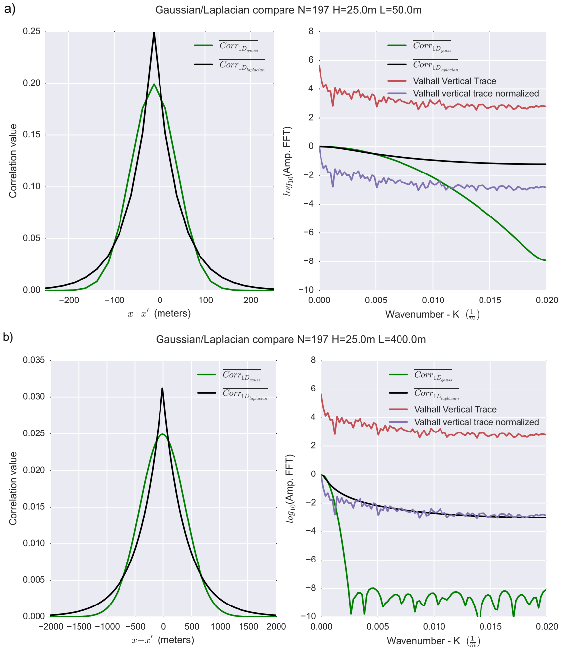
Figure 2.26: The 1D normalized Laplacian correlation operator \overline{Corr}_{1D} (black) and the 1D normalized Gaussian correlation operator \overline{Corr}_{1D_{GAUSSIAN}} (green). A short, 50 m correlation length a) is contrasted with a longer 400 m correlation length b). Note the Gaussian decays quite quickly. The Laplacian function decays more slowly as it is a "long-tailed" distribution. This means that although it decreases, it doesn't decrease at a rate much greater than is suggested by the geological model.
