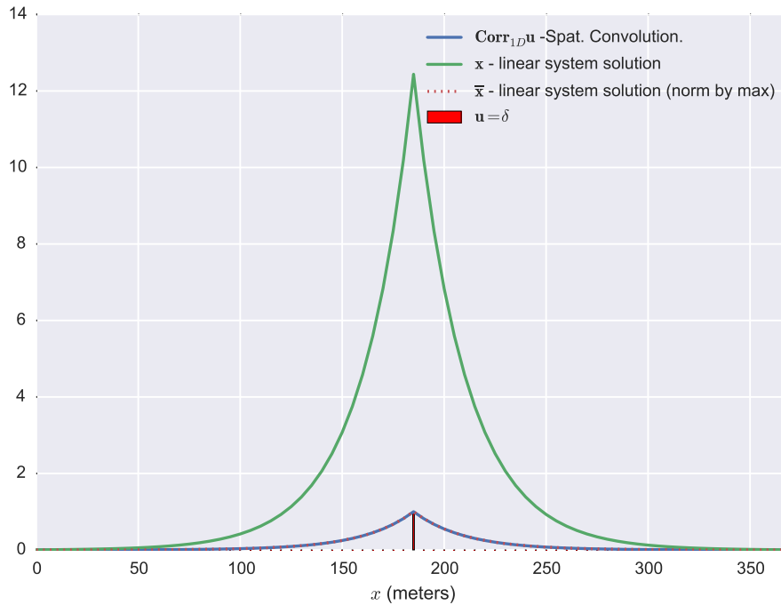
Figure 2.29: Comparison of the result from solving the sparse linear system ( \mathbf{x} ) vs the analytical result ( \mathbf{Corr}_{1D}\mathbf{u} ) calculated by spatial convolution. Note that \mathbf{x} has a much higher maximum value than what is suggested from \mathbf{Corr}_{1D}\mathbf{u} . If we compare \mathbf{x} when it is normalized by it's maximum value ( \bar{\mathbf{x}} ) it appears to be equivalent to \mathbf{Corr}_{1D}\mathbf{u} .
