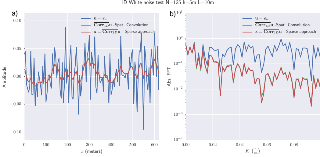
Figure 2.32: Comparison of calculating \overline{\text{Corr}}_{1D}^{-1}\mathbf{u} using the normalized 1D analytical correlation function (green) vs solving the linear system involving \overline{\text{Corr}}_{1D}^{-1} (red). We see that both results are close to identical and that application of the normalized Laplacian correlation function decreases the high-wavenumber content of the noise (shown in blue). a) Vectors in space domain b) Vectors in the wavenumber domain.
