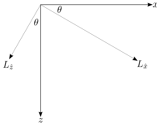
Figure 2.17: Rotated correlation length vectors. The angle, \theta rotates the Cartesian correlation lengths L_x and L_z to L_{\hat{x}} and L_{\hat{z}}
