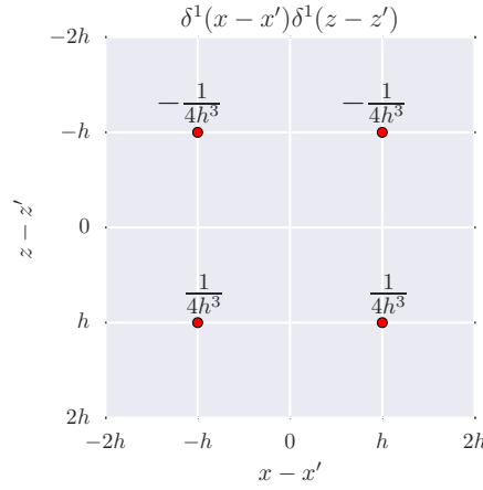
Figure 2.37: The discretization of \delta^1(x - x')\delta^1(z - z') using centred finite difference
