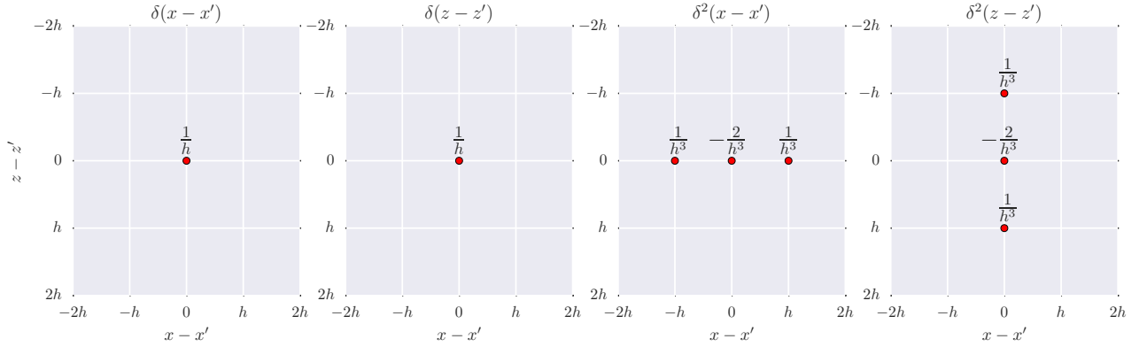
Figure 2.33: The discretization of \delta(x - x') , \delta(z - z') , \delta^2(x - x') and \delta^2(z - z') using centred finite differences
