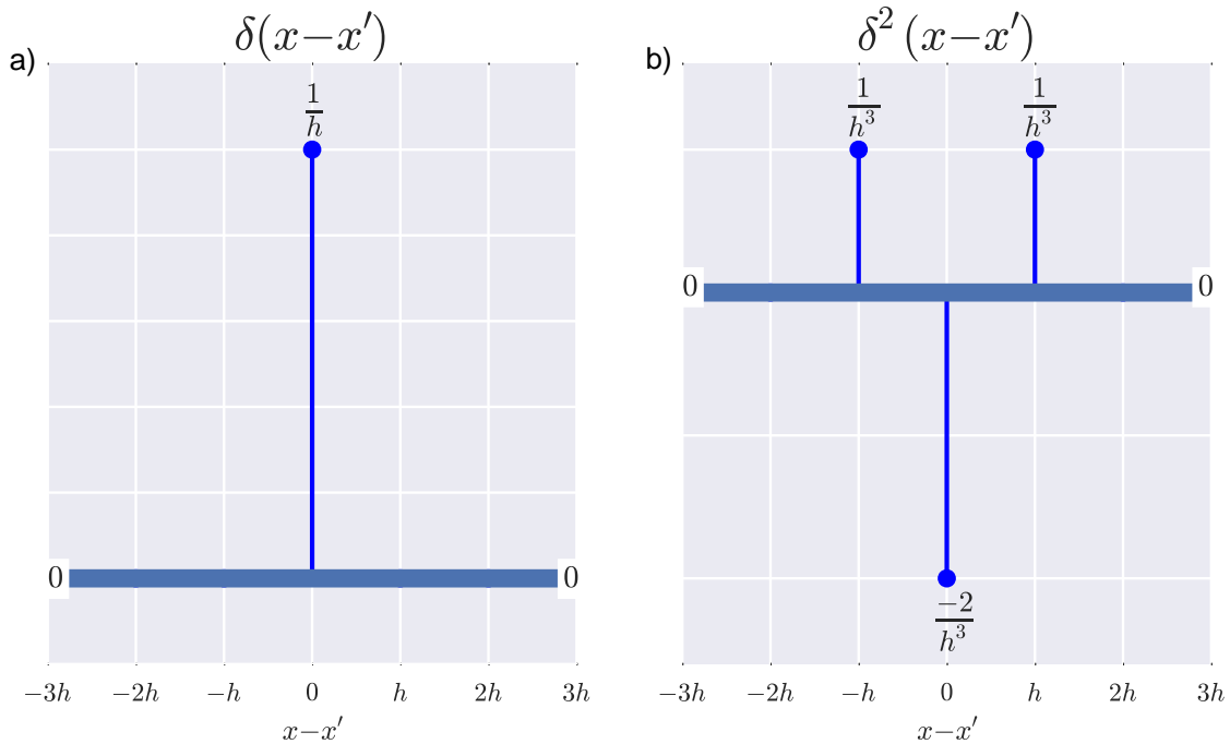
Figure 2.27: The finite discretization of a) \delta(x-x') and b) \delta^2(x-x') . This discretization means the operator \mathbf{Corr}^{-1} will be sparse and only require 3 non-zero elements per grid point.
