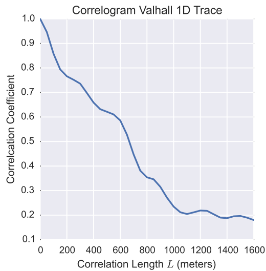
Figure 2.12: The correlation function calculated for increasing correlation length. Note when the correlation length L is zero, the correlation between the head and tail is equal to 1. As the correlation length increases this correlation coefficient decreases.
