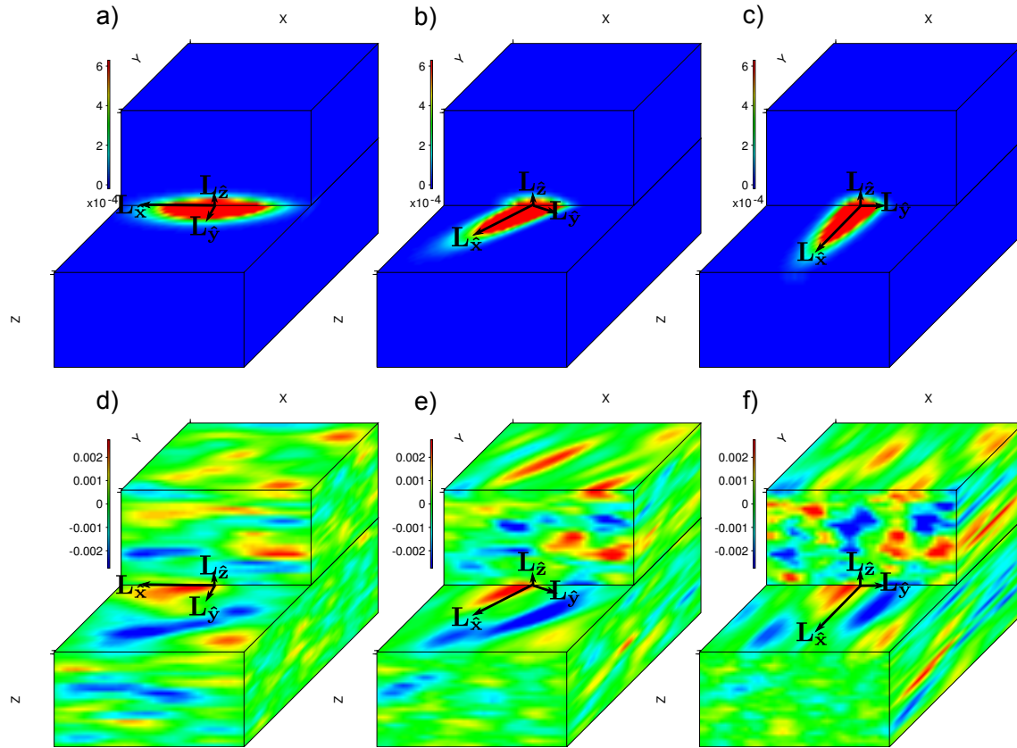
Figure 2.47: The calculation of \mathbf{x}_{3D_3} for two vectors, \mathbf{u} . with L_x = 6h , L_y = 2h and L_z = h . The input vectors for a-c) is a unit spike ( \mathbf{u} = \boldsymbol{\delta} ) and d-f) is a white noise vector ( \mathbf{u} = \boldsymbol{\epsilon}_w ). The correlation lengths are rotated around the z axis by the angle \varphi to become L_{\hat{x}} , L_{\hat{y}} and L_{\hat{z}} . a,d) \varphi = 0^\circ b,e) \varphi = 45^\circ c,f) \varphi = 90^\circ .
