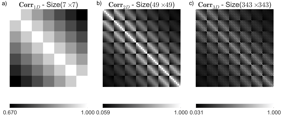
Figure 2.1: The correlation matrix describes how each point in the vector \mathbf{u} is related to every other point. a) The number of elements N in the correlation matrix for a 1D vector of length n = 7 ( N = n^2 ). b) The correlation matrix for a 2D vector with the dimensions 7 \times 7 ( N = n^4 ). c) The correlation matrix for a 3D vector with the dimensions 7 \times 7 \times 7 ( N = n^6 ).
