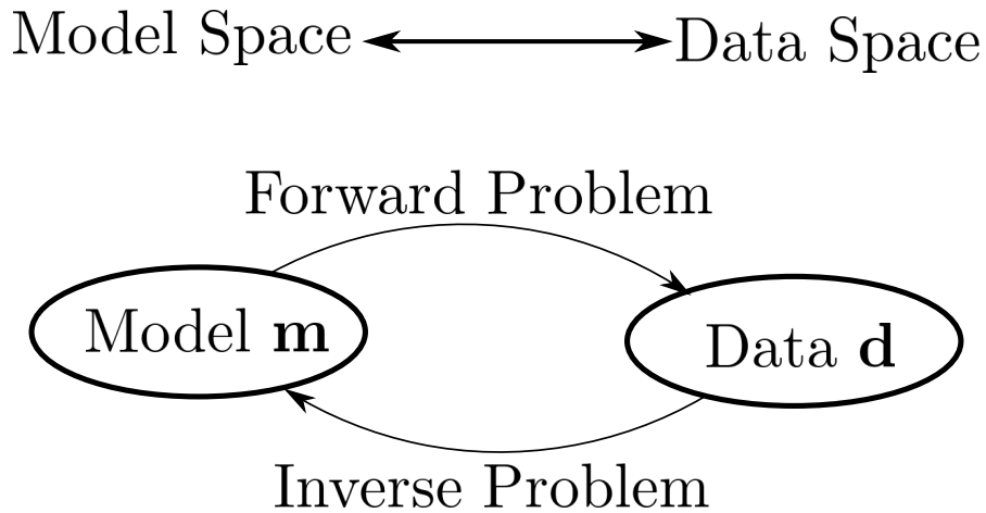
Figure 1.1: The transformation from the model space to the data space occurs from solving the often deterministic forward problem. Moving from the data space to the model space is referred to as the inverse problem
