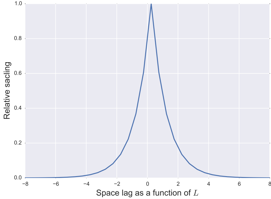
Figure 2.21: The rate of decay of the Laplacian correlation function. The space lag axis, represents the contribution of a point at x' to x for x' = x + N \times L . At 4L the scaling value is \approx 0.02
