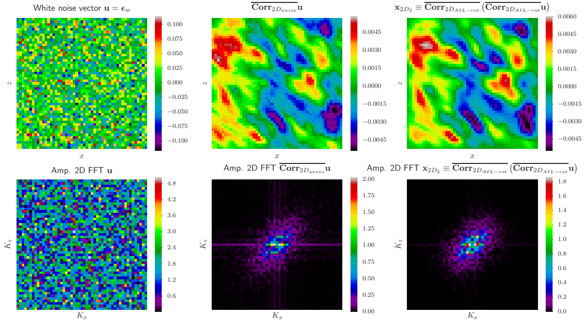
Figure 2.40: Application of the correlation operator to a white noise vector ( \mathbf{u} = \epsilon_w ) a). Comparison of \overline{\text{Corr}}_{2D_{aniso}} \mathbf{u} (b,e) and \mathbf{x}_{2D_2} (c,f). Note both results show similar features in the space domain (b,c) and in the 2D wavenumber domain (e,f).
