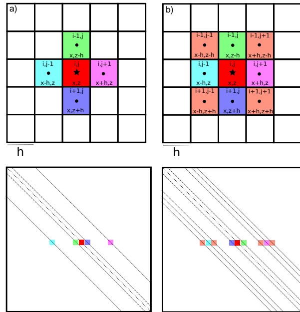
Figure 2.39: a) \overline{\text{Corr}}_{2D_{AIL}}^{-1} b) \overline{\text{Corr}}_{2D_{AIL-rot}}^{-1}
