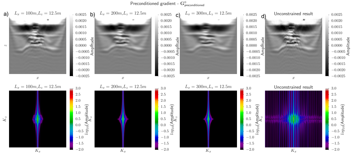
Figure 3.13: The sparse Laplacian preconditioned gradient \mathbf{G}_{\text{preconditioned}}^0 from the first iteration of FWI for the gradient preconditioning using a) L_x = 100 m, b) L_x = 200 m and c) L_x = 300 m compared to the d) unconstrained gradient \mathbf{G}_{\text{data}}^0 . The top row is the gradient in the space domain while the bottom row is in the wavenumber domain.
