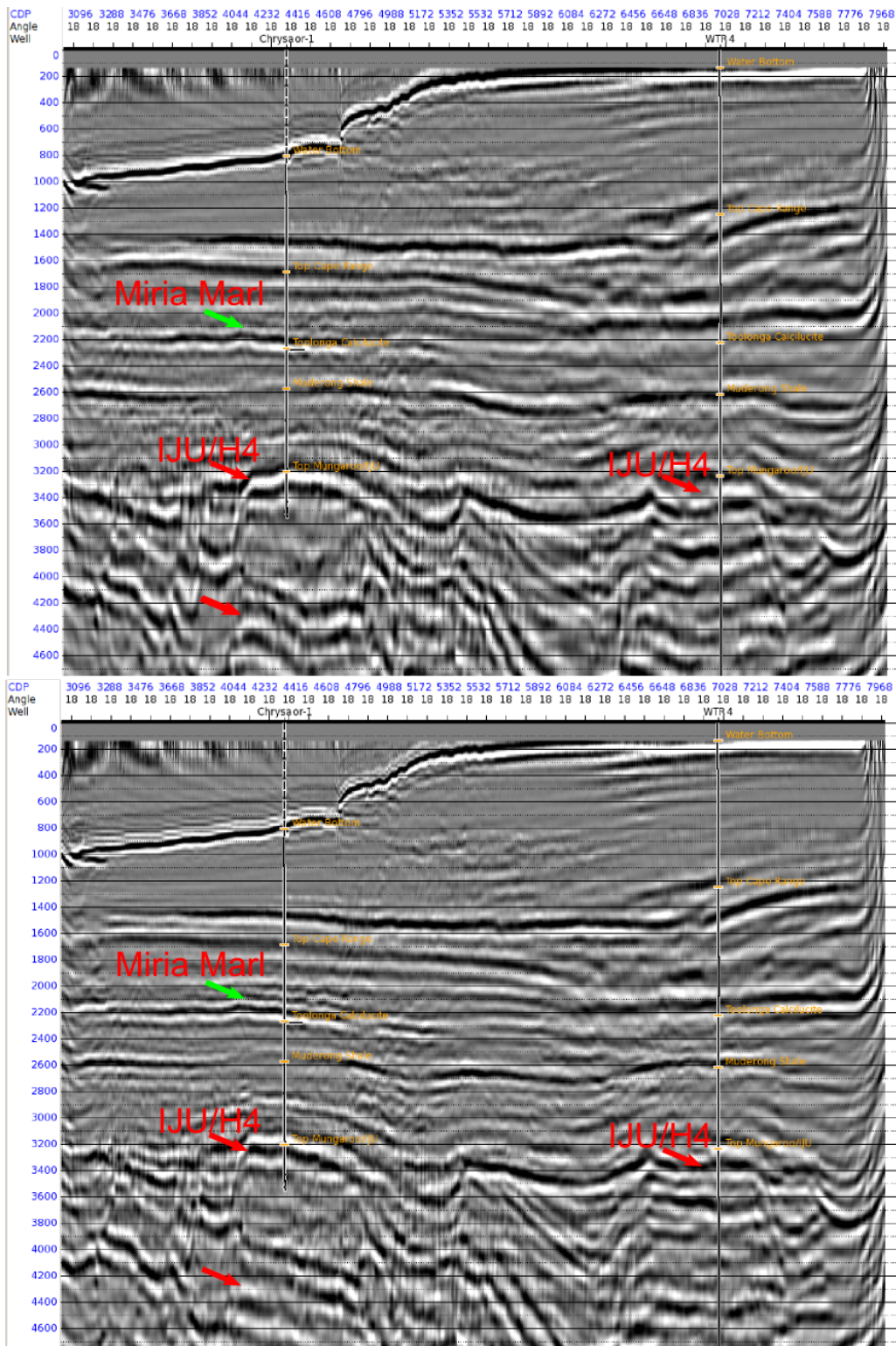
Figure 4.11: 0-30° stack computed using ( TOP ) crude initial model and ( BOTTOM ) the anisotropic reflection tomography model. The red arrows indicate where the reservoir structure is much more consistent with the WAPIMS interpretation report. A green arrow highlights the higher amplitude Miria Marl.
