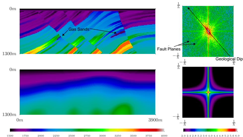
Figure 3.21: TOP : The true velocity model BOTTOM : The initial velocity model. The wavenumber spectrums for each velocity model are shown on the right. Notice there is significant intermediate/high wavenumber information missing from the initial model. When we look at the true model we see that unlike the Valhall synthetic model the wavenumber amplitude are not aligned in the vertical wavenumber orientation. The fault planes can be seen to be approximately orthogonal to this geological dip.
