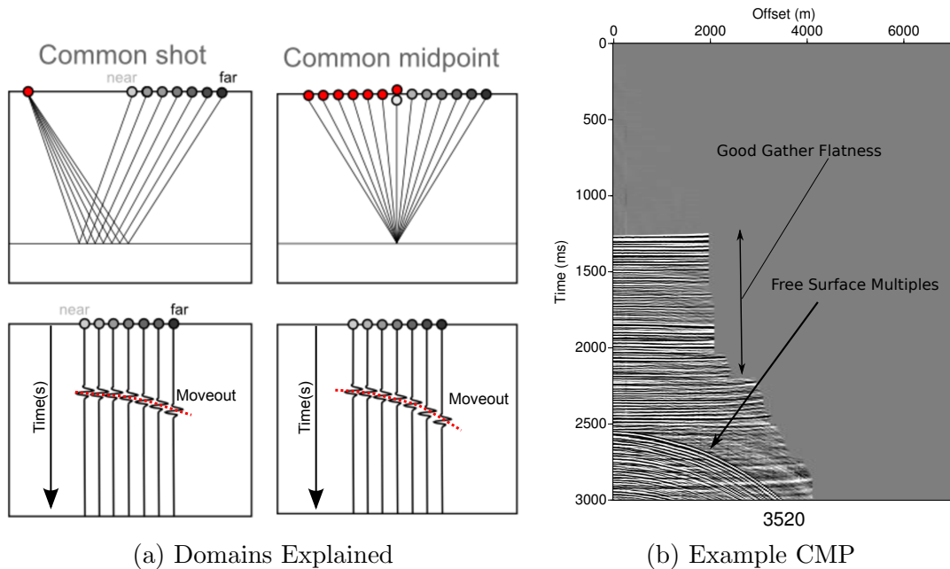
Figure 4.2: a) The common shot (CS) and common mid point (CMP) domains. In the common shot domain, seismic information is measured at offset receivers for a given shot (red), the mid point between source and receivers occur at a different positions in the earth. The CMP domain involves using sources and receivers pairs that share a common mid point. Notice that the wiggle plot also shows the associated travel-time. As source to receiver offset increases, this change in travel time is referred to as move-out. b) An example CMP from a deep-water section of the NWA-006 line that has been corrected for normal move-out. Super-critical reflections and transmitted waves have been removed. Notice many events are flat. A large amount of non-flat energy comes into the CMP at 2500 ms. This is the first water bottom multiple.
