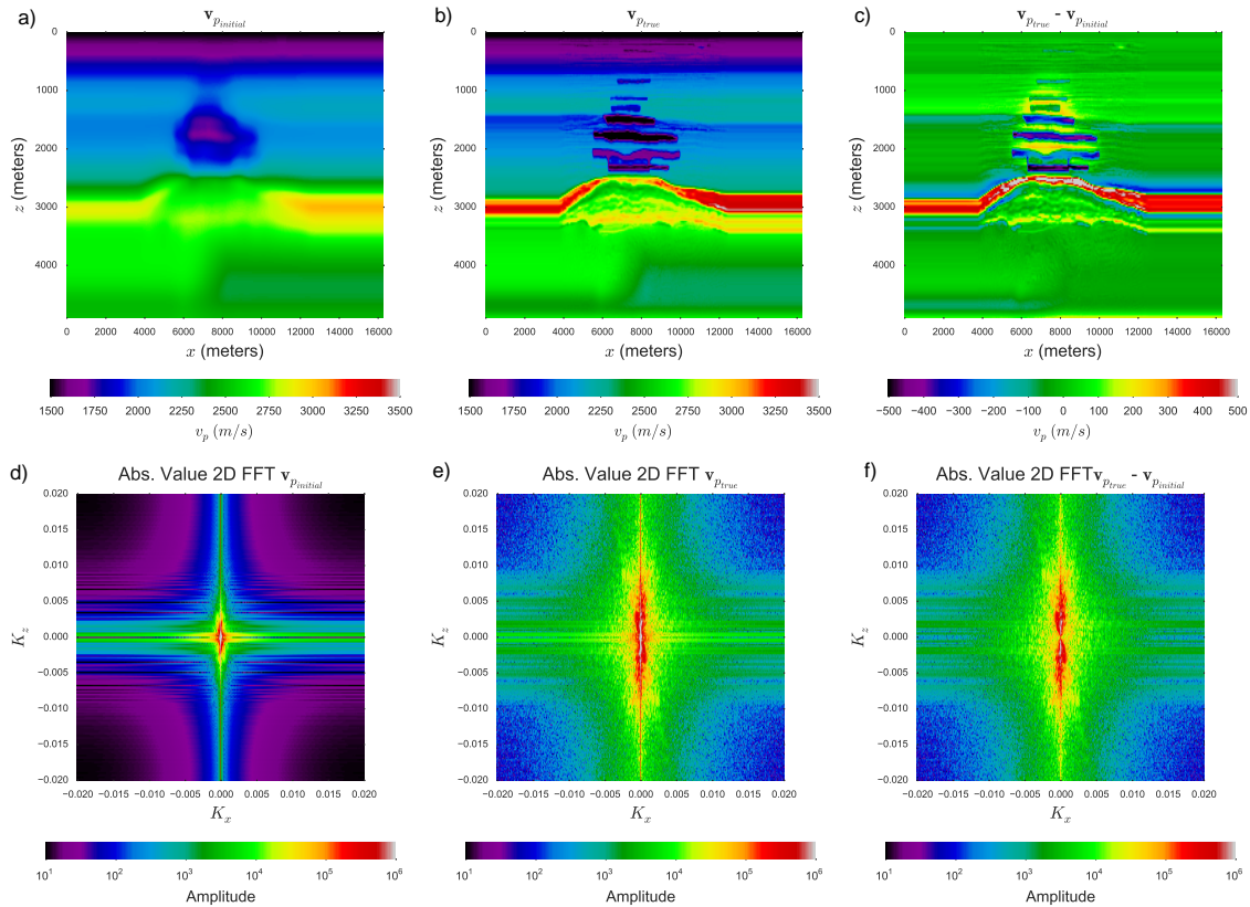
Figure 2.3: a) The initial velocity model ( \mathbf{v}_{p_{initial}} ) used for the Valhall synthetic FWI example. b) The true velocity model ( \mathbf{v}_{p_{true}} ) that we hope to recover from FWI c) The difference between the initial and true velocity model ( \mathbf{v}_{p_{true}} - \mathbf{v}_{p_{initial}} ). The bottom row shows the wavenumber spectrum for d) \mathbf{v}_{p_{initial}} e) \mathbf{v}_{p_{true}} f) \mathbf{v}_{p_{true}} - \mathbf{v}_{p_{initial}} .
