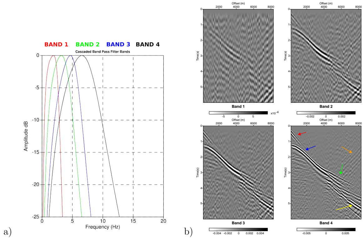
Figure 4.14: a) 4 Band pass filter bands to help asses signal to noise in different frequency ranges. A preprocessed shot record for the different frequency bands. Note the lower frequency bands have a lower signal to noise ratio than the higher bands. The coloured arrow highlight key seismic events. RED : The direct wave. BLUE : The water bottom reflection. GREEN : The first arrival. YELLOW : Post critical reflection events. ORANGE : Potentially noise from another survey.
