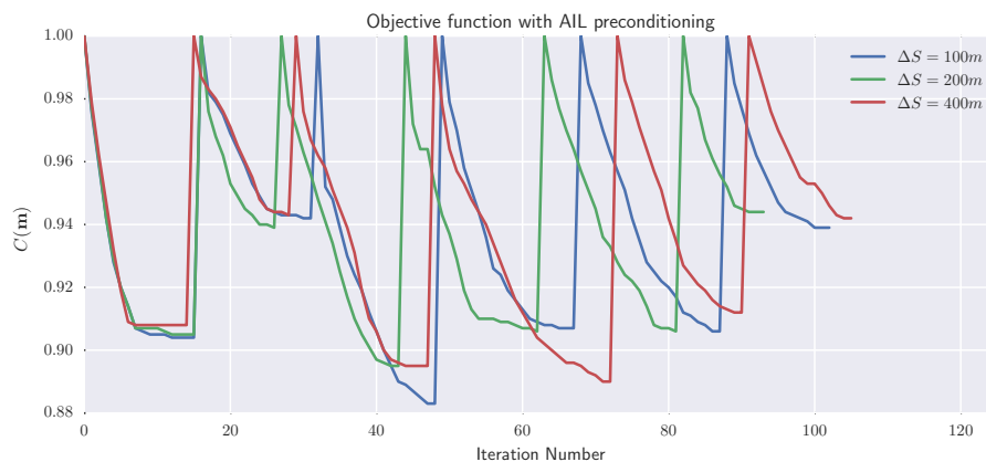
Figure 4.30: The evolution of the objective function for different levels of shot decimation when AIL preconditioning is applied
