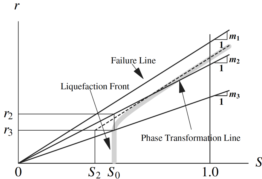
Fig. 1.9 Schematic plot of liquefaction front of Iai et al. (1990) [69] model in normalized stress space (after Iai et al., 1990 [69]). S holds for normalized mean effective stress and r is the normalized deviatoric stress.
