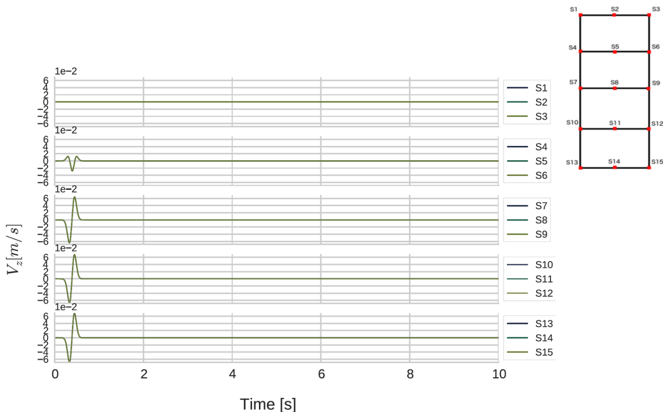
Fig. 4.23 Vertical velocity outputs for all the stations of P-SV wave propagation model with upward attenuation C-PML element.
