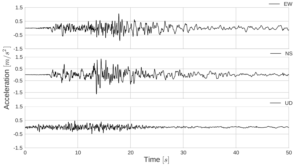
Fig. 3.3 Acceleration time histories at GL-7.5 m depth in east-west (EW), north-south (NS) and vertical (UD) directions recorded at WRLA.
