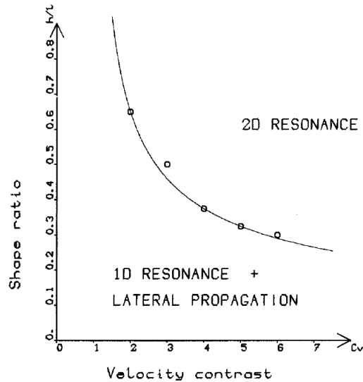
Fig. 5.2 Existence conditions of the two-dimensional (2D) resonance in the SH case (after Bard and Bouchon, 1985 [10]).
