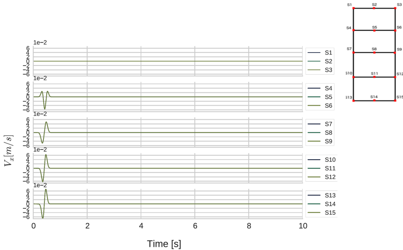
Fig. 4.22 Horizontal velocity outputs for all the stations of P-SV wave propagation model with upward attenuation C-PML element.
