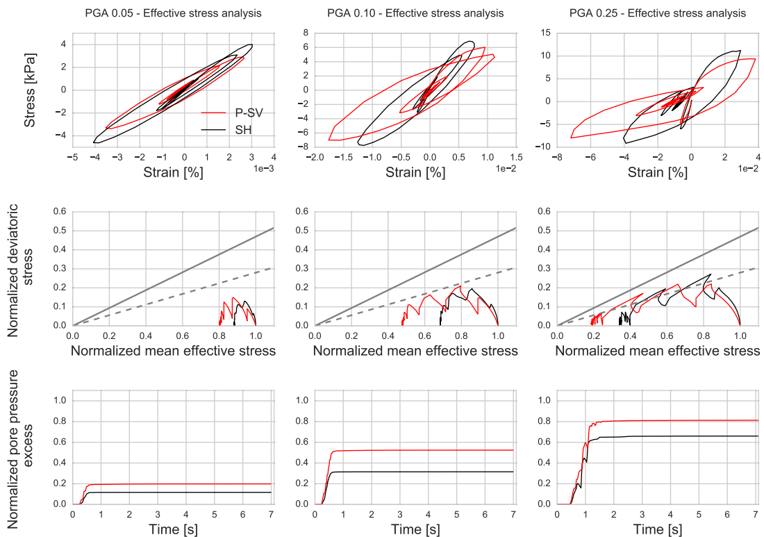
Fig. 5.31 Stress-strain curves at the middle of layer 1 ( z = -3.5m ) (top), stress path (middle) and temporal change of normalized pore pressure excess (bottom) for SH (in black) P-SV (in red) models under loading of impulse signal with PGA 0.05g (left), 0.10g (middle) and 0.25g (right).
