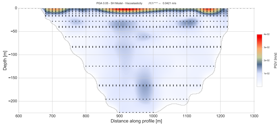
Fig. 5.16 Peak ground velocity distribution inside the viscoelastic basin media for SH model of the 2D sedimentary basin model under loading of impulse source with PGA 0.05g.
