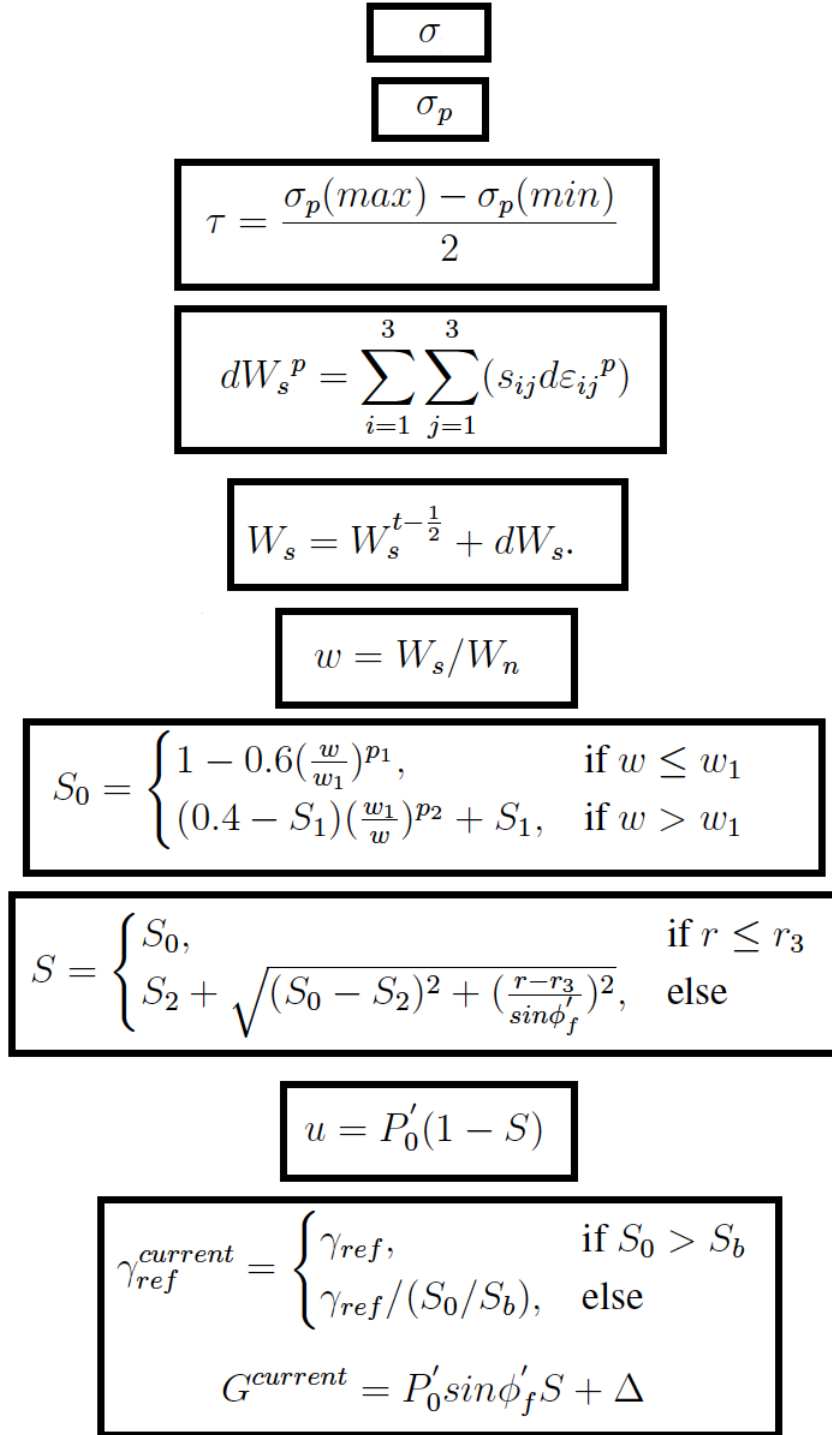
Fig. 1.10 Numerical flow followed for coupling of pore pressure effects and MPlI model.
