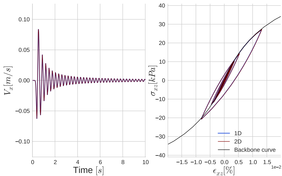
Fig. 4.32 Comparison of velocity outputs on x direction (left); comparison of stress-strain curves of xz component at midlayer (right) for 1D (in blue) and 2D (in red) SEM codes for pressure-independent nonlinear P1 model under biaxial loading.
