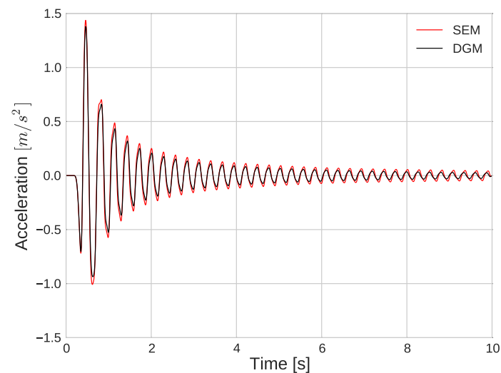
Fig. 2.13 Acceleration time histories at surface computed with SEM (in red) and DGM (in black) for the P1 model simulation under elastoplastic conditions.
