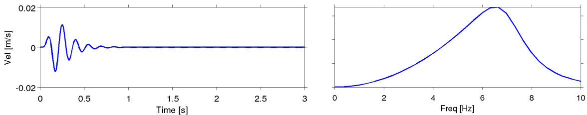
Figure 8: Input motion for the Volvi soil column: (left) velocity time history and (right) Fourier spectrum.
