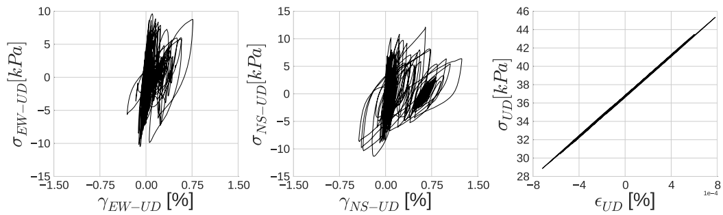
Fig. 3.36 Stress-strain curves on EW-UD component (left), NS-UD component (middle) and UD component (right) for point at GL-2.75 m of the OP.
