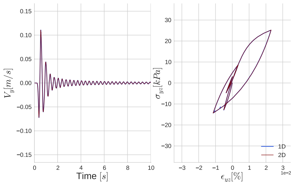
Fig. 4.43 Comparison of velocity outputs on y direction (left); comparison of stress-strain curves of yz component at midlayer (right) for 1D (in blue) and 2D (in red) SEM codes for pressure-dependent nonlinear P1 model under uniaxial loading effective stress analysis.
