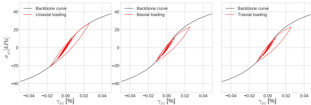
Fig. 3.1 Comparison of stress-strain curve for the P1 model under uniaxial loading (left), biaxial loading (middle) and triaxial loading (right). The backbone curve is shown in black.
