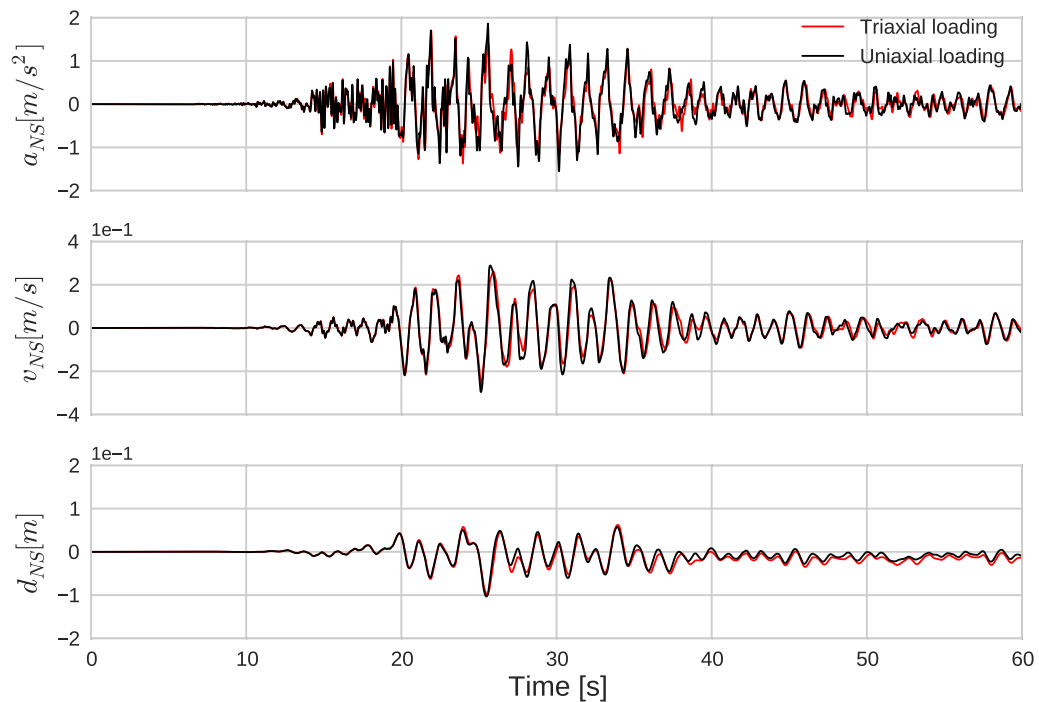
Fig. 3.28 Surface acceleration (top), velocity (middle) and displacement (bottom) comparison between uniaxial (in black) and triaxial (in red) loading for NS component.
