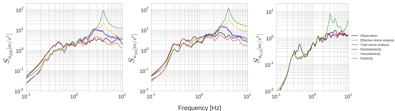
Fig. 3.12 Spectral acceleration comparison between elastic (in green), viscoelastic (in orange), elastoplastic (in purple), visco-elastoplastic with no excess pore pressure development (in blue) and visco-elastoplastic with excess pore pressure development (in red) models for three components.
