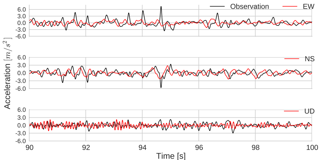
Fig. 3.33 Output acceleration time histories on [90-100] seconds time interval calculated in visco-elastoplastic model with excess pore pressure generation (in red) and real records (in black) of OP.
