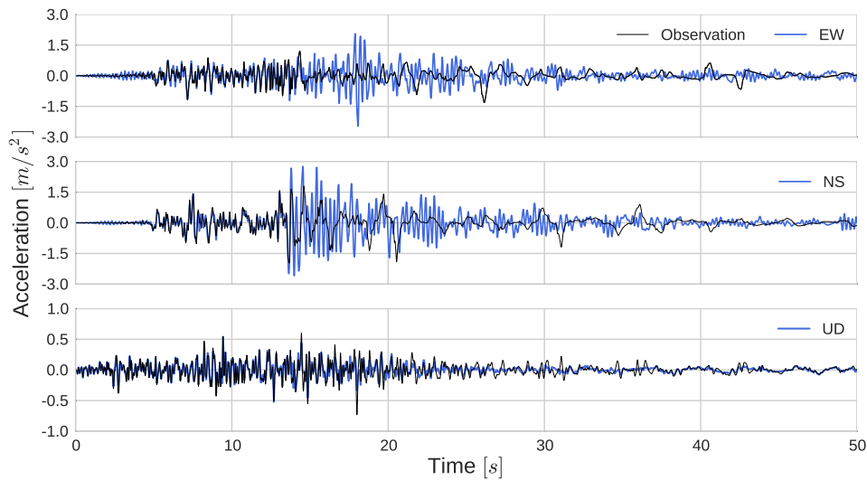
Fig. 3.9 Surface acceleration time histories on three directions for the simulation without pore pressure effects (in blue) and observation (in black) at the WRLA.
