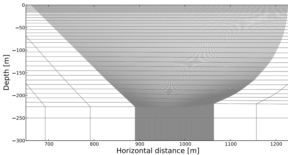
Fig. 5.7 2D mesh grid of the basin section of the 2D model .
