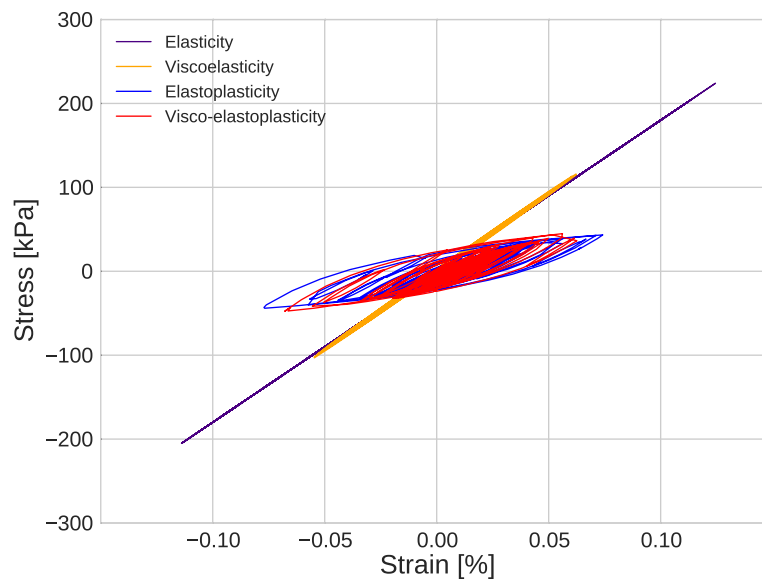
Fig. 2.19 Stress-strain curves for elasticity (in purple), viscoelasticity (in yellow), elastoplasticity (in blue) and visco-elastoplasticity (in red) for simulations under Real source #3 signal in the P1 model.
