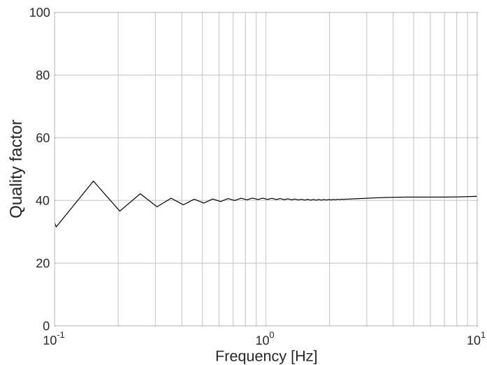
Fig. 2.3 Calculated quality factors for simulation with the Ricker source on the frequency band 0.1 - 10 Hz.
