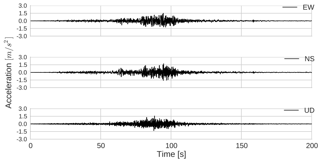
Fig. 3.31 Acceleration time histories at GL-11 m depth in east-west (EW), north-south (NS) and vertical (UD) directions recorded at OP.
