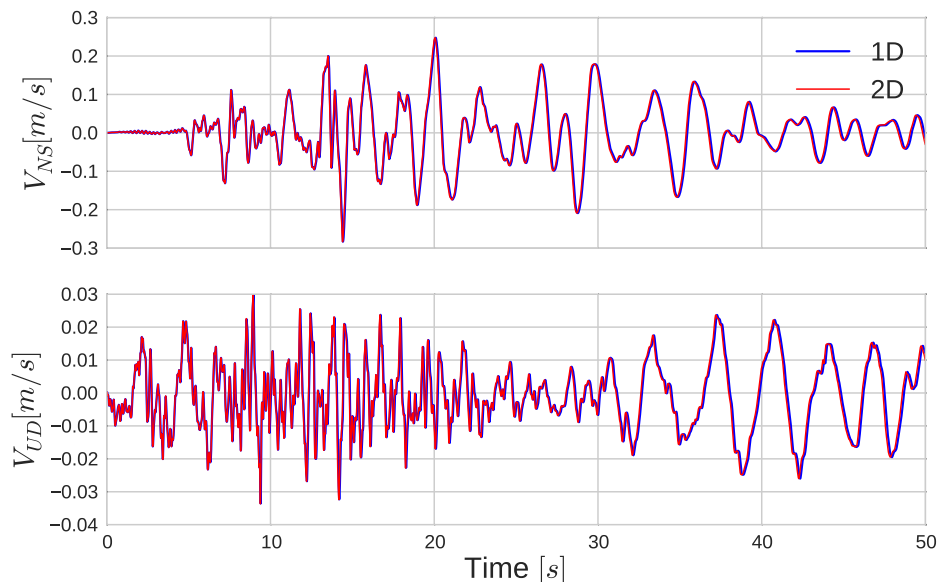
Fig. 4.47 Comparison of surface velocity outputs of WRLA model with single lateral element for NS (top) and for UD (bottom) directions between 1D (in blue) and 2D (in red) SEM codes.
