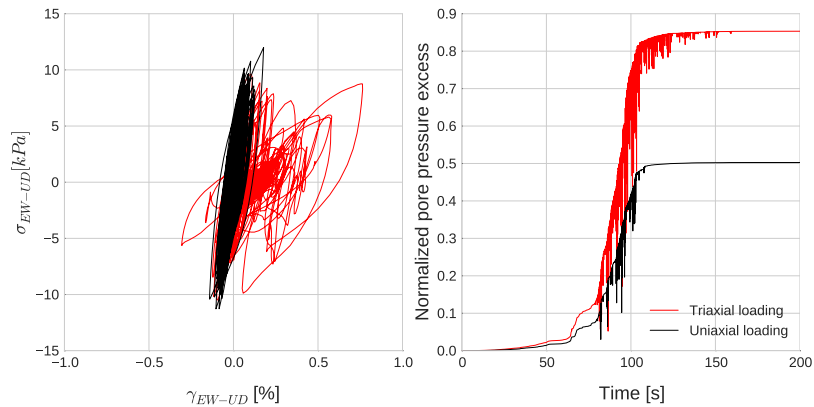
Fig. 3.45 (a) Stress-strain curve comparison between uniaxial (in black) and triaxial (in red) loading results for EW-UD component at GL-2.75 m, (b) Excess pore pressure vs time comparison between uniaxial (in black) and triaxial (in red) loading results at GL-2.75 m.
