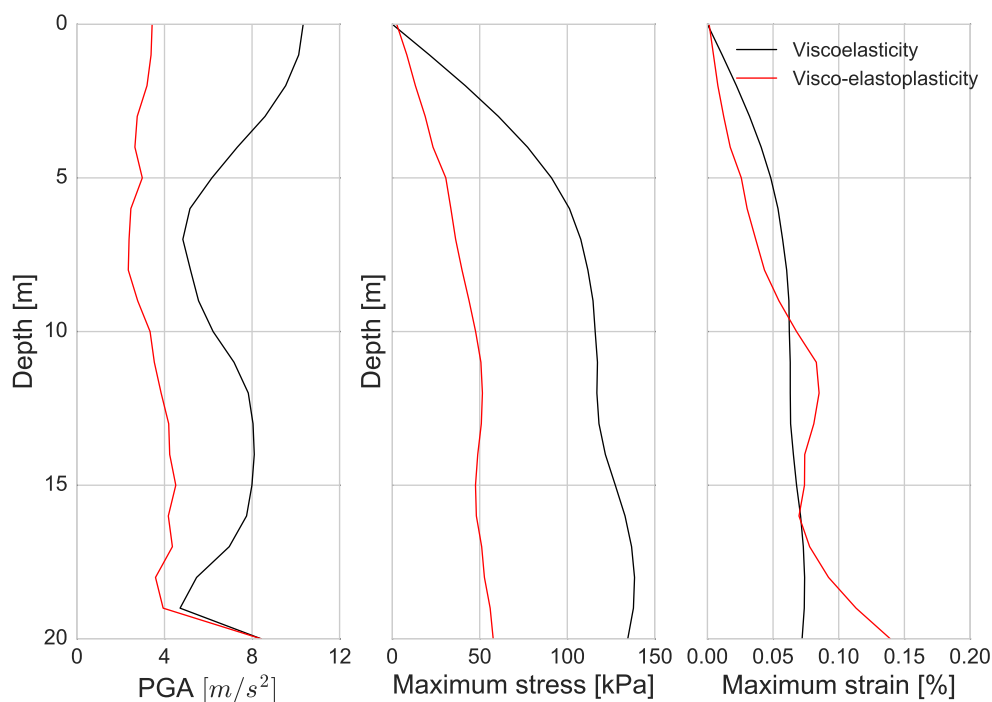
Fig. 2.21 Maximum PGA profile of P1 model under Real source #3 signal for viscoelasticity (in black) and visco-elastoplasticity (in red) (left); Maximum stress profile of P1 model under Real source #3 signal for viscoelasticity (in black) and visco-elastoplasticity (in red) (middle); Maximum strain profile of P1 model under Real source #3 signal for viscoelasticity (in black) and visco-elastoplasticity (in red) (right).
