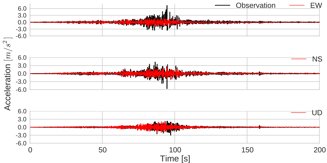
Fig. 3.32 Output acceleration time histories calculated in visco-elastoplastic model with excess pore pressure generation (in red) and real records (in black) of OP.
