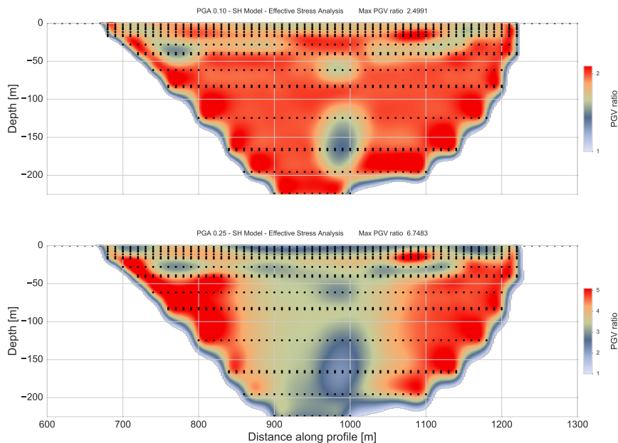
Fig. 5.21 Peak ground velocity ratio distribution of the basin for effective stress analysis of SH models of the 2D sedimentary basin model under loading of impulse source with PGA 0.10g (top) and 0.25g (bottom).
