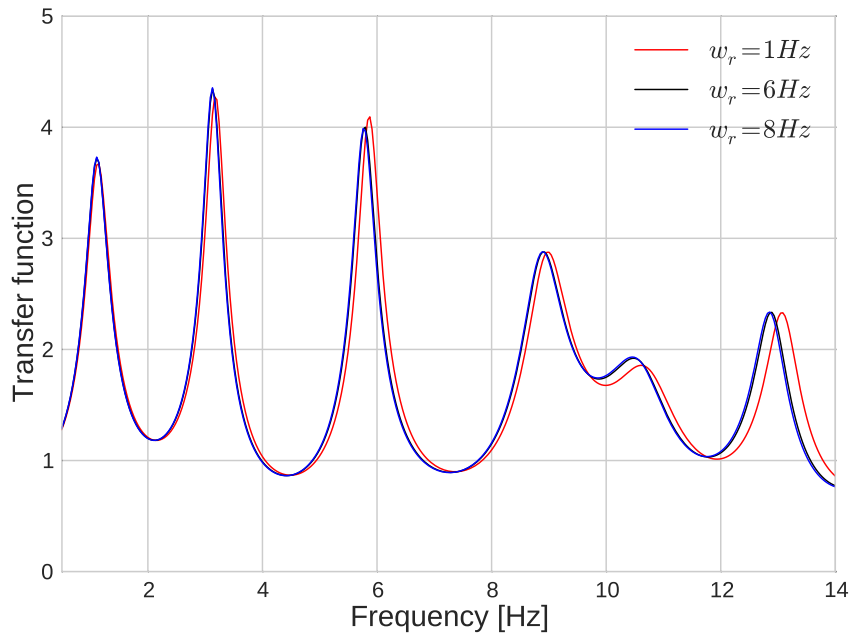
Fig. 2.8 Comparison between transfer functions obtained with SEM for models with reference frequency of 1 Hz (in red), 6 Hz (in black) and 8 Hz (in blue).
