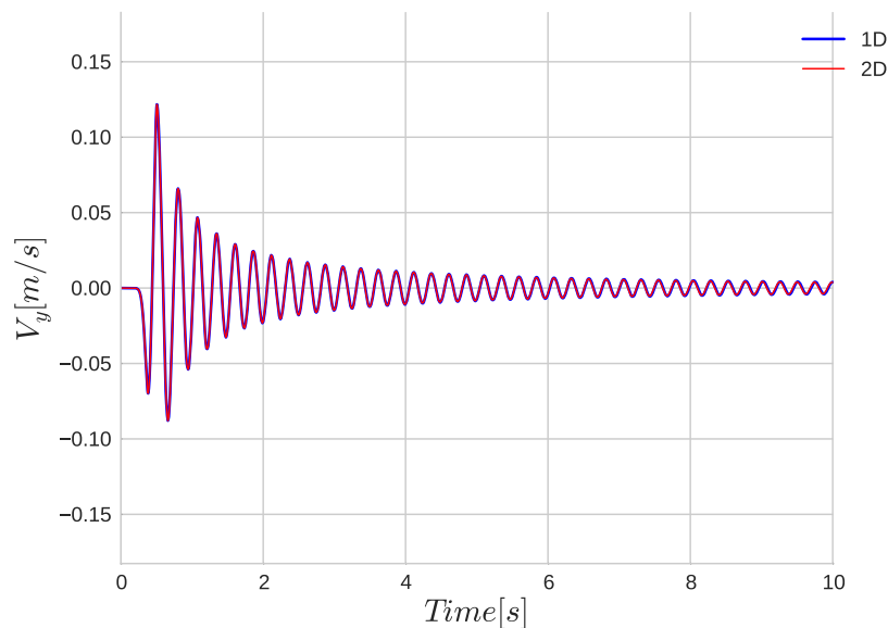
Fig. 4.40 Comparison of velocity outputs on y direction (at left); comparison of stress-strain curves of yz component at midlayer (at right) for 1D (in blue) and 2D (in red) SEM codes for pressure-dependent nonlinear P1 model with water table at midlayer under uniaxial loading.
