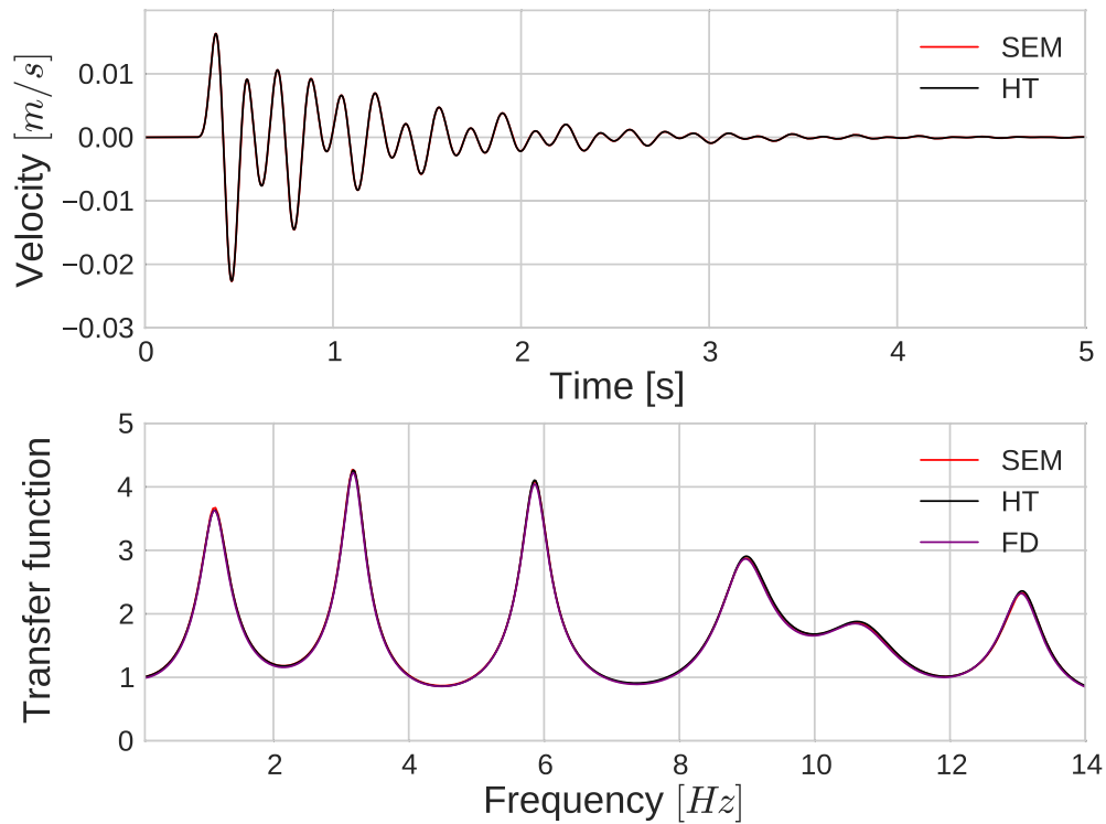
Fig. 2.6 Comparison between velocity time histories at surface from SEM (in red) and HT (in black) (top); Transfer functions obtained with SEM (in red), HT (in black) and FD (in purple) (bottom) for viscoelasticity.
