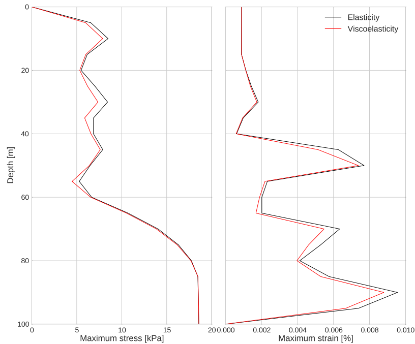
Fig. 2.7 Maximum stress profiles throughout the soil profile of Rome model for elasticity (in black) and viscoelasticity (in red) (left); Maximum strain profiles throughout the soil profile of Rome model for elasticity (in black) and viscoelasticity (in red) (right).
