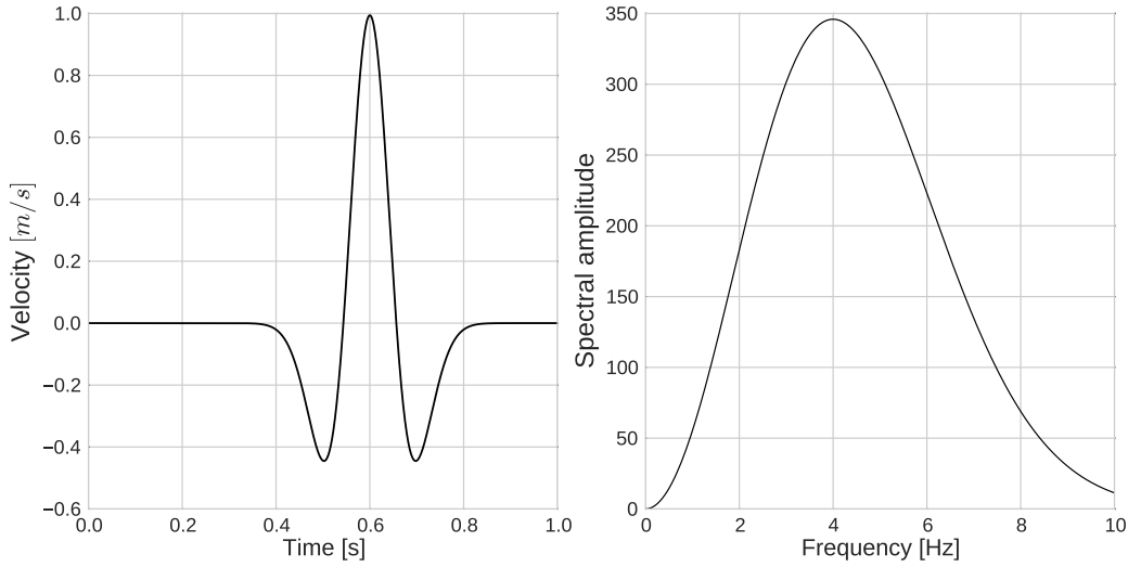
Fig. 2.2 Velocity time history of the Ricker source (left); Spectral amplitude of the Ricker source (right).
