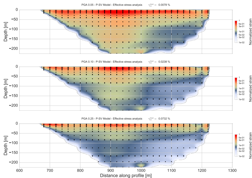
Fig. 5.26 Maximum strain distribution of the basin for xz component of effective stress analyses on P-SV models of the 2D sedimentary basin model under loading of impulse source with PGA 0.05g (top), PGA 0.10g (middle) and 0.25g (bottom).
