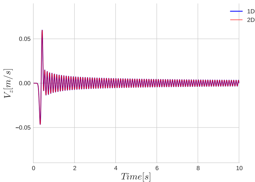
Fig. 4.33 Comparison of velocity outputs on z direction for 1D (in blue) and 2D (in red) SEM codes for pressure-independent nonlinear P1 model under biaxial loading.
