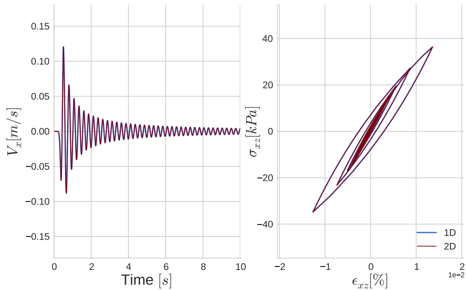
Fig. 4.38 Comparison of velocity outputs on x direction (left); comparison of stress-strain curves of xz component at midlayer (right) for 1D (in blue) and 2D (in red) SEM codes for pressure-dependent nonlinear P1 model with water table at midlayer under biaxial loading.
