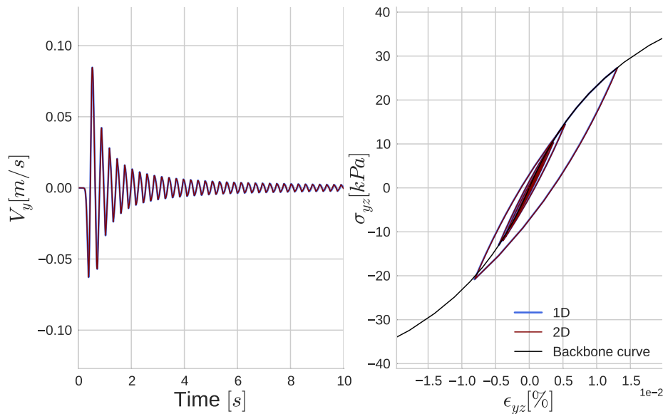
Fig. 4.34 Comparison of velocity outputs on y direction (at left); comparison of stress-strain curves of yz component at midlayer (at right) for 1D (in blue) and 2D (in red) SEM codes for stress-independent nonlinear P1 model under uniaxial loading.
