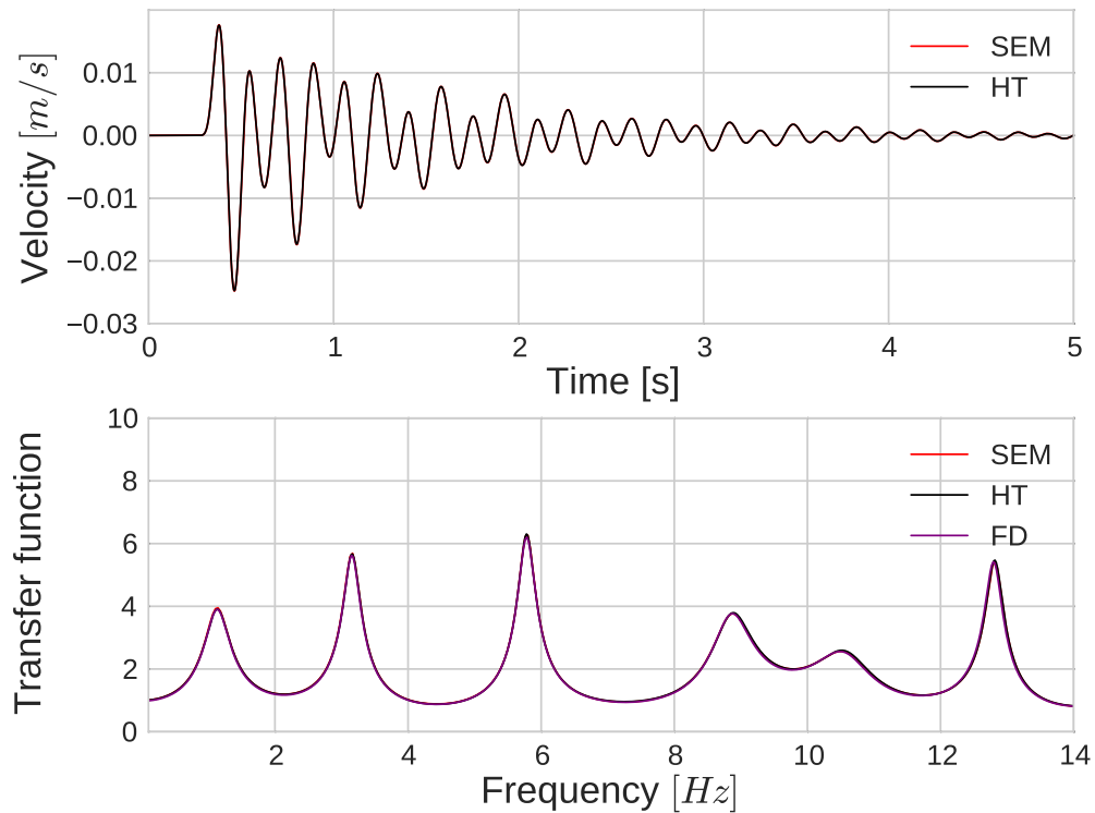
Fig. 2.5 Comparison between velocity time histories at surface from SEM (in red) and HT (in black) (top); Transfer functions obtained with SEM (in red), HT (in black) and FD (in purple) (bottom) for elasticity.
