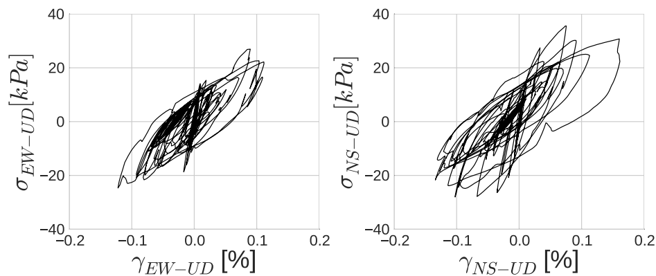
Fig. 3.22 Stress-strain curves on EW-UD component (left) and NS-UD component (right) for point at GL-15 m of the KP.
