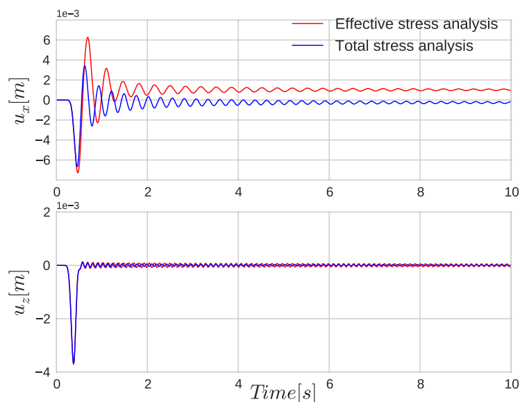
Fig. 4.44 Comparison of ground surface displacements on x direction (top) and on z direction (bottom) for total stress analysis (in blue) and effective stress analysis (in red) in 2D P1 nonlinear model.
