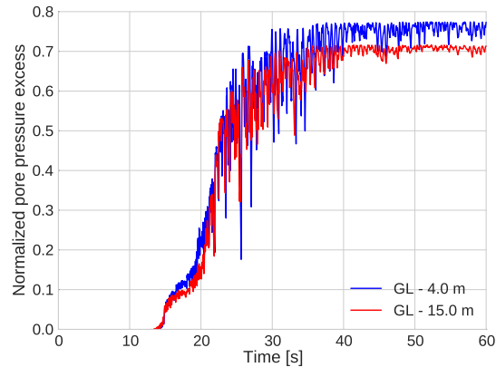
Fig. 3.19 Pore pressure excess temporal change for the point at GL-4.0 m (in blue) and for the point at GL-15.0 m (in red) of the KP.
