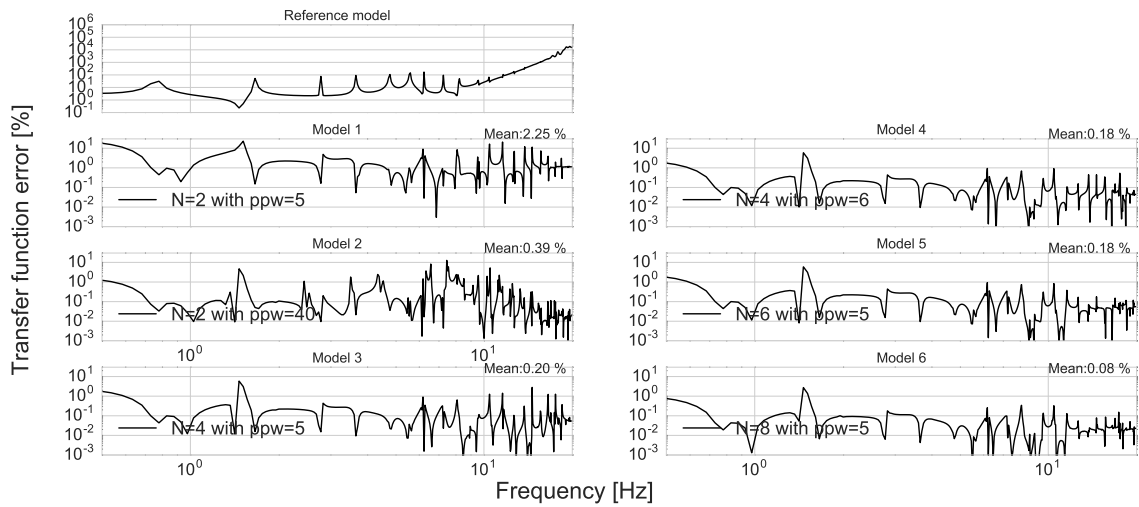
Fig. 2.23 Relative error in frequency domain for the solutions of all the models.
