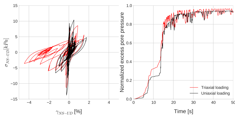
Fig. 3.15 (a) Stress-strain curve comparison between uniaxial (in black) and triaxial (in red) loading results for NS-UD component at GL-4.0 m; (b) Pore pressure excess temporal change comparison between uniaxial (in black) and triaxial (in red) loading results at GL-4.0 m.
