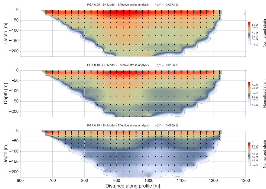
Fig. 5.20 Maximum strain distribution of the basin for yz component of effective stress analyses on SH models on the 2D sedimentary basin model under loading of impulse source with PGA 0.05g (top), PGA 0.10g (middle) and 0.25g (bottom).
