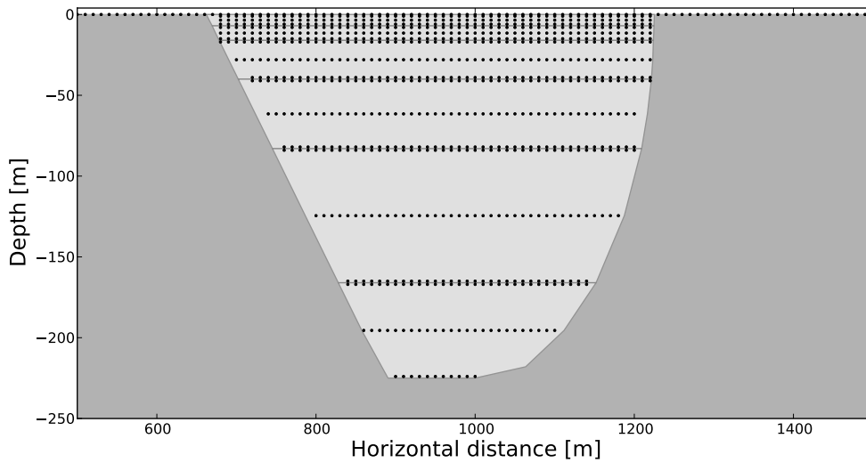
Fig. 5.8 Velocity receivers located on the 2D model.
