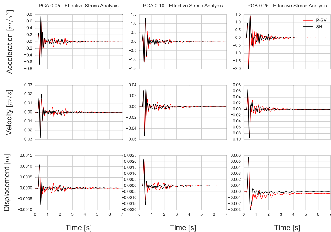
Fig. 5.32 Acceleration (top), velocity (middle) and displacement (bottom) time histories for effective stress analyses in SH (in black) and P-SV (in red) models under loading of impulse signal with PGA 0.05\text{g} (left), 0.10\text{g} (middle) and 0.25\text{g} (right).
