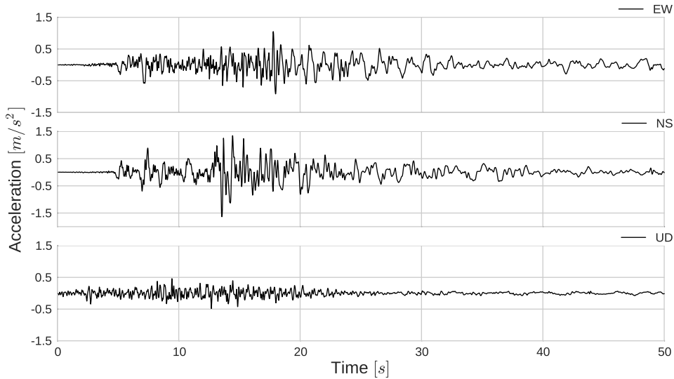
Fig. 3.3 Acceleration time histories at GL-7.5 m depth in east-west (EW), north-south (NS) and vertical (UD) directions recorded at WRLA.
