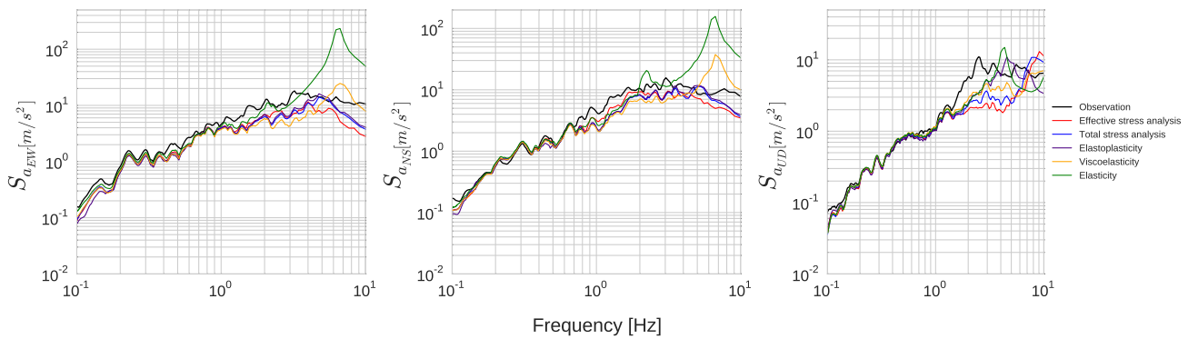
Fig. 3.41 Spectral acceleration comparison between elastic (in green), viscoelastic (in orange), elastoplastic (in purple), visco-elastoplastic with no excess pore pressure development (in blue) and visco-elastoplastic with excess pore pressure development (in red) models for three components of Kushiro Port site.
