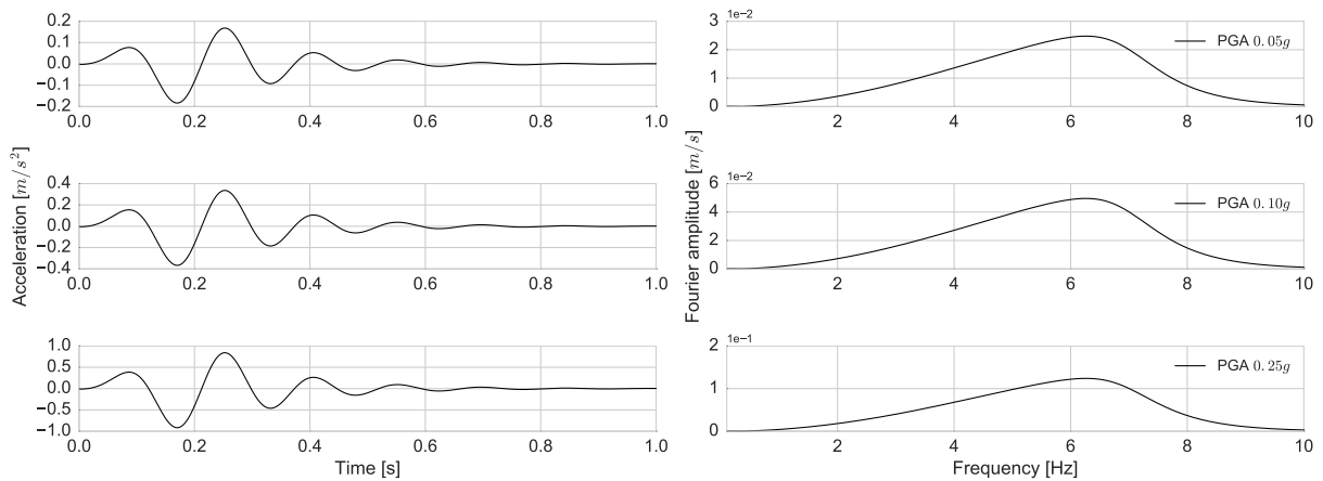
Fig. 5.10 Acceleration time histories (left column) and Fourier amplitudes (right column) of impulse sources with PGA 0.05g (top), PGA 0.10g (middle) and PGA 0.25g (bottom).
