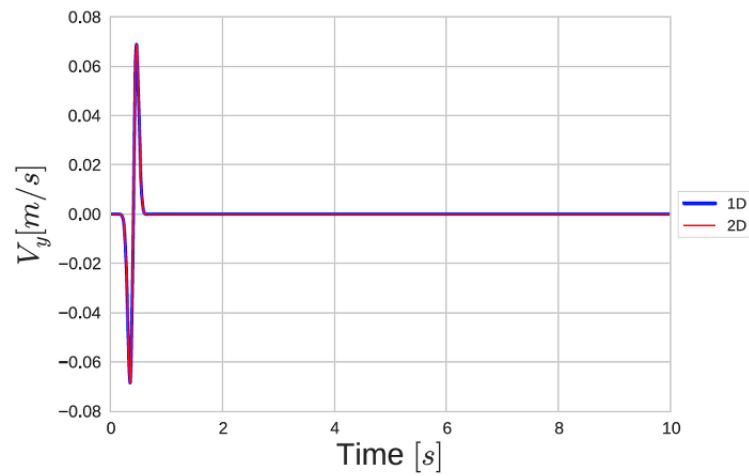
Fig. 4.16 Comparison of velocity outputs on horizontal direction of SH wave propagation model with single-element C-PML between 1D (in blue) and 2D (in red) SEM codes.
