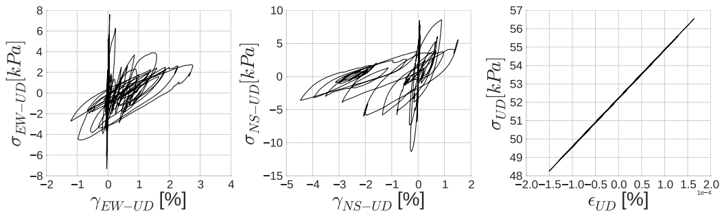
Fig. 3.7 Stress-strain curves on EW-UD component (left), NS-UD component (middle) and UD component (right) for point at GL-4.0 m of the WRLA.
