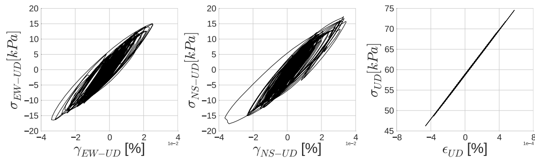
Fig. 3.37 Stress-strain curves on EW-UD component (left), NS-UD component (middle) and UD component (right) for point at GL-5 m of the OP.
