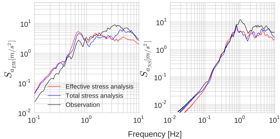
Fig. 3.24 Acceleration spectra of recorded surface acceleration (in black), visco-elastoplastic SEM simulation with excess pore pressure development (in red) and without excess pore pressure development (in blue) for EW component (left); for NS component (right)
