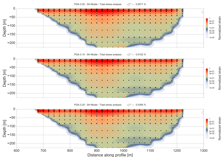
Fig. 5.17 Maximum strain distribution of the basin for yz component of total stress analyses on SH models on the 2D sedimentary basin model under loading of impulse source with PGA 0.05g (top), PGA 0.10g (middle) and 0.25g (bottom).
