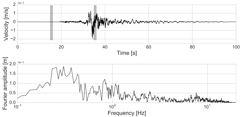
Fig. 2.14 Velocity time histories of Real source #3 signal where [15 - 16]s and [35 - 36]s time intervals are shaded (top); Fourier amplitude (bottom) of Real source #3 signal.
