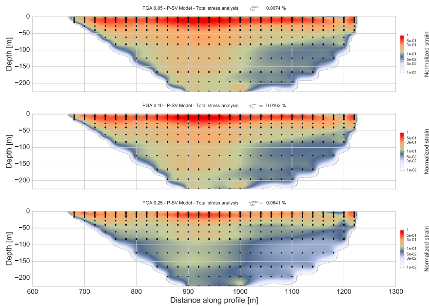
Fig. 5.23 Maximum strain distribution of the basin for xz component of total stress analyses on P-SV models of the 2D sedimentary basin model under loading of impulse source with PGA 0.05g (top), PGA 0.10g (middle) and 0.25g (bottom).
