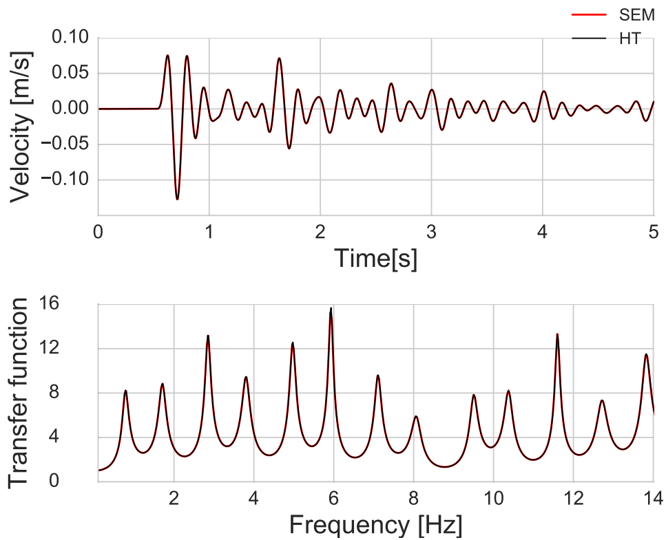
Fig. 2.9 Comparison between velocity time histories at surface obtained with SEM (in red) and HT (in black) (top); transfer functions obtained with SEM (in red) and HT (in black) (bottom) for elasticity.
