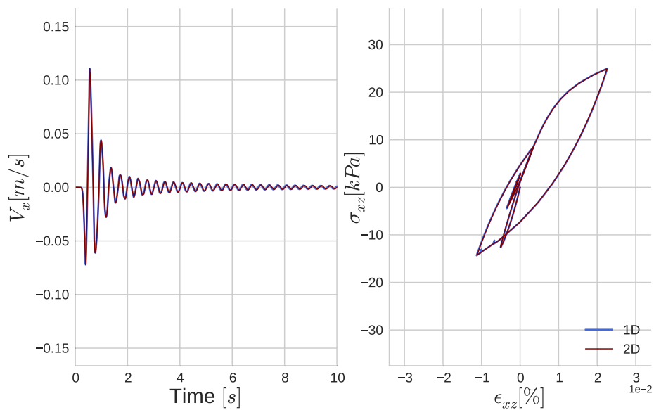
Fig. 4.41 Comparison of velocity outputs on x direction (left); comparison of stress-strain curves of xz component at midlayer (right) for 1D (in blue) and 2D (in red) SEM codes for pressure-dependent nonlinear P1 model under biaxial loading effective stress analysis.
