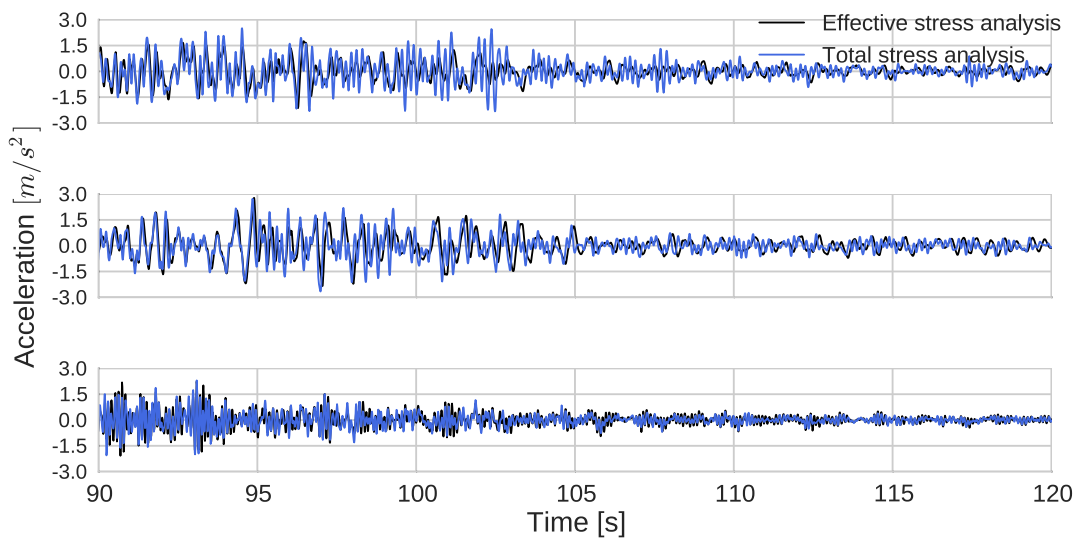
Fig. 3.38 Surface acceleration time histories on [90-120] seconds time interval for three directions for the simulation without pore pressure effects (in blue) and with pore pressure effects (in black) at the OP.
