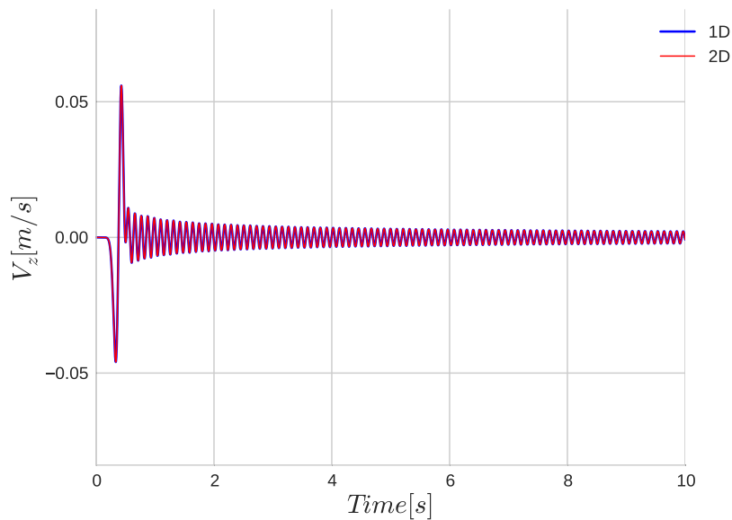
Fig. 4.36 Comparison of velocity outputs on z direction for 1D (in blue) and 2D (in red) SEM codes for pressure-dependent nonlinear P1 model with water table at surface level under biaxial loading.
