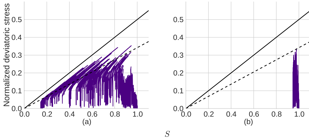
Fig. 3.35 (a) Deviatoric plan for point at GL-2.75 m, (b) Deviatoric plan for point at GL-5 m of the OP model with failure line (solid line) and phase transformation line (dashed line).
