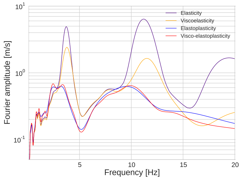
Fig. 2.16 Fourier amplitudes of surface velocities for elasticity (in purple), viscoelasticity (in yellow), elastoplasticity (in blue) and visco-elastoplasticity (in red) for simulations under Real source #3 signal in the P1 model.
