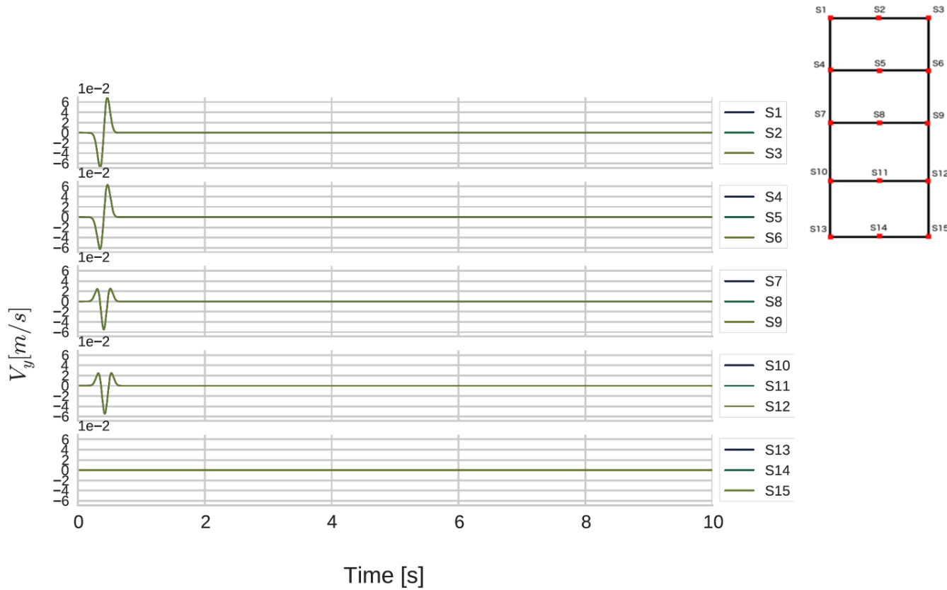
Fig. 4.15 Horizontal velocity outputs for all the stations of SH wave propagation model with single-element C-PML model.
