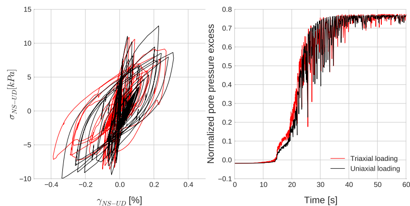
Fig. 3.29 (a) Stress-strain curve comparison between uniaxial (in black) and triaxial (in red) loading results for NS-UD component at GL-4 m, (b) Excess pore pressure vs time comparison between uniaxial (in black) and triaxial (in red) loading results at GL-4 m.
