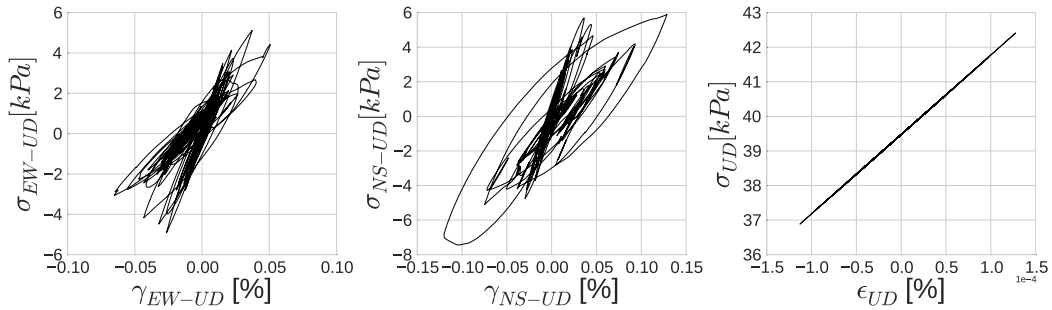
Fig. 3.6 Stress-strain curves on EW-UD component (left), NS-UD component (middle) and UD component (right) for point at GL-2.9 m of the WRLA.
