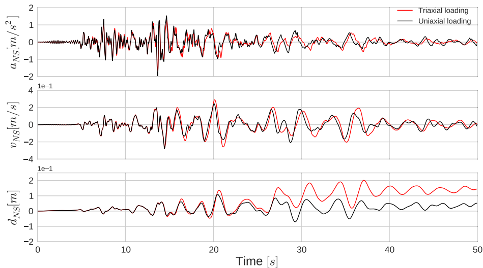
Fig. 3.14 Surface acceleration (top), velocity (middle) and displacement (bottom) comparison between uniaxial (in black) and triaxial (in red) loading for NS component.
