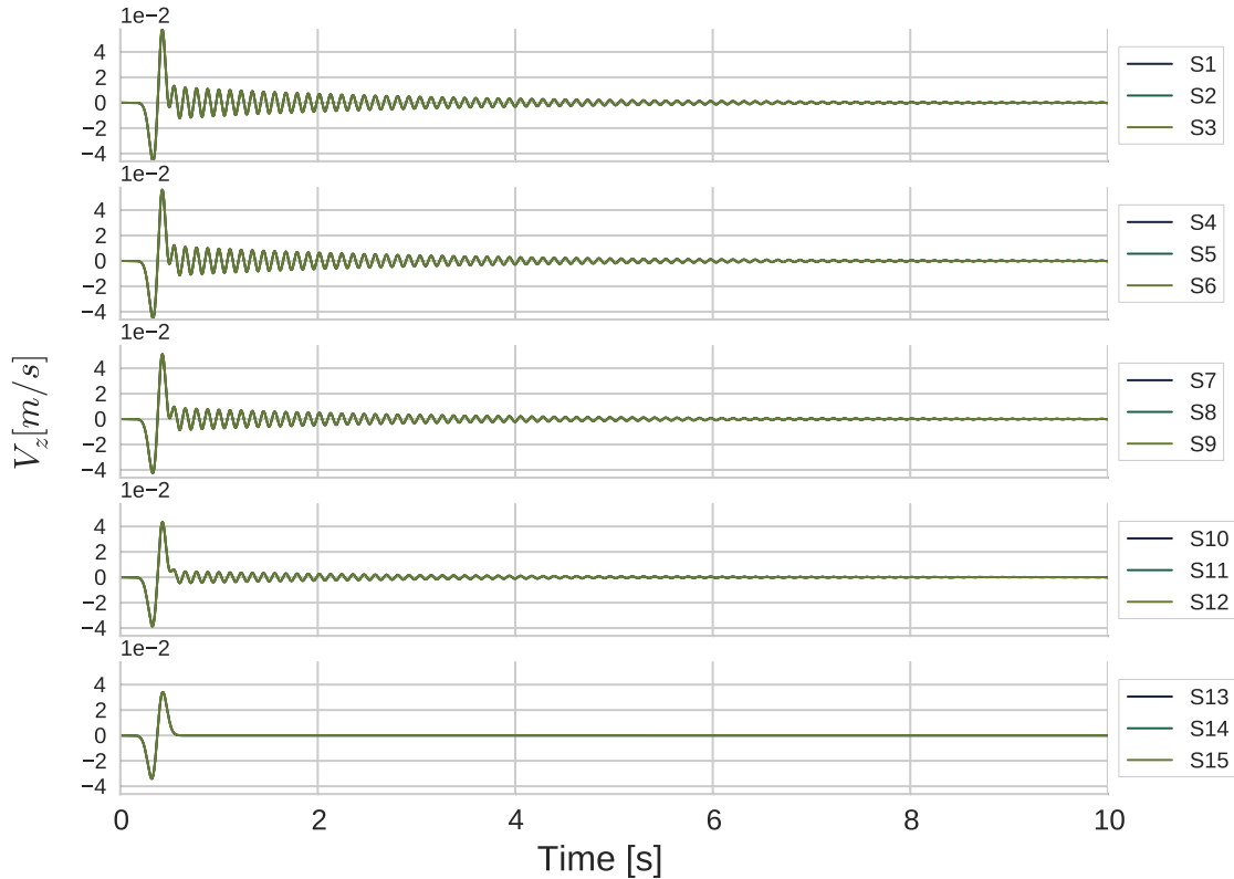
Fig. 4.28 Vertical velocity outputs for all the stations of P-SV wave propagation model with viscoelastic rheology in P1 medium.
