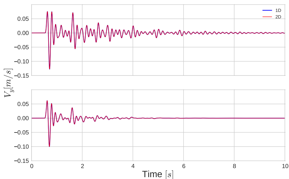
Fig. 4.46 Comparison of velocity outputs of Volvi model with two-element C-PML for elasticity (top) and for viscoelasticity (bottom) between 1D (in blue) and 2D (in red) SEM codes.
