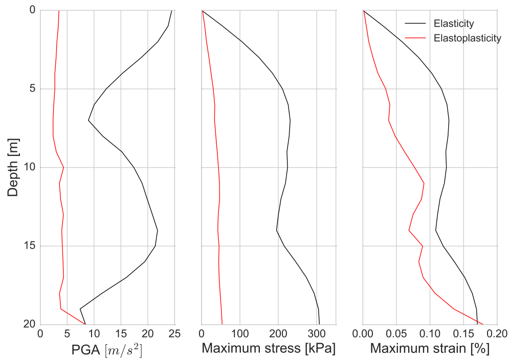
Fig. 2.20 Maximum PGA profile of P1 model under Real source #3 signal for elasticity (in black) and elastoplasticity (in red) (left); Maximum stress profile of P1 model under Real source #3 signal for elasticity (in black) and elastoplasticity (in red) (middle); Maximum strain profile of P1 model under Real source #3 signal for elasticity (in black) and elastoplasticity (in red) (right).
