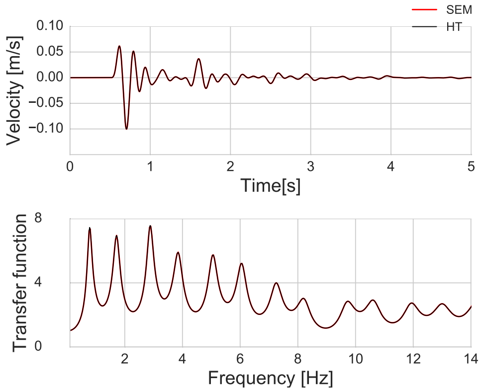
Fig. 2.10 Comparison between surface velocities obtained with SEM (in red) and HT (in black) (top); transfer functions obtained with SEM (in red) and HT (in black) (bottom) for viscoelasticity.
