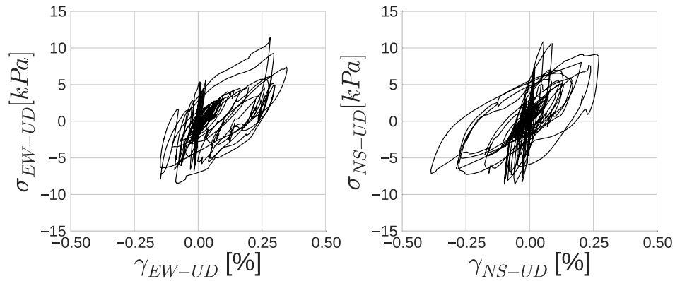
Fig. 3.21 Stress-strain curves on EW-UD component (left) and NS-UD component (right) for point at GL-4 m of the KP.
