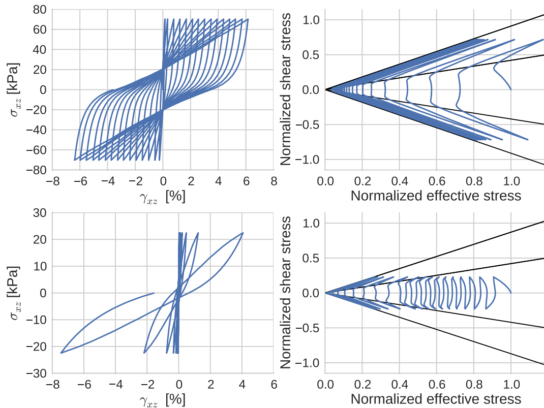
Fig. 1.13 Stress-strain curves for x-component (at left) and stress path (at right) for dense sand (top panel); for loose sand (bottom panel).
