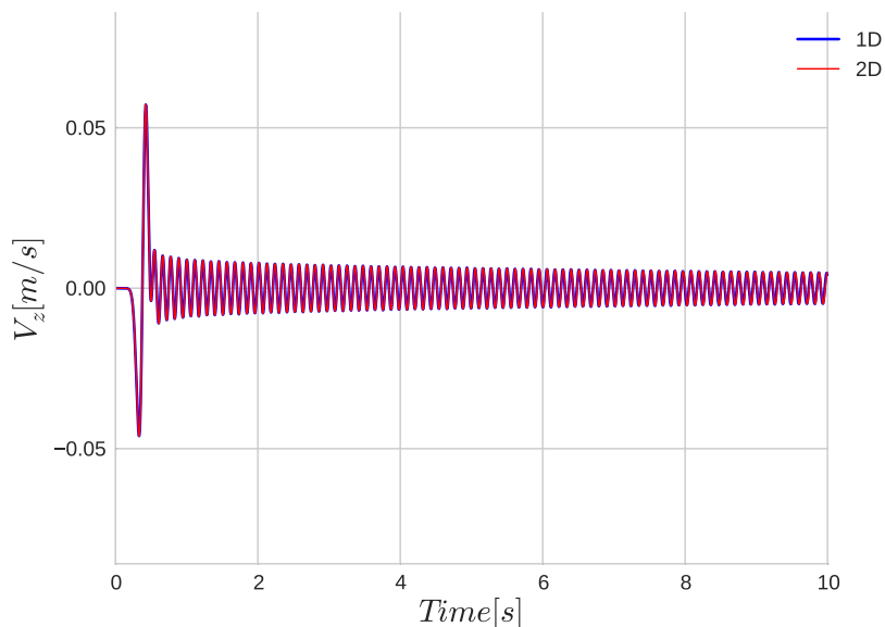
Fig. 4.42 Comparison of velocity outputs on z direction for 1D (in blue) and 2D (in red) SEM codes for pressure-dependent nonlinear P1 model under biaxial loading effective stress analysis.
