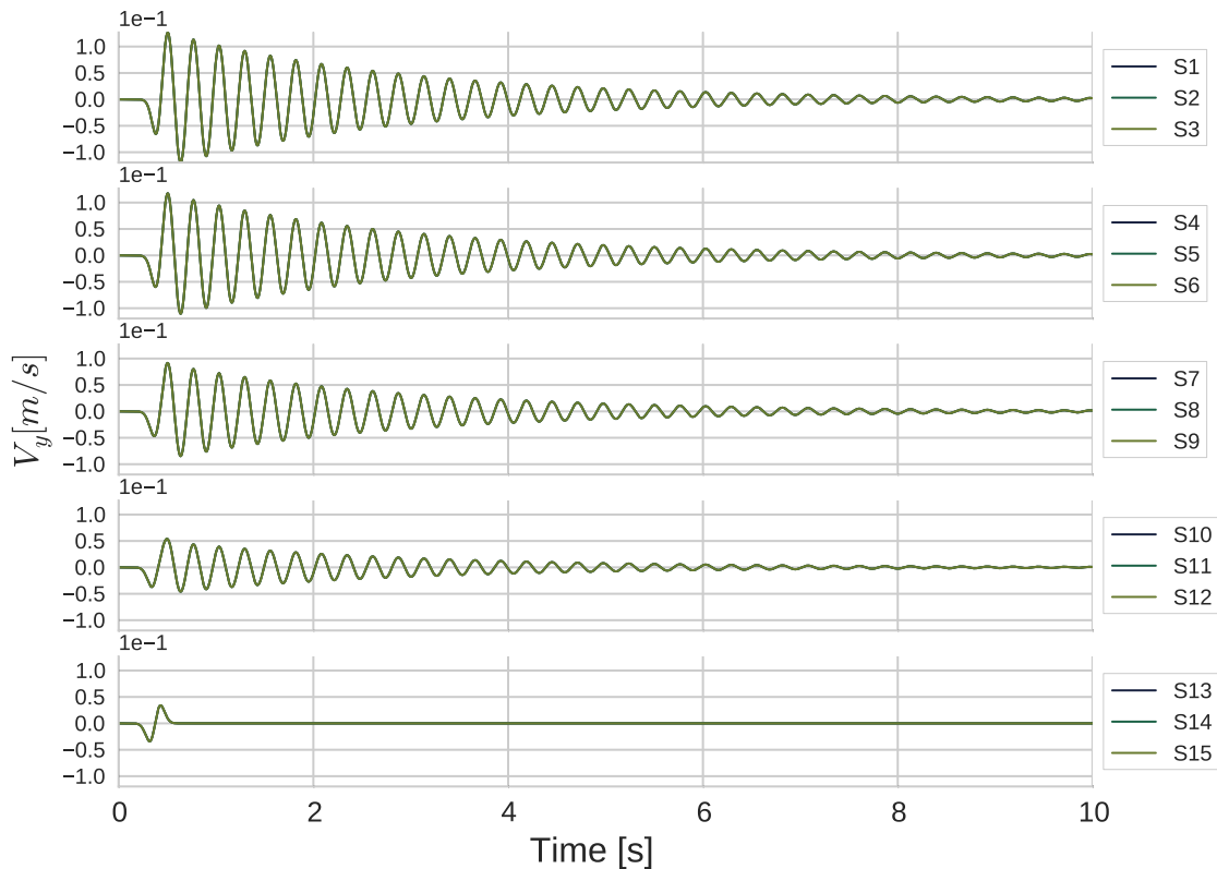
Fig. 4.30 Horizontal velocity outputs for all the stations of SH wave propagation model with viscoelastic rheology in P1 medium.
