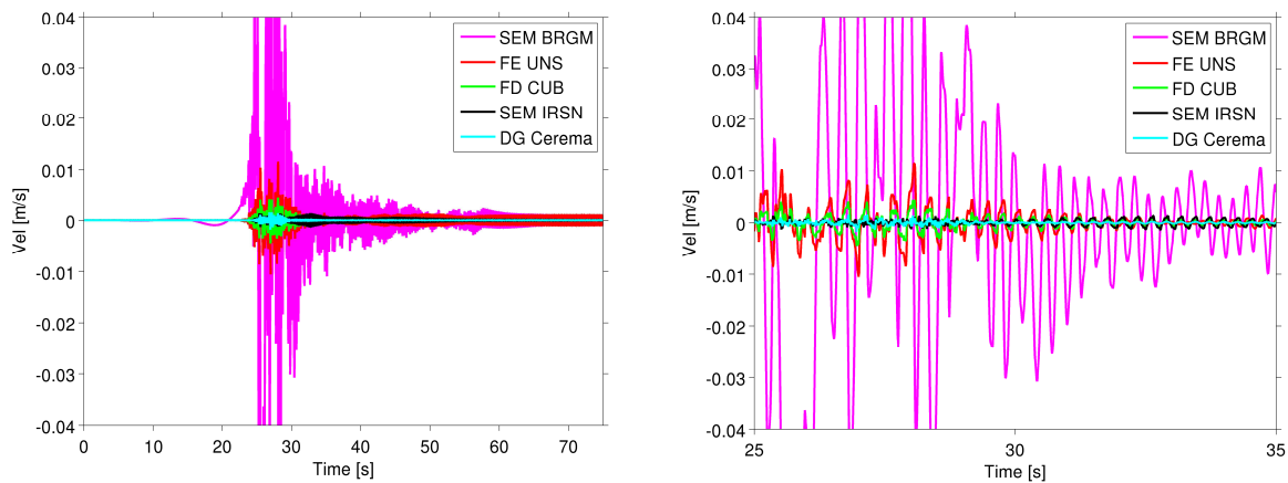
Figure 7: (left) Velocity seismograms at the top of the soil layer for the LF input signal. Reference solution in pink and differences of the other solutions to the reference. (right) Zoom from t=25 s to t=35 s.
