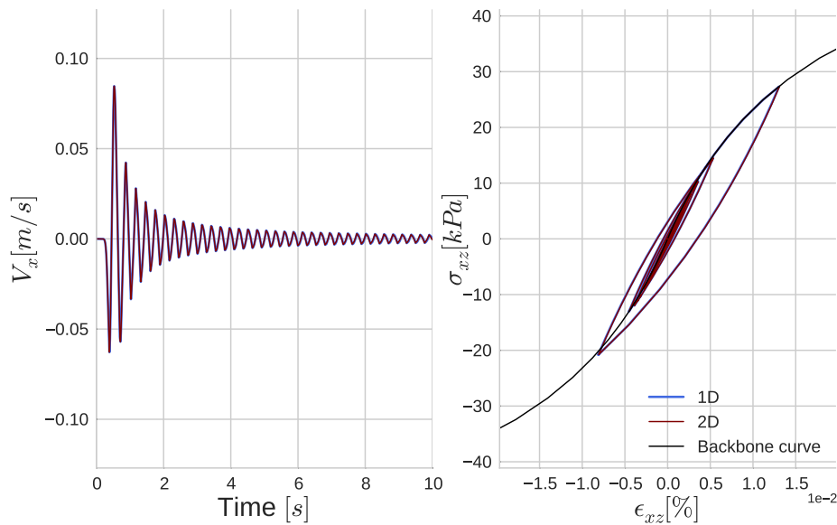
Fig. 4.31 Comparison of velocity outputs on x direction (left); comparison of stress-strain curves of xz component (right) at midlayer for 1D (in blue) and 2D (in red) SEM codes for pressure-independent nonlinear P1 model under uniaxial loading.
