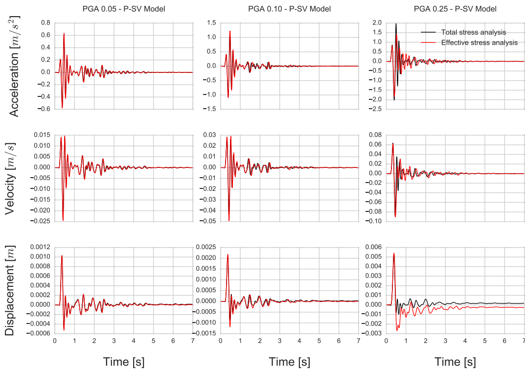
Fig. 5.30 Acceleration (top), velocity (middle) and displacement (bottom) time histories for total stress analysis (in black) and effective stress analysis (in red) of P-SV model under loading of impulse source with PGA 0.05g (left), 0.10g (middle) and 0.25g (right).
