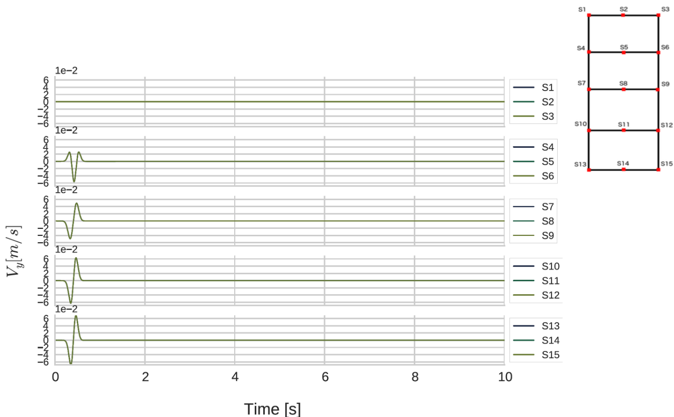
Fig. 4.25 Horizontal velocity outputs for all the stations of SH wave propagation model with upward attenuation C-PML element.
