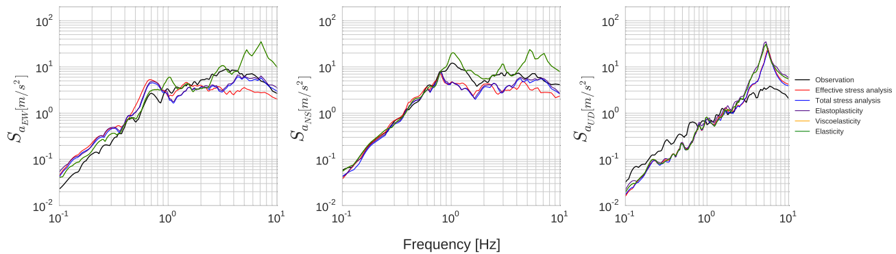
Fig. 3.26 Spectral acceleration comparison between elastic (in green), viscoelastic (in orange), elastoplastic (in purple), visco-elastoplastic with no excess pore pressure development (in blue) and visco-elastoplastic with excess pore pressure development (in red) models for three components of Kushiro Port site.
