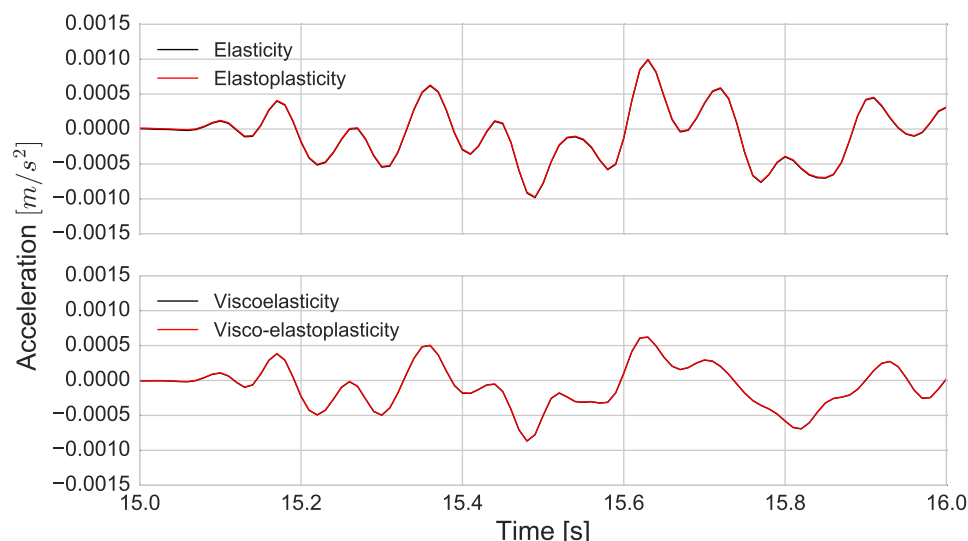
Fig. 2.17 Acceleration time histories for elasticity (in black) and elastoplasticity (in red) (top); Acceleration time histories for viscoelasticity (in black) and visco-elastoplasticity (in red) (bottom) on [15-16] s time interval for simulations under Real source #3 signal in the P1 model.
