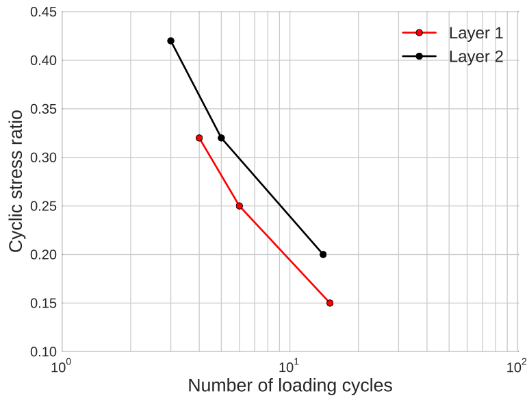
Fig. 5.4 Target liquefaction resistance curves for layer 1 (in red) and layer 2 (in black) of the 2D model.
