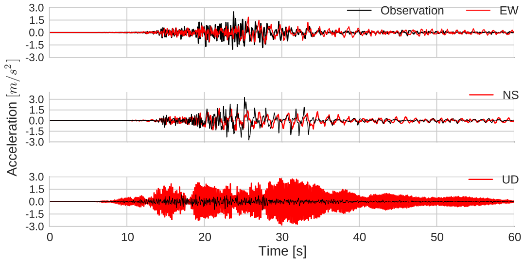
Fig. 3.18 Surface acceleration time histories calculated using the visco-elastoplastic model (in red) and real records (in black) for the KP site.
