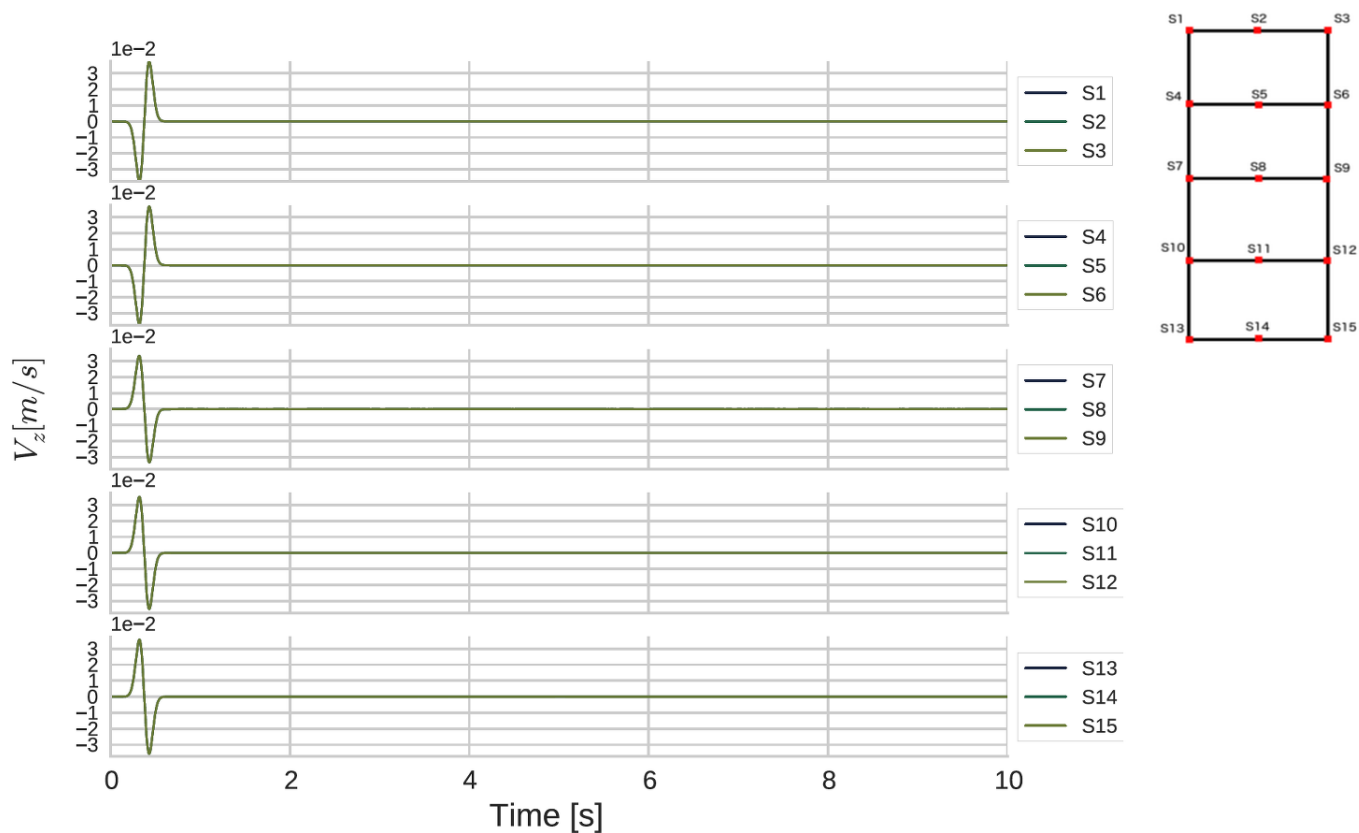
Fig. 4.8 Vertical velocity outputs for all the stations of P-SV wave propagation model with incident wave field.
