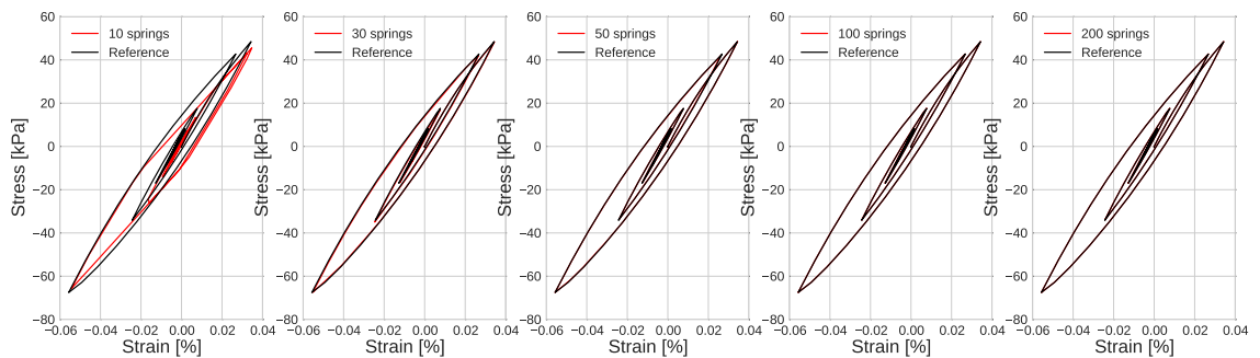
Fig. 2.27 Stress-strain curves for all the models with reference model solution (in black).
