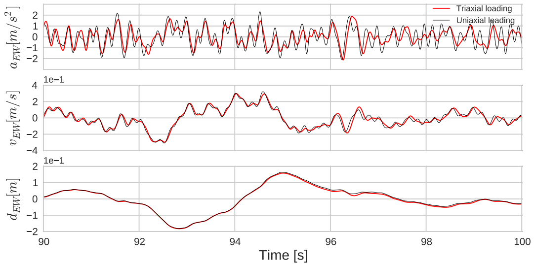
Fig. 3.44 Surface acceleration (top), velocity (middle) and displacement (bottom) comparison between uniaxial (in black) and triaxial (in red) loading for EW component.
