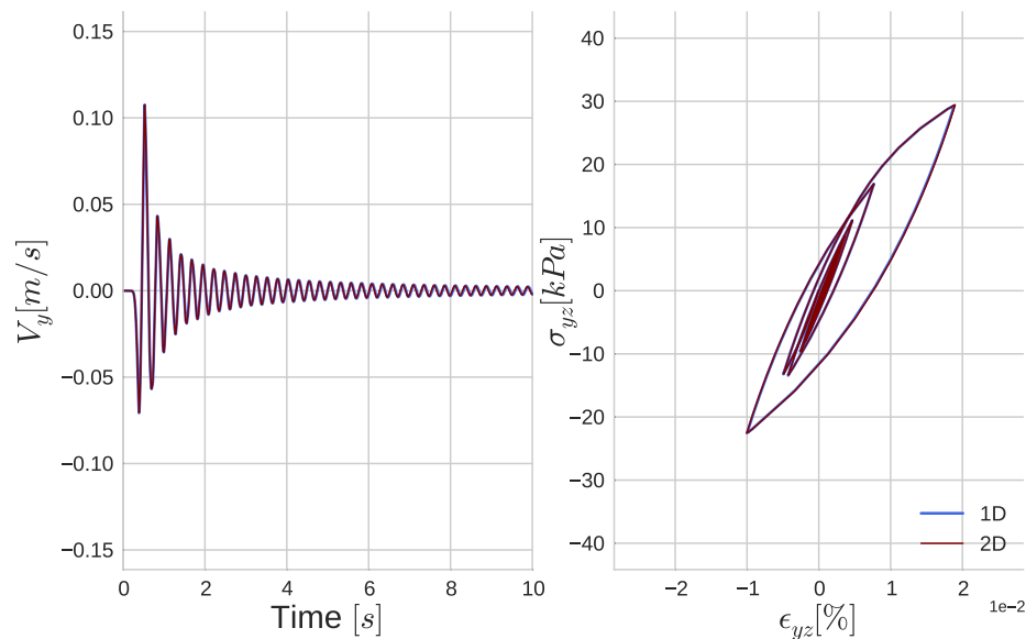
Fig. 4.37 Comparison of velocity outputs on y direction ( left); comparison of stress-strain curves of yz component at midlayer (right) for 1D (in blue) and 2D (in red) SEM codes for pressure-dependent nonlinear P1 model with water table at surface level under uniaxial loading.
