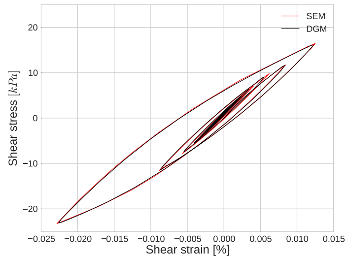
Fig. 2.12 Stress-strain curves computed with SEM (in red) and DGM (in black) for the P1 model simulation under elastoplastic conditions.
