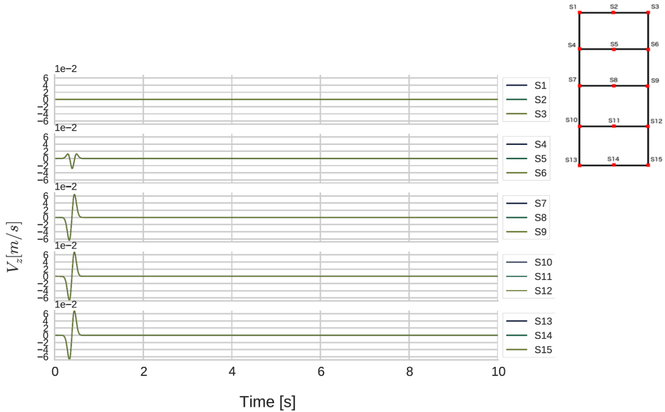
Fig. 4.23 Vertical velocity outputs for all the stations of P-SV wave propagation model with upward attenuation C-PML element.
