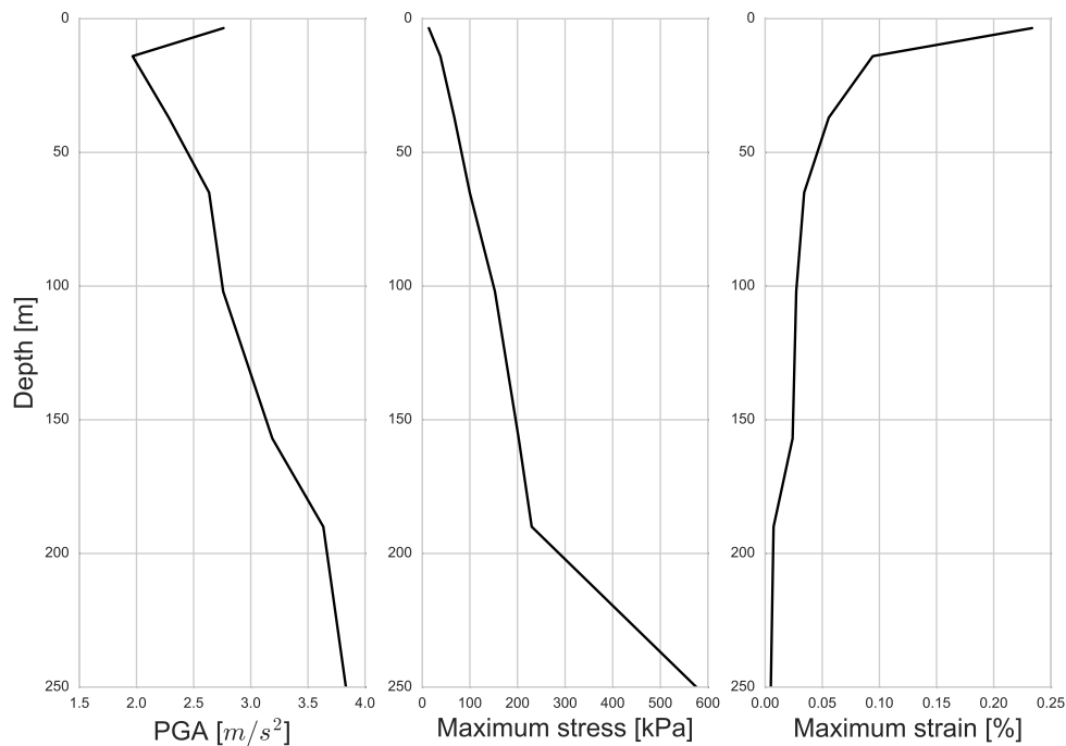
Fig. 2.25 Peak ground acceleration (left), maximum stress (middle) and maximum strain (right) distribution on soil model of Volvi model.
