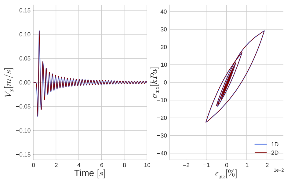
Fig. 4.35 Comparison of velocity outputs on x direction (left); comparison of stress-strain curves of xz component at midlayer (right) for 1D (in blue) and 2D (in red) SEM codes for pressure-dependent nonlinear P1 model with water table at surface level under biaxial loading.
