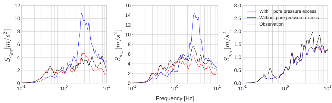
Fig. 3.10 Acceleration spectra of recorded surface acceleration (in black), visco-elastoplastic SEM simulation with excess pore pressure development (in red) and without excess pore pressure development (in blue) for EW component (left); for NS component (middle); for UD component (right).
