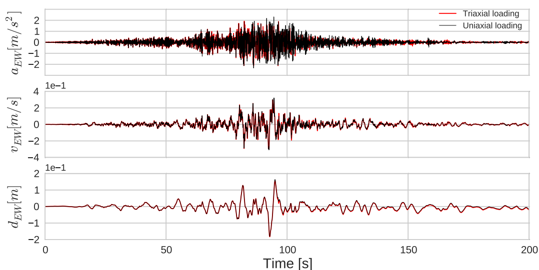
Fig. 3.43 Surface acceleration (top), velocity (middle) and displacement (bottom) comparison between uniaxial (in black) and triaxial (in red) loading for EW component.
