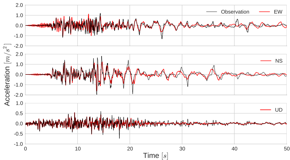
Fig. 3.4 Surface acceleration time histories calculated using the visco-elastoplastic model with pore pressure effects (in red) and real records (in black) for the WRLA site.
