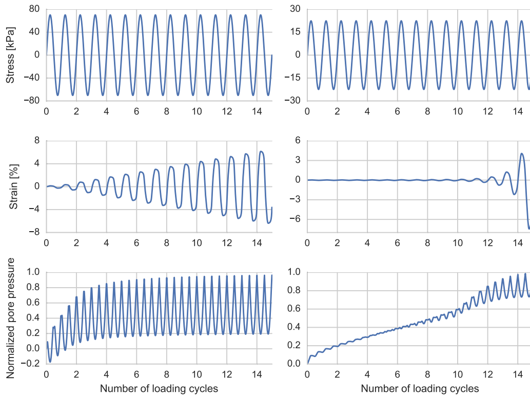
Fig. 1.14 Temporal change of stress (top), strain (middle) and pore pressure excess (bottom) for dense soil (left column) and loose soil (right column).
