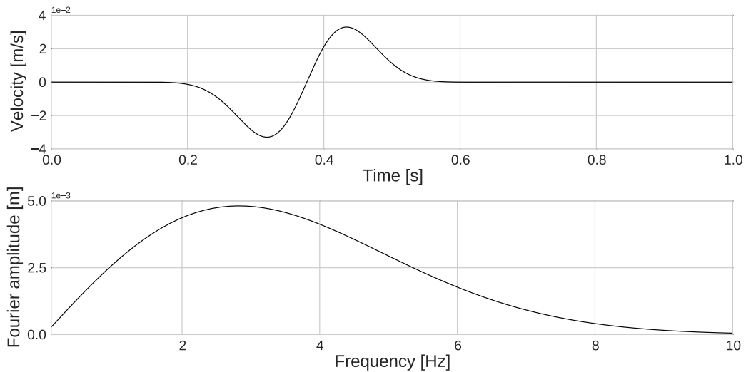
Fig. 2.11 Velocity time histories (top); Fourier amplitude (bottom) of Ricker signal used in the P1 model.
