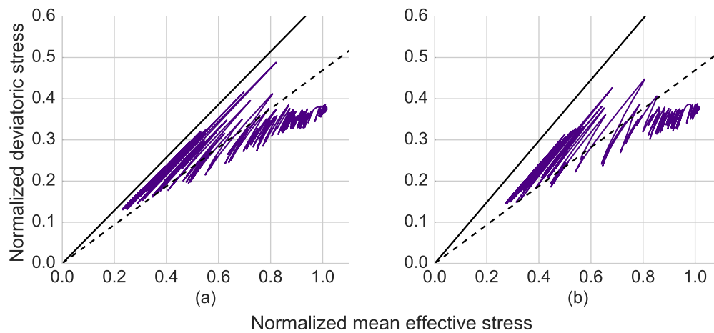
Fig. 3.20 (a) Deviatoric plan for point at GL-4 m, (b) Deviatoric plan for point at GL-15 m of the KP model with failure line (solid line) and phase transformation line (dashed line).
