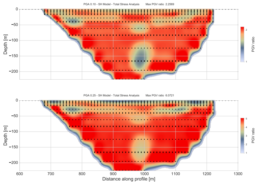
Fig. 5.18 Peak ground velocity ratio distribution of the basin for total stress analysis of SH models of the 2D sedimentary basin model under loading of impulse source with PGA 0.10g (top) and 0.25g (bottom).
