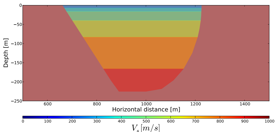
Fig. 5.1 Shear wave velocity profile of the 2D sedimentary basin model where bedrock shear velocity is 2000 m/s.
