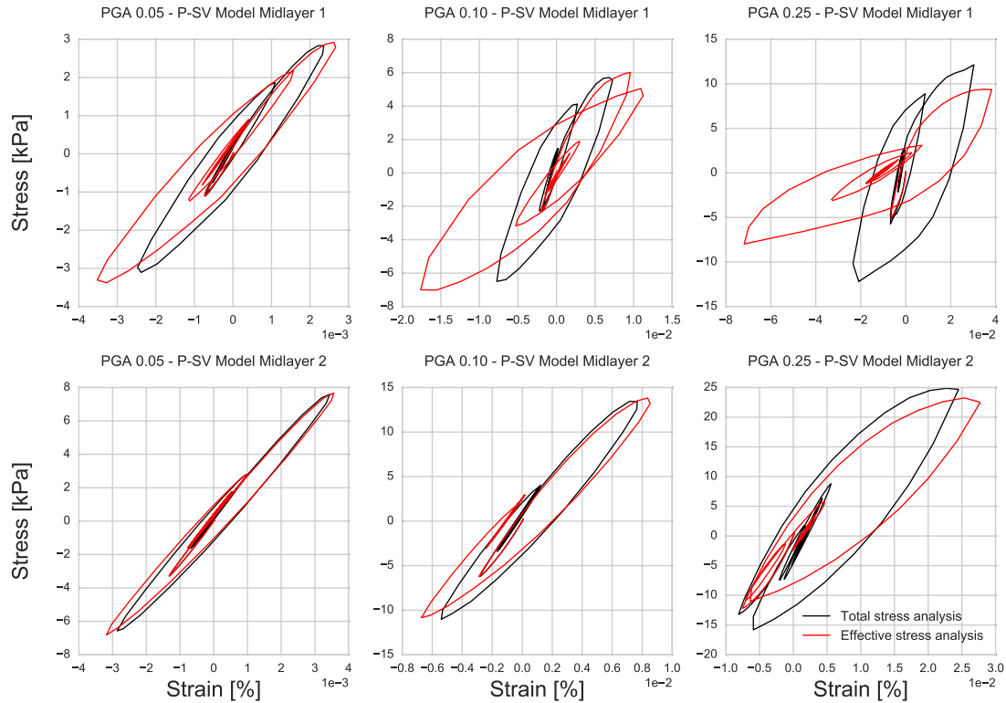
Fig. 5.29 Stress-strain curves at the middle of layer 1 (GL-3.5 m) (top) and layer 2 (GL-11.5 m) (bottom) for total stress analysis (in black) and effective stress analysis (in red) of P-SV model under loading of impulse source with PGA 0.05g (left), 0.10g (middle) and 0.25g (right).
