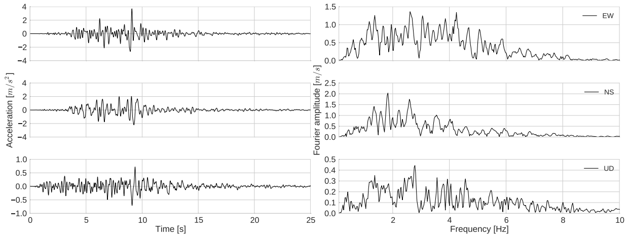
Fig. 5.11 Acceleration time histories (left column) and Fourier amplitudes (right column) of Northridge earthquake records for EW component (top), NS component (middle) and vertical component (bottom).
