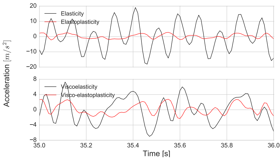
Fig. 2.18 Acceleration time histories for elasticity (in black) and elastoplasticity (in red) (top); Acceleration time histories for viscoelasticity (in black) and visco-elastoplasticity (in red) (bottom) on [35-36] s time interval for simulations under Real source #3 signal in the P1 model.
