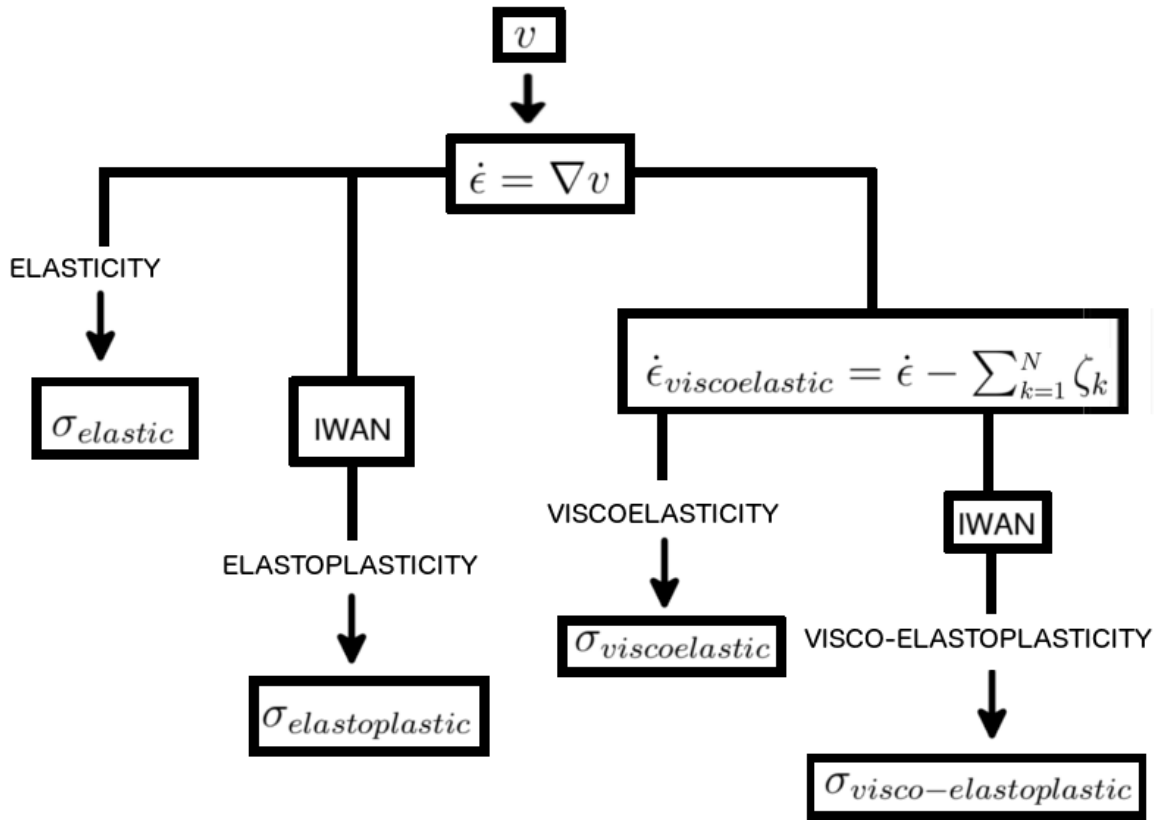
Fig. 2.1 Numerical work flow of 1D SEM code for different material constitutive models.
