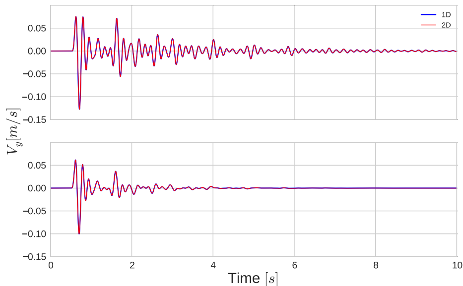
Fig. 4.45 Comparison of velocity outputs of Volvi model with single-element C-PML for elasticity (top) and for viscoelasticity (bottom) between 1D (in blue) and 2D (in red) SEM codes.
