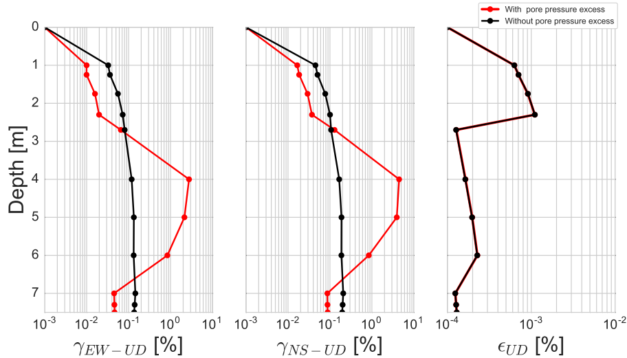
Fig. 3.11 Comparison of maximum strain profiles as a function of depth between visco-elastoplastic simulations with excess pore pressure development (in red) and without excess pore pressure development (in black) for EW-UD (left), NS-UD (middle) and UD (right) components.
