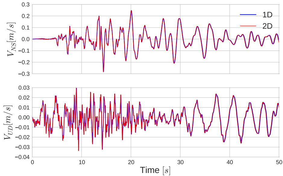
Fig. 4.48 Comparison of surface velocity outputs of WRLA model with two lateral elements for NS (top) and for UD (bottom) direction between 1D (in blue) and 2D (in red) SEM codes.
