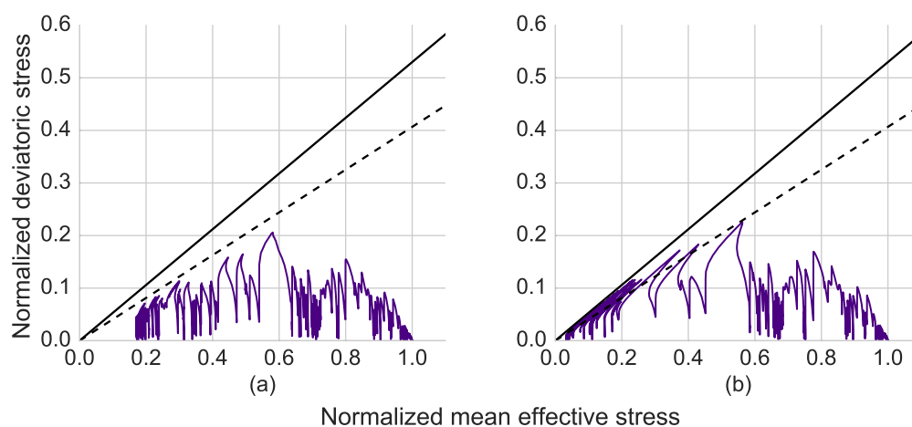
Fig. 3.5 (a) Deviatoric plan for point at GL-2.9 m, (b) Deviatoric plan for point at GL-4.0 m of the WRLA model with failure line (solid line) and phase transformation line (dashed line).
