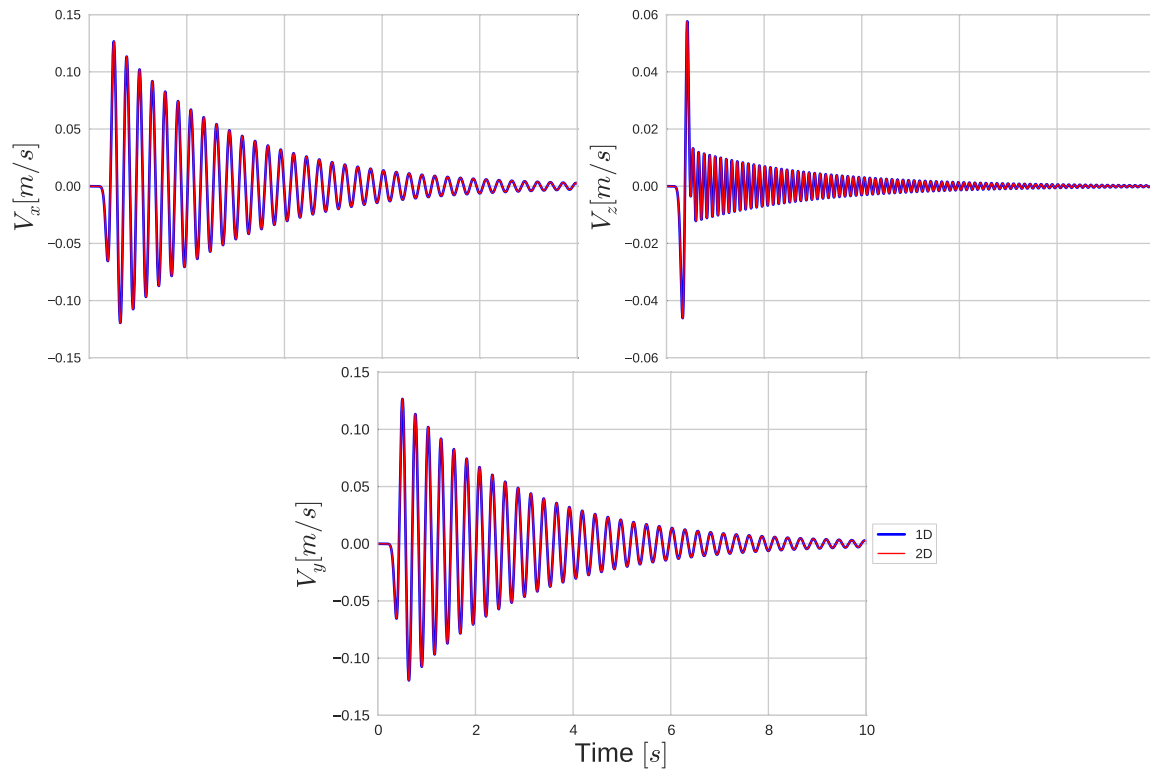
Fig. 4.29 Comparison of velocity outputs on horizontal (top left) and vertical (top right) directions of P-SV wave propagation model with viscoelastic rheology; on horizontal direction (bottom) of SH wave propagation model with viscoelastic rheology between 1D (in blue) and 2D (in red) SEM codes.
