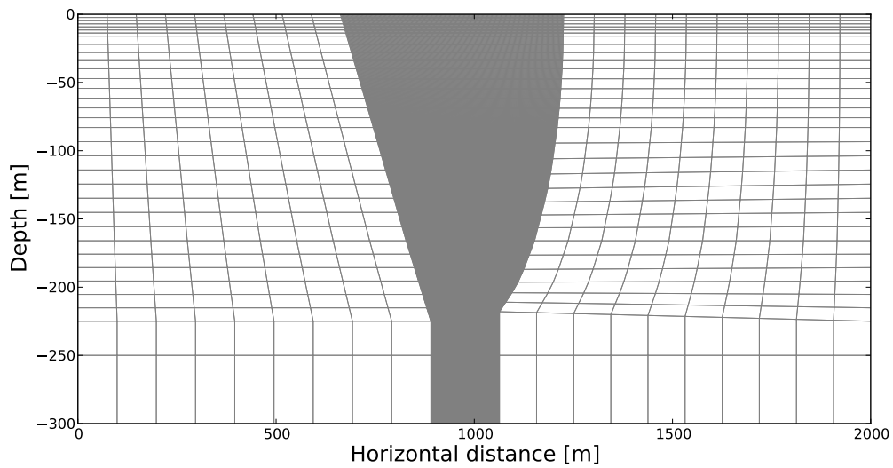
Fig. 5.6 2D mesh grid of the 2D model.
