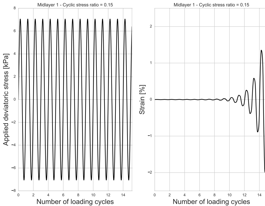
Fig. 5.5 Deviatoric stress applied on the middle of soil layer 1 (left) and strain (right) as a function of number of loading cycle.
