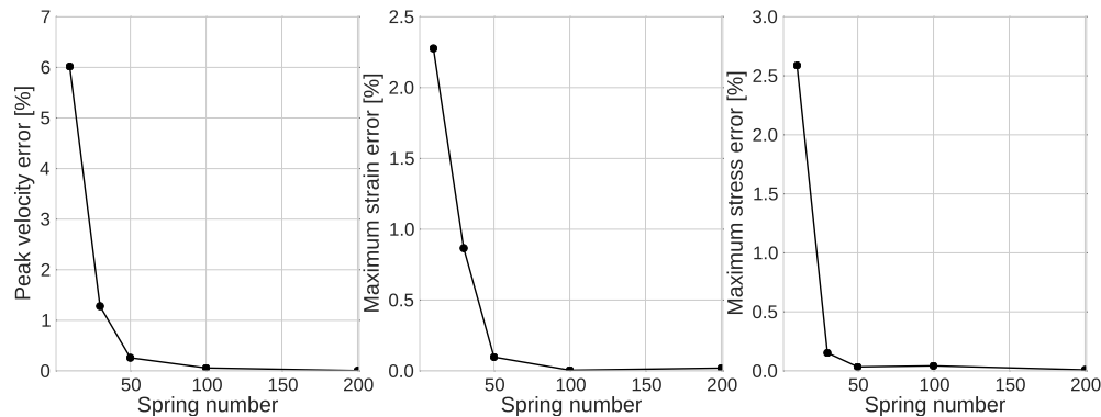
Fig. 2.26 Peak velocity error percentage (left); Maximum strain error percentage (middle); Maximum stress error (right) for the solutions of all the models.
