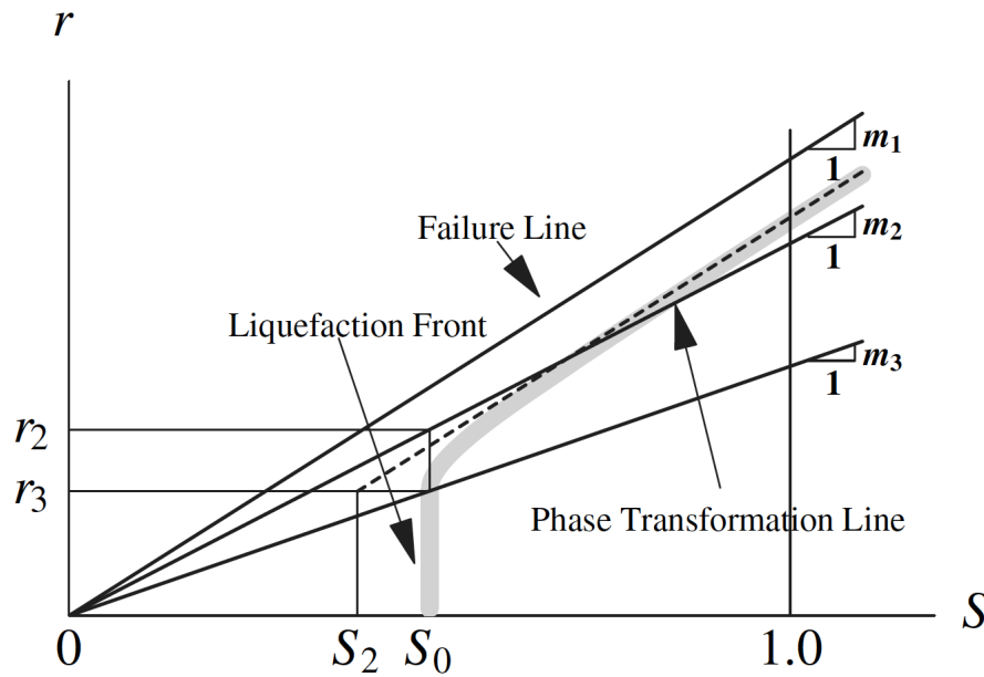
Fig. 1.9 Schematic plot of liquefaction front of Iai et al. (1990) [69] model in normalized stress space (after Iai et al., 1990 [69]). S holds for normalized mean effective stress and r is the normalized deviatoric stress.
