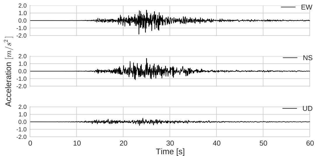
Fig. 3.17 Acceleration time histories at GL-77 m depth in east-west (EW), north-south (NS) and vertical (UD) directions recorded at KP.
