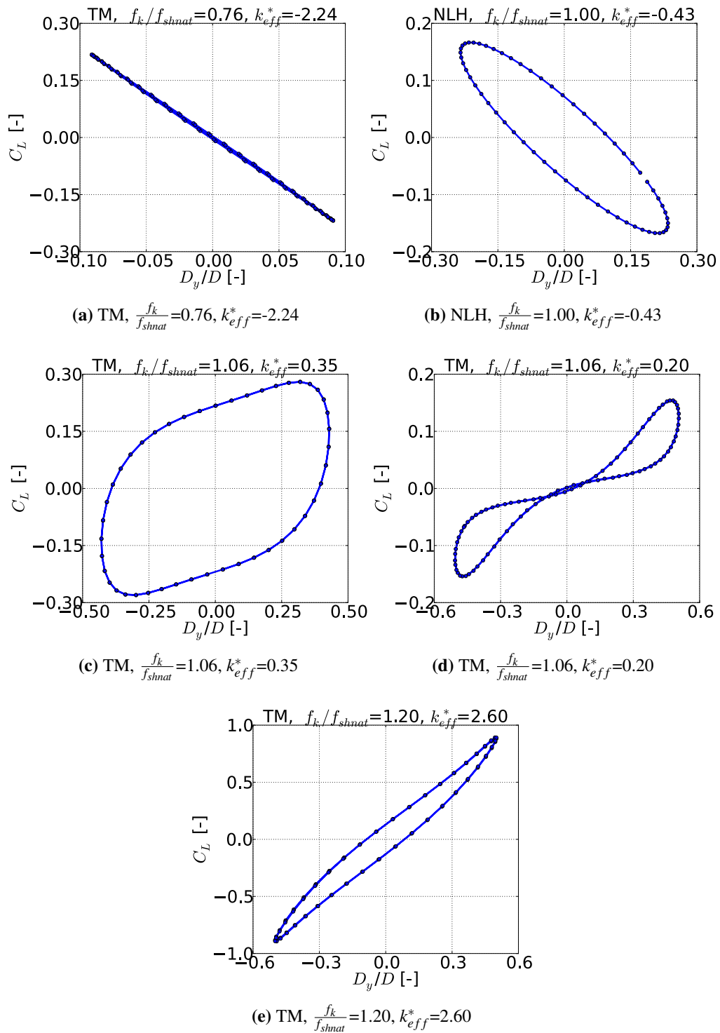
Figure 4.41: Free oscillation cylinder phase portraits. Pre lock-in region: (a), (b), Full lock-in region: (c), (d), (e), Post lock-in region: (f), (g). NLH simulations account for 2 harmonics. Markers do not represent data sampling. Continued on next page...
