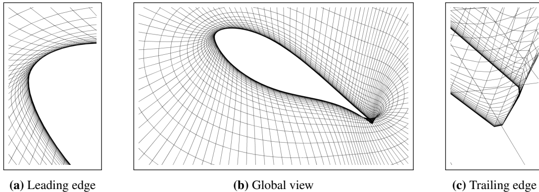
Figure 3.21: FFA-w3-241 deformed mesh, Laplacian Smoothing , DLC1
