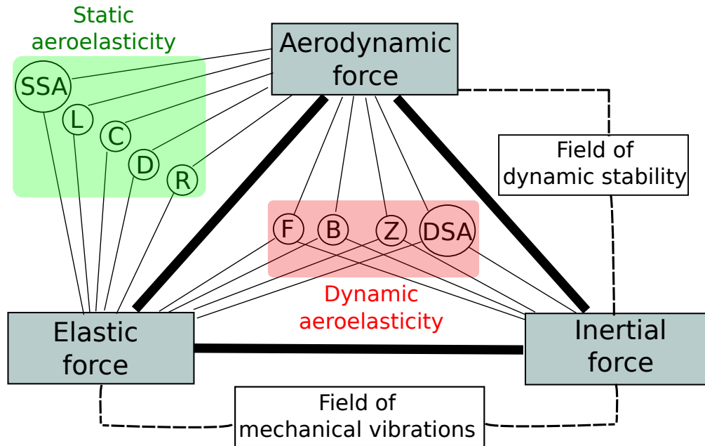
Figure 2.7: Collar's diagram applied to aircraft design, adapted from Bisplinghoff et al. (1995). SSA: Aeroelastic effects on static stability, L: Load distribution, C: Control effectiveness, D: Divergence, R: Control system reversal, F: Flutter, B: Buffeting, Z: Dynamic response, DSA: Aeroelastic effects on dynamic stability
