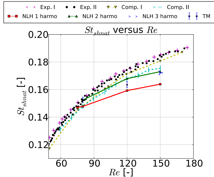
Figure 4.18: Fixed cylinder, comparison of identified St_{shnat} . NLH and TM stand for the Non-Linear Harmonic and time marching computations performed in the present study, respectively. Exp. I refers to the experimental data from Williamson (1996). Exp. II refers to the experiments of Fey et al. (1998). Comp. I. refers to the computational results of Spiker et al. (2006) using the Harmonic balance method. Comp. II refers to the computational results of McMullen (2003) using the Non-Linear Frequency Domain .
