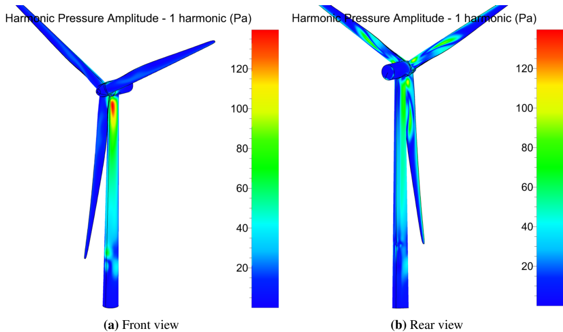
Figure 6.9: Amplitude of first pressure harmonic on DTU 10MW RWT surface, 1h simulation
