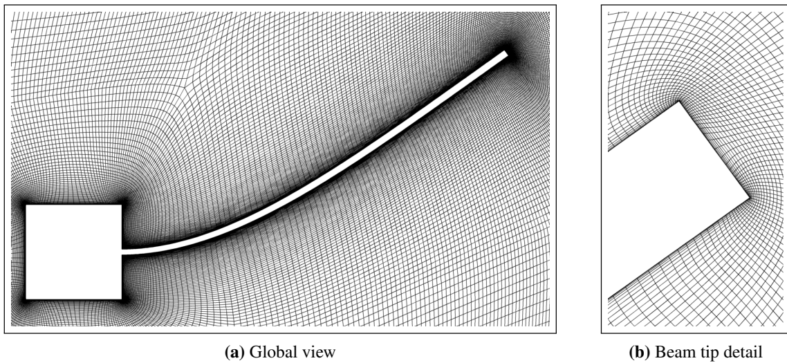
Figure 3.18: VIV Test Case, RBF+TFI+ELA deformation
