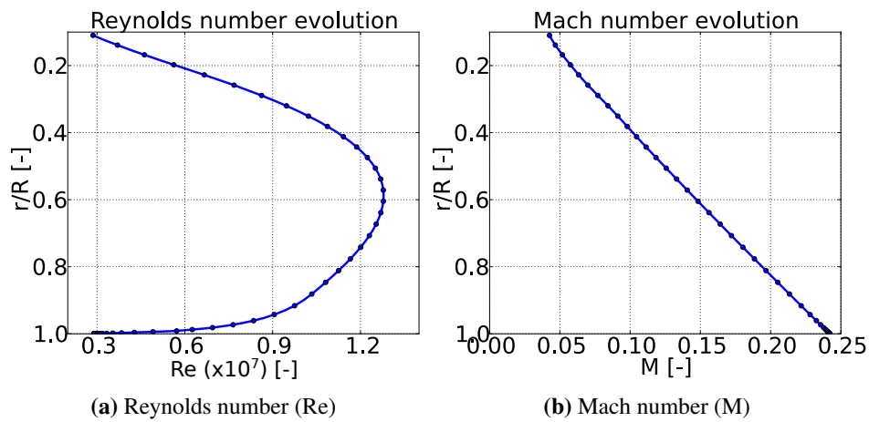
Figure 5.10: DTU 10MW RWT, relative Mach and Reynolds numbers radial evolution at nominal operating point
