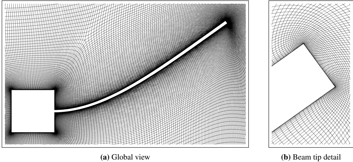
Figure 3.12: VIV Test Case, Elastic Analogy deformation
