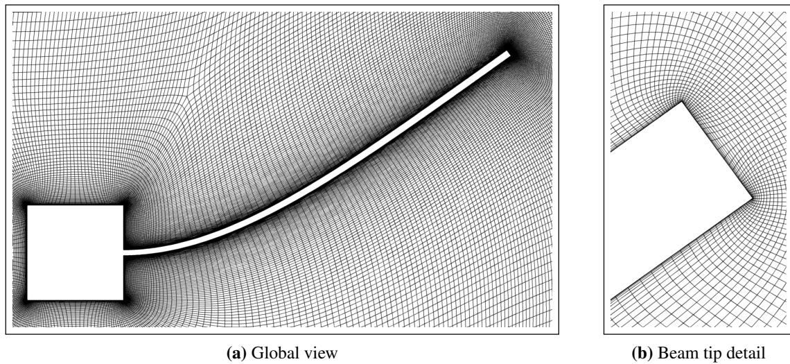
Figure 3.4: VIV Test Case, Radial Basis Functions deformation
