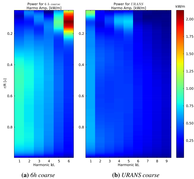
Figure 6.19: Amplitude of blade power harmonics [kW/m] as a function of r/R [-], with URANS coarse
