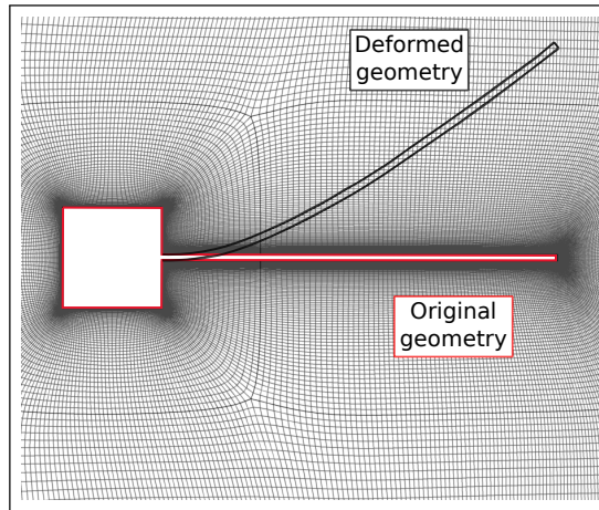
Figure 3.3: VIV test case, original and deformed geometries
