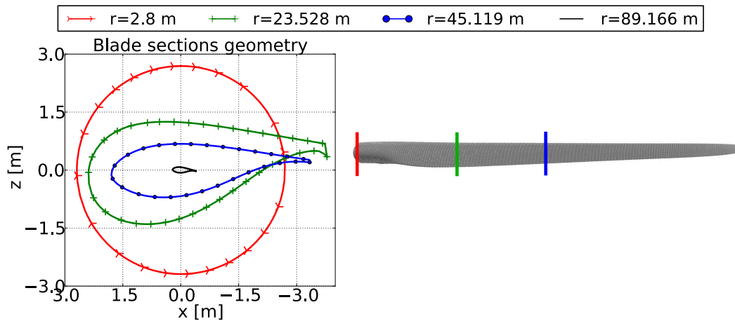
Figure 5.4: Cross sections of DTU 10MW RWT blade for different radii. Markers do not represent data sampling. A sketch of the cross sections location on the blade span was added for clarity purposes
