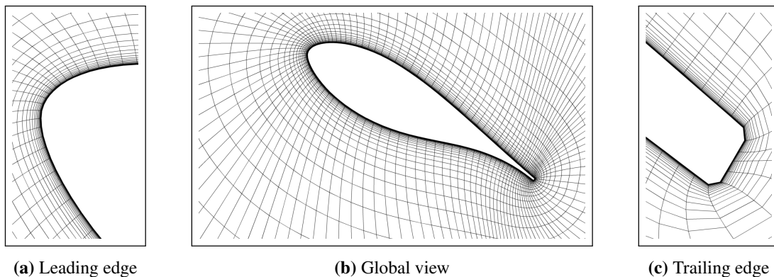
Figure 3.23: FFA-w3-241 deformed mesh, RBF+TFI+ELA, DLC1
