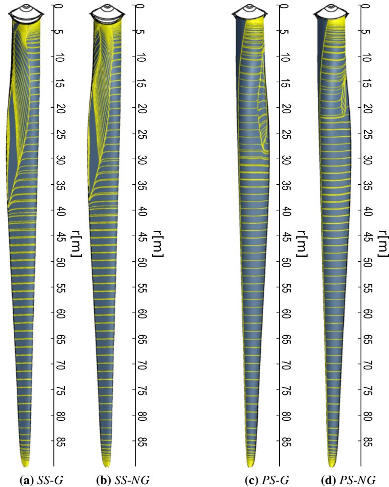
Figure 5.31: Friction streamlines at 11 \text{ ms}^{-1} for suction and pressure surfaces (referred as SS and PS respectively). Rigid simulations of G (Gurney) and NG (no-Gurney) configurations. Flow separation regions can be observed on both the pressure side and the suction side for both configurations
