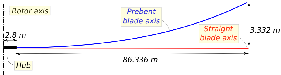
Figure 5.5: DTU 10MW RWT blade axis prebending
