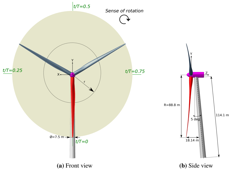
Figure 6.1: Sketch of the DTU 10MW RWT assembly
