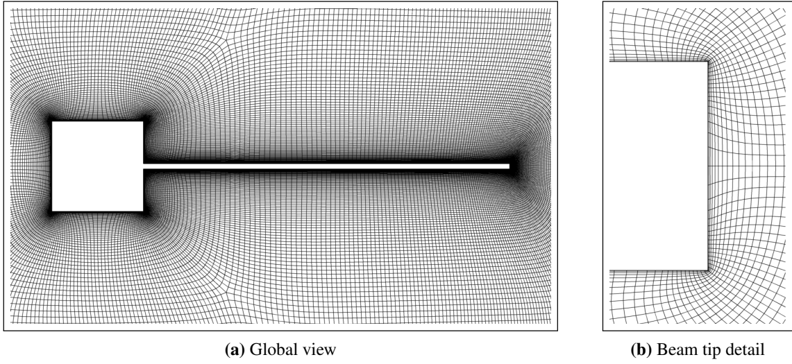
Figure 3.2: VIV test case, original mesh
