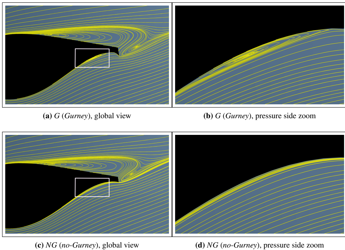
Figure 5.30: Cross-section streamlines at 11 \text{ ms}^{-1} for r=22.3 \text{ m} ( r/R=0.25 ). Rigid simulations of G ( Gurney ) and NG ( no-Gurney ) configurations
