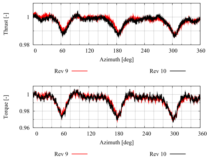
Figure 2.15: Normalized rotor thrust and torque for the last two revolutions of a simulation of the SIEMENS 3.6MW wind turbine [source: Zahle and Sørensen (2008)]
