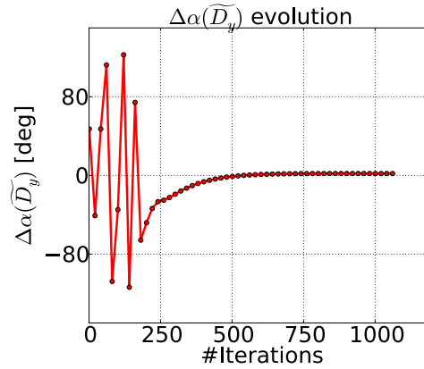
Figure 4.33: Free oscillation cylinder \Delta\alpha(\tilde{D}_y) [deg] vs. solver iterations, corresponding to the NLH computation at f_k/f_{shnat}=1.0 and \xi=0.0012 solved for a frequency \neq f_{shed} . Markers correspond to every call to the harmonic structural equation
