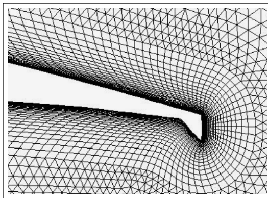
(b) CFD computations of Salcedo et al. (2006)
