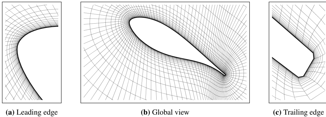
Figure 3.22: FFA-w3-241 deformed mesh, RBF+TFI, DLC1
