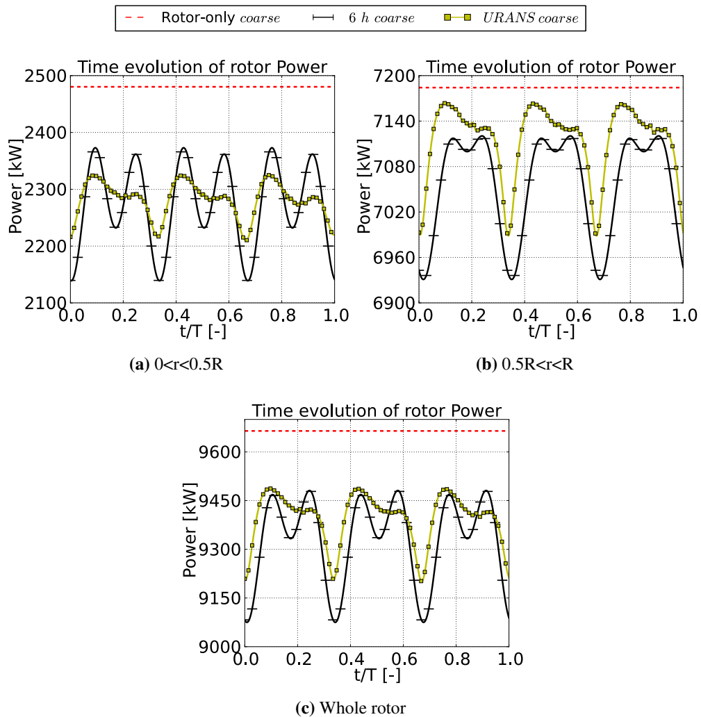
Figure 6.22: Rotor power [kW] time evolution, including URANS coarse . Markers do not correspond to data sampling
