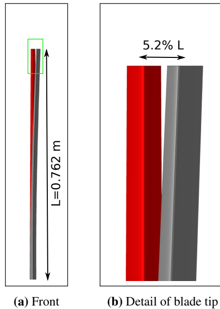
Figure 3.30: Original (red) and deformed (grey) AGARD 445.6 wing, DLC1
