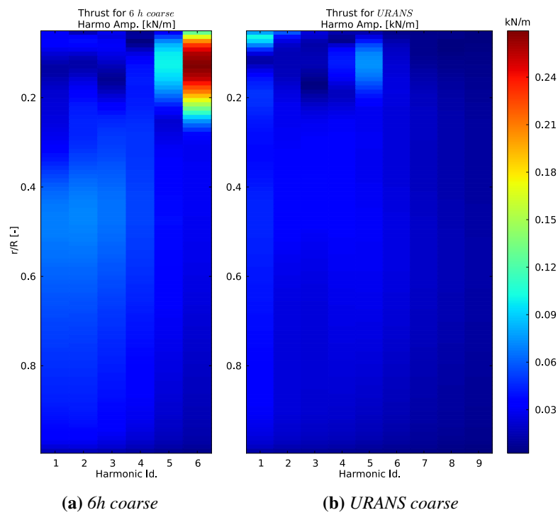
Figure 6.18: Amplitude of blade thrust harmonics [kN/m] as a function of r/R [-], with URANS coarse
