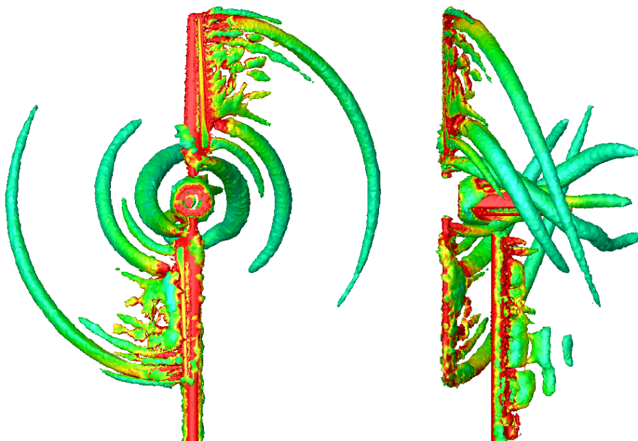
Figure 2.13: Vorticity of the NREL Phase VI, illustrated by means of the Q-criterion isosurfaces for a value of 0.1. URANS computation of Lynch (2011) at 15 \text{ m}\cdot\text{s}^{-1} .
