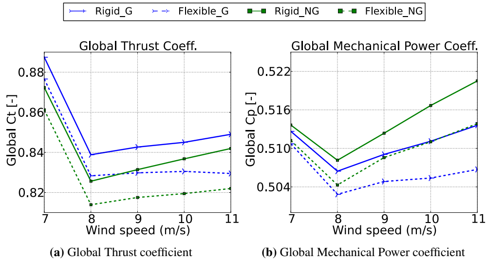
Figure 5.32: Global load coefficients in function of wind speed for G (Gurney) and NG (no-Gurney) configurations
