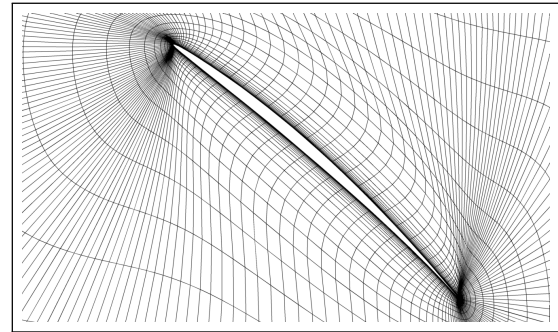
(c) Def. RBF+TFI+ELA
