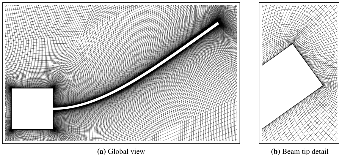
Figure 3.17: VIV Test Case, RBF+TFI deformation
