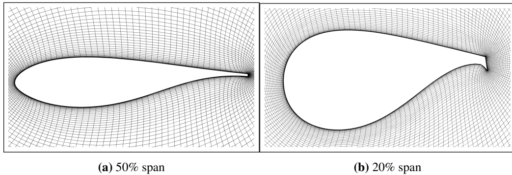
Figure 5.9: DTU 10MW RWT cross-section meshes, 20% and 50% span
