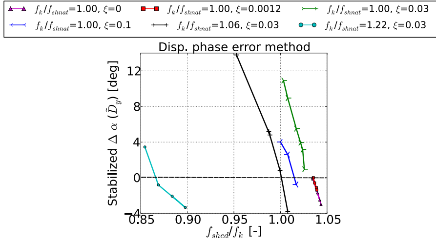
Figure 4.34: Free oscillation cylinder, stabilized \Delta\alpha(\tilde{D}_y) for different NLH (2 harmonics) computations as a function of f_{shed}/f_k
