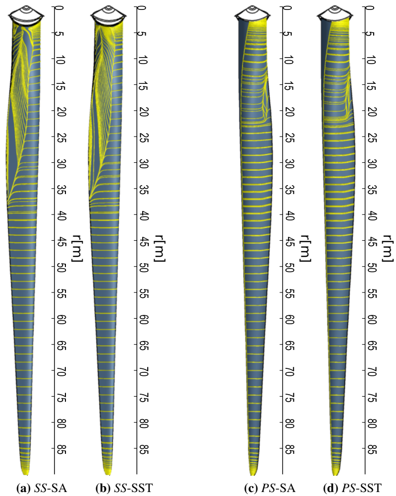
Figure C.1: Friction streamlines at 11 \text{ ms}^{-1} for suction and pressure surfaces (referred as SS and PS respectively). Rigid simulations of prebent/precone blade without Gurney flaps . SA refers to Spalart-Allmaras turbulence model. SST refers to k-\omega SST turbulence model
