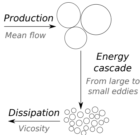
Figure 2.3: Turbulence phenomenon, sketch of eddies evolution
