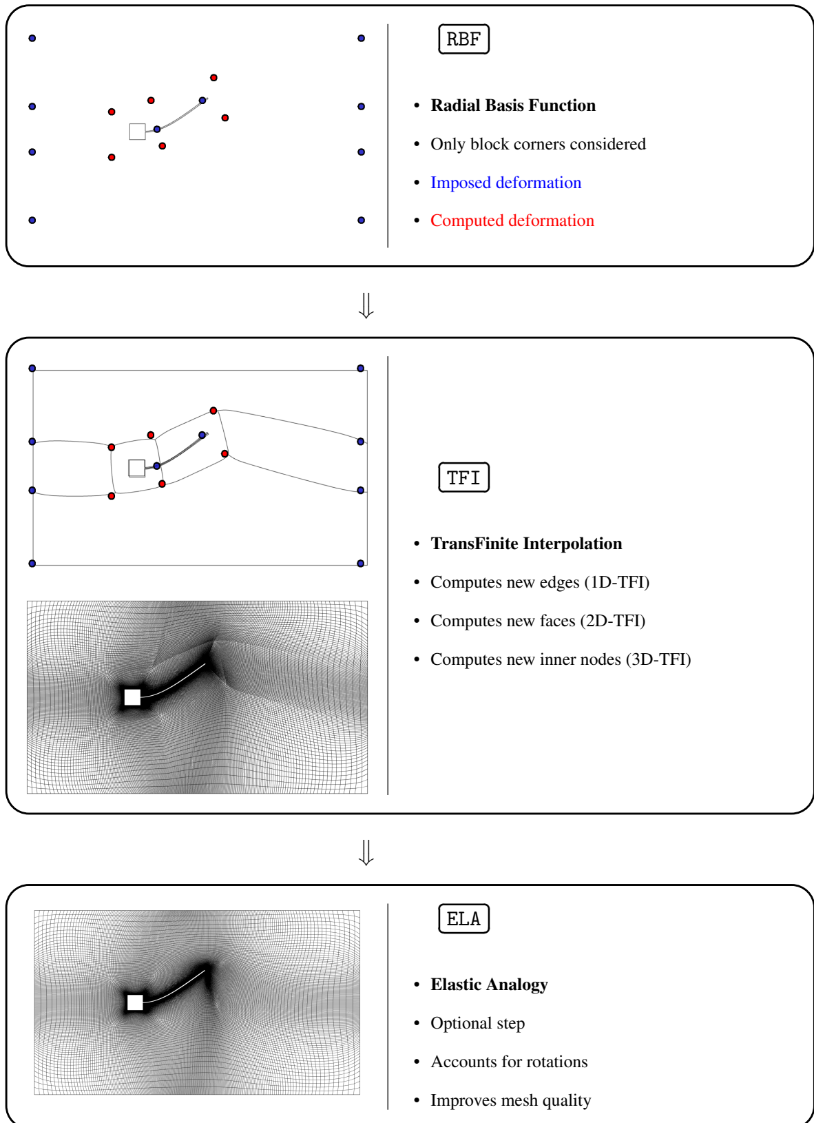
Figure 3.16: Mesh Hybrid method schema
