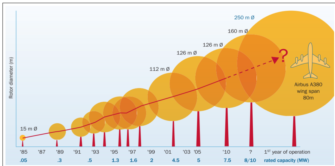
Figure 1.1: Wind turbines rotor evolution [source: UpWind Consortium (2011)]
