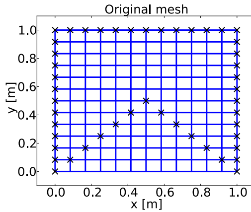
Figure 3.7: Original Cartesian mesh (in blue). Black crosses refer to the imposed displacements through Dirichlet boundary conditions
