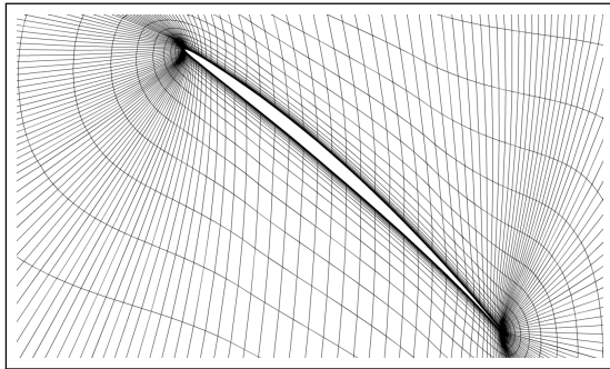
(b) Def. RBF+TFI
