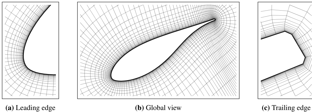
Figure 3.28: FFA-w3-241 deformed mesh, RBF, DLC2
