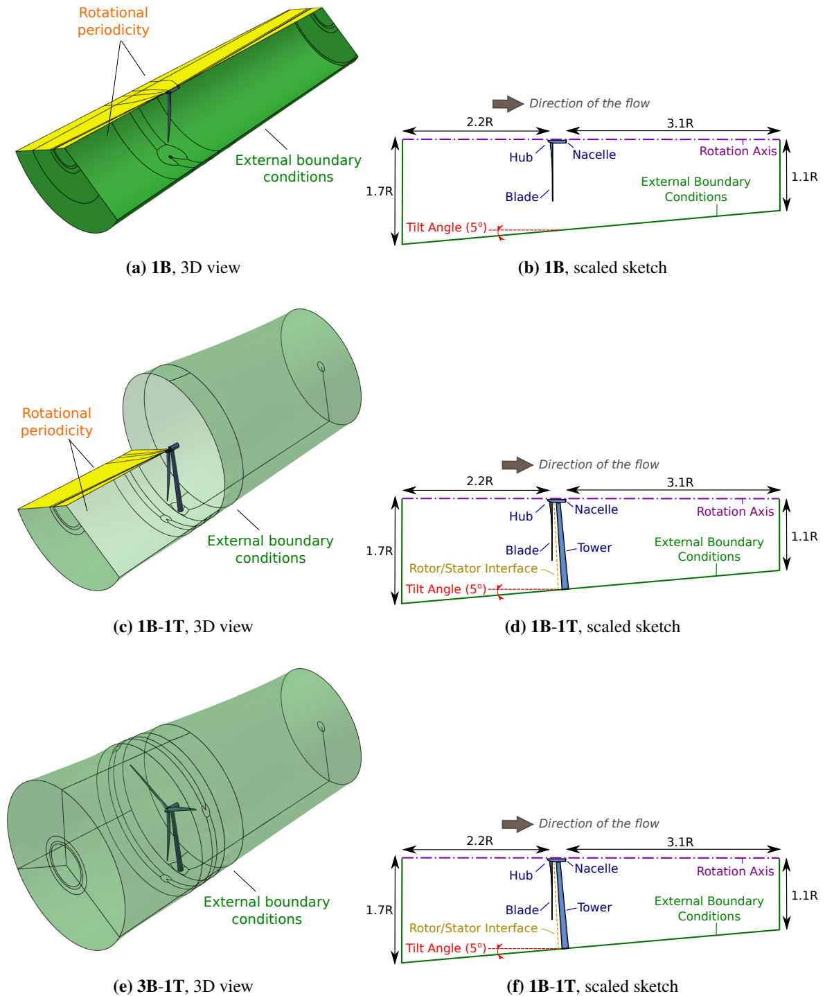
Figure 6.2: Description of the computational domains for 1B , 1B-1T and 3B-1T meshes. Solid lines represent mesh blocking. In (a) and (c), one of the periodic boundary conditions was removed to allow the visualization of the interior of the domain. In (c) and (e), the domain of the tower side was set to translucent to get a clearer visualization
