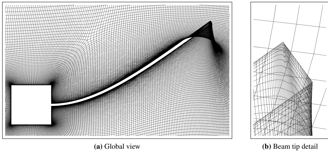
Figure 3.5: VIV Test Case, Laplacian Smoothing deformation
