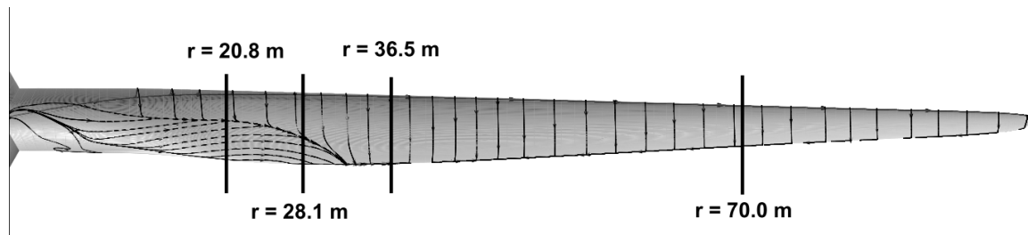
Figure 2.16: Friction streamlines of the DTU 10MW RWT blade suction surface at 10 \text{ m}\cdot\text{s}^{-1} and 8.06 RPM [source: Zahle et al. (2014)]
