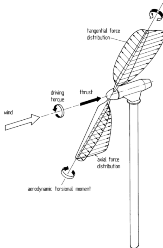
Figure 2.1: Basic principle of a horizontal axis wind turbine [source: Hau (2006)]
