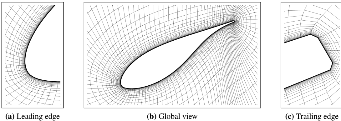
Figure 3.27: FFA-w3-241 deformed mesh, RBF+TFI+ELA, DLC2
