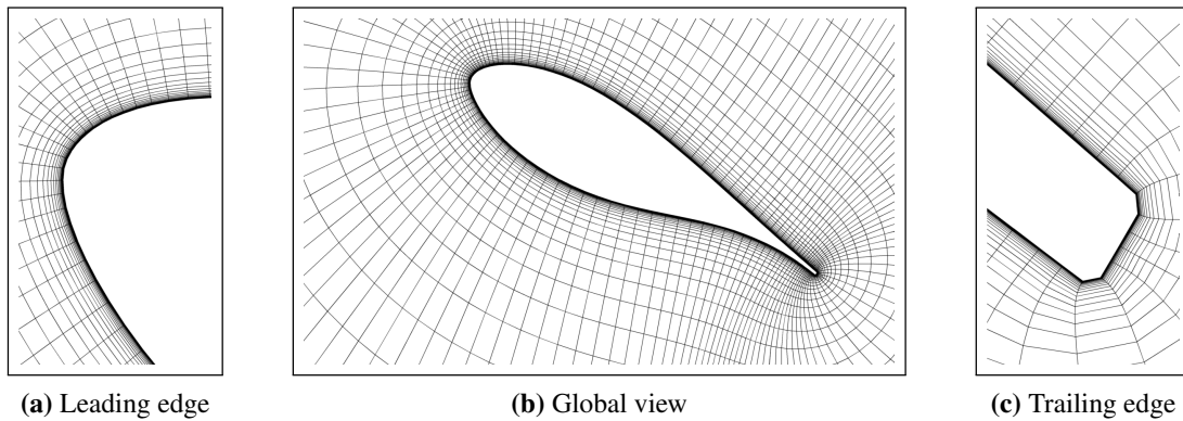
Figure 3.24: FFA-w3-241 deformed mesh, RBF, DLC1
