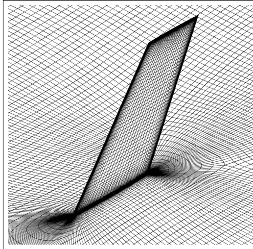
Figure 3.29: AGARD 445.6 mesh detail
