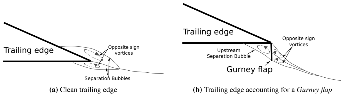
Figure 5.27: Expected effects on trailing edge flow due to Gurney flaps installation
