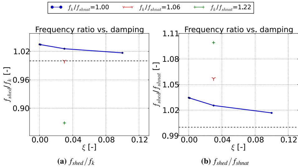
Figure 4.36: Free oscillation cylinder, evolution of the shedding frequency f_{shed} with respect to the damping for NLH computations (2 harmonics)
