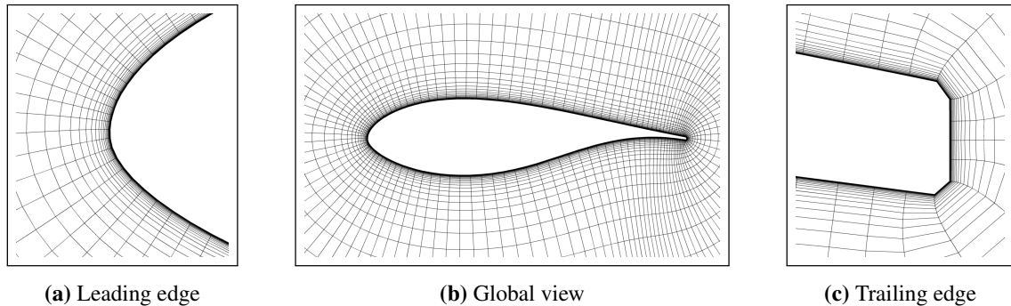
Figure 3.19: FFA-w3-241 original mesh
