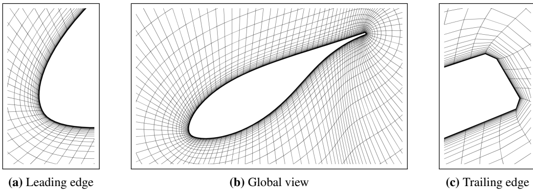
Figure 3.26: FFA-w3-241 deformed mesh, RBF+TFI, DLC2
