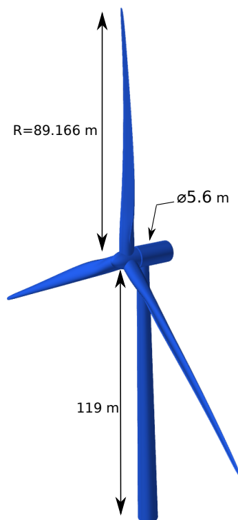
Figure 5.1: 3D view of DTU 10MW RWT
