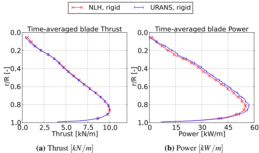
Figure 6.23: DTU 10MW RWT, radial evolution of time-averaged blade loads for rigid configuration.
