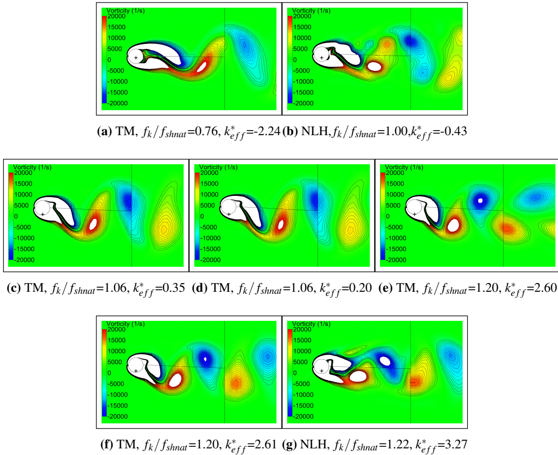
Figure 4.42: Vorticity contours of free cylinder motion at maximum displacement. Pre lock-in region: (a), (b), Full lock-in region: (c), (d), (e), Post lock-in region: (f), (g). Isolines increment corresponds to 1000 \text{ s}^{-1} . Solid lines represent block lines, and the cross sign is included at the center of the initial cylinder position
