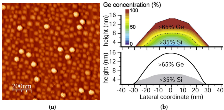
Figure 1.15: (a) AFM image of spontaneous quantum dots through deposition of 1.9 nm Si_{0.25}Ge_{0.75} on Si(001), unpublished result. (b) upper image is the real space chemical composition map for Ge domes; AFM line scans in lower image are taken on two Ge domes, before and after 31% H_2O_2 selective etching. It was concluded from these experiments that Si-rich core is present in the islands (The selective etching rate can be also dependent on strain state or crystallographic direction, which may modify these results). [29]
