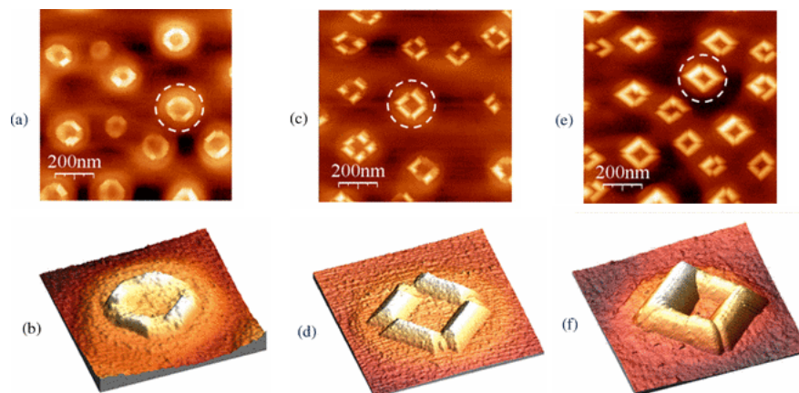
Figure 1.22: STM images ( 1 \times 1 \mu m^2 ) of the groups of closely spaced SiGe islands grown at 660 °C on a three-layered QD superlattice template with different thickness of deposited Ge:(a) 3.5 MLs, (c) 4 MLs, (e) 5 MLs. Image sides are oriented along the [011] directions. Figures (b), (d), and (f) correspond to three-dimensional representations of the fourfold symmetric QDMs, marked by dash circles in (a), (c), and (e), respectively[35].
