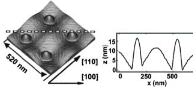
Figure 1.26: (Left) AFM image of the prepatterned Si substrate with 5 ML of Ge. (Right) Line scan in [100] direction along the dashed line in (a).
