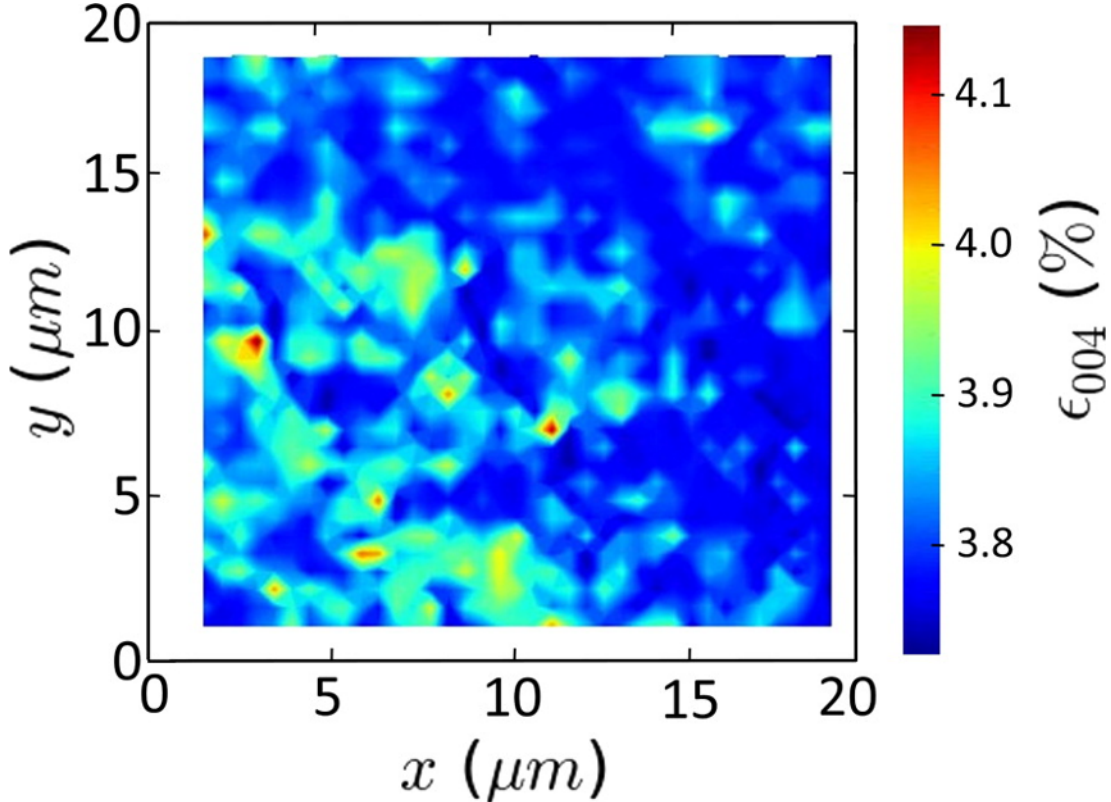
Figure 5.8: Map of a region of 20 \times 20 \mu\text{m}^2 of the strain of the 004 planes of the SiGe layer for sample A. The strain is calculated with strain-free silicon as a reference ( a_{\text{Si}} = 5.4309\text{\AA} ).
