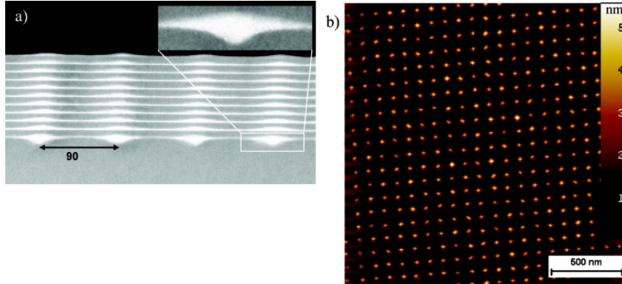
Figure 1.28: (a) TEM cross-section image of 10 period stacks of Ge islands and Si spacer layer (10 nm) deposited on a pre-patterned area, (b) AFM images of the surface of the same sample. The inset in (a) shows a closeup of a dot in the first layer. The comparison of the cross-sectional TEM micrographs and the AFM images demonstrates that the vertical and the lateral ordering is maintained after 10 periods on the pre-patterned substrate. [44]
