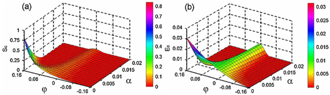
Figure 1.25: Critical size of Island nucleation (a) and energy barrier (b) as a function of \alpha and \varphi . The size is in unit of \gamma_0^2/\varepsilon_0^2 and barrier in unit of \gamma_0^2/\varepsilon_0 [39]
