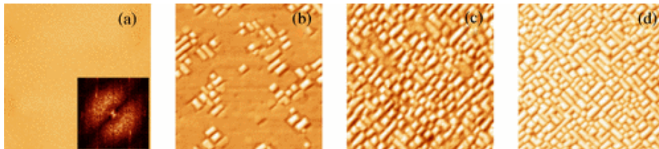
Figure 1.13: AFM images of a 5-nm-thin Si_{0.70}Ge_{0.30} layer (a) as grown (Fourier transform in inset), (b) after 18-h annealing, and (c) after 54-h annealing at 550 °C. (d) Image of a 8nm film after 18h annealing. The \langle 110 \rangle direction is horizontal. The scan area is 3\mu m \times 3\mu m , and the vertical scale for all the images is 32 nm. [28]
