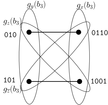
Figure 5.2 – The four infinite binary words avoiding AA.ABA.ABBA .
