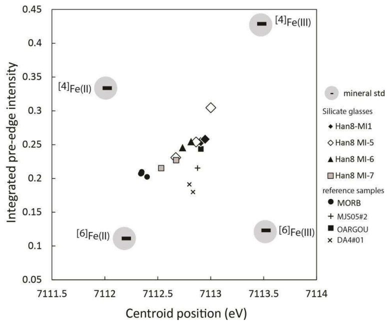
Fig. V.4 Pre-edge characteristics (centroid position and integrated pre-edge intensity) for trachytic silicate glasses (Han8), reference samples (MORB, OARGOU, MJS05#02, DA4#01) and iron standards, i.e. [4]Fe^{2+} (staurotide), [6]Fe^{2+} (siderite), [4]Fe^{3+} (sanidine), and [6]Fe^{3+} (andradite).
