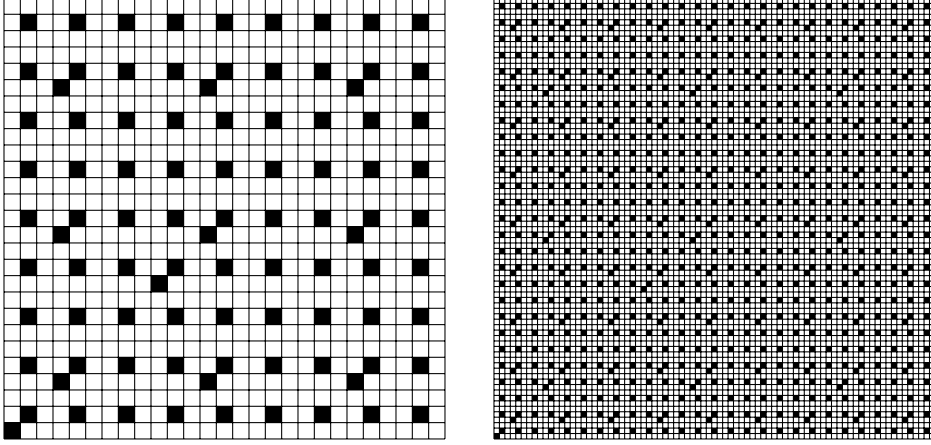
Figure 3.3: The patterns of order 3 and 4 of \mathbf{s}_v for v = (1, 1) .
