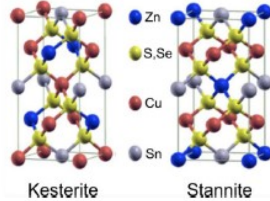
FIGURE 2.3 – Structures cristallines du \text{Cu}_2\text{ZnSn}(\text{S},\text{Se})_4
