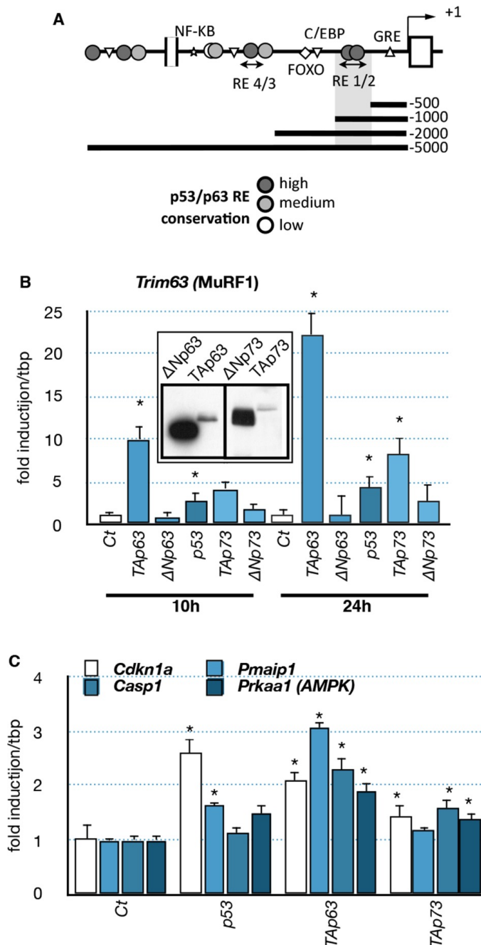
Fig. 6 – Effects of p53-family expression on Trim63 and p53-family target genes. (A) Schematic representation of the Trim63 promoter indicating the location of putative p53/p63 binding sites. (B, C) C2C12 myoblasts were transfected (inserted panel: western blot) with various p53-family members (TAp63 \gamma , \Delta Np63 \gamma , p53, TAp73 \beta , \Delta Np73 \beta ). Total C2C12 RNA was subjected to RT-qPCR after 10 hr or 24 hr of transfection and Trim63 (B) or p63 target (C, Cdkn1a, Pmaip1, Casp1, Prkaa1) expressions are shown relative to control-transfected cells. Bars are means of fold induction versus the control (Ct) with SD (n=3). *p<0.01 as calculated by a one-way ANOVA test followed by a Tukey post-test.
