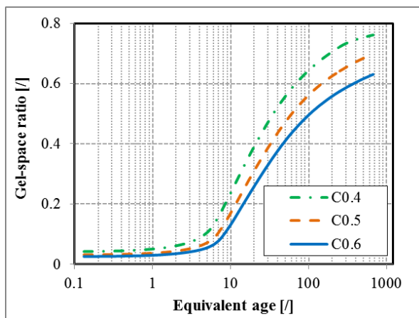
Figure 39 - Evolution of the gel-space ratio for different water-cement ratios (VCCTL V9.5).
