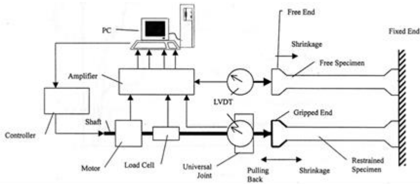
Figure 19. System for monitoring free and restraint shrinkages at the Israel Institute of Technology [41]
