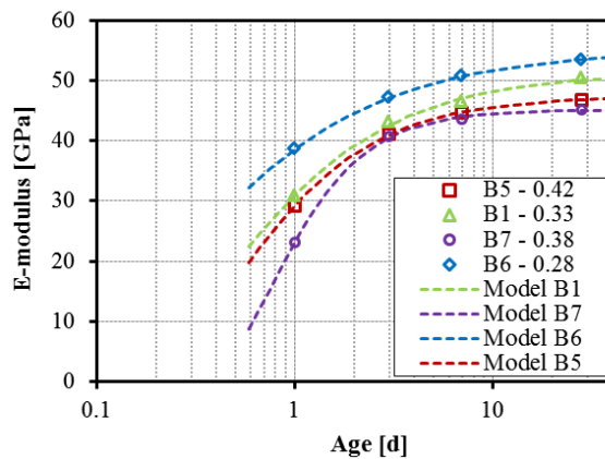
Figure 27 – E-modulus evolution for the different concrete composition of Le Roy [41] and modelling with Equation 27.
