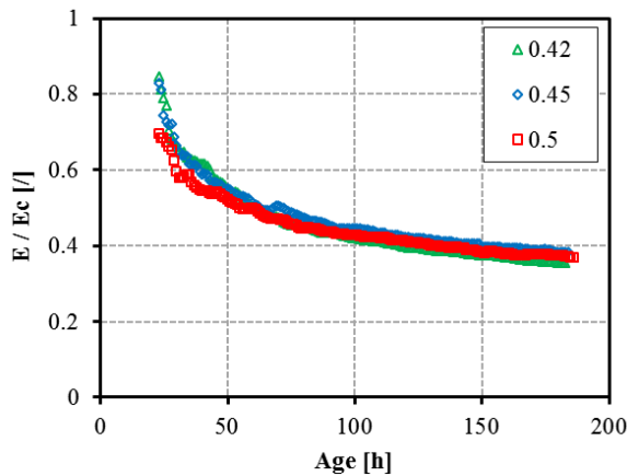
Figure 24 – Evolution of the ratio between the elastic modulus and the creep modulus for three cement pastes with different water-cement ratio (based on results of [40])
