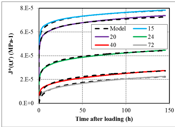
Figure 125 – Comparison between experimental creep curves, creep curves coming from a model inspired by the model code 2010.
