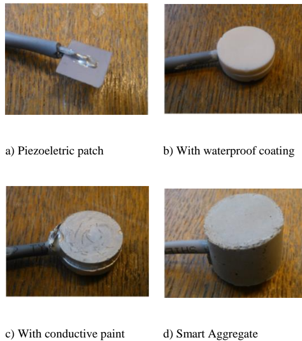
Figure 71 – SMAGs sensors (HF 3 ) for high frequency E-modulus monitoring.
