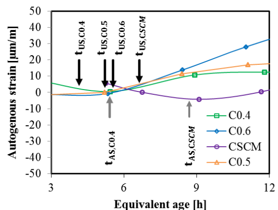
Figure 10 - Comparison between the final setting times determined with ultrasonic criterion (index US) and ASTM C304 (index AS) and the evolution of the autogenous strain during the setting process.
