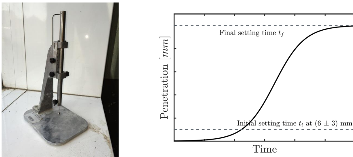
Figure 2 – The Vicat apparatus (left). Evolution of the needle penetration (right)
