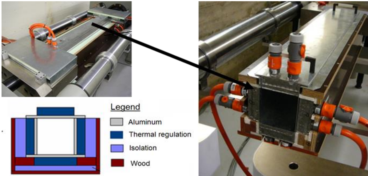
Figure 20 - Thermal insulation
