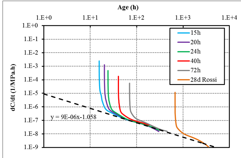
Figure 115 – Derivative of the creep function according to the age of the concrete for results obtained in this study and results obtained by Rossi [205].
