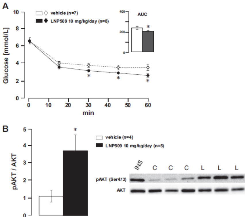
Fig. 4. LNP509 enhances insulin action in aged rats. Aged rats were treated for 7 days with vehicle or LNP509 ( 10 \text{ mg}\cdot\text{kg}^{-1}\cdot\text{day}^{-1} ip). A: insulin ( 1.5 \text{ U/kg} ) was administered ip at t_0 ; plasma glucose concentration was then determined after 15, 30, 45, and 60 min, and AUC was calculated from these values. Data are means \pm SE. * P < 0.05 vehicle ( n = 7 ) vs. LNP-treated rats ( n = 8 ). B: Akt activation was evaluated by the ratio Akt phosphorylated on Ser 473 (pAkt)/total Akt determined by Western blot analysis in hepatic tissues from rats after glucose challenge (C, vehicle-treated; L, LNP509-treated; INS, positive control with cultured PC12 cells stimulated with 100 \text{ nM} insulin for 30 min). Data are means \pm SE. * P < 0.05 vehicle ( n = 4 ) vs. LNP-treated rats ( n = 5 ).
