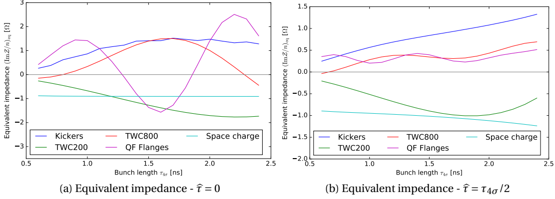
Figure 2.7 – The equivalent impedance (\text{Im}\tilde{Z}/n)_{\text{eq}} of the main SPS impedance sources (shown in Fig. 1.3), taken separately for a bunch distribution with \mu = 1 , and for small (left) and large (right) particle oscillation amplitudes \hat{\tau} .
