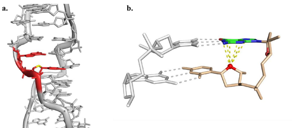
Figure 3.5. O4'- \pi stacking in a Z-DNA CpG step. (a) A CpG step (red) in the context of a Z-DNA helix (PDB: 1ICK res.: 0.95 Å; Dauter and Adamiak 2001) (b) Close-up showing the stacking between the cytosine ribose and the guanine in syn . Interatomic distances < 3.5 Å are represented by dashed lines. The atom-based colored guanine is residue 14 of chain B.
