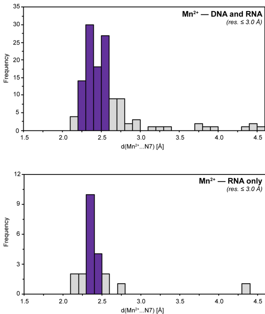
Figure S2. d(Mn 2+ ...N7) histograms derived from the PDB (May 2016; resolution ≤ 3.0 Å). These histograms emphasize the quasi-absence of coordination above 2.6 Å. For the first histogram, the largest number of data comes from nucleosomes (top).
