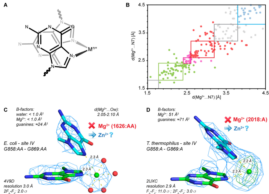
Figure 5. M^{n+} bound to a double N7 motif. (A) Schematic representation of this ion binding pattern with two guanines. Guanine-adenine combinations were also identified (Table 2). (B) 2D diagram showing \text{Mg}^{2+} distances with respect to each of the bound N7 atoms. The \text{Mg}^{2+} dots are colored according to their distance to the closest N7 atom (see Figure 2). The colored rectangular boxes frame the ions with respect to both coordination distances. (C) A \text{Mg}^{2+} placed close to site IV in an E. coli structure (Table 2). Though the coordination distance is correct, this ion assignment is ambiguous since ion and water B -factors < 1.0 \text{ \AA}^2 are not consistent with those of the guanines. These facts hint to the presence of a more electron dense ion such as \text{Zn}^{2+} . (D) \text{Mg}^{2+} placed close to site IV in a T. thermophilus structure. This ion assignment is ambiguous since, although the coordination distances are in agreement with those of \text{Mg}^{2+} , the F_o - F_c density (in orange) points to the presence of a more electron dense ion, possibly \text{Zn}^{2+} .
