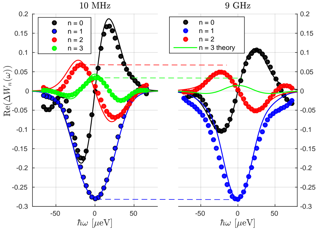
FIGURE 5.10: Left. \text{Re}(\Delta W_n(\omega)) (after deconvolution) for n from 0 to 3 for a sine drive at 10 MHz and 33 \pm 2 \mu V . Right. Same results for a sine drive at 9 GHz and V_{exc} = 31 \pm 1 \mu V . Full lines correspond to theory after deconvolution. Guides for the eyes enable to observe the relative weight of each harmonic. Although n=1 contributions have the same amplitude. The other harmonics have a higher weight for the classical drive.
