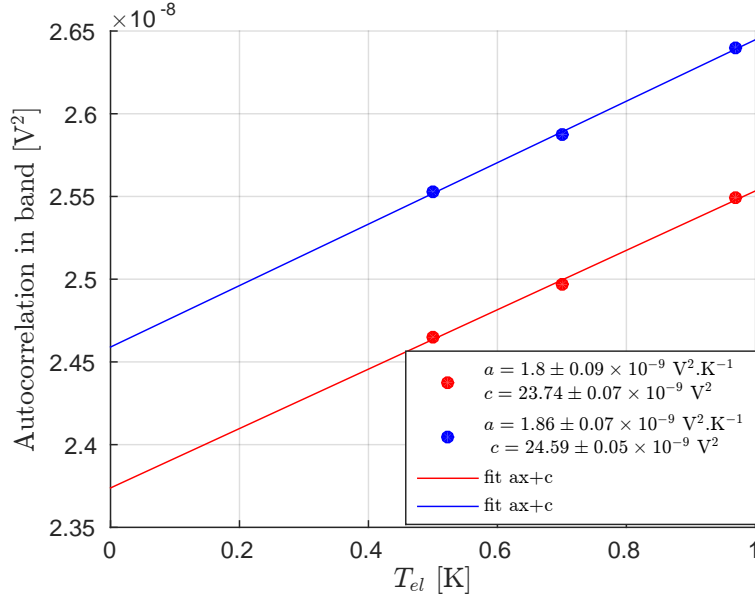
FIGURE 2.13: Autocorrelation power spectrum for each amplification output versus electronic temperature measured on a 50 \, \Omega load. From the offset we can deduce the voltage noise contribution of the HEMT amplifiers.
