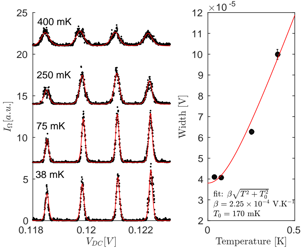
FIGURE 2.7: Left. I_\Omega versus V_{DC1} for different electronic temperatures. Drive frequency: 1.2 GHz, amplitude around eV_{\text{exc}} = \Delta/8 . After estimation of \Delta we can recover that \tau_e = 20 ps (or equivalently D = 0.35 ). Following [7], we fit each peak with a/\cosh^2((V - V_i)/2W) where V_i is the position of peak i and W the peaks width in Volts. Each curve is shifted upward for clarity. Right. Width W extracted from fits as a function of temperature. We fit this with \beta\sqrt{T^2 + T_0^2} where \beta^{-1} is the coupling between top gate and the energy level.
