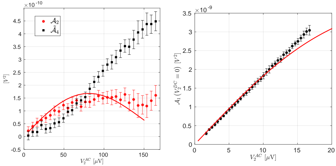
FIGURE 5.14: Left. Amplitude of oscillations with \delta\tau at n = 2 (i.e. \mathcal{A}_2 ) versus V_2^{\text{AC}} at fixed V_2^{\text{DC}} = 29.2\mu\text{V} . (Source at f = 9 GHz and amplitude \simeq 25\mu\text{V} ). Theory for \mathcal{A}_2 is in full red line. \mathcal{A} is extracted with a fit where the period is imposed. Actually we noticed another oscillation superimposing with twice the frequency so we fitted the noise oscillation with the sum of two sine (one at 18 GHz the other at 36 GHz) and plotted here the deduced two amplitudes. \tilde{\mathcal{A}}_4 is this second amplitude. Note that it is not exactly the same as \mathcal{A}_4 which would have required to impose only 36 GHz and to be able to calibrate the amplitude of the drive. The appearance of such doubling of oscillation might be due to some nonlinear effects in the mechanical dephaser generating a second harmonic on the probe. This non-linearity is negligible in the regime of the tomography where we imposed V_2^{\text{AC}} = 32\mu\text{V} on the probe. We still recover a linear behavior for \mathcal{A}_2 at low V_2^{\text{AC}} . Right. Amplitude of oscillations with \delta\tau at n = 1 ( \mathcal{A}_1 ) versus V_2^{\text{AC}} at fixed V_2^{\text{DC}} = 0\mu\text{V} . Source at 10 MHz with \simeq 31\mu\text{V} amplitude. \mathcal{A} is extracted with a fit where the period is imposed. Theory is in plain red line. The linear regime is nicely resolved and fits to theory to a large extent.
