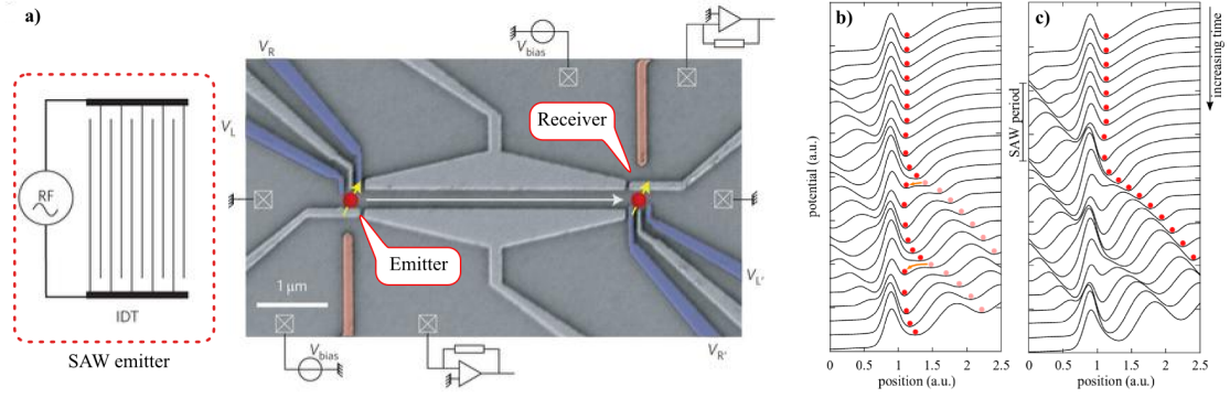
FIGURE 1.6: Figure extracted from [40, 41] a) . Scanning electron microscope image of the device. b) and c) . Time evolution of the dot potential for two different amplitudes of SAW excitation. The time increases going from top to bottom traces. In c) the amplitude of SAW drive is large enough and deeper moving quantum dots are defined compared to b). Tunneling back of the electron to the source dot is negligible in c) so probability to transfer exactly one electron converges to one.
