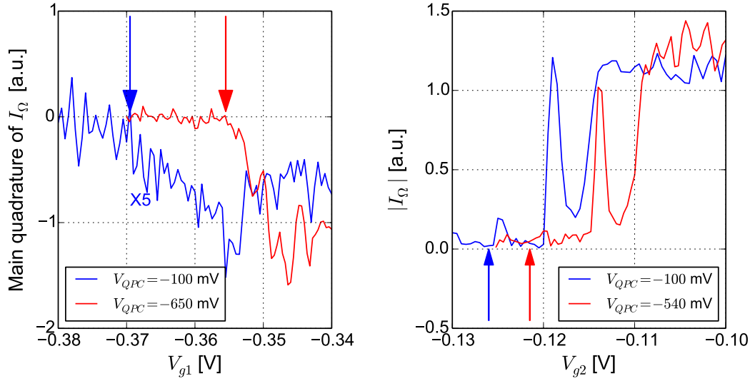
FIGURE 3.10: Illustration of the iterative method first measurements to find a working triplet point V_{QPC} , V_{g1} , V_{g2} . Left. Main quadrature of I_{1\Omega} as a function of V_{g1} when the QPC is fully closed (red) and when inner channel is partitioned (blue line is multiplied by 5). The signal is small because almost no current, apart from parasitic coupling, is injected from the dot to the inner edge. Part of this current also comes from capacitive coupling between edges. Right. Here the current is large enough so we can plot the modulus of I_{2\Omega} as a function of V_{g2} . Arrows represent V_g values we chose as the closing of the dots. From both figures, we deduce we have to apply a shift of 14 mV for source 1 and 4.5 mV for source 2 to the initial values of V_g corresponding to D \approx 0.4 .
