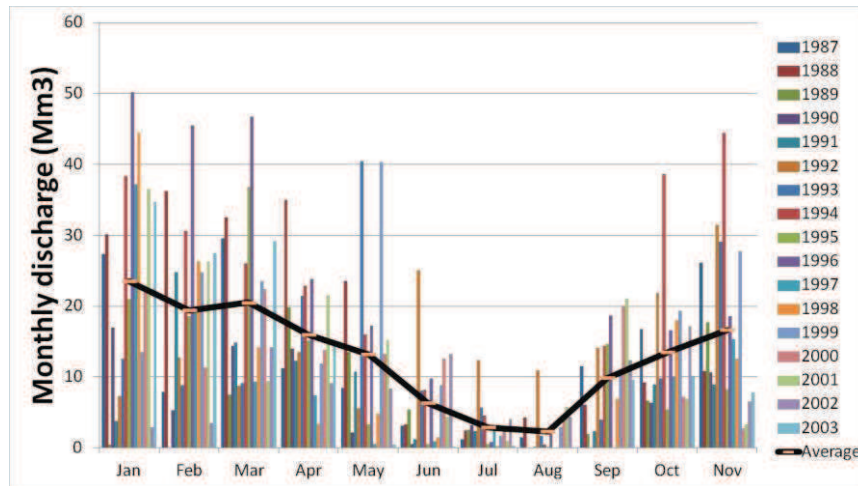
Figure 4–6 Monthly releases from the Montahut hydropower plant (adapted from Vier and Aigoui, 2011)
