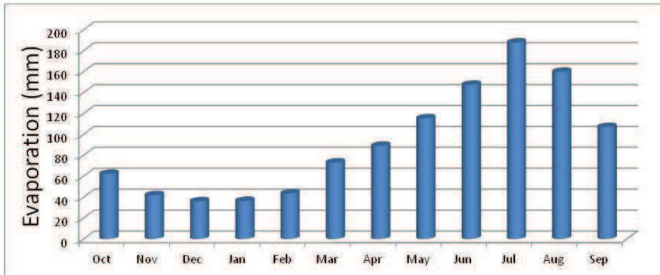
Figure H-2 Monthly evaporation rates on the Monts d'Orb reservoir
