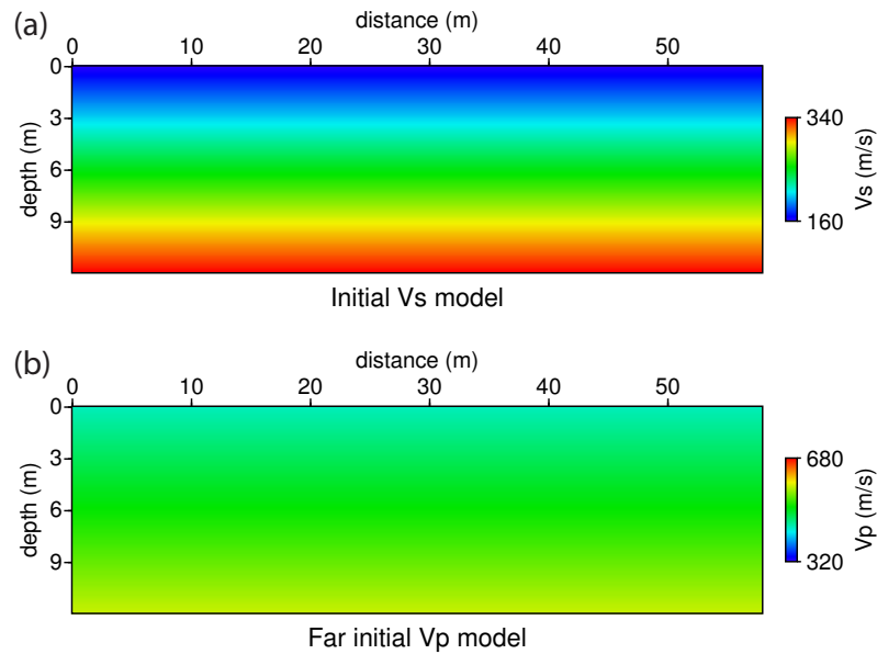
Figure 3.26: Initial shear wave velocity model (a) and initial far P-wave velocity model (b) used for inversion.
