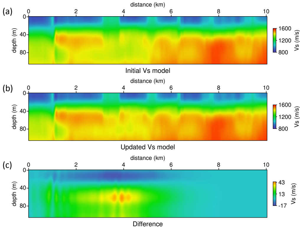
Figure 4.26: Initial shear velocity model (a), updated shear velocity model after FWI (b), and the difference between the two (c).
