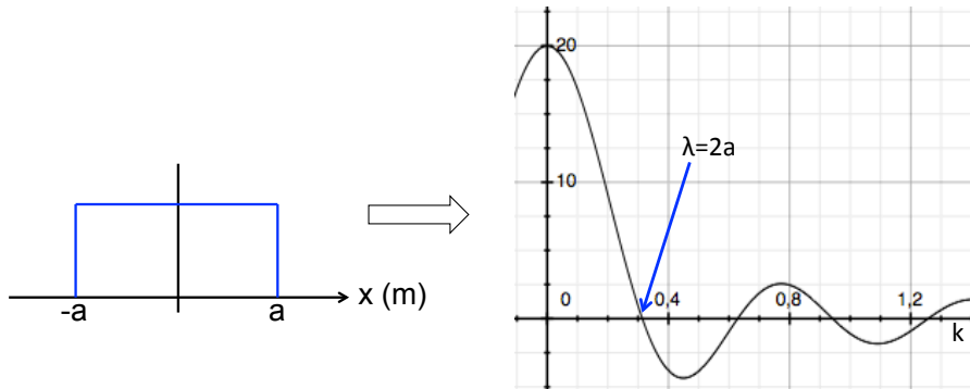
Figure 4.17: Schematic of spatial filter and impulse response applied to the data due to the array acquisition.
