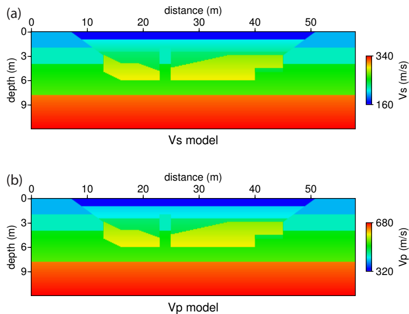
Figure 3.1: The true S-wave (a) and P-wave (b) velocity models used to create the synthetic dataset for this investigation. A homogeneous density of 1000 \text{ kgm}^{-3} is considered. Models used with permission from Pérez Solano et al. (2014).
