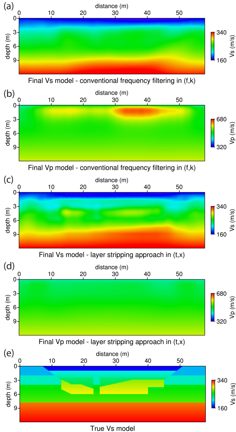
Figure 3.27: Final shear wave and P-wave velocity models obtained for the conventional low-to-high frequency FWI and a (\omega, k) domain misfit function (a-b); and for layer stripping FWI with the (t, x) domain misfit function (c-d). The true shear velocity model (e) is shown for comparison.
