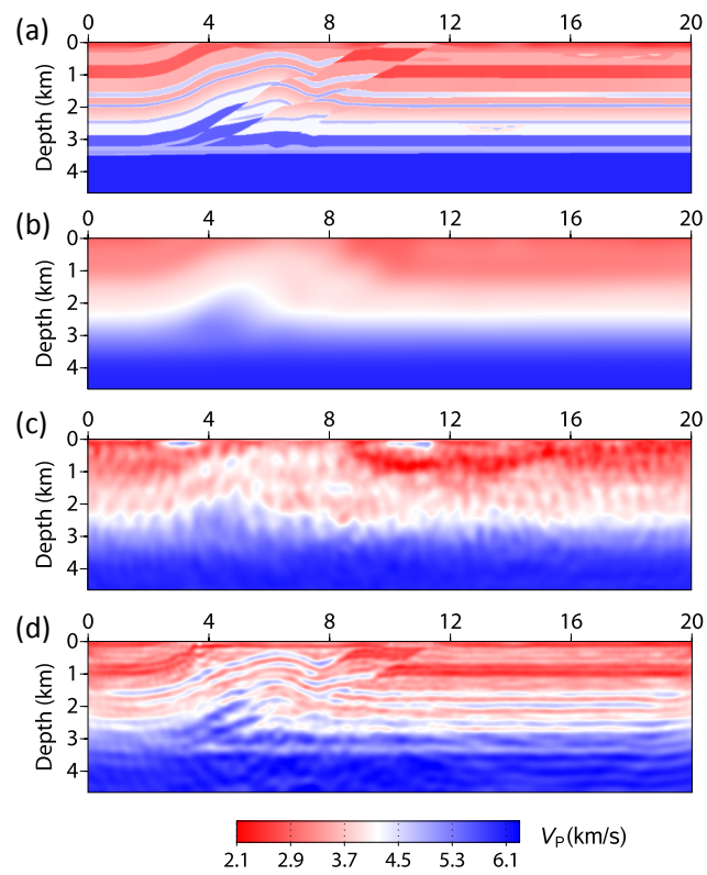
Figure 1.15: True model (a), initial model (b), and the resulting models from 2D frequency domain FWI without (c) and with (d) the implementation of a time-damping approach. Figure modified from Brossier et al. (2009) .
