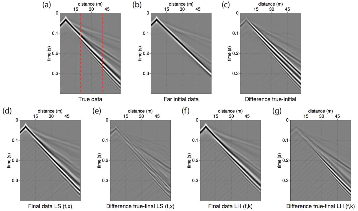
Figure 3.24: Example of a common shot gather for the true data (a); the far initial data (b) and the difference to the true data (c); the final data after a layer stripping FWI with a (t, x) domain misfit function (d) and the difference to the true data (e); the final data after conventional low-to-high frequency FWI with a (\omega, k) domain misfit function (f) and the difference to the true data (g). A small gain is applied to the true data (a) for visualization purposes, all other figures (b) to (f) have the same color scale.
