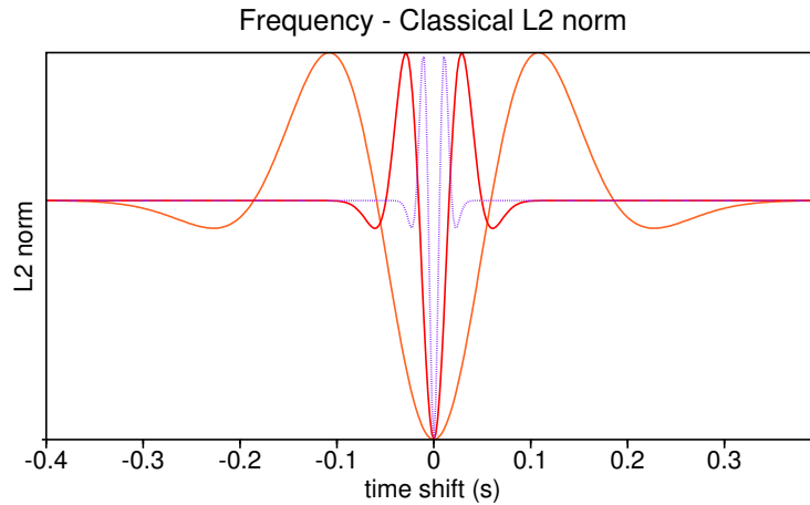
Figure 1.11: Classical difference-based L2 norm misfit of two Ricker wavelets, both with a peak frequency of 4\text{ Hz} (orange), 15\text{ Hz} (red) and 40\text{ Hz} (dashed purple). The wavelets are time shifted compared to each other, simulating a velocity difference between the true and estimated velocity models. The convexity of the misfit shape depends on the frequency content of the data.
