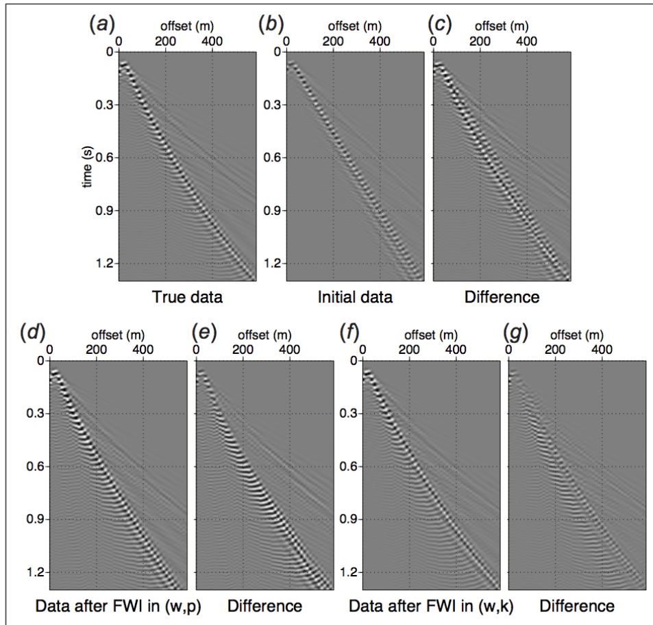
Figure 2.6: The true data with strong energetic dispersive surface waves (a); the initial data for the two-layered model (b) and the difference to the true data (c); the final data after FWI in the \omega - p domain (d) and the difference to the true data (e); and the final data after FWI in the \omega - k domain (f) and the difference to the true data (g). In this example, the FWI performs better in the \omega - k domain than in the \omega - p domain.
