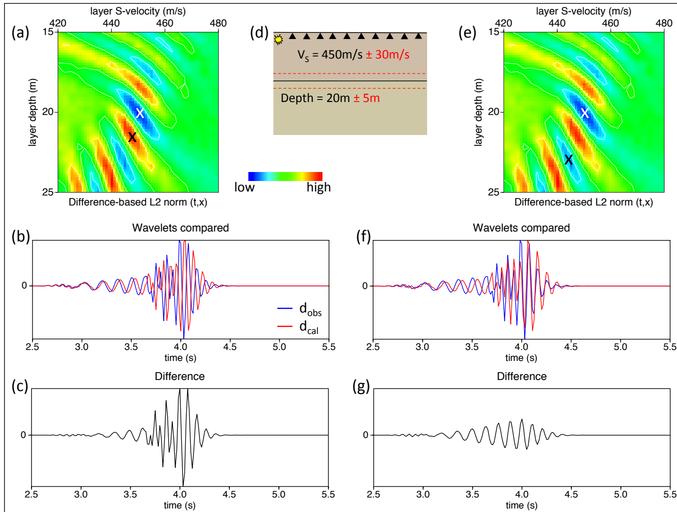
Figure 1.10: 2D misfit maps for the classical difference-based misfit are shown in (a) and (e), as two model parameters are perturbed in (d). The white cross marks the global minimum. The perturbed ( d_{cal} ) and reference ( d_{obs} ) data traces are shown in (b) and (f) for the two cases marked by the black cross in (a) and (e) respectively. The data difference is shown in (c) and (g) respectively. The difference in (g) is smaller because the wrong phases match up in (f) causing a local minima.
