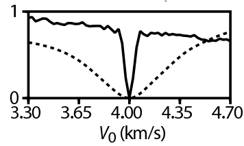
Figure 1.13: The misfit for a full dataset (solid) and a damped dataset (dashed) as a function of one model parameter. Figure modified from Brossier et al. (2009) .
