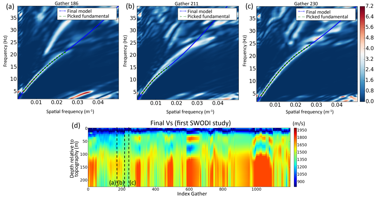
Figure 4.15: Selected CMP gathers in the (\omega, k) domain located before (a), during (b) and after (c) a lateral velocity discontinuity retrieved by both shear velocity models just after the first 2 km. The final model of the first study is shown for reference, on which the CMP locations are marked by the dashed lines. The picked fundamental mode (green dashed line) and the fundamental mode of the final model obtained by the first study (blue solid line) are plotted. Note that a normalisation is applied on both frequency and spatial frequency axis for better visualisation of the spectrum.
