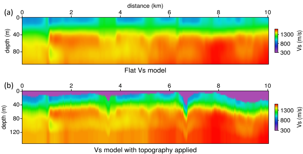
Figure 4.31: Shear velocity model without (a) and with (b) topography, used for forward modelling with the curvilinear propagator. Note that the vertical axis is exaggerated.
