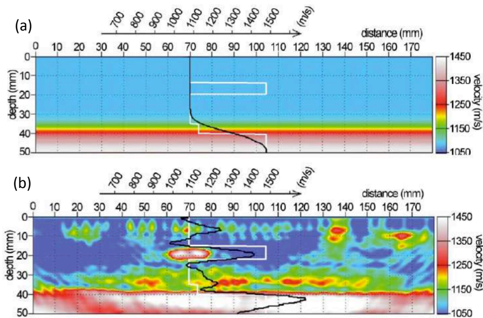
Figure 1.12: Image of the initial Vs model (a), and the recovered Vs model using FWI (b). The white velocity profile is for the true lab-scale medium, and the black velocity profile is shown for the initial and final estimated velocity models. Artifacts in the result are related to the imperfect source wavelet inversion and noise during the "real" experiment. Figure modified from Bretaudeau et al. (2013).
