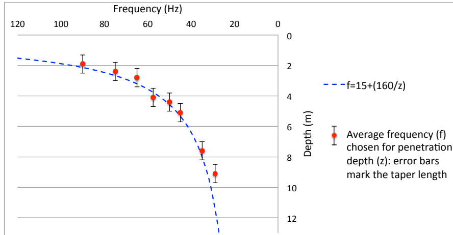
Figure 3.17: The relation given in Equation 3.8, and considering the initial shear velocity model used for FWI, is plotted (blue dashed). The average frequency and relative penetration depth parameter values used for layer stripping FWI are also plotted (red) with depth error bars representing the taper length.
