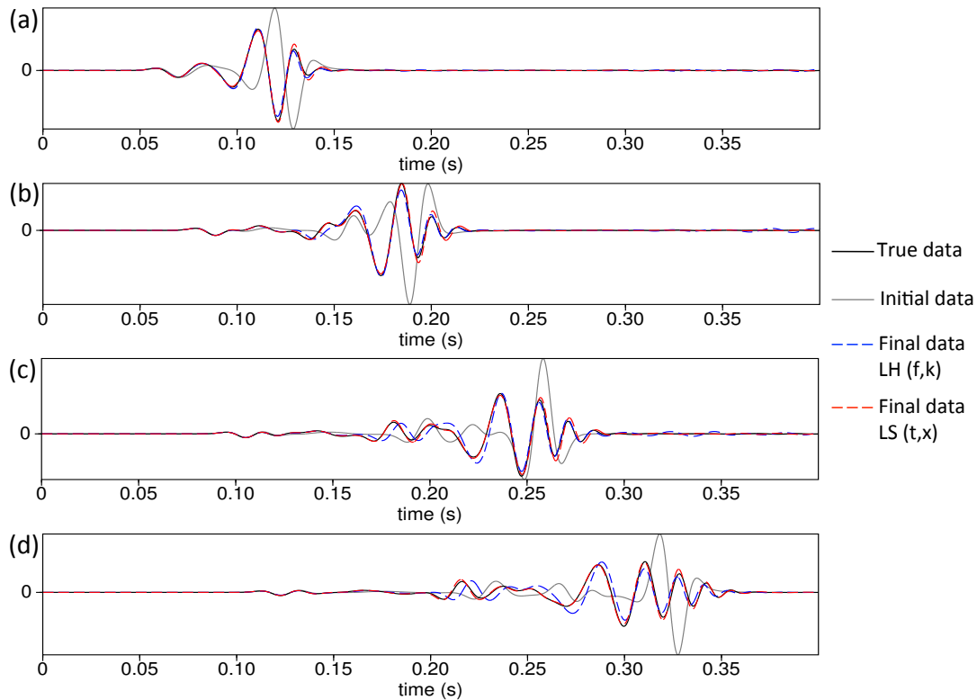
Figure 3.11: Comparison of a single trace at varying offsets of 15 m (a), 25 m (b), 35 m (c), and 45 m (d), located by the red dotted lines on the common shot gather in Figure 3.9. The compared traces are: the true data (black), the initial data (grey), the final data after conventional low-to-high (LH) frequency FWI with an (\omega, k) domain misfit function (blue dashed), and the final data after layer stripping (LS) FWI with a (t, x) domain misfit function (red dashed).
