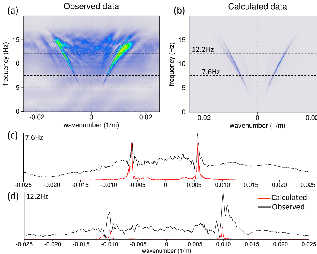
Figure 4.22: A selected common shot gather in the middle of the line, filtered between 4 - 15 \text{ Hz} , shown for the observed data (a) and the calculated data (b) in the frequency-wavenumber (\omega, k) domain. Two traces, located by the black dashed lines, at a frequency of 7.6 \text{ Hz} (c) and 12.2 \text{ Hz} (d) are selected and compared. The peak of the fundamental mode appears to correlate well between observed and calculated data. Note that the amplitudes of the observed and calculated data are shown at the same scale.
