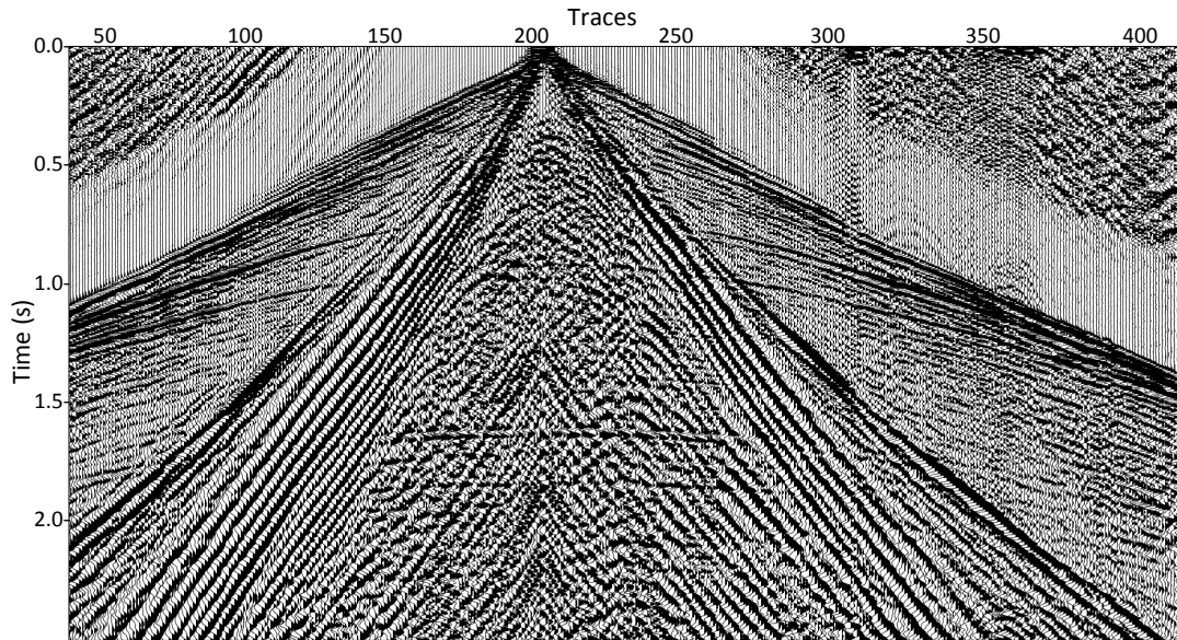
Figure 4.5: Detail of a common shot gather (shot 198) illustrated in wiggle form with an AGC applied.
