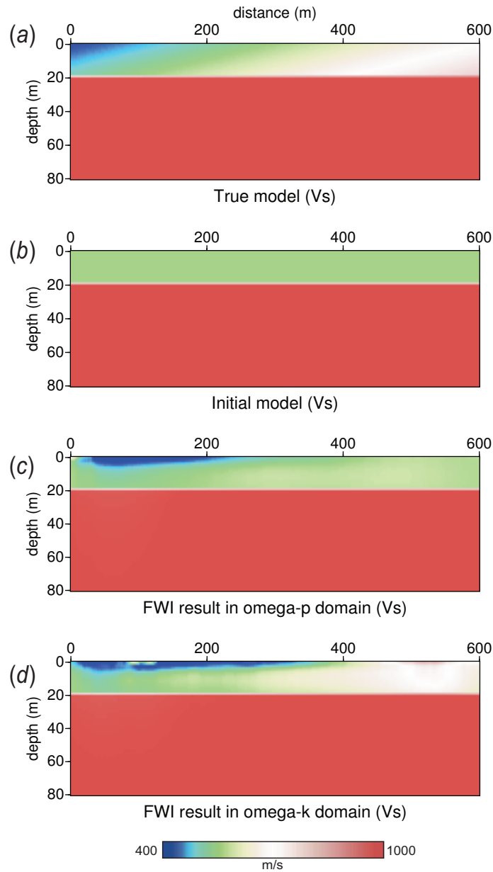
Figure 2.5: Model description and reconstruction: the top two models represent the true model with an oblique gradient (a) and the initial two-layered model (b). The bottom two models represent the reconstructed model when performing FWI in the \omega - p domain (c) and the reconstructed model when performing FWI in the \omega - k domain (d). Please note that in this example the horizontal gradient reconstruction is more successful for FWI in the \omega - k domain.
