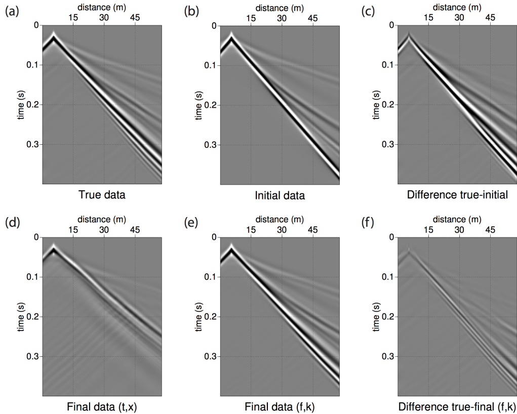
Figure 3.2: Example of a common shot gather for the true data (a); the initial data (b) and the difference with the true data (c); the final data after FWI using the conventional (t, x) domain misfit (d); the final data after FWI using the (\omega, k) domain misfit and depth preconditioning (e) and the difference with the true data (f). A small gain is applied to the true data (a) for visualization purposes only, all other figures (b) to (f) have the same color scale as (a).
