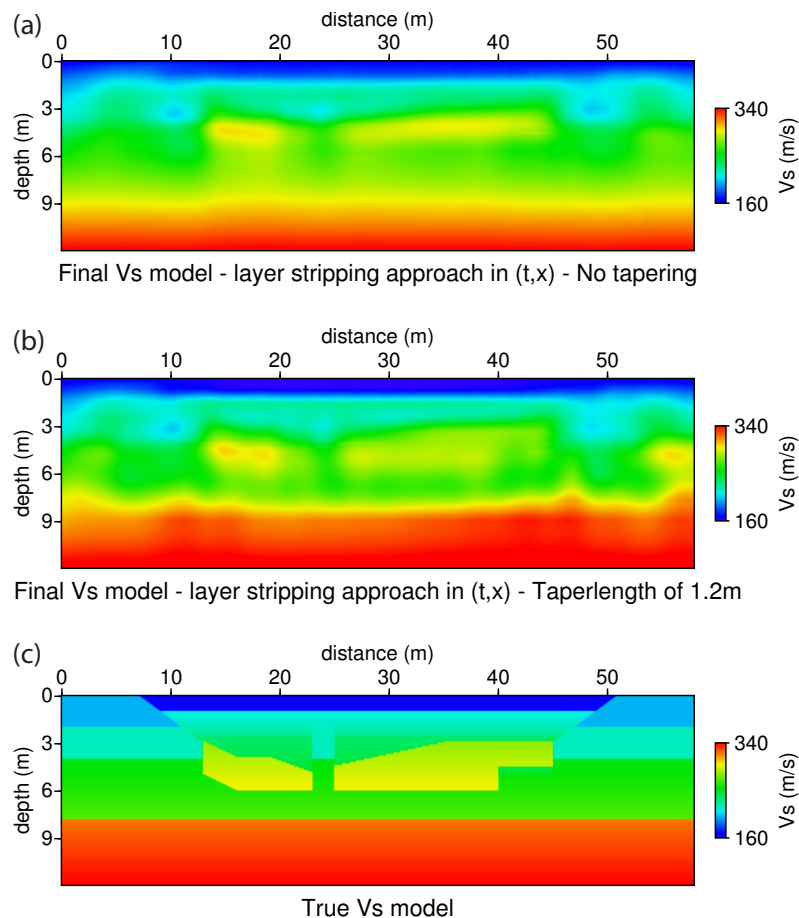
Figure 3.18: Final shear velocity models using the layer stripping approach, and a misfit in the (t, x) domain: when no depth window tapering is applied (a), and when a depth window tapering of 1.2 m is applied (b). The true shear velocity model is shown for reference (c). The tapering reduces the sensitivity to the chosen depth parameters, and improves the inversion result. Similar results are obtained when the misfit in the (\omega, k) domain is used.
