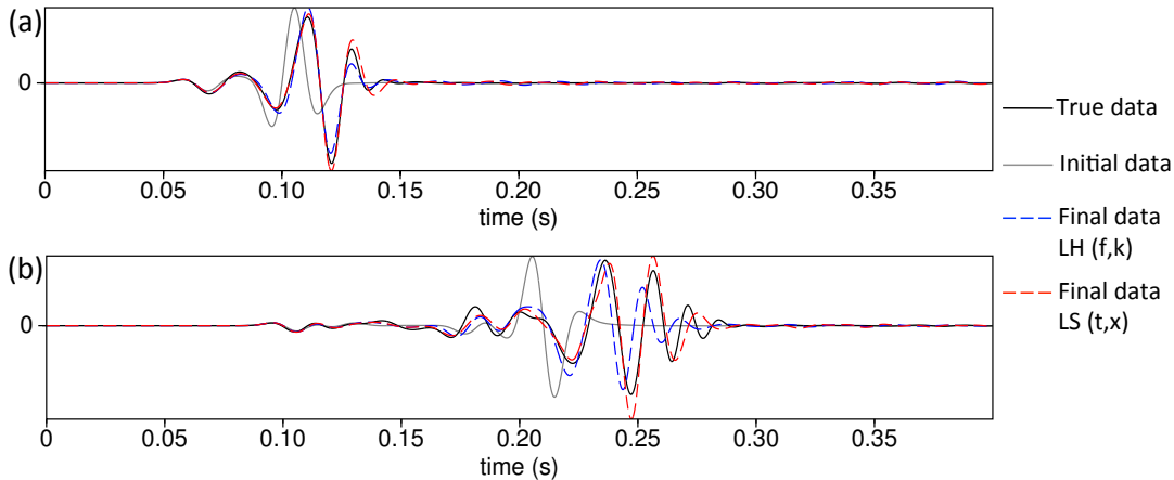
Figure 3.25: Comparison of a single trace at short offset (a) and at far offset (b), located by the red dotted lines on the common shot gather in previous Figure 3.24. The traces compared are: the true data (black), the initial data (grey), the final data after conventional low-to-high (LH) frequency FWI with an (\omega, k) domain misfit function (blue dashed), and the final data after layer stripping (LS) FWI with a (t, x) domain misfit function (red dashed).
