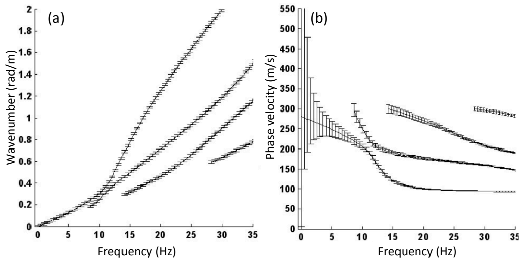
Figure 1.6: Dispersion curves for a synthetic three-layered model. The uncertainty distribution for picking the spectral maxima of the fundamental and higher modes is shown for the frequency-wavenumber ( \omega - k ) domain (a), and for the frequency-phase velocity ( \omega - c ) domain (b). Although the different modes appear to merge, they do not intersect. Image modified from Socco and Strobbia (2004) .
