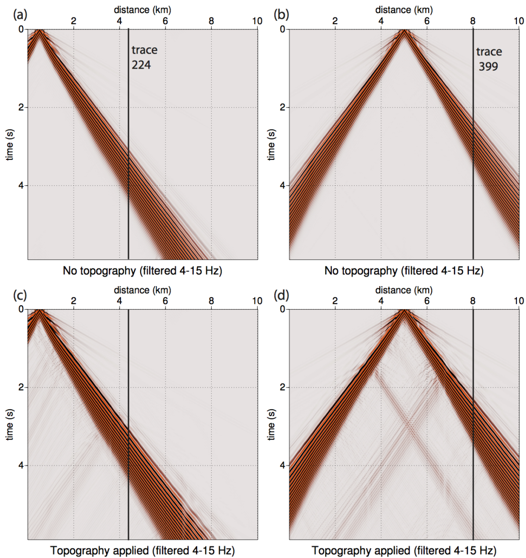
Figure 4.32: Example common shot gathers for data modeled without topography (a-b) and with topography (c-d) using the curvilinear propagator. The data are low bandpass filtered between 4 – 15 Hz . A comparison of individual traces, located by the solid black line is shown in Figure 4.34.
