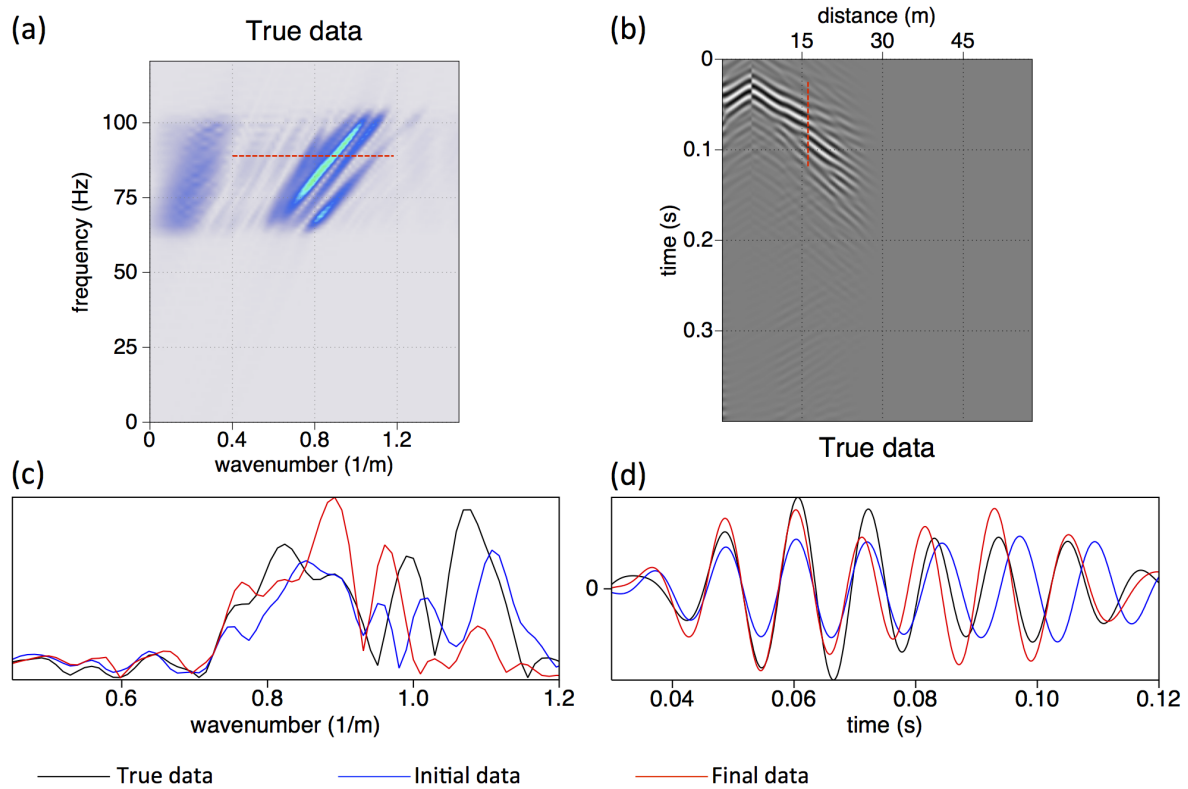
Figure 3.21: Comparison of the true data, after offset windowing and frequency filtering according to the first frequency band step, at the moment when the misfit is computed, for the misfit function in the (\omega, k) domain (a) and the misfit function in the (t, x) domain (b). An example trace, is plotted for the true data (black), the initial data (blue) and the final data after the first frequency band step has been inverted (red), for the (\omega, k) domain misfit function (c) and the (t, x) domain misfit function (d). The chosen traces are marked in red on (a) and (b) respectively. One can observe that cycle skipping occurs in (c) in the (\omega, k) domain but not in (d) in the (t, x) domain.
