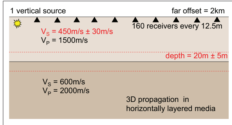
Figure 2.2: Design of a simple model with two parameters defined as the depth of the interface and the S-wave velocity in the upper layer
