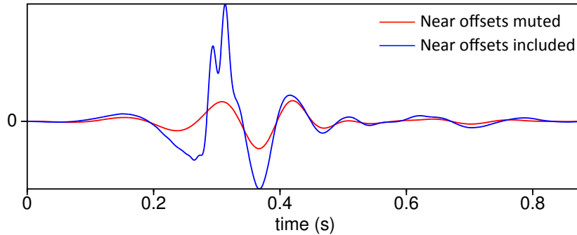
Figure 4.20: Source function obtained with a wide mute allowing surface waves and the direct wave: with near offsets removed (red); and near offsets included (blue).
