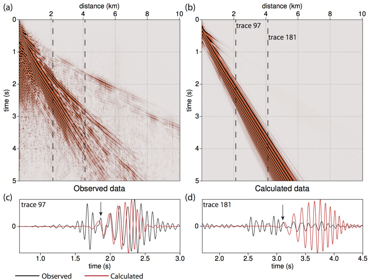
Figure 4.21: A selected common shot gather at the beginning of the line, filtered between 4 - 15 \text{ Hz} , shown for the observed data (a) and the calculated data (b) in the time-offset ( t, x ) domain. Two traces, located by the black dashed lines, are visualized and compared in (c) and (d). The arrow marks the start of the surface wave package. Although the initial phases of the surface waves appear to roughly match, cycle-skipping of surface wave phases is also present at both offsets. Note that the amplitudes of the observed and calculated data are shown at the same scale.
