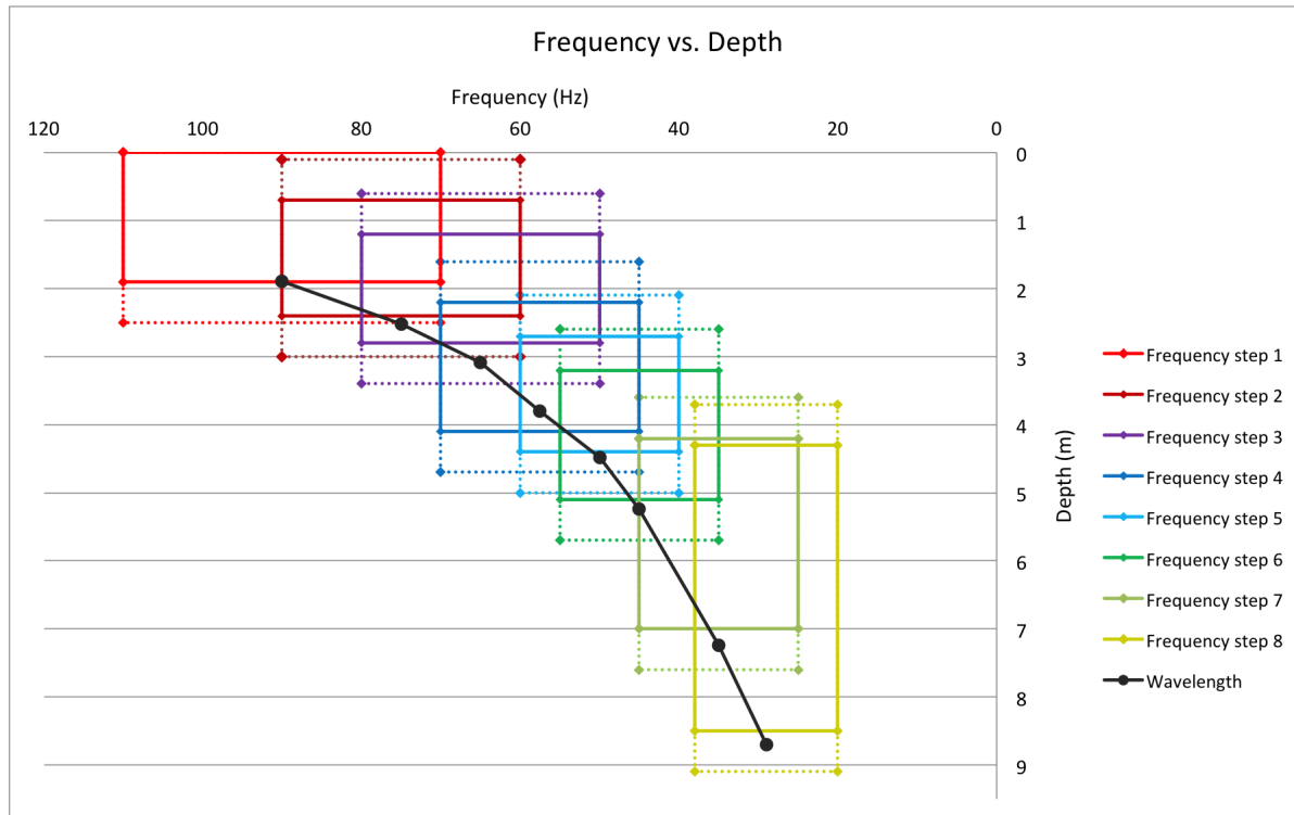
Figure 3.16: Plot of frequency band against depth window parameters used for FWI with a layer stripping approach to produce the results in Figures 3.6 and 3.7. Each color corresponds to a frequency band inversion step. The dotted lines correspond to the extent of the taper outside of the depth value chosen; for simplicity the extent of the inside taper, equivalent in length, is not plotted. The tapering implemented for the frequency windowing is also not illustrated. An estimation of the average wavelength is plotted in black, obtained from average frequency and shear velocity values using Equation 3.6.
