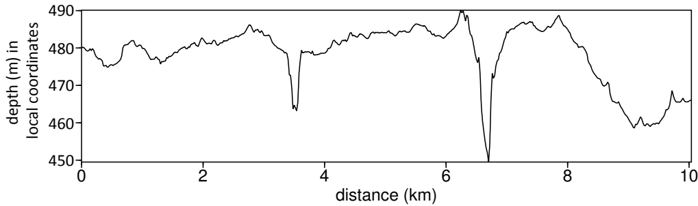
Figure 4.29: Topography profile of the acquired line for the real data considered in Chapter 4, showing the location of the two canyons. Note that the vertical axis is exaggerated.
