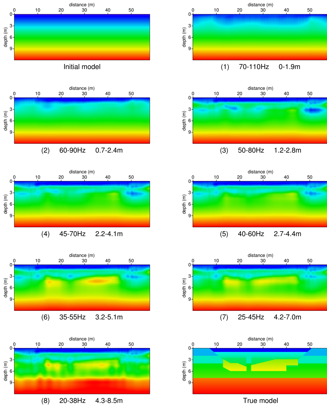
Figure 3.6: Evolution of the resulting shear velocity model at each frequency band step (1) to (8) when using the misfit function in the (\omega, k) domain. For each step a frequency band and depth layer are given as parameters to filter the data and window the model update. The depth values mark the mid-point of the 1.2 m taper applied during the depth windowing. This layer stripping strategy progressively updates the model in a top-to-bottom manner, using a high-to-low frequency approach. The initial and true shear velocity models are also shown for reference.
