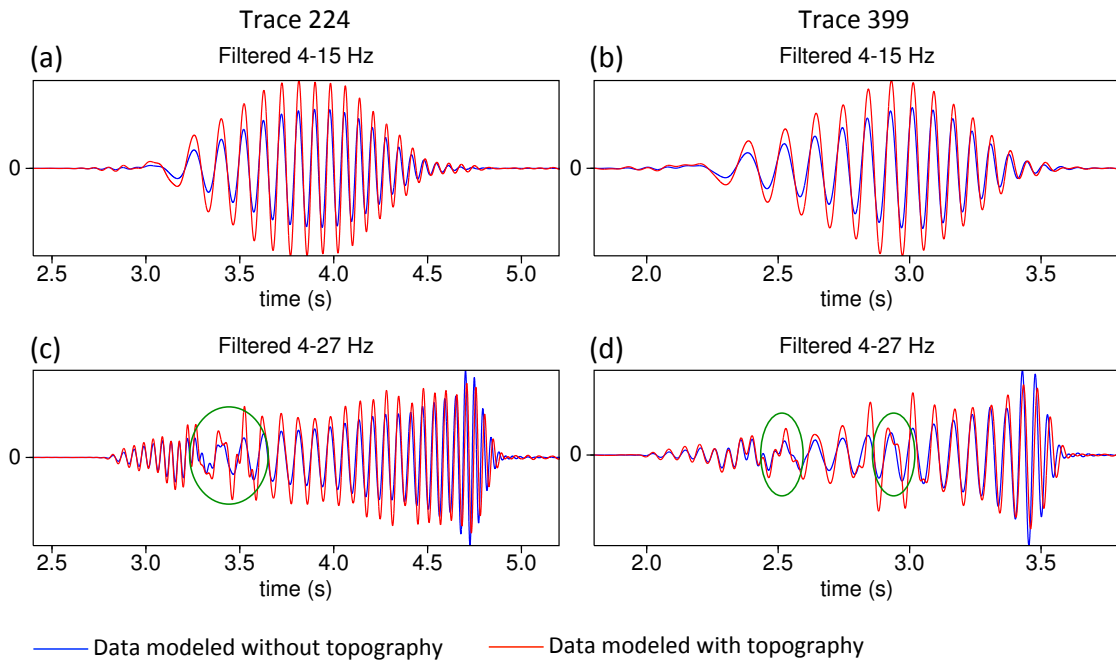
Figure 4.34: Comparison of individual traces, located by the solid black lines in Figure 4.32, for data filtered between 4 – 15 Hz in (a-b) and for data filtered between 4 – 27 Hz in (c-d). The blue line represents data modelled without topography, and the red line represents data modelled with topography. The green circles highlight phase differences visible in the higher frequency band.
