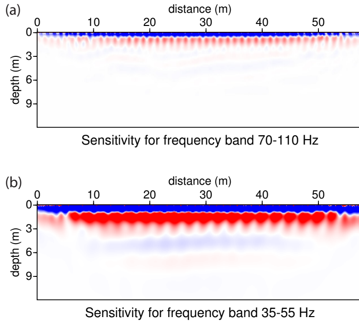
Figure 3.4: Sensitivity kernels, summed over all sources and receivers, for data of frequency band 70 – 110 Hz (a) and 35 – 55 Hz (b). One can observe that with the lower frequency band the model is updated at greater depths, but is also of lower resolution. The color scale for the amplitude is the same for both sensitivity kernels. Note that a wider frequency range is chosen for the high frequency window, due to a lower amplitude of the data spectrum at these frequencies, to compensate for an equal amount of energy (see section 3.2.4).
