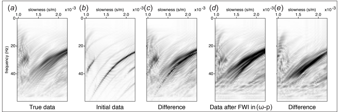
Figure 2.8: The true data in the (\omega, p) domain (a); the initial data and the difference to the true data (b,c); the recovered data after FWI in the (\omega, p) domain and the difference to the true data (d,e). Some particularly energetic packets can be observed.
