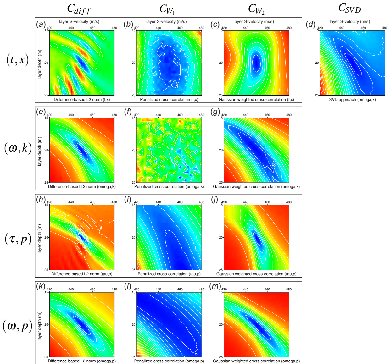
Figure 2 Two-parameter grid analysis for all misfit functions tested in this study (a-m), for an observed dataset with the true global minimum at 450 m/s layer S-velocity and 20 m layer depth.
