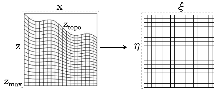
Figure 4.30: Initial Cartesian models with topography are transformed into models with curvilinear coordinates and having a flat topography. Modified from Tarrass et al. (2011).
