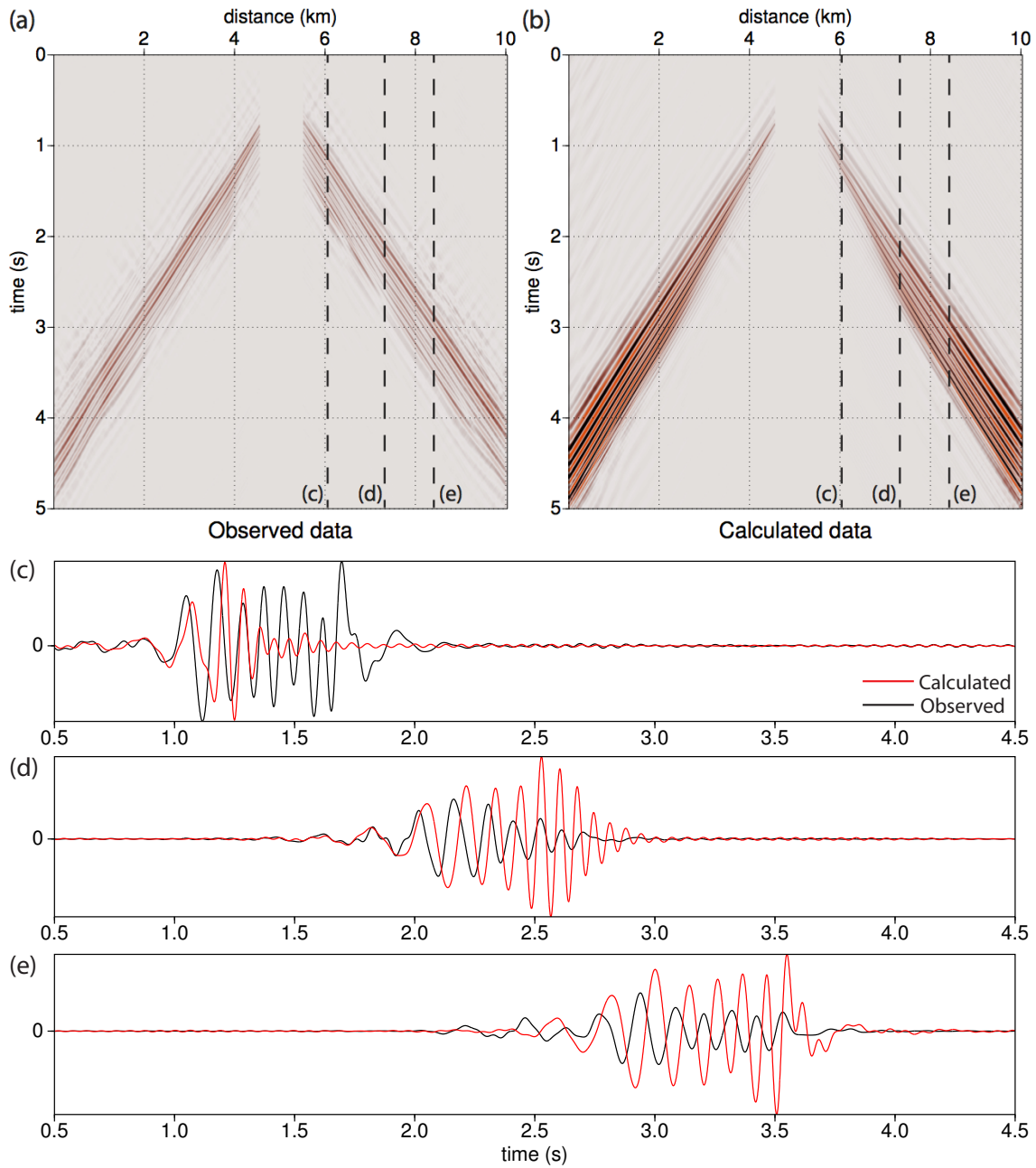
Figure 4.25: The same common shot gather as in Figure 4.24 is shown for observed (a) and calculated (b) data, transformed back to the time-offset ( t, x ) domain, after a weighting has been applied in the (\omega, k) domain. Example traces comparing observed and calculated data, located by the black dashed lines, are shown in (c) to (e). Note that the amplitudes of the observed and calculated data are shown at the same scale.
