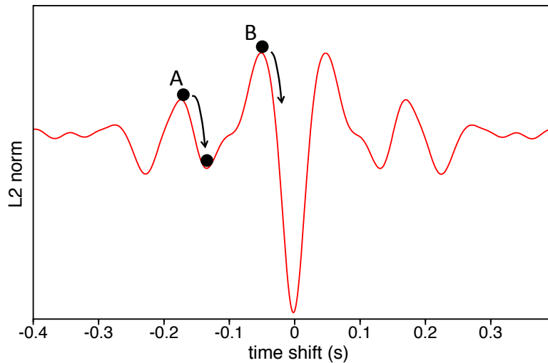
Figure 1.9: The shape of the classical difference-based L2 norm misfit function for a 1D example, produced from comparing two wavelets that are time shifted compared to each other, simulating a velocity difference between the true and estimated velocity models. When the initial model is at point A, the inversion will converge towards a local minimum and remain stuck there. However when the initial model is closer to the true model at point B, the inversion will converge towards the global minimum.
