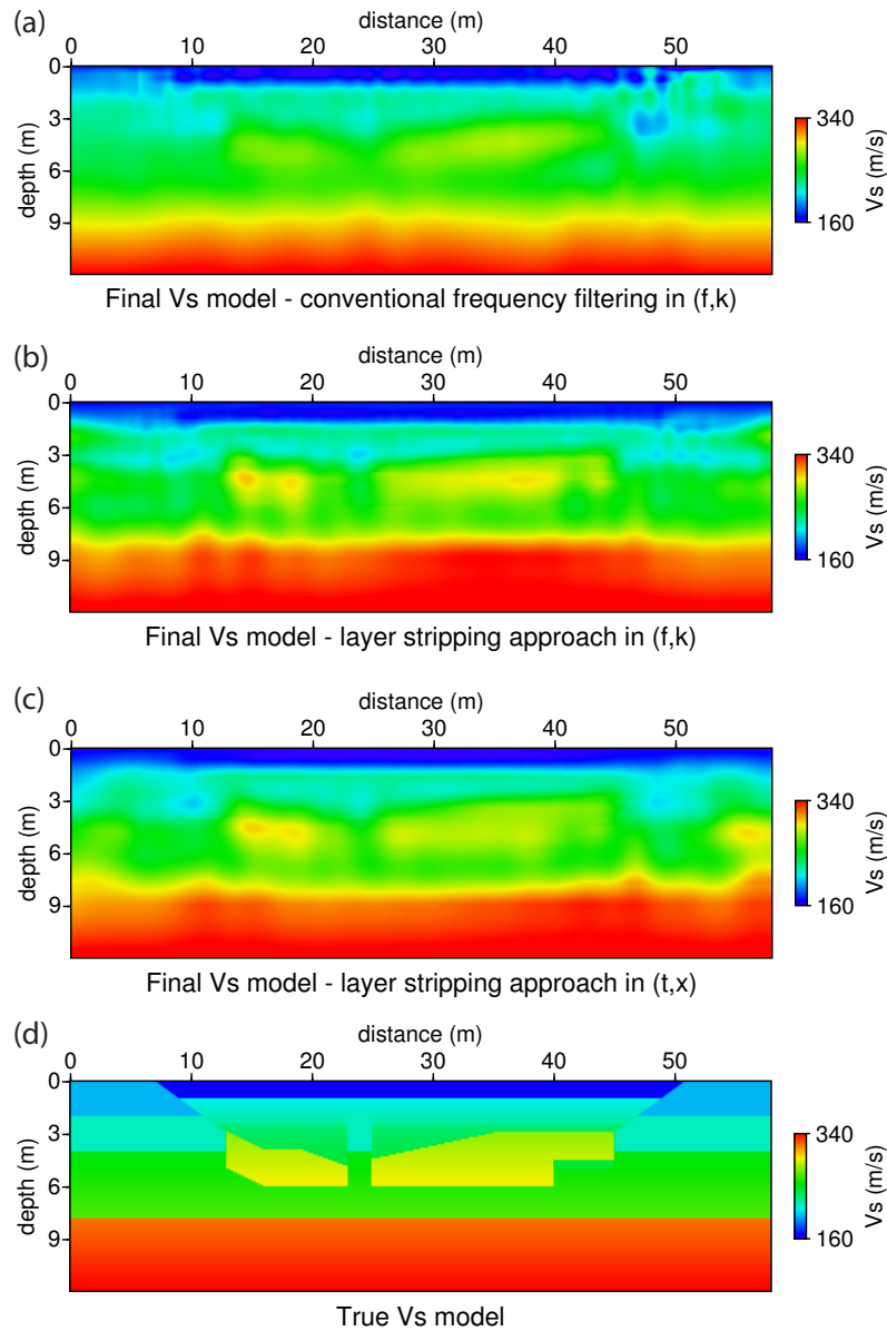
Figure 3.8: Comparison of final shear velocity models obtained after FWI using a low-to-high frequency approach and a misfit function in the (\omega, k) domain (a); using a layer stripping approach and a misfit function in the (\omega, k) domain (b); using a layer stripping approach and the conventional misfit function in the (t, x) domain (c). The true shear velocity model (d) is shown below for reference.
