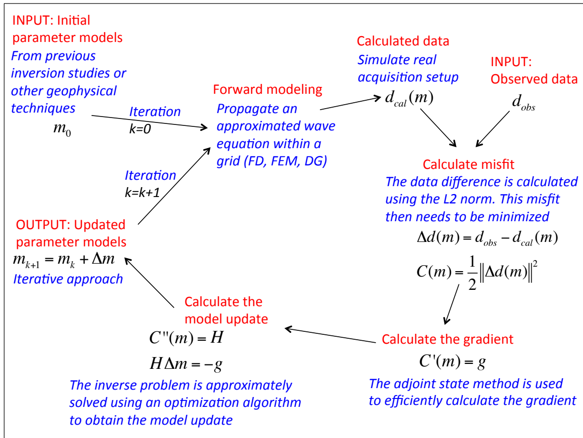
Figure 1.7: A generalized workflow for conventional FWI. The method requires a priori information in the form of initial models, to compute synthetic data which are then compared to the observed data. The data difference is minimized by a gradient-based optimization algorithm, for which the gradient is computed, and the inverse problem to obtain the model update is approximately solved. The model parameters are updated in an iterative approach until a minimum in the data difference is obtained.
