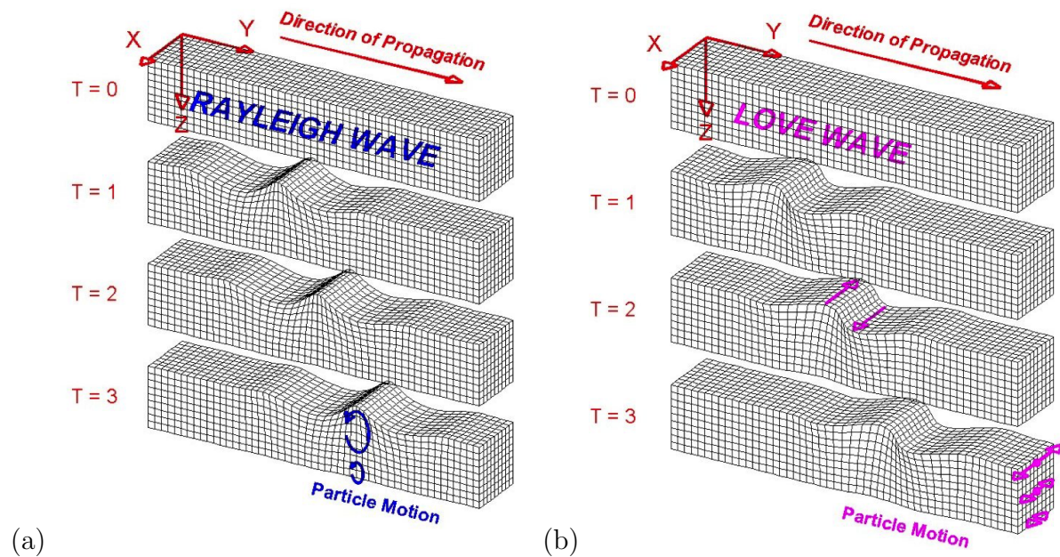
Figure 1.1: Perspective view of surface waves propagating through a grid representing an elastic homogeneous medium. Rayleigh wave propagation generates a retrograde elliptical particle motion (a). Love waves generate a horizontal particle motion, perpendicular to the direction of wave propagation, and are considered as a layer mode (b). The amplitude of the surface waves decreases with depth. Illustration from Braile (2010) .
