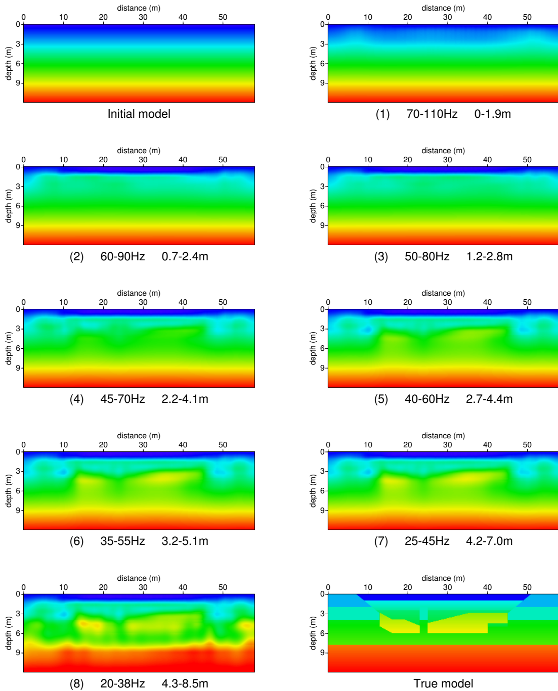
Figure 3.7: Evolution of the resulting shear velocity model at each frequency band step (1) to (8) when using the conventional L2 norm of the difference in the (t, x) domain. For each step a frequency band and depth layer are given as parameters to filter the data and window the model update. This layer stripping strategy progressively updates the model in a top-to-bottom manner, using a high-to-low frequency approach. The initial and true shear velocity models are also shown for reference.
