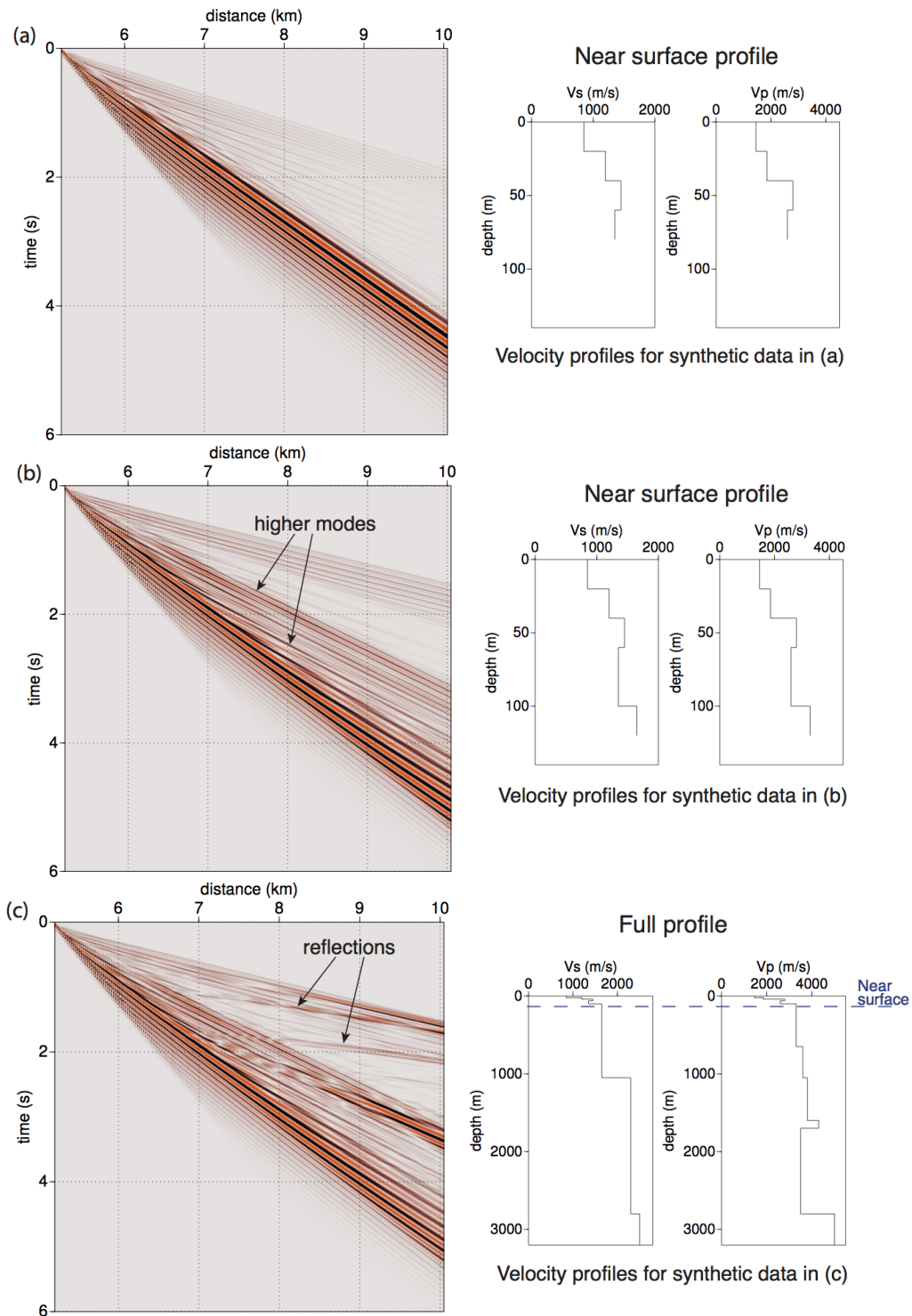
Figure 4.4: Synthetic shot gathers computed with a layered velocity model, considering depths up to 80 m in (a), 120 m in (b) and 3.2 km in (c). The surface wave package does not significantly change when depths below 120 m are considered.
