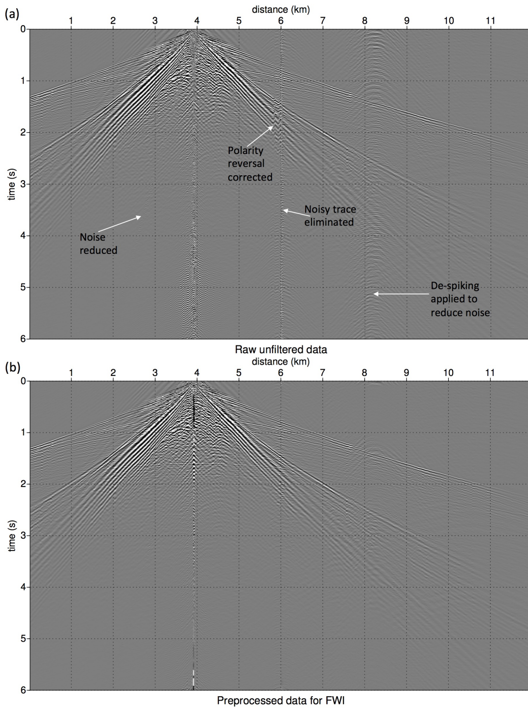
Figure 4.9: An example common shot gather of the raw data (a) and of the pre-processed data (b) after noise removal and regularisation processing steps. Different sources of noise that are corrected for during the pre-processing step are pointed out in (a).
