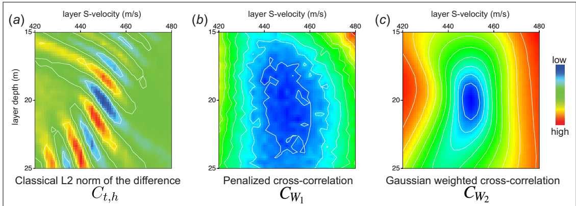
Figure 2.3: Misfit values for the three different misfit functions we have investigated. On the left panel (a), one can see that the classical misfit function has many local minima while the middle panel (b), penalising values far from zero-lag, is more noisy. The right panel (c) presents a nice smooth valley, given by the Gaussian windowing which needs to be carefully designed.
