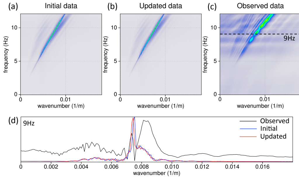
Figure 4.28: The same common shot gather as in Figure 4.27, filtered between 4–15 Hz , is shown in the (\omega, k) domain for the initial data (a), the updated data (b) and the observed data (c). An example trace, located by the black dashed line, shows the effects of cycle-skipping in (d).
