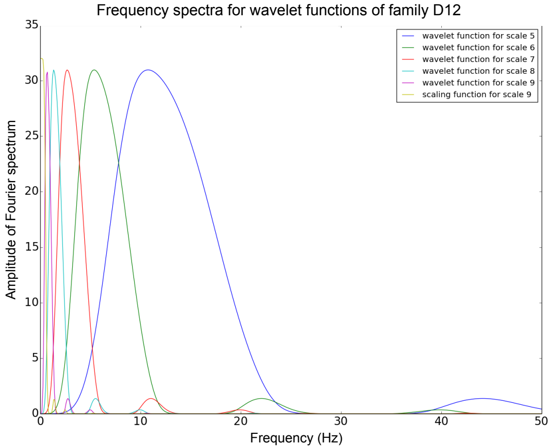
Figure 2.10: Frequency spectra for wavelet functions of family D12 as used by Yuan et al. (2015) . Courtesy of Jean-Baptiste Laffitte, 2015
