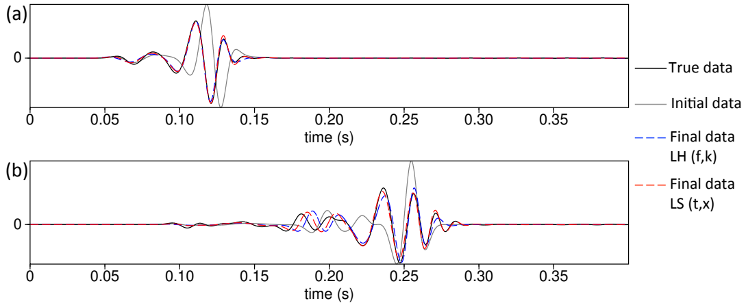
Figure 3.29: Comparison of a single trace at short offset (a) and at far offset (b), located by the red dotted lines on the common shot gather in previous Figure 3.28a. The traces compared are: the true data (black), the initial data (grey), the final data after conventional low-to-high (LH) frequency FWI with an (\omega, k) domain misfit function (blue dashed), and the final data after layer stripping (LS) FWI with a (t, x) domain misfit function (red dashed).
