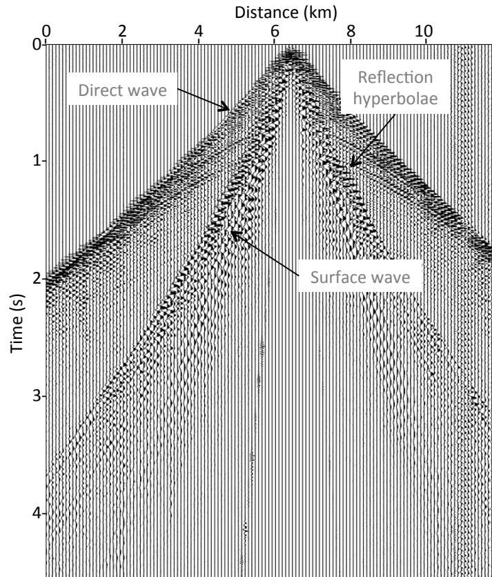
Figure 0.1: Example of a seismic record acquired on land. This common shot gather contains traces from receivers spread out for a few kilometers on either side of the source position. The surface waves travel the slowest through the subsurface and have the largest amplitudes as they are confined near the free surface. They can often mask reflections of lower amplitude, which contain information on properties of the medium at the target depth. Note that an amplitude gain has been applied for better visualization of the data.
