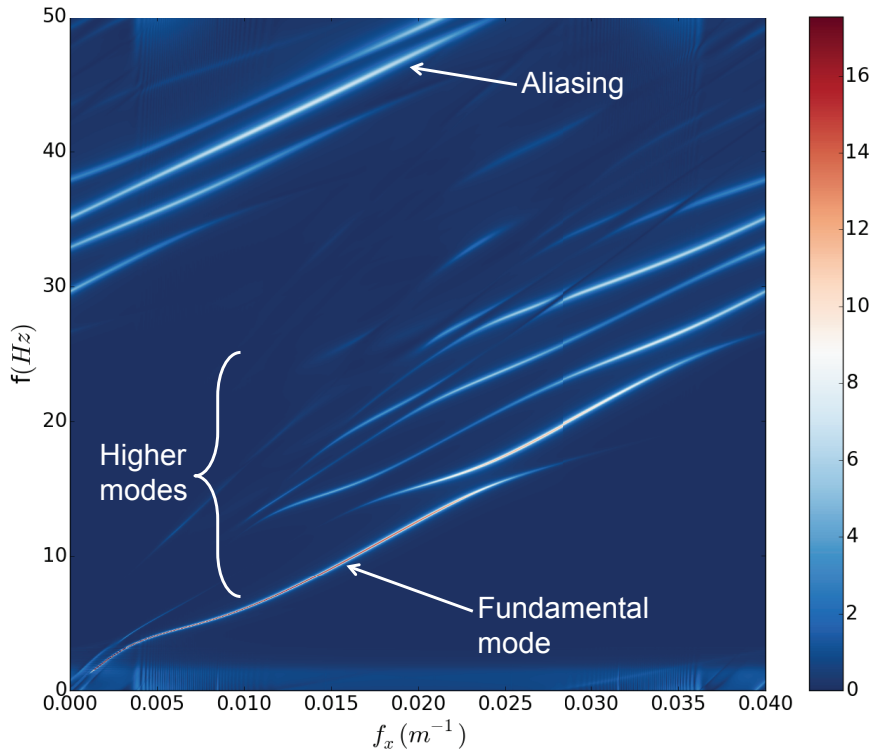
Figure 1.4: Synthetic example of dispersion curves, shown in the frequency-wavenumber (\omega, k) domain, for a simple layered medium. The fundamental mode is the most energetic and can be distinguished relatively clearly. The higher modes appear to merge one with another, although they do not intersect. For noisy datasets or when considering a more complex medium, the higher modes, and sometimes even the fundamental mode, could be easily misinterpreted. Aliasing of the data may further contribute to problems with automated picking algorithms. Courtesy of Jean-Baptiste Laffitte, 2015.
