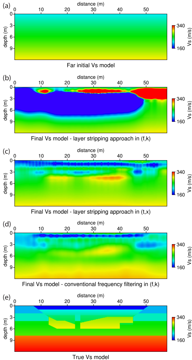
Figure 3.23: Far initial shear velocity model (a); final shear velocity model obtained with layer stripping FWI and the (\omega, k) domain misfit function (b); final shear velocity model obtained with layer stripping FWI and the (t, x) domain misfit function (c); final shear velocity model obtained with conventional low-to-high frequency FWI and the (\omega, k) domain misfit function (d); and true shear velocity model (e).
