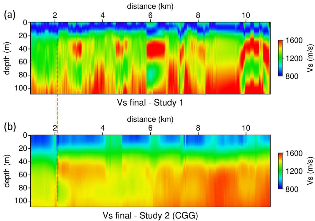
Figure 4.13: Final shear wave velocity models obtained from two separate SWODI studies. Note that only the first 110 m are shown of the velocity model in (a), for a fair comparison to the velocity model in (b) provided by CGG. The topography is also flattened for both models. The red dashed line marks a strong lateral velocity discontinuity.
