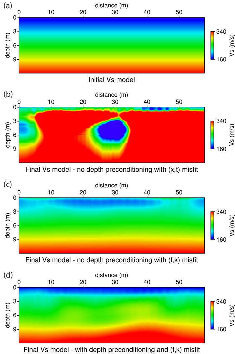
Figure 3.3: Shear velocity model inversion results, using the initial model (a); using the conventional (x, t) misfit (b); using the more robust (\omega, k) domain misfit without a depth preconditioning (c); and using the more robust (\omega, k) domain misfit with a depth preconditioning implemented (d).
