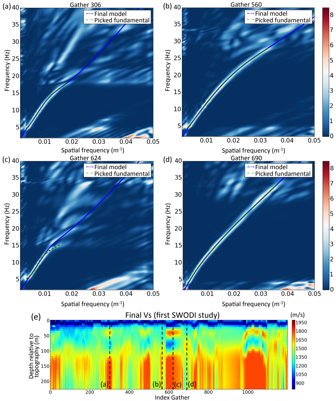
Figure 4.14: Selected CMP gathers in the (\omega, k) domain (a-d), on which the fundamental mode was picked (green dashed line). The fundamental mode of the final SWODI model from the first study, and shown for reference in (e) is also plotted for a quality control (blue solid line). Note that a normalisation is applied on both frequency and spatial frequency axis for better visualisation of the spectrum and all spectra have the same color scale. The final shear wave velocity model is flattened, as required by the FWI algorithm, and velocities above 1800\text{ m/s} where clipped. The location of the CMP gathers is marked by black dashed lines.
