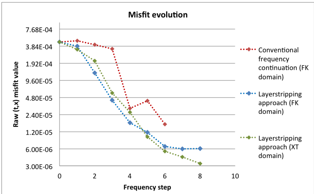
Figure 3.14: The conventional (t, x) domain misfit is used to calculate the difference between the true data, and the data corresponding to the model obtained after each frequency band step, to provide a misfit evolution. The misfit evolution for both the conventional low-to-high frequency strategy and the layer stripping strategy are plotted. This objective comparison shows how the layer stripping approach has a smoother misfit evolution, and gives a greater final reduction of the misfit value. Note that the y-axis is plotted on a log scale.
