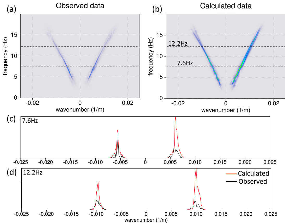
Figure 4.24: A selected common shot gather, muted in the (t, x) domain, filtered between 4 - 15 \text{ Hz} , is shown in the frequency-wavenumber (\omega, k) domain for the observed data (a) and the calculated data (b). A weighting has been applied in the (\omega, k) domain to focus on the fundamental mode. Two example traces, at a frequency of 7.6 \text{ Hz} (c) and 12.2 \text{ Hz} (d) are selected and compared. The peak of the fundamental mode appears to correlate well between observed and calculated data. Note that the amplitudes of the observed and calculated data are at the same scale.
