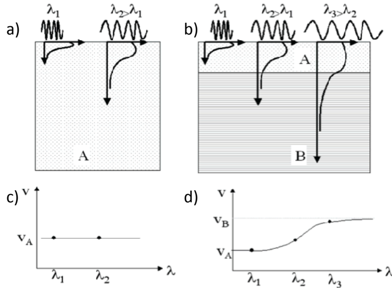
Figure 1.3: Schematic of how the phase velocity is dependent on the wavelength of the propagating wave. For the homogeneous medium depicted in (a) all wavelengths, each associated to one frequency, propagate with velocity A as shown on graph (c). For the layered medium shown in (b), the phase velocity, which now has a more complex frequency relation, is different for each wavelength on the graph (d). Figure taken from Strobbia (2002).
