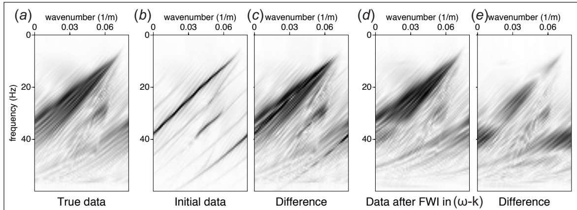
Figure 2.9: The true data in the (\omega, k) domain (a); the initial data and the difference to the true data (b,c); the recovered data and the difference to the true data (d,e). One can see a significantly reduced misfit between the initial data difference and the final data difference with less energetic patterns than for the (\omega, p) domain.
