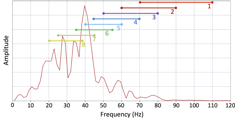
Figure 3.15: Frequency spectrum of the whole true observed data. The energy peaks can be related to the source wavelet with peak frequency of 40 Hz , and also correspond to frequencies which contain information on the main velocity anomalies in the parameter models. The frequency band ranges for layer stripping FWI steps 1-8 (see Figure 3.16) are superimposed on the graph.
