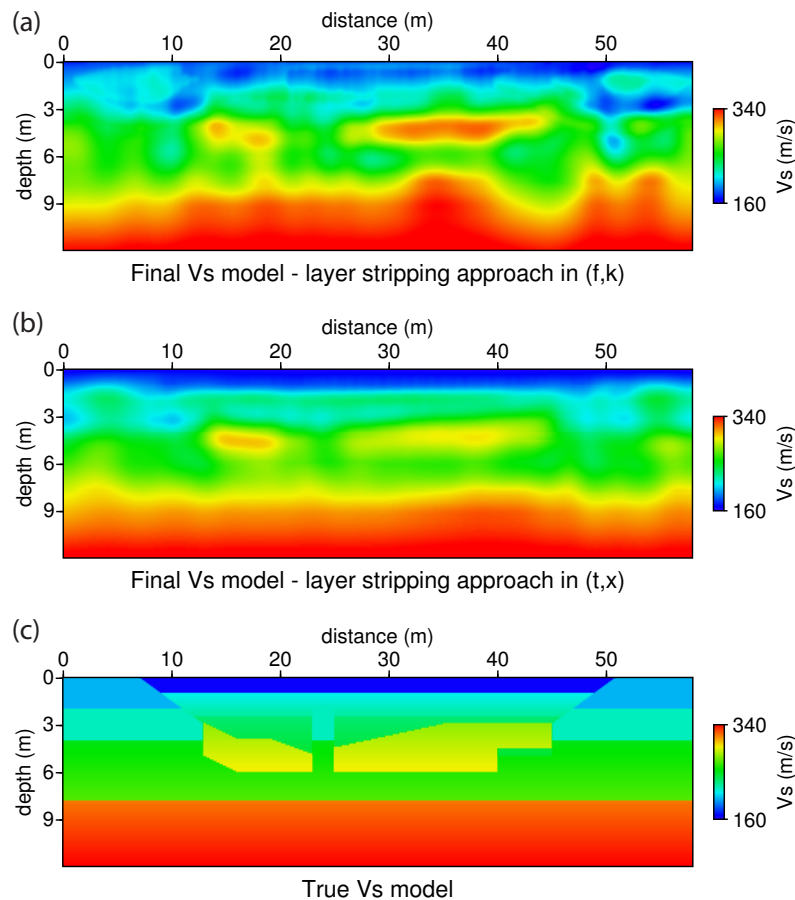
Figure 3.20: Final shear velocity models using the layer stripping approach with a misfit function in the (\omega, k) domain (a) and a misfit function in the (t, x) domain (b). The true shear velocity model is shown for reference (c). Frequency and depth windowing parameters are chosen to linearly increase during each inversion step.
