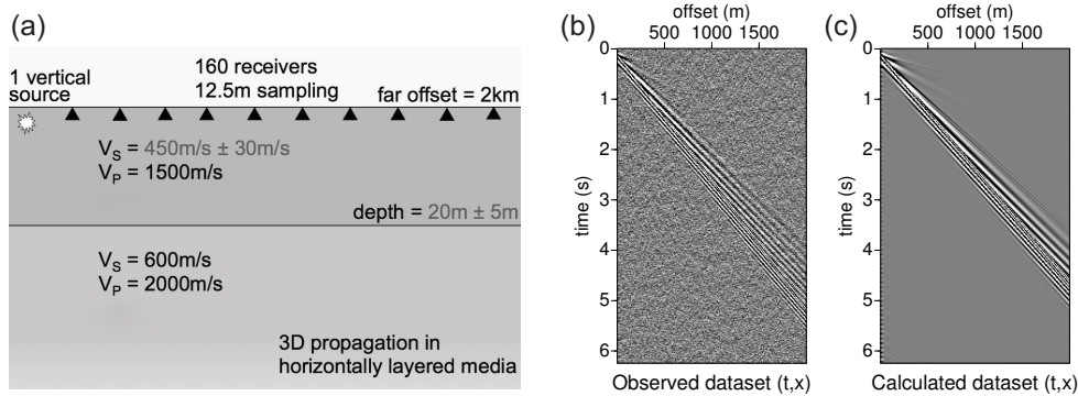
Figure 1 Two-layer model (a) used to create the observed dataset with added random Gaussian noise (b), and an example of the calculated dataset for a layer S-velocity at 480 m/s and depth of 15 m (c).
