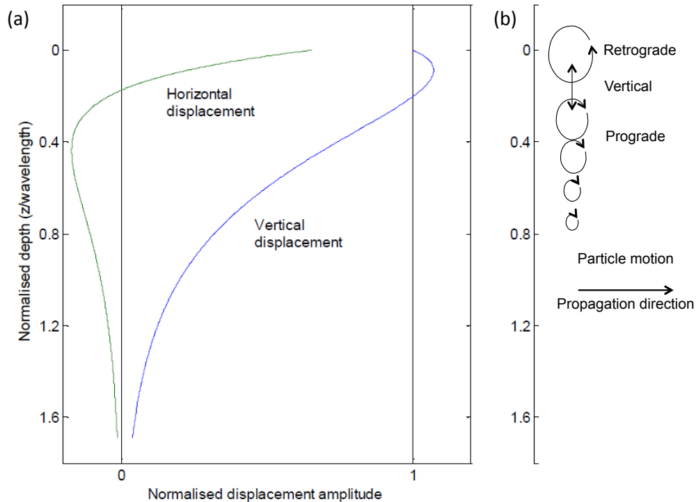
Figure 1.2: The graph in (a) depicts the vertical (blue) and horizontal (green) displacement amplitudes for a Rayleigh wave in an isotropic, homogeneous, elastic half-space, as a function of depth z , given in terms of the wavelength. The amplitudes are normalized against the amplitude of the motion perpendicular to the propagation direction at the surface. Illustrations of the partial motion of a Rayleigh wave corresponding to the respective changes with depth, starting as a retrograde ellipse, to linear vertical motion and finally becoming a prograde ellipse are shown in (b). Figure modified from Gedge and Hill (2012) .
