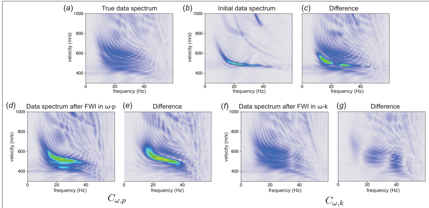
Figure 2.7: Represented in the top row are the true velocity spectrum (a), the initial spectrum for the simple two-layer model (b) and the velocity spectrum differences (c). The bottom row represents the final velocity spectrum for the FWI result in the \omega - p domain (d), and the difference with the true velocity spectrum (e); and the final velocity spectrum for the FWI result in the \omega - k domain (f), and the difference (g). In this example, the FWI performs better in the \omega - k domain than in the \omega - p domain.
