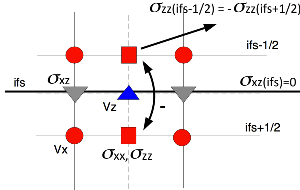
Figure 1.8: Implementation of the free surface boundary condition for the finite difference Virieux-Levander staggered grid stencil, using image theory. The free surface is along the \sigma_{xz} = 0 grid. Modified from (Operto et al., 2007).
