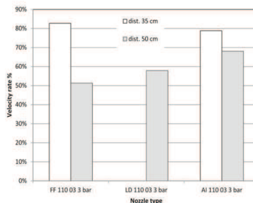
Fig. 8. Velocity rate of various nozzles – effect of nozzle type and measurement distance. FF: Flat Fan; LD: Pre orifice; AI: Air Injection nozzle. 100% corresponds to theoretical initial velocity with data from Nuyttens et al. (2007a,b, 2009) and Miller et al. (2008).
