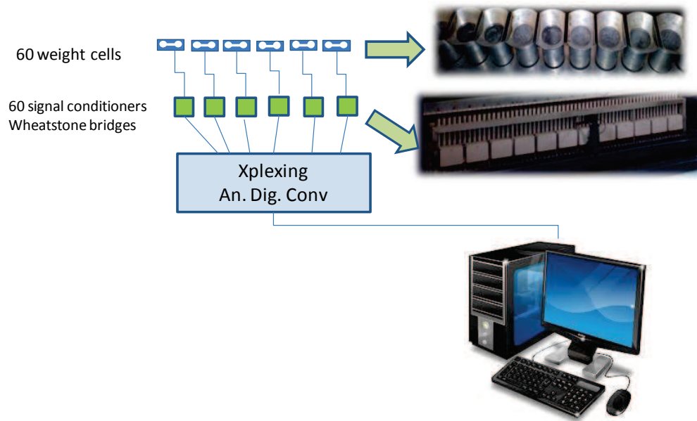
Figure 25: Weight cells
