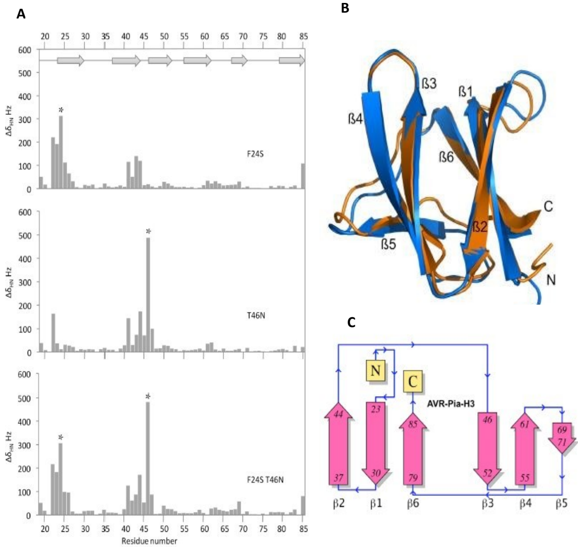
Figure 1. The AVR-Pia-H3 NMR structure is similar to the structure of wild-type AVR-Pi
