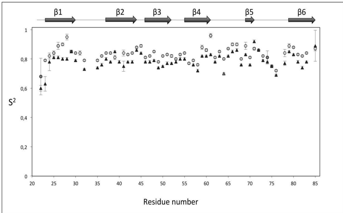
Supplemental Figure 1. Comparison of NMR relaxation of AVR-Pia and AVR-Pia-H3.
