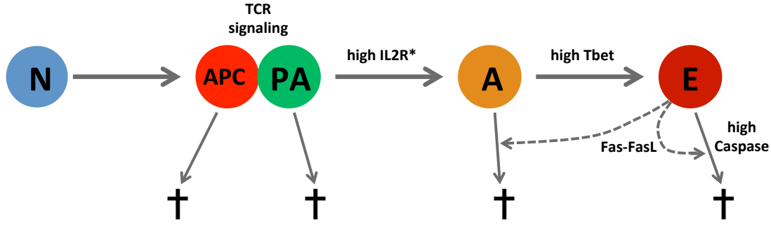
Figure 2.3 – Schematic diagram of the linear activation pathway for the CD8 T-cells. Due to TCR signaling (as shown in Figure 2.2), once a naïve T-cell comes into contact with an APC it becomes preactivated, then evolves to an activated cell when its IL2R* dynamically crosses a threshold and, eventually, to an effector stage when Tbet dynamically crosses a threshold. The caspase activation level is essential for cell apoptosis. Fas-FasL signaling further enhances apoptosis of activated and effector stages if activated-effector or effector-effector cells come into contact (cytotoxic effect). In contrast, the death of APC is independent of caspase levels, because the molecular network does not apply for APC. Key: N, naïve; PA, preactivated; A, activated; E, effector; APC, antigen presenting cell.
