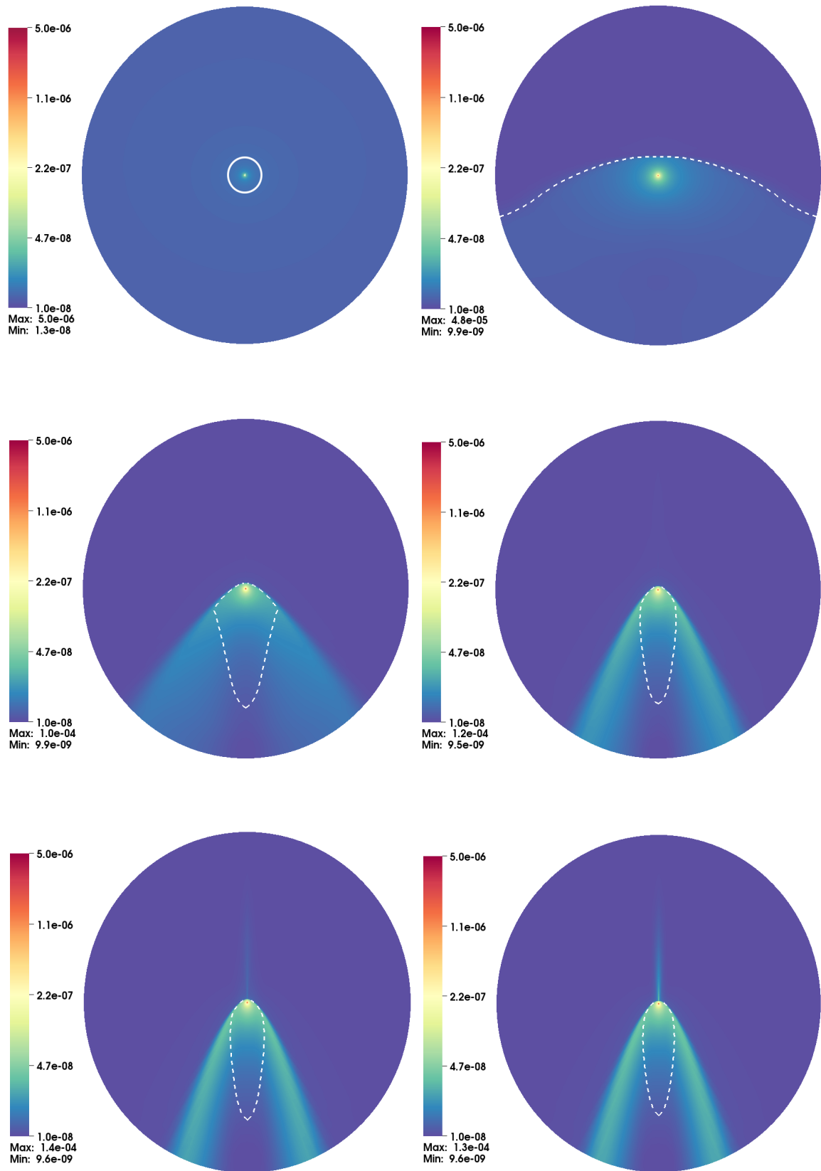
Figure 5.9: Logarithmic color maps (arbitrary units) of the stationary density profiles for r_{\text{in}} = 10^{-3} \zeta_{\text{HL}} and, in reading order, \mathcal{M}_{\infty} = 0.5, 1.1, 2, 4, 8 and 16 . The outer Mach 1 surface has been plotted (not the sonic one) as a white dashed line. On the first plot, subsonic, the solid white line stands for the approximate size of the critical impact parameter, \zeta_{\text{HL}} ( \zeta_{\text{HL}} \sim 0.15 r_{\text{out}} ).
