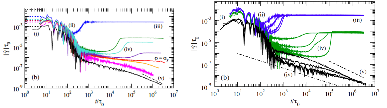
Figure 6.1: Strain rate versus time for different applied stresses across the yield stress in a colloidal glass. Left: Creep for different imposed stresses. Right: the three colors correspond to three different imposed stresses. From the left to the right of the four curves for each imposed the stress, the waiting times are t_w = 60, 600, 3600, 6000s , i.e. the age of the sample is increasing [Siebenbürger et al., 2012].
