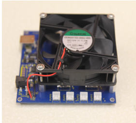
Figure 4.38: PumpSpark Control Board – © Microsoft
