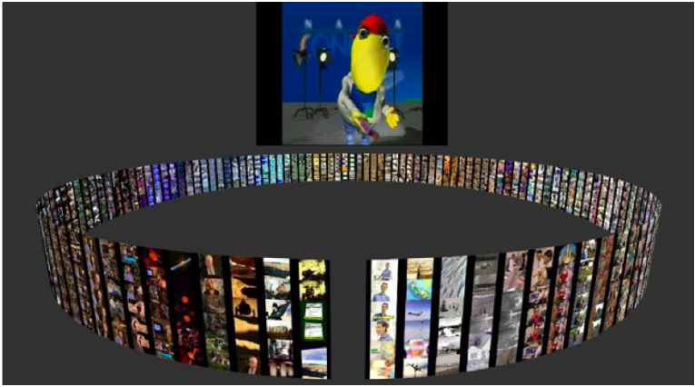
Figure 2.43: Screenshot
