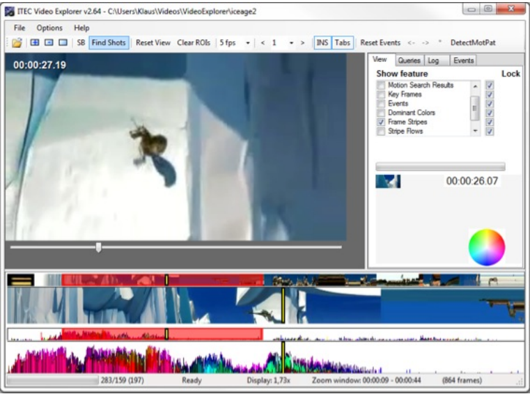
Figure 2.37: Screenshot
