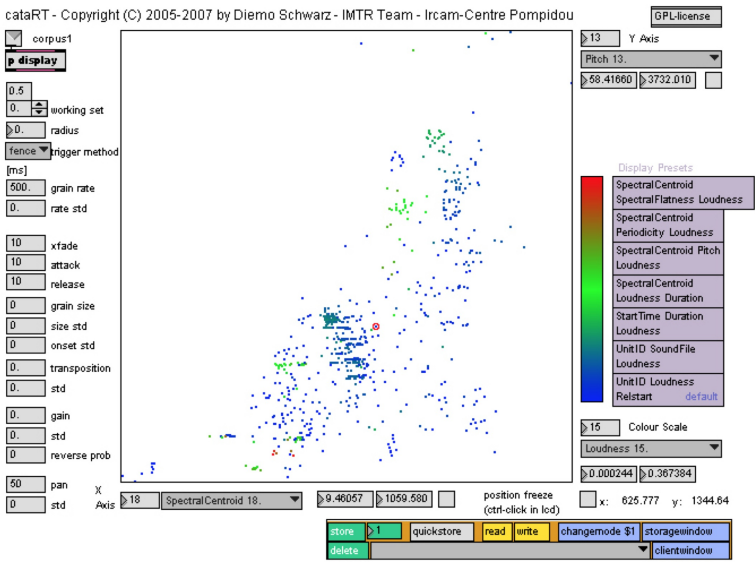
Figure 2.21: Screenshot
