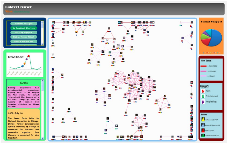
Figure 2.40: Screenshot
