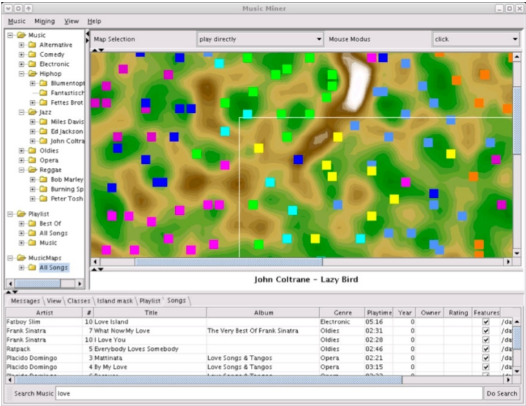
Figure 2.23: Screenshot
