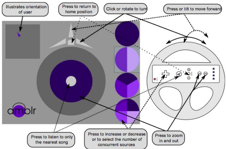
Figure 2.10: Screenshot
