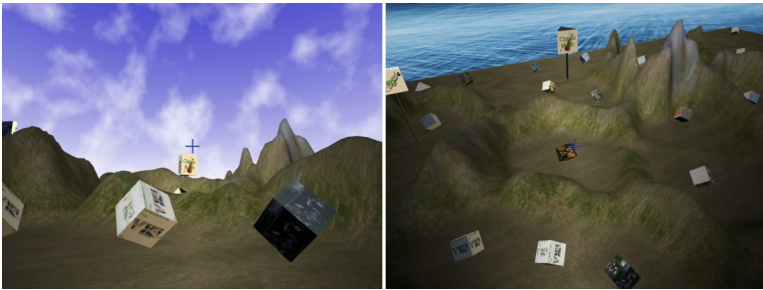
Figure 2.28: Screenshots
