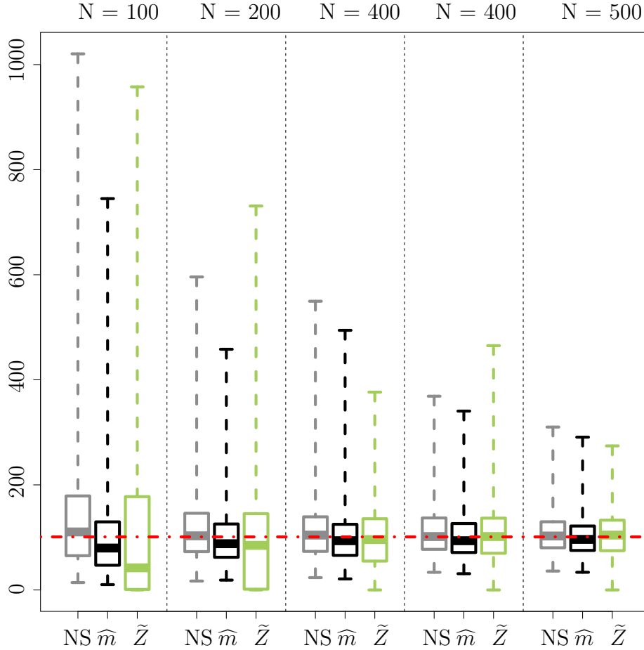
Figure 4.4: Boxplots of ideal infinite nested sampling \widehat{m} of Eq. (4.4) and (NS) of Eq. (4.5) and randomly truncated \widetilde{Z} (Corollary 4.2) for the estimation of E[g(\mathbf{X})] with g as in Eq. (4.30) and \mathbf{X} \sim \mathcal{U}\left(-\left[\frac{1}{2}, \frac{1}{2}\right]^d\right) , d = 20 . (NS) Ideal nested sampling is got with N_{\text{iter}} = 100N as this is known to be enough in this case. (NS) and \widehat{m} are obtained from the same runs. The (red) dot-dashed line is the theoretical value of m .
