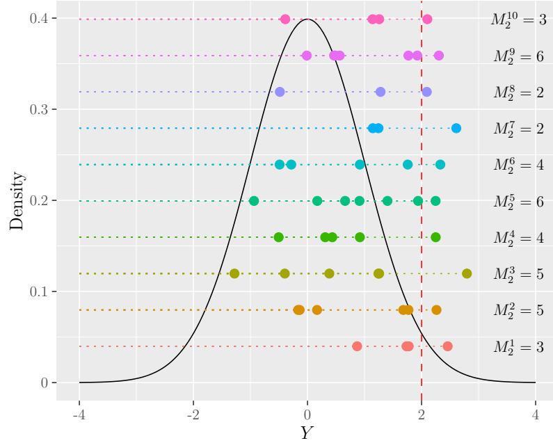
Figure 3.3: N = 10 simulations of a random walk associated with a standard normal Gaussian random variable. The statistic \bar{M}_2 = 40 and so the estimated probability is \hat{p}_2 = (1 - 1/10)^{40} \approx 1.48 \times 10^{-2} with \text{CV}[\hat{p}_y] \approx 0.43 . Animated figure online.
