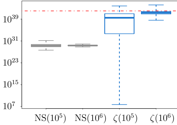
Figure 4.6: Estimation of m = \mathbb{E}[g_{\text{ht}}(\mathbf{X})] with \mathbf{X} \sim \mathcal{U}\left(-[\frac{1}{2}, \frac{1}{2}]^d\right) , d = 20 . (NS): nested sampling stopped after 100N iterations; \zeta : estimator of Section 4.3.4 with \beta_{\text{app}} (Eq. 4.18) and N = 20 . 10^5 and 10^6 are the computational budgets used. The (red) dot-dashed line is the theoretical value of m .
