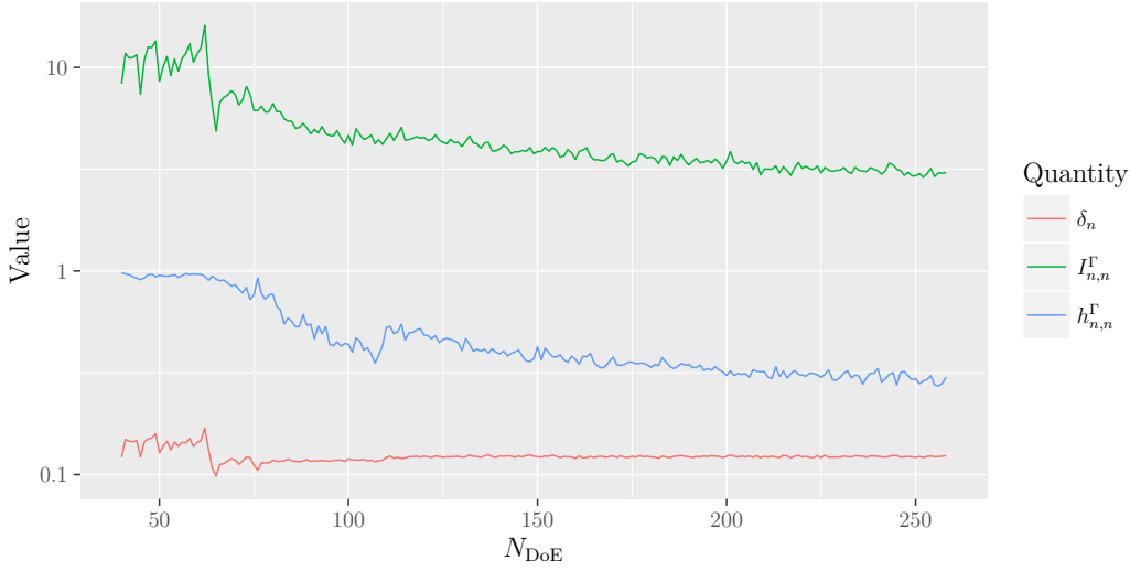
Figure 5.7: Evolution of the SUR criteria I_{n,n}^\Gamma and h_{n,n}^\Gamma = J_{n,n}^\Gamma / \alpha_n against the number of points added to the Design of Experiments by minimising at each iteration I_{n,n+1}^\Gamma . \delta_n is the estimated coefficient of variation such that \delta_n^2 = -\log \widehat{\alpha}_n / N_{\text{SUR}} . The first 40 samples of the DoE are drawn in a uniform hypersphere of radius 6.5. N_{\text{SUR}} = 800 and N_{\text{SUR, PPP}} = 100 .
