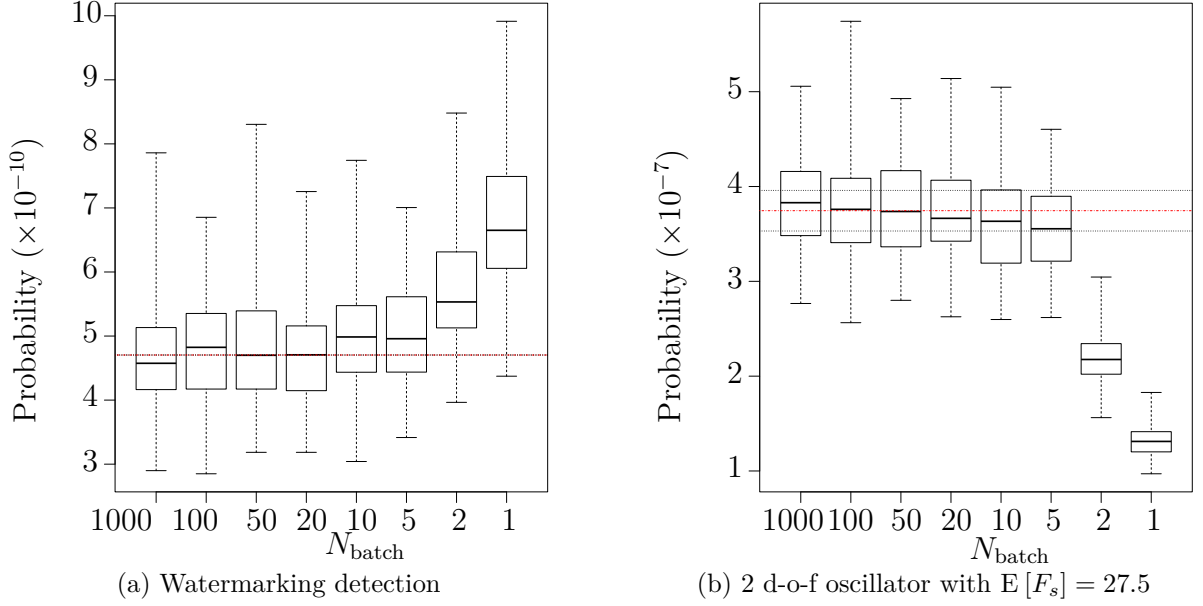
Figure A.2: Boxplots of the probability estimator given by Algorithm 20 with a total of N = 1000 random walks generated by batches of size N_{\text{batch}} . Results over 100 simulations, whiskers extending to the extreme values. The dashed lines stand for the references values.
