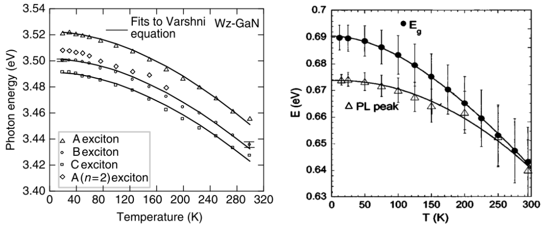
Figure 1.11: Energy bandgap dependence of temperature for Wurtzite GaN (left) and for InN (right).
