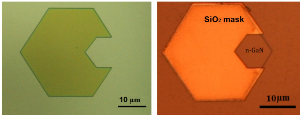
Figure 3.98: Image issued from optical microscopy demonstrating SiO 2 cover-plate before second etch (left) and after (right).
