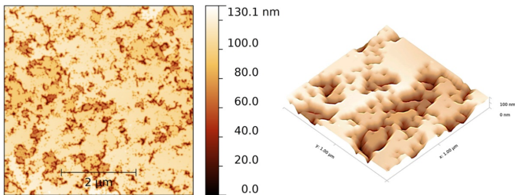
Figure 2.53: AFM analysis of 5 \times 5 \mu\text{m}^2 for sample MQ30 (left) and 3D surface morphology (right).
