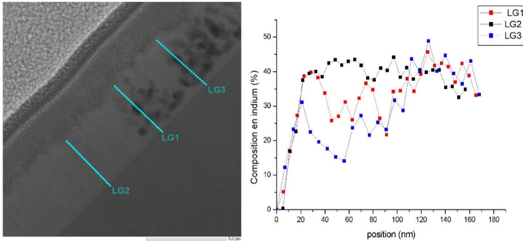
Figure 2.57: EDX analysis for indium content for sample SL50.
