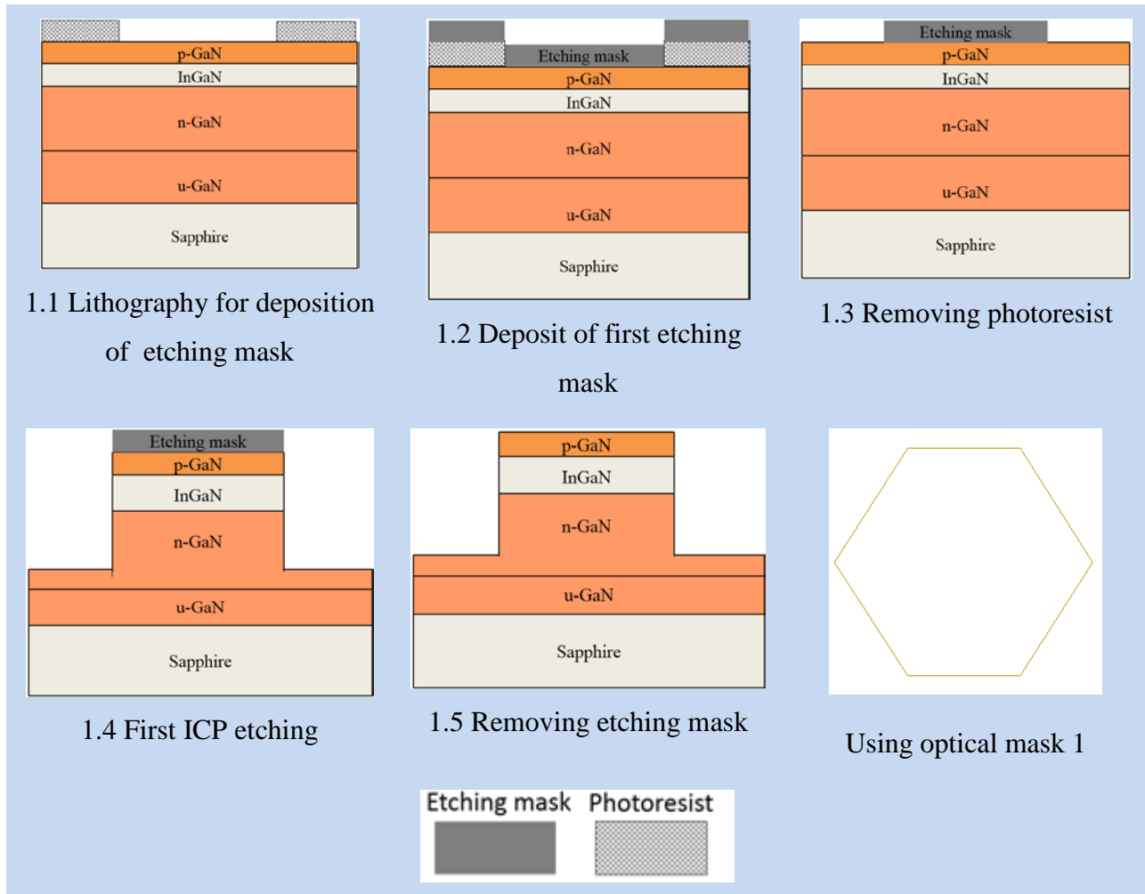
Figure 3.96: Flowchart of phase-1 for mesa etching process.
