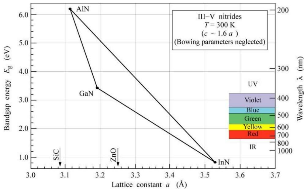
Figure 1.1: Bandgap energy vs. lattice constant a for III-nitrides at 300 K
