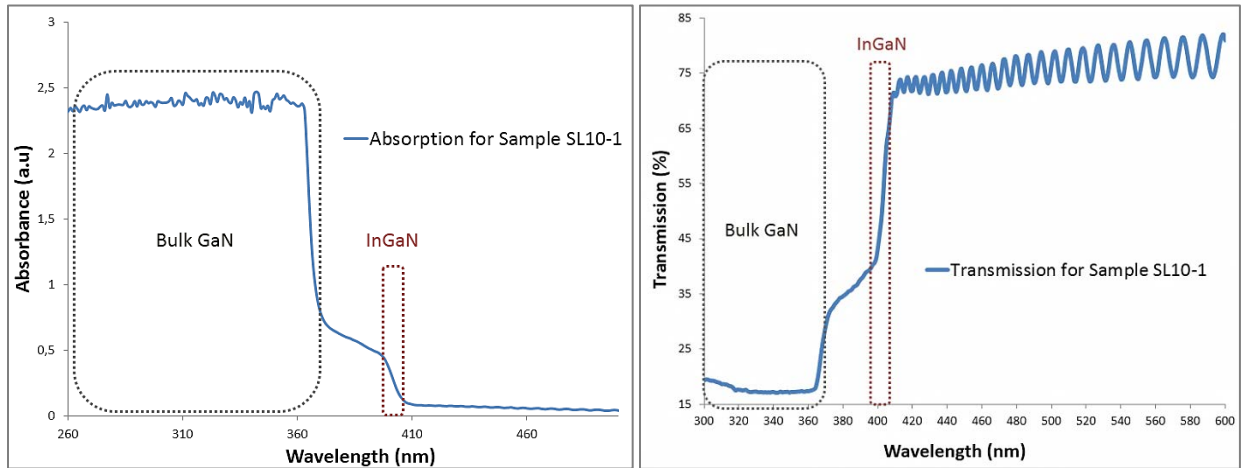
Figure 2.40: Absorption spectrum (left) and Transmission spectrum (right) for the sample SL10-1 at room temperature.
