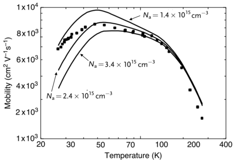
Figure 1.14: Experimental and calculated electron mobilities using iterative BTE method as a function of temperature for different acceptor concentrations.
