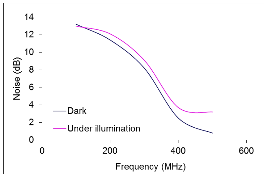
Figure 3.113: Noise measurement for 100 \times 100 \mu\text{m}^2 photodiode using Noise-Figure-Meter.
