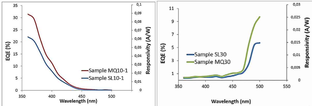
Figure 3.87: Responsivity and EQE of samples SL10-1 and MQ10-1 (left), samples SL30 and MQ30 (right).
