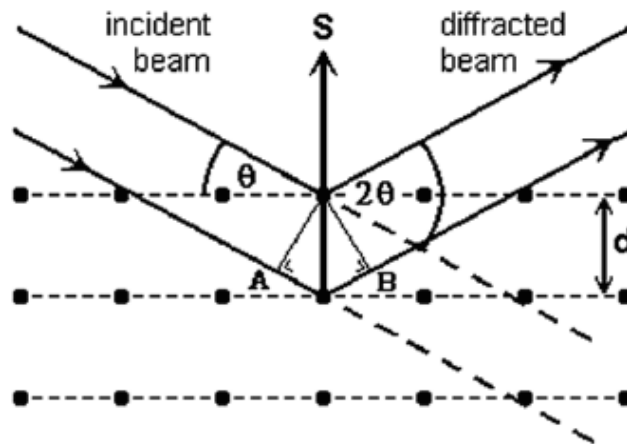
Figure 2.22: Schematic of XRD.
