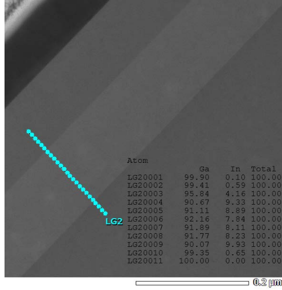
Figure 2.31: EDX for Ga and In composition via TEM cross section image along [1112] zone axis for sample SL10-1 grown by MOCVD.
