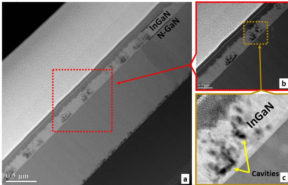
Figure 2.56: TEM cross section image of general view along [11\bar{2}0] for sample SL50 grown by MOCVD (a), zoomed area (b) and (c).
