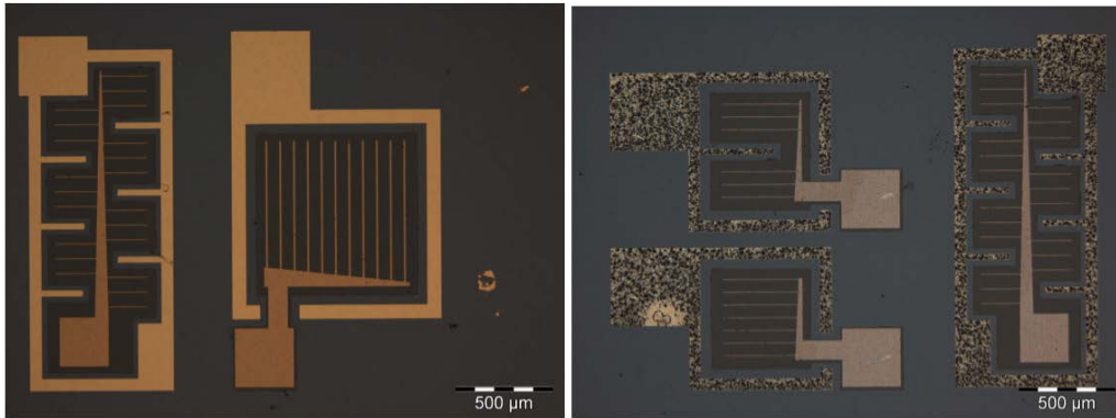
Figure 3.78: Images issued from optical microscopy for fabricated photodiodes in photovoltaic design before (left) and after annealing (right).
