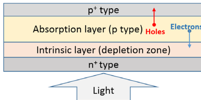
Figure 3.117: UTC-photodiode structure.
