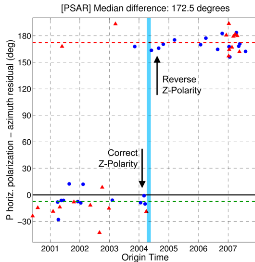
Figure 2.15: Validation of a flip in the polarity of the vertical component of the surface station PSAR between April and May 2004 (later confirmed to have occurred between 16 and 17 April), using the CRL 2000-2007 dataset (Chapter 6). Compressive and dilatational first motion polarities are denoted by blue circles and red triangles, respectively.
