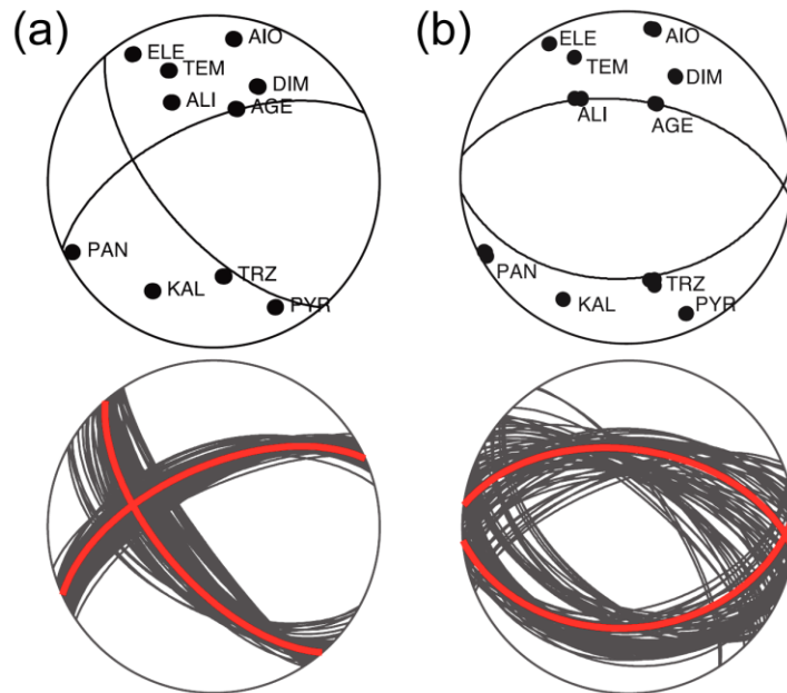
Figure 6.45: Comparison of a composite focal mechanism (multiplet #04432) from Godano et al. (2014), a) using the 1D velocity model of Rigo et al. (1996), b) using the 3D velocity model of Gautier et al. (2006). Upper beachballs show the distribution of stations and the respective first motion polarities (all compressive). Lower beachballs show the optimal fault plane solution (red) with its uncertainty domain within the respective confidence interval (dark nodal planes). Figure modified after Godano et al. (2014). The focal mechanism is in the same region and similar to Fig. 6B.23.
