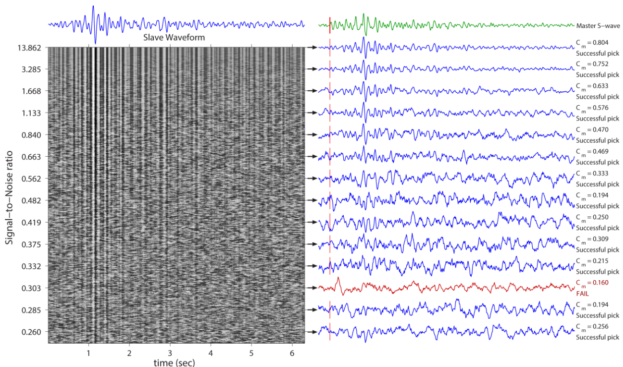
Figure 4.15: Same as Fig. 4.14, but using low-frequency (smoothed) rather than high-frequency Gaussian noise. Figure after Kapetanidis & Papadimitriou (2011).
