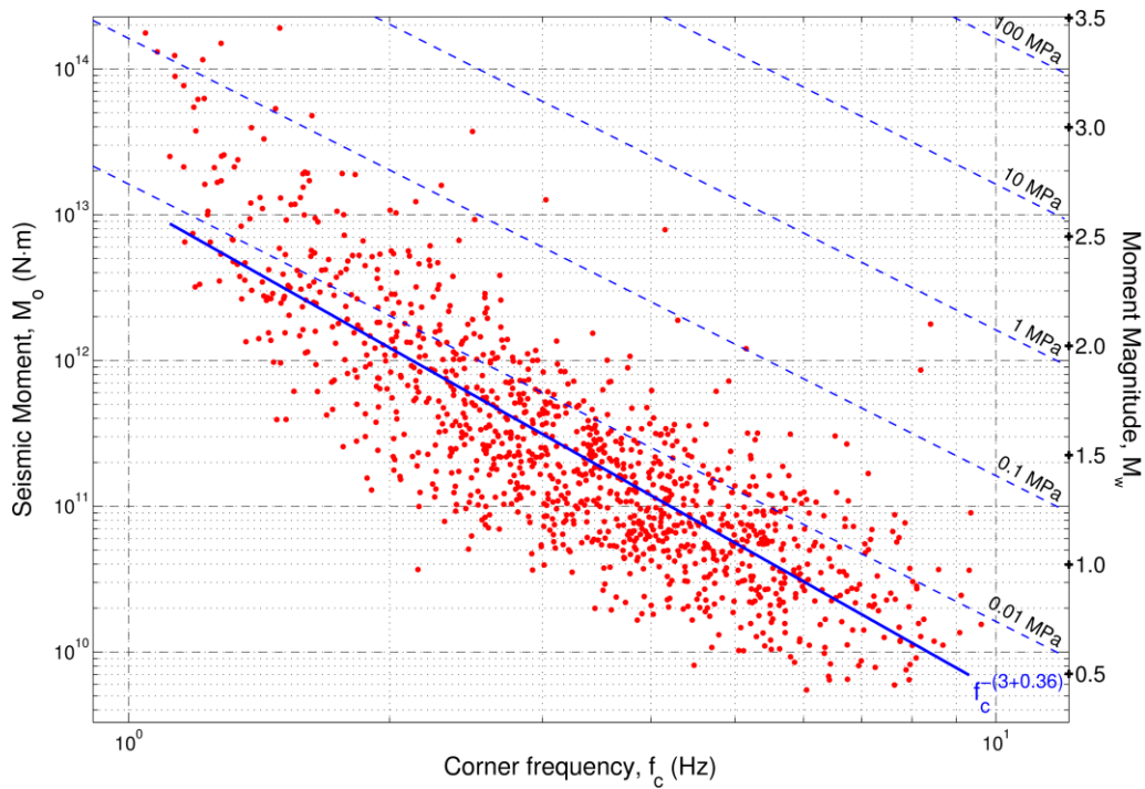
Figure 3.12: Relation between M_o and f_c for measurements of the 2013 Helike swarm on station TEME, using model #3 (Brune, 1970). A series of f_c^{-3} lines for typical values of constant stress drop, \Delta\sigma , are also displayed for reference.
