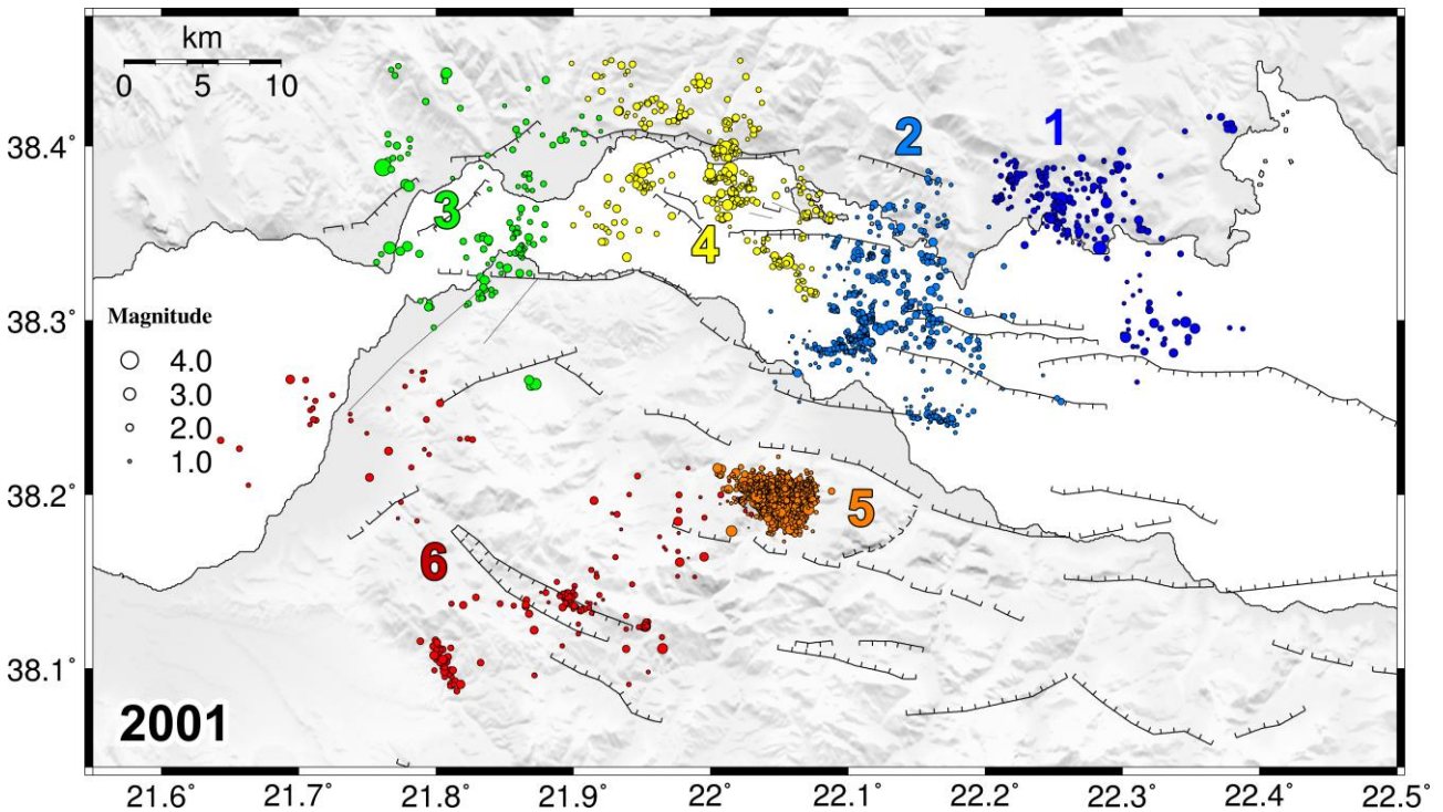
Figure 6.3: Same as Fig. 6.2, but for the seismicity of year 2001. Details on the 6 spatial groups are presented in Tables 6.3 and 6B.2.
