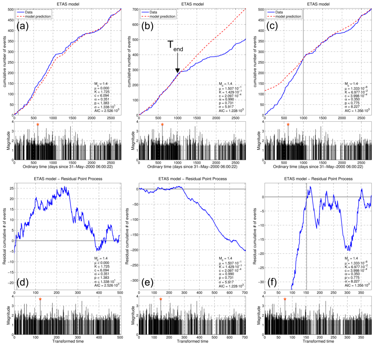
Figure 6.44: ETAS model for Group #9 (Eratini) in the western Corinth Rift, (a, b, c) in ordinary time and (d, e, f) residual between data and model in transformed time, with M_{\text{th}}=M_c=1.4 , M_r=3.7 parameters determined by MLE (a, d) for the whole period 2000-2007 with forced \mu=0 , excluding the first 100 days (vertical gray line), (b, e) only for the first 1000 days (up to T_{\text{end}} marked with an arrow), and (c, f) excluding the first 100 days (vertical gray line).
