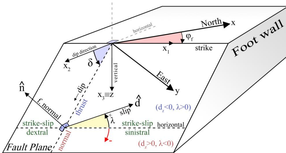
Figure 2.6: Fault geometry and associated vectors. Two types of coordinate systems are displayed, one (\mathbf{x}_1, \mathbf{x}_2, \mathbf{x}_3) aligned to the fault’s strike ( \mathbf{x}_1 ) and dip direction ( \mathbf{x}_2 ) and Aki & Richards (2002) geographical coordinate system (\mathbf{x}, \mathbf{y}, \mathbf{z} \equiv \mathbf{x}_3) , with positive orientations: \mathbf{x} \rightarrow North, \mathbf{y} \rightarrow East and \mathbf{z} \rightarrow downwards. The fault’s normal unit vector, \hat{\mathbf{n}} , and the slip unit vector, \hat{\mathbf{d}} are also displayed. (Figure based on Stein & Wysession, 2003, but using a different coordinate system)
