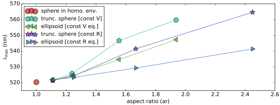
Figure 1.27: Comparison of the LSPR wavelengths of the truncated spheres and ellipsoids (figure 1.26) in a homogeneous environment of n = 1 as a function of their aspect ratio ar . [FEM calculations]
