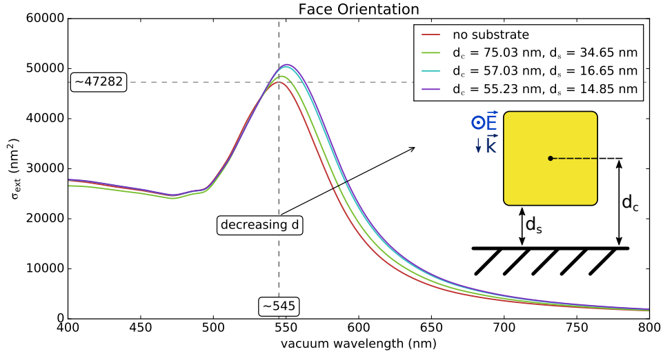
Figure F.2: Extinction cross-section of a rounded gold cube ( l = 80.76 nm, r = 5 nm) in air ( n = 1 ) on its face at varying distance from a glass substrate ( n = 1.5 ). Barycenter-to-surface distances are comparable to the edge-oriented cube shown in figure 1.35b on page 73. [FEM calculations]
