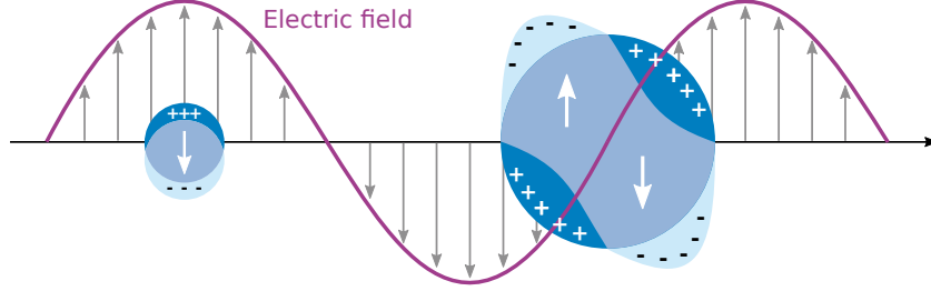
Figure 1.9: Schematic overview of dipolar and quadripolar modes of a nanoparticle under incident radiation. When the dimension of the object is of the same order or greater than the wavelength, the quasi-static approximation is no longer valid and higher-order modes are excited, such as the quadripolar mode represented on the right. Note that the figure is only schematic and not an accurate representation of electron distribution.
