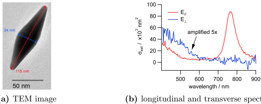
Figure 3.2: TEM image and spectra of a unique BP. The characteristic strong and narrow LSPR peak arises from an oscillation along the longitudinal axis of the object. Source: Navarro et al. [32]
