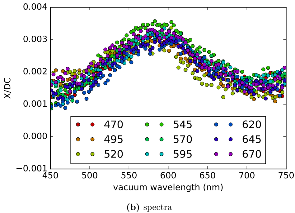
Figure D.1: Using MICA, a gold sphere of 120 nm on a glass substrate in air was tracked using local maps at wavelengths ranging from 470 nm to 670 nm with a step size of 25 nm. Each map was automatically analyzed to determine the optimal point to acquire a spectrum and the spectrum was then measured. The resulting spectra were independent of the mapping wavelength. The maps are shown with the same z-scale for comparison. The region is approximately 3 \mu\text{m} \times 4 \mu\text{m} .
