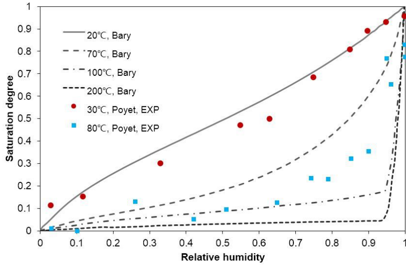
Figure 1.4: The converted results according to (Poyet, 2009) and the calculated results from (Bary et al. , 2012)
