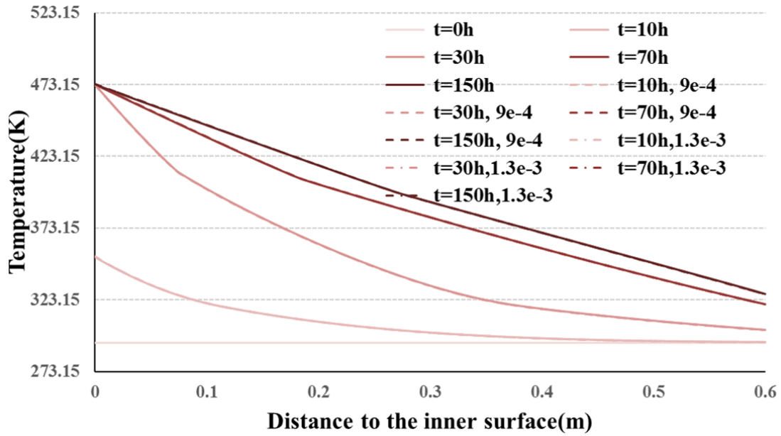
Figure 3.6: Evolution of temperature distribution with different coefficient
