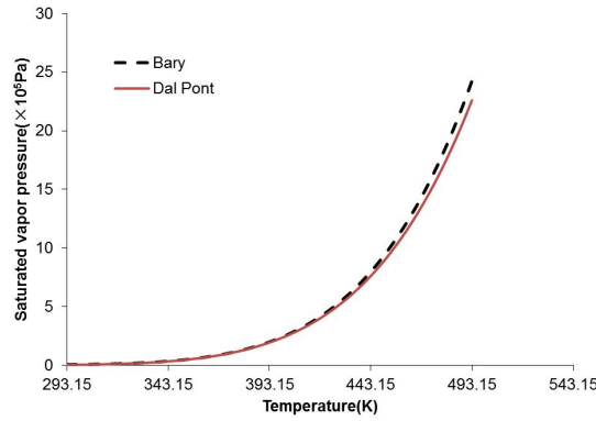
Figure 1.13: Saturated vapor pressure of water from Bary(Bary et al. , 2012) and Dal Pont(Dal Pont and Ehrlicher, 2004)
