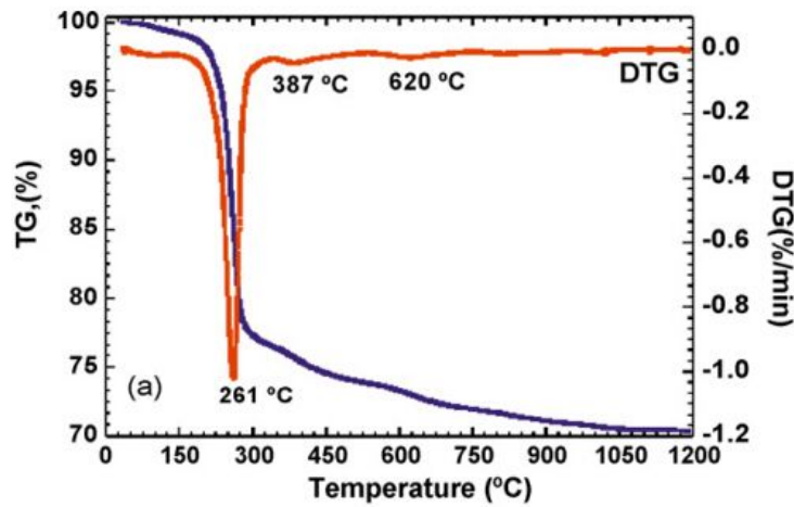
Figure 1.4: TG/DTG experiment by Mercury(Rivas-Mercury et al. , 2008)
