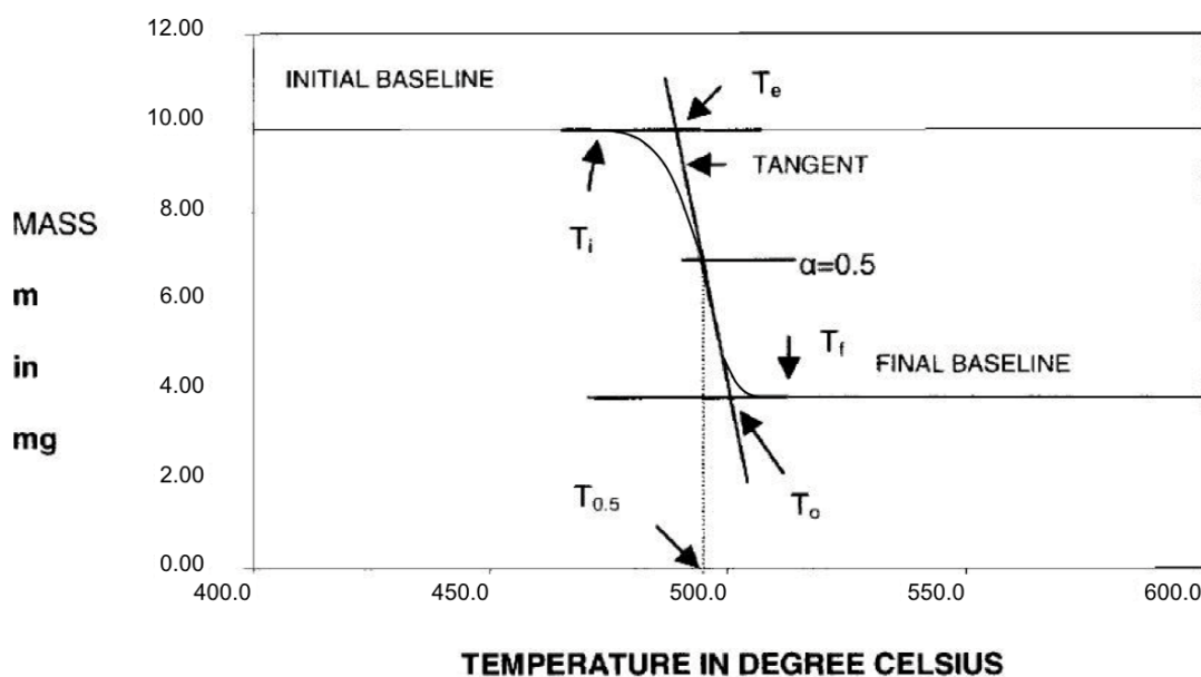
Figure 1.9: Definition of the decomposition temperature on a TG curve(Haines, 2002)
