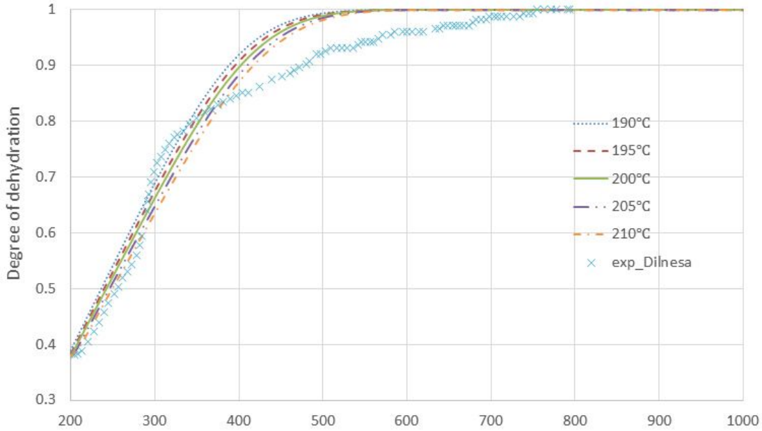
Figure 2.19: Influence of main layer dehydration onset temperature
