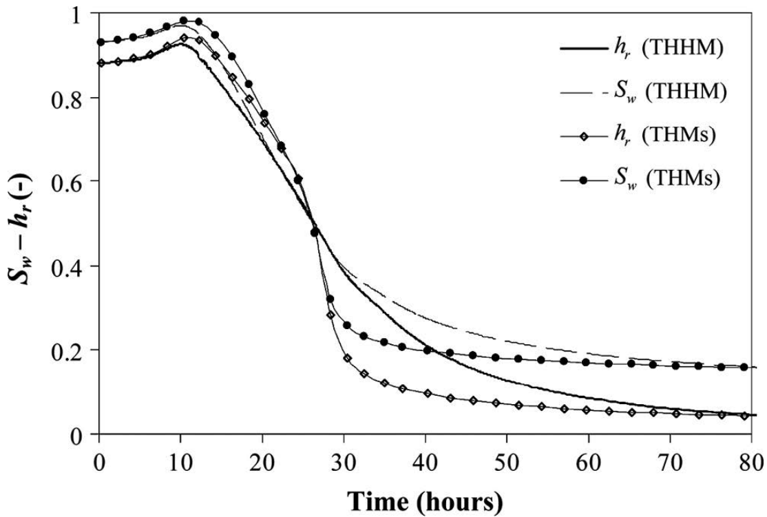
Figure 1.19: Evolution of S_l and relative humidity in the center of the specimen (De Moraes et al. , 2009)
