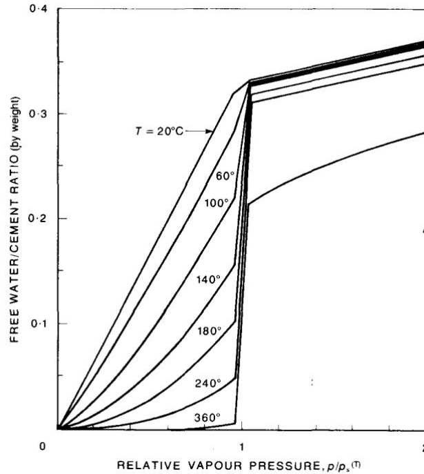
Figure 1.1: Calculated relation between free water/cement ratio and vapor pressure at various temperatures(Bazant and Thonguthai, 1979)
