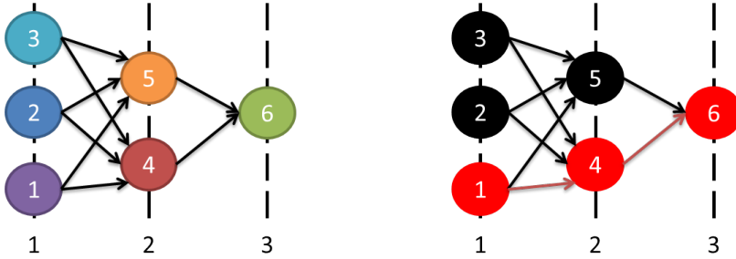
Figure 2.28: Generated graph and selected connected components from the example of Figure 2.27.
