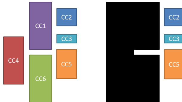
Figure 2.27: Schematic example of a selected left vertical border; the left side of this figure shows the connected components of this border, the right side shows the mask.
