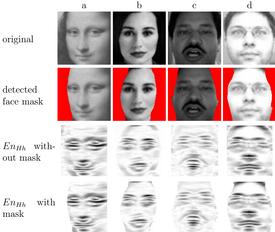
Figure 2.31: From top to bottom: original face window, detected face mask, normalized horizontal energy map of the original image, normalized horizontal energy map after applying the face mask.
