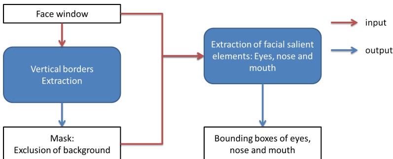
Figure 2.17: Global view of face salient anatomic element extraction.
