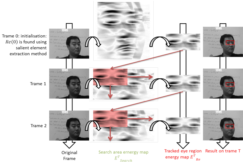
Figure 4.1: Scheme of the tracking process based on similarity of energy maps.
