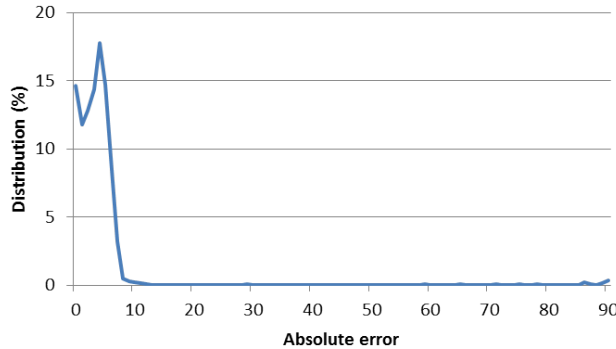
Figure 3.16: Distribution of face images (%) according to the absolute error in Color Feret database.
