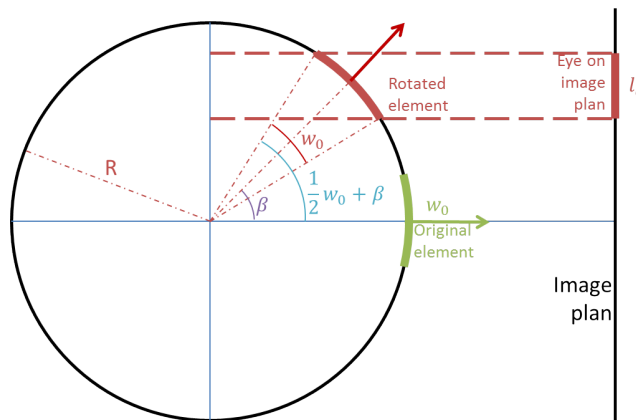
Figure 3.9: Schematic view of eye image plan projection.
