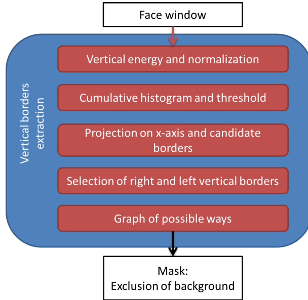
Figure 2.18: Scheme of vertical face borders extraction, the result is a mask which separates the face from the background.
