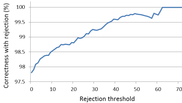
Figure 3.15: Correctness (%) according to the rejection threshold T .
