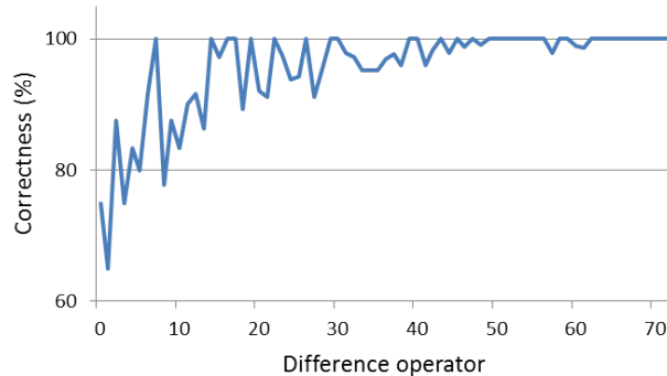
Figure 3.14: Correctness (%) according to \Delta .
