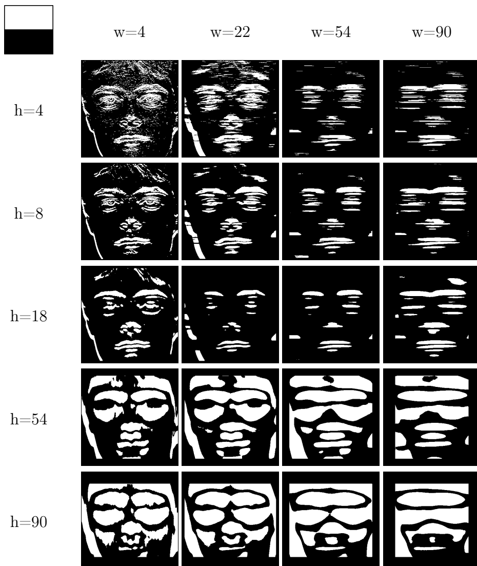
Figure 2.11: Binarized horizontal energy maps. Thresholds are chosen manually with a visually suitable value to illustrate.
