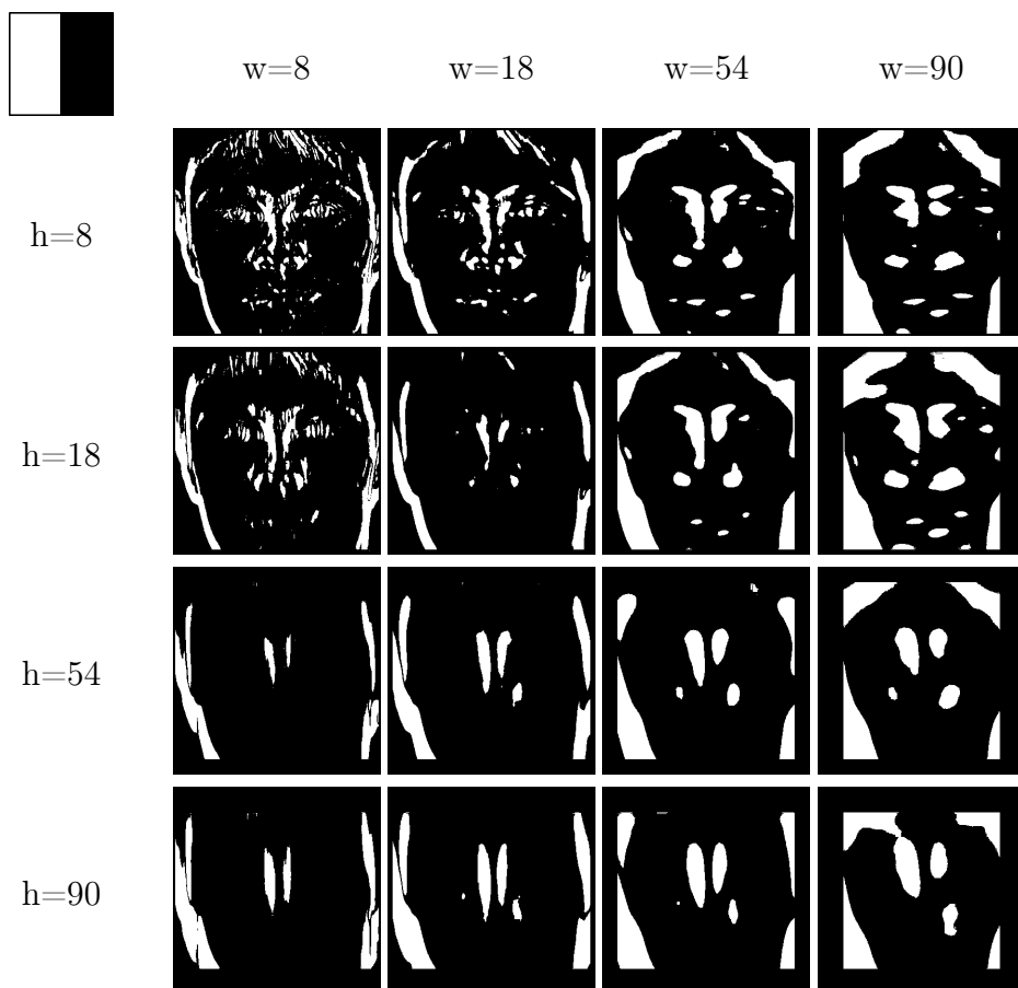
Figure 2.13: Binarized vertical energy maps. Thresholds are chosen manually with a visually suitable value to illustrate.
