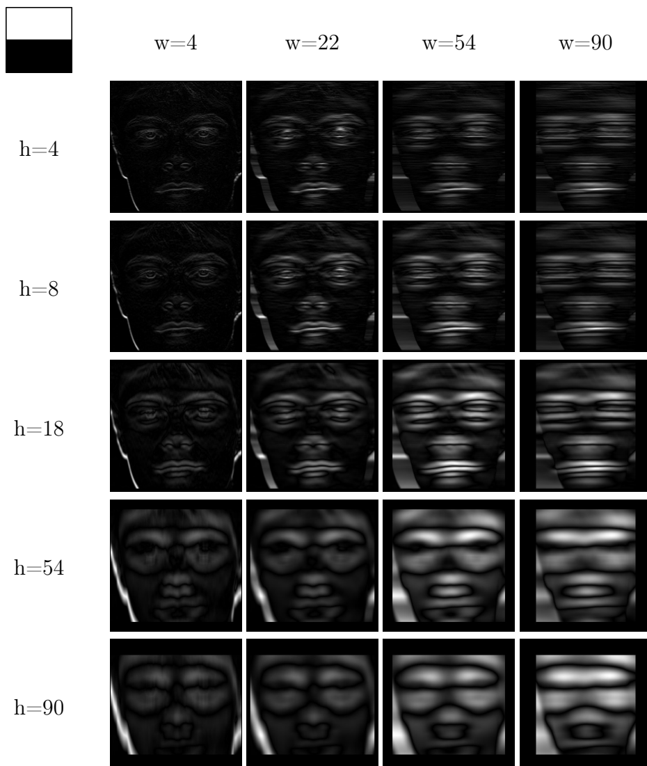
Figure 2.10: Energies of horizontal Haar filter according to the filter width w and height h in pixels. The face window width and height equal both to 364 pixels
