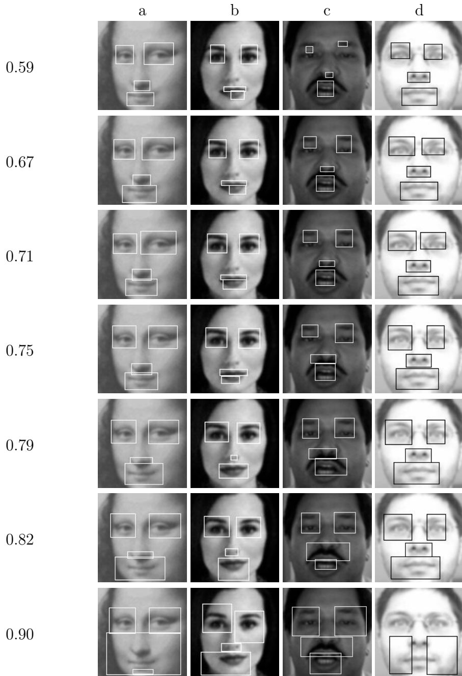
Figure 2.42: Candidate anatomic regions extraction according to threshold t applied on normalized horizontal energy map.
