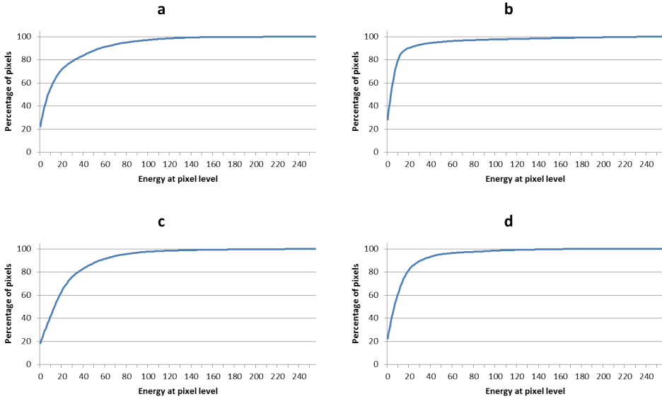
Figure 2.22: Cumulative histograms in percentage of vertical energy map. Original images are those of Figure 2.21.
