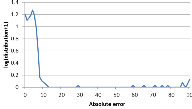
Figure 3.17: Logarithm of the distribution of face images according to the absolute error in Color Feret database.
