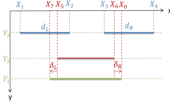
Figure 3.12: Parameters extracted from face salient element bounding boxes.
