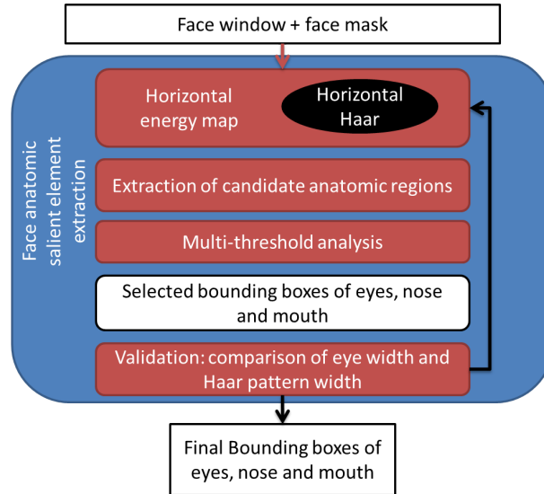
Figure 2.19: Extraction of face salient elements extraction.
