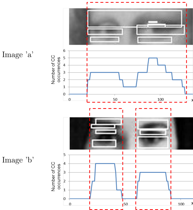
Figure 2.37: Histogram of occurrences of connected component bounding boxes on x-axis.
