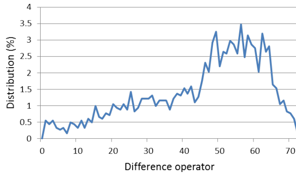
Figure 3.13: Distribution of face images (%) according to the difference operator \Delta .
