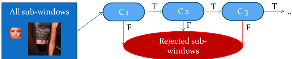
Figure 2.4: Cascade of classifiers.
