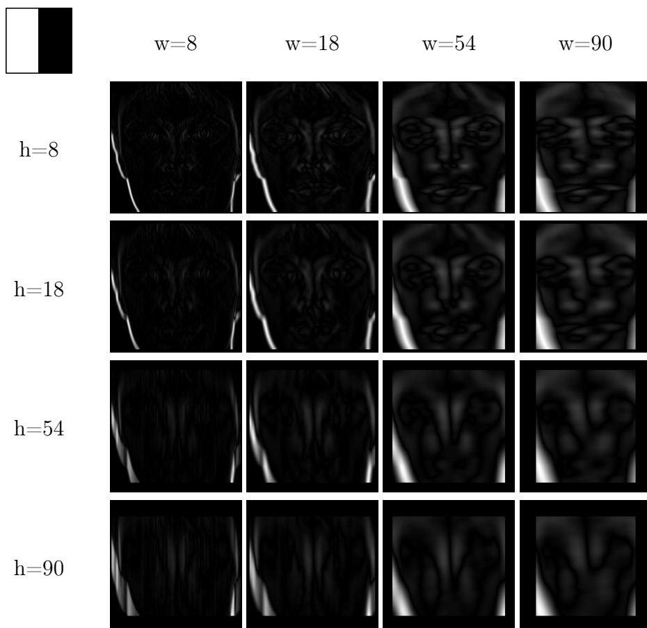
Figure 2.12: Normalized energy maps of vertical Haar filter according to the filter width w and height h in pixels. The face window width and height equal both to 364 pixels.
