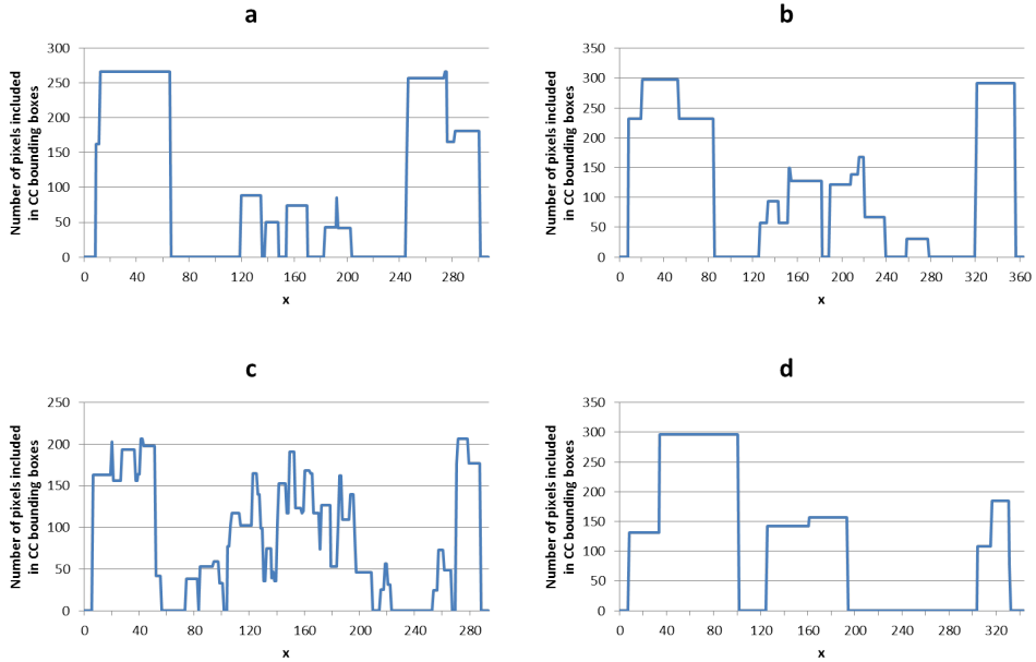
Figure 2.25: Number of pixels belonging to connected component bounding boxes according to the image column.
