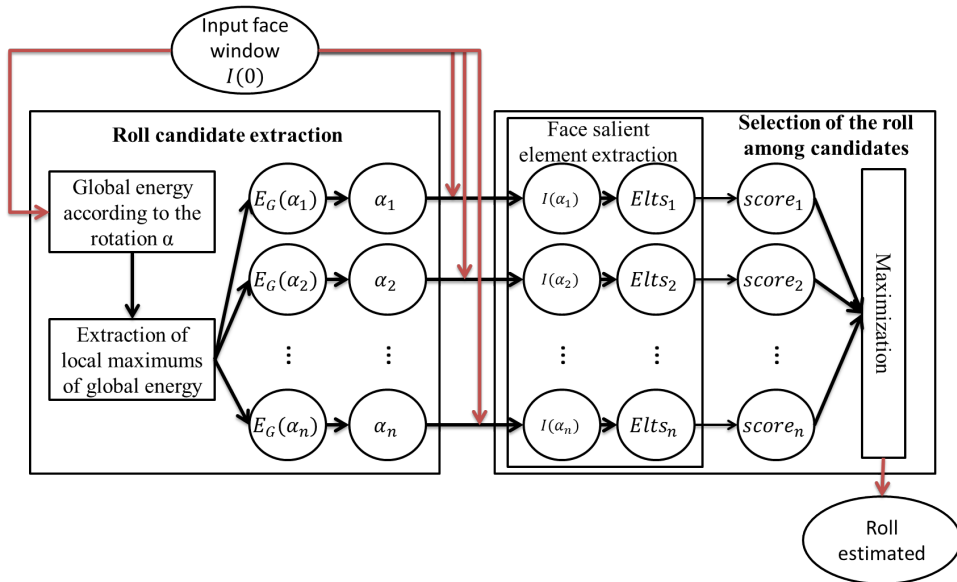
Figure 3.7: Global scheme of the roll estimation method.
