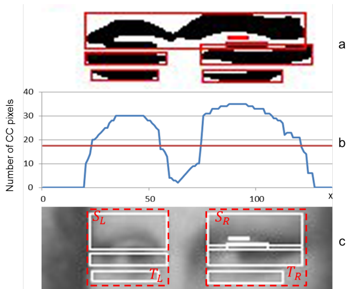
Figure 2.38: a) Initial connected components and their bounding boxes of candidate anatomic region containing both eyes. b) Number of connected component pixels according to the abscissa as well as the upper level set. c) Separation of left and right candidate anatomic regions using this level set.
