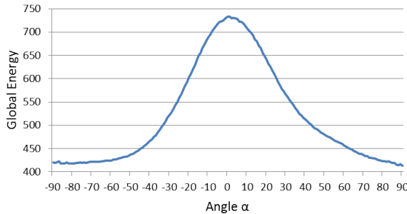
Figure 3.5: Graph of the global horizontal energy of Figure 3.4a according to the rotation \alpha . In the original image, the roll of the face is almost null.
