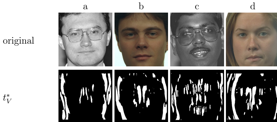
Figure 2.23: Binarized vertical energy map using adaptive threshold.
