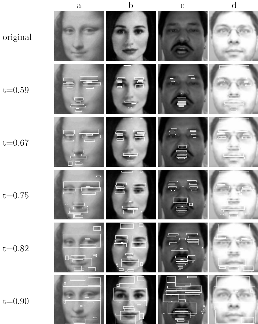
Figure 2.33: Bounding boxes of connected components according to threshold t .
