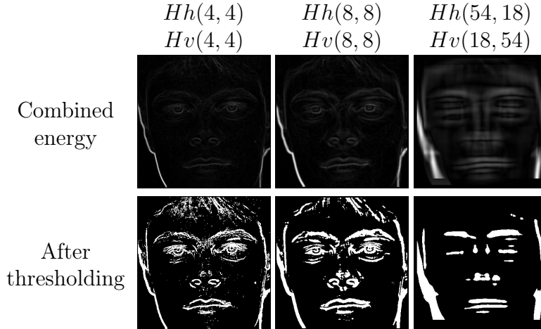
Figure 2.15: Linear combination of horizontal and vertical Haar energies. the result is an edge detector.
