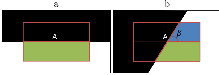
Figure 3.3: Image a illustrates a horizontal straight line with the horizontal Haar filter. Image b illustrates an oblique straight line with the horizontal Haar filter centered in A. In (a), the energy is the area of the green zone. In (b), the energy is the difference of the areas of the blue and green zones.
