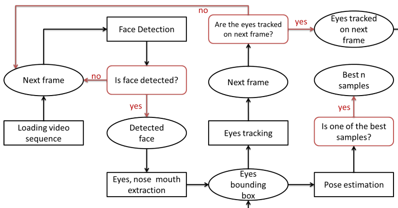
Figure 5.1: Overview of this thesis giving the best face samples among those present in a video sequence.
