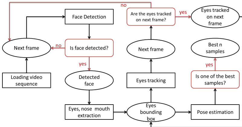
Figure 1.2: Overview of this thesis giving the best face samples among those present in a video sequence.
