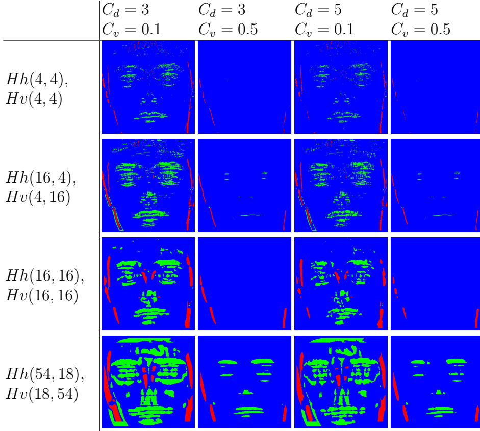
Figure 2.16: Visual results of non-linear combination of horizontal and vertical energies. Values which belong to S_{hori} is represented in green, values of S_{verti} is represented in red and other values of the combination (belonging to S_{other} ) in blue.
