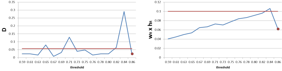
Figure 2.44: Functions D and w_R \times h_R associated with the left eye region area of image 'd' according to the threshold t .
