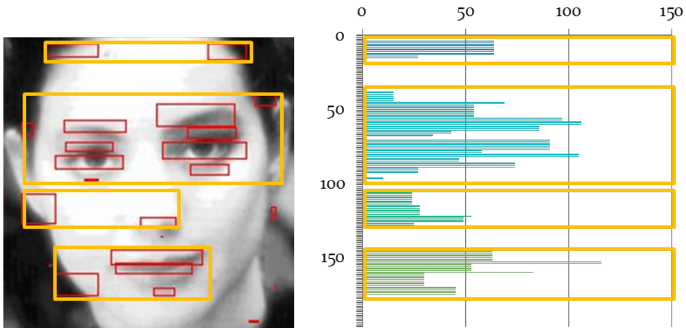
Figure 2.36: Candidate anatomic regions obtained after merging close candidate regions. four candidate anatomic regions are extracted from this histogram.
