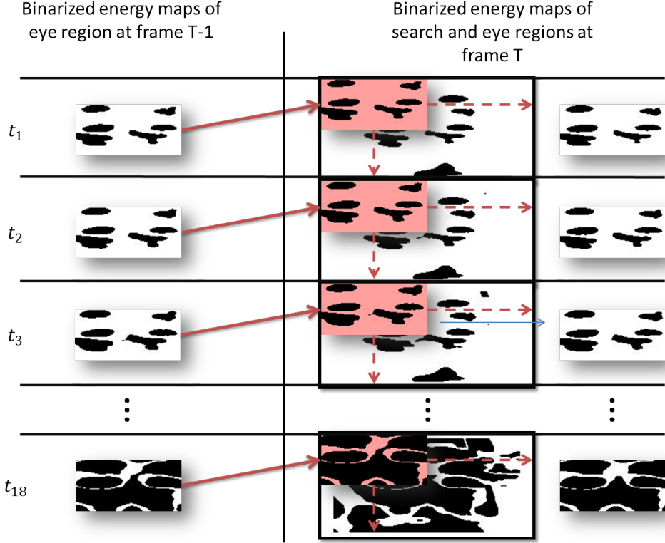
Figure 4.2: Scheme of the tracking process based on similarity of binarized energy maps.
