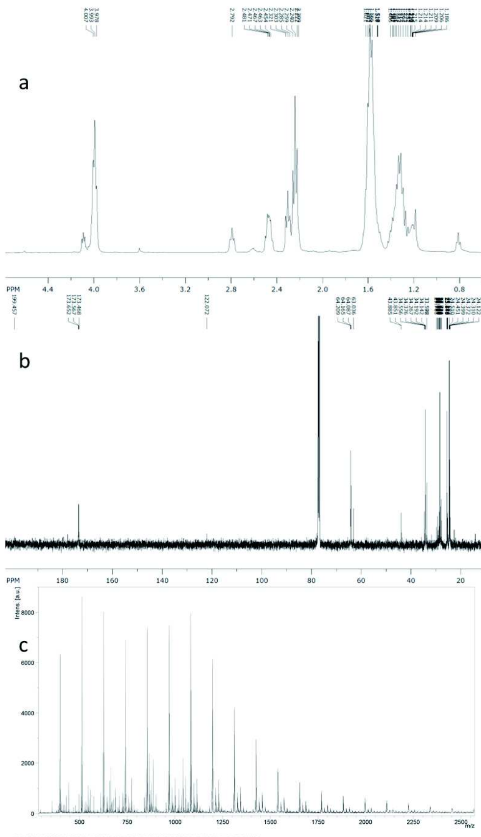
Figure SI IV-9. Copolymers N°7 (19% ε-thiocaprolactone content) synthesized by the two steps strategy; a- 1 H NMR spectrum, b- 13 C NMR spectrum, c- MALDI-ToF spectrum
