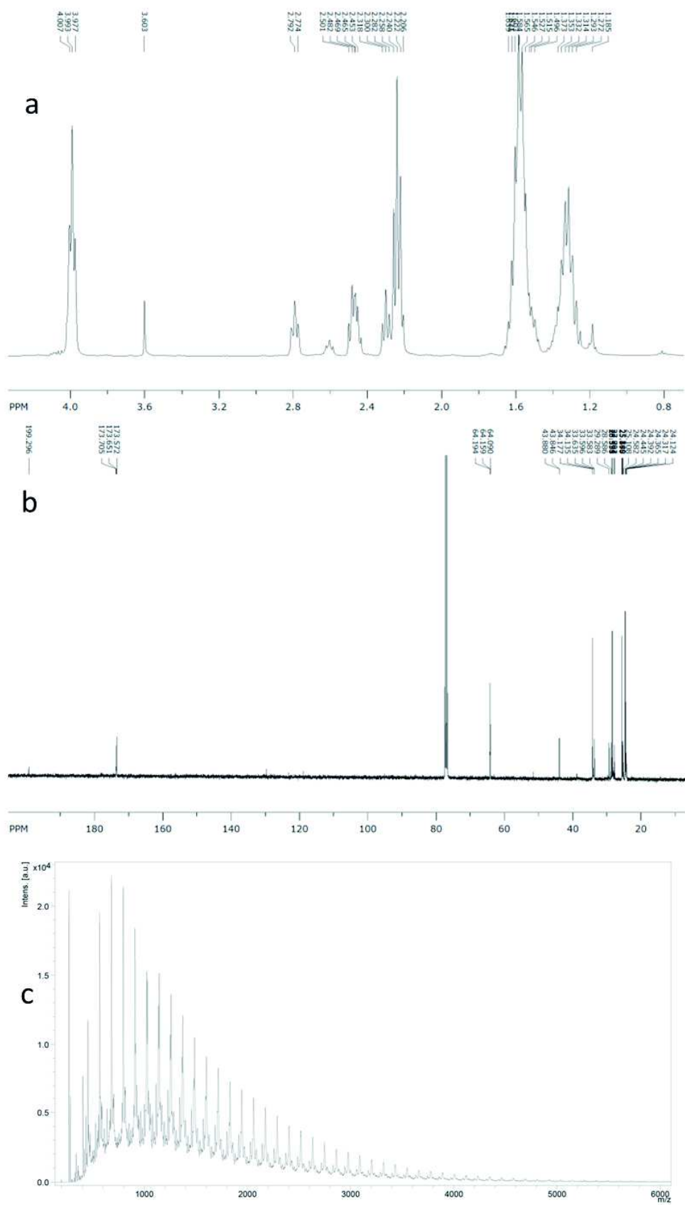
Figure SI IV-7. copolymers N°3 (27% \epsilon -thiocaprolactone content) synthesized by the one step strategy; a- ^1\text{H} NMR spectrum, b- ^{13}\text{C} NMR spectrum, c- MALDI-ToF spectrum
