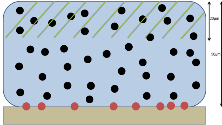
FIGURE 3.2: Schematic picture of the gel with embedded beads. The typical height of the gel is 50 to 70 \mu\text{m} , the region used for tracking is about 20 \mu\text{m}^2 (green overlay), reference beads are melted on the glass slide of the petri dish (red circles).
