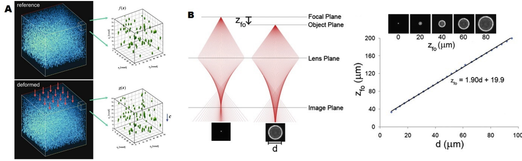
FIGURE 2.4: (a) Schematic illustration of the digital volume correlation. Sub-olumes of substrates are correlated in a stress-free (reference) state and in a deformed state. Adapted from [61] (b) Three-dimensional defocused particle-tracking method. Left : A ray-tracing diagram of light traveling through a lens. The source of light in the focal plane converges to a point at the image plane. If the point source is displaced by a distance z_{f0} , rays do not converge and they produce a defocused ring on the image plane (diameter d ). Representative images of a point source under each condition are also shown (bottom). Right : Experimentally derived calibration curve of fluorescent beads. Adapted from [62]
