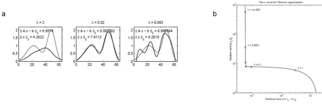
FIGURE 2.6: Figure (a) : the exact solution (thin lines) and Tikhonov regularized solutions x (thick lines) for an inverse problem Ax = b (for three values of the regularization parameter). An over- or under-estimation of \lambda yields an over- or under-smoothing of the regularized solution. Figure (b) : the L-curve for a zero-order Tikhonov regularization of the same problem as in figure (a). Adapted from [73]
