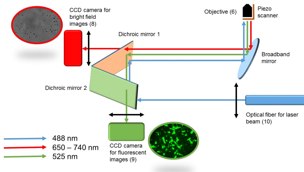
FIGURE 3.5: Setup : imaging
