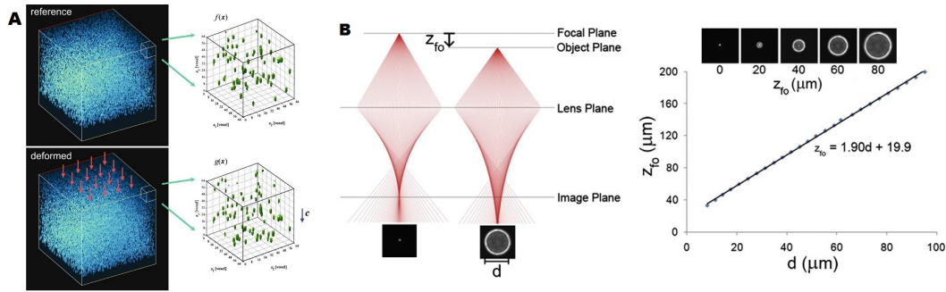
FIGURE 2.4: (a) Schematic illustration of the digital volume correlation. Sub-volumes of substrates are correlated in a stress-free (reference) state and in a deformed state. Adapted from [61] (b) Three-dimensional defocused particle-tracking method. Left : A ray-tracing diagram of light traveling through a lens. The source of light in the focal plane converges to a point at the image plane. If the point source is displaced by a distance z_{f_0} , rays do not converge and they produce a defocused ring on the image plane (diameter d ). Representative images of a point source under each condition are also shown (bottom). Right : Experimentally derived calibration curve of fluorescent beads. Adapted from [62]
