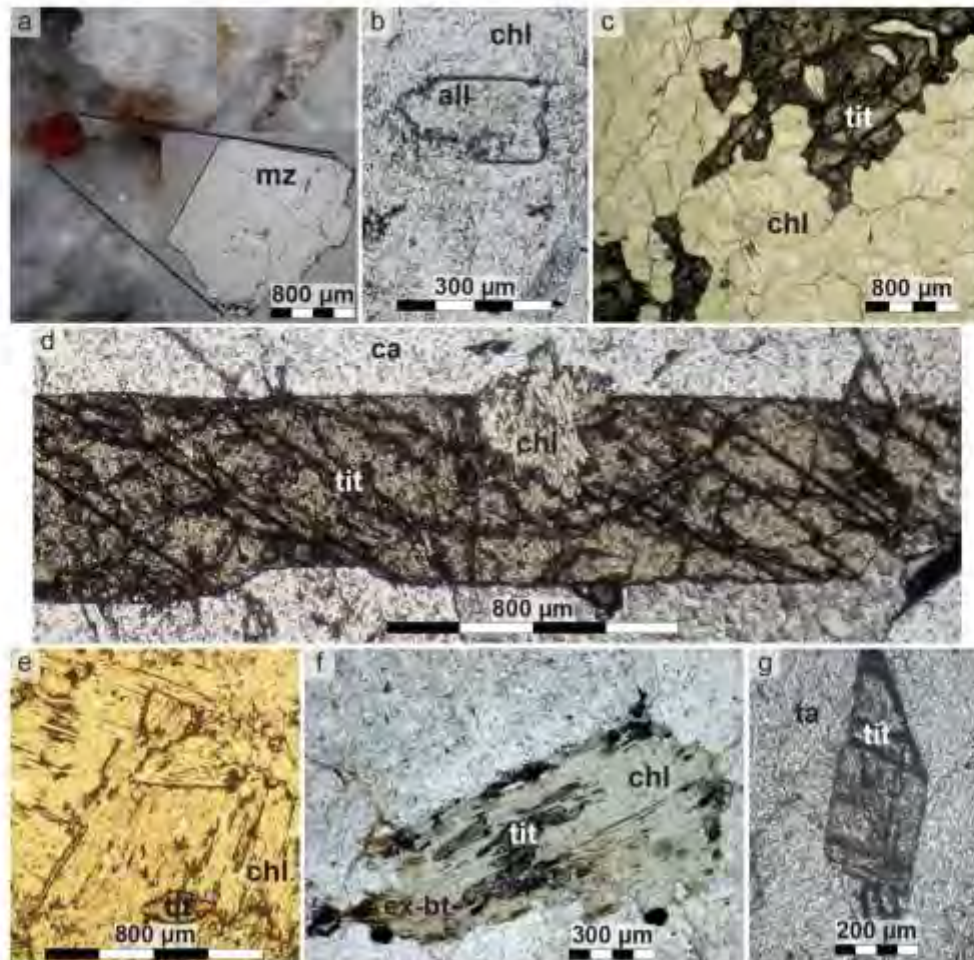
Fig. 3 Microscopic view of the minerals sampled. Trimouns: a monazite ( mz ) in dolostone geodes, macro- and SEM view, b hydrothermal allanite ( all ) in chloritized pegmatite, c anhedral titanite ( tit ) and d euhedral titanite from chlorite ( chl ) mineralization. Col de Jau: e
