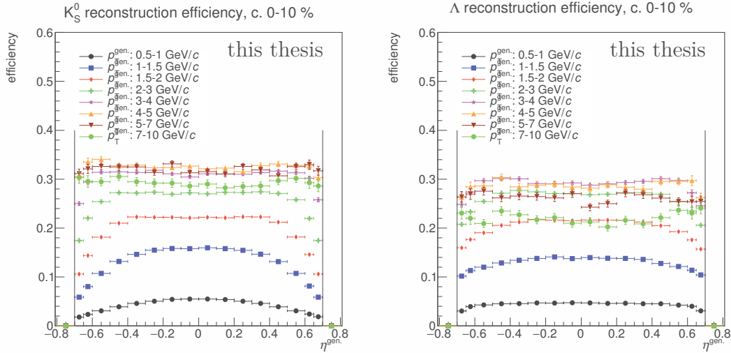
Figure 4.9: Reconstruction efficiency of inclusive K_S^0 and \Lambda as a function of p_T^{V0} and \eta_{V0} in central (0–10%) Pb–Pb collisions at \sqrt{s_{NN}} = 2.76 TeV from year 2011.
