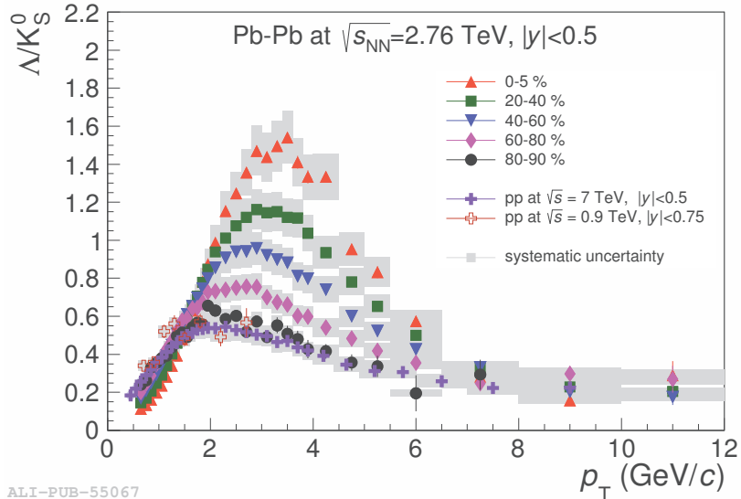
Figure 1.8: Inclusive \Lambda/K_S^0 ratio in Pb–Pb collisions at \sqrt{s_{\text{NN}}} = 2.76 \text{ TeV} measured by ALICE as a function of centrality compared with the ratio in p–p collisions [64].
