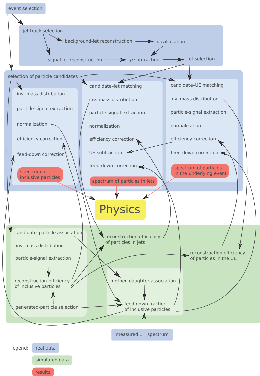
Figure 4.1: Analysis workflow.
