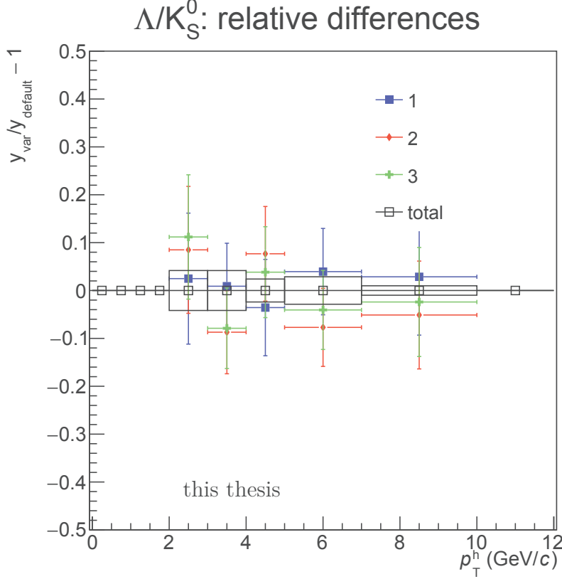
Figure 4.19: Deviations of the (\Lambda + \bar{\Lambda})/2K_S^0 ratio in jets ( R = 0.2, p_T^{\text{jet, ch}} > 10 \text{ GeV}/c ) in central (0–10%) Pb–Pb collisions at \sqrt{s_{NN}} = 2.76 \text{ TeV} from year 2011 resulting from changing boundaries of the signal extraction regions.
