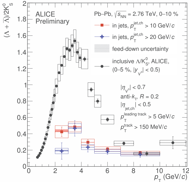
Figure 5.8: \Lambda/K_S^0 ratio in charged jets reconstructed with R = 0.2 in central (0–10%) Pb–Pb collisions at \sqrt{s_{\text{NN}}} = 2.76 \text{ TeV} from year 2011 for p_T^{\text{jet, ch}} > 10 \text{ GeV}/c and p_T^{\text{jet, ch}} > 20 \text{ GeV}/c , compared with the inclusive ratio.
