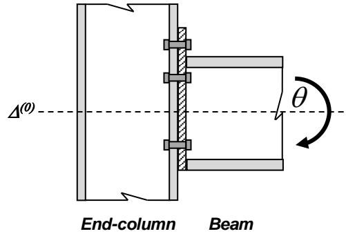
Figure 2.9: Extended end-plate connection
