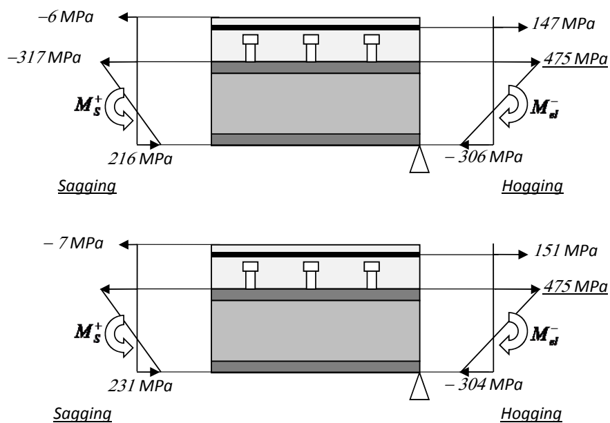
Figure 4.17: (a) Stress distribution in sagging and hogging cross-sections Calculation1 (ALM)– \mathbf{p} = 280 \text{ kN/m} . (b)Stress distribution in sagging and hogging cross-sections Calculation2 (ALM + FNC) – \mathbf{p} = 264 \text{ kN/m} .
