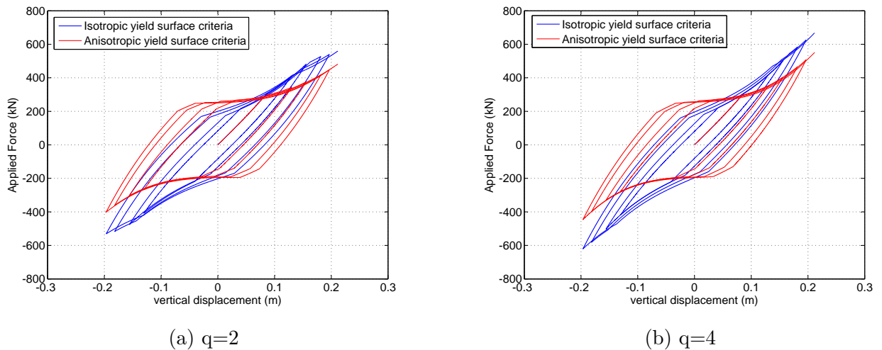
Figure 3.14: Reversed displacement-controlled cyclic loading with increasing amplitude: Isotropic versus Anisotropic yield criteria
