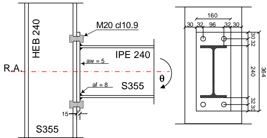
Figure 2.14: Example for the gap effect
