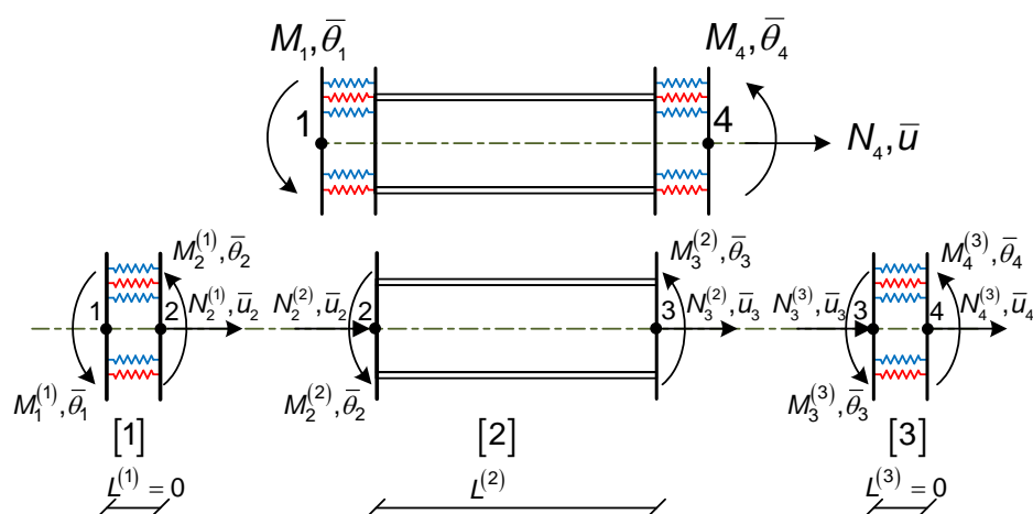
Figure 2.12: Finite joint element
