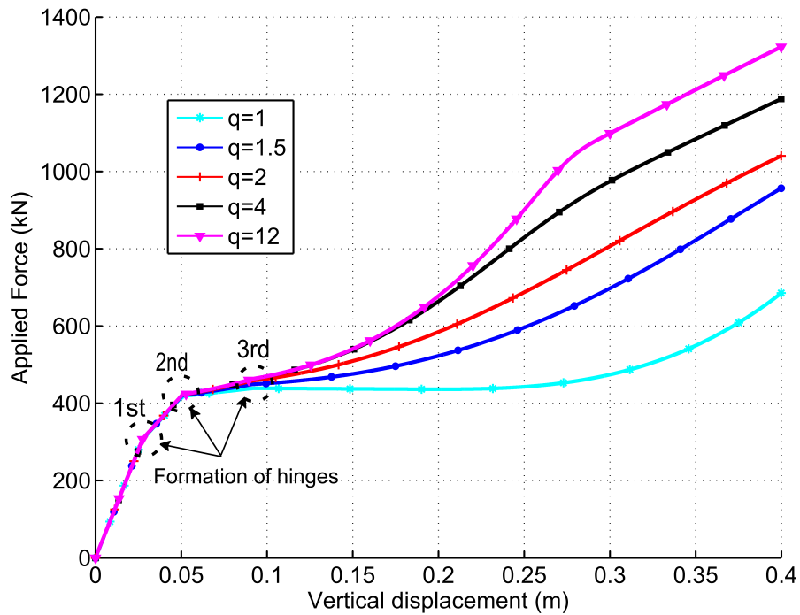
Figure 3.12: Beam load-deflection curve
