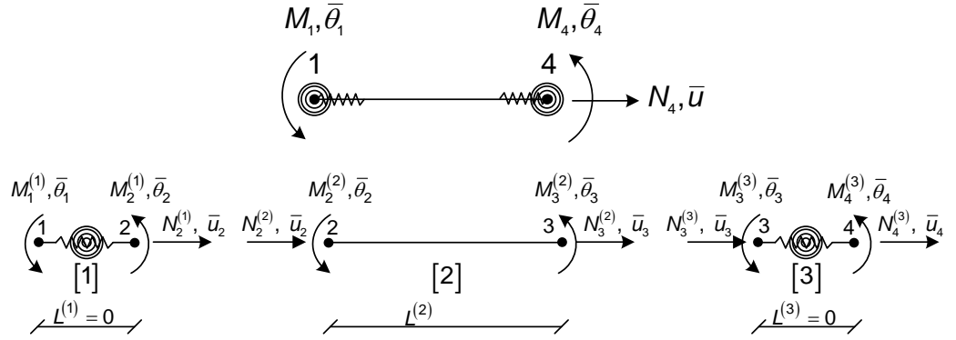
Figure 3.1: Local superelement
