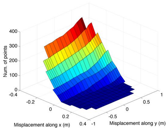
Figure 8.11: Dimension of the volume having magnetic flux density higher than the limit value of 27 \mu\text{T} . Missing points refer to conditions of coupling in correspondence of which the system is turned off.
