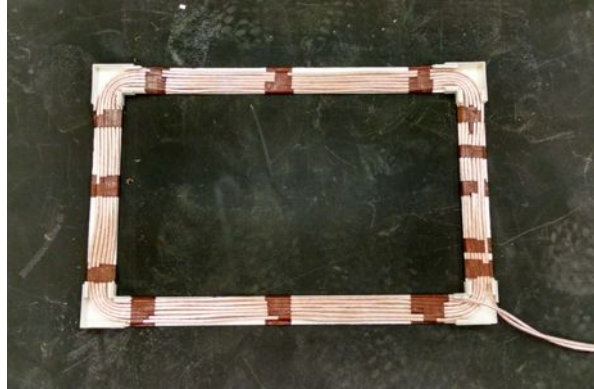
Figure 7.8: Coil for the laboratory tests.
