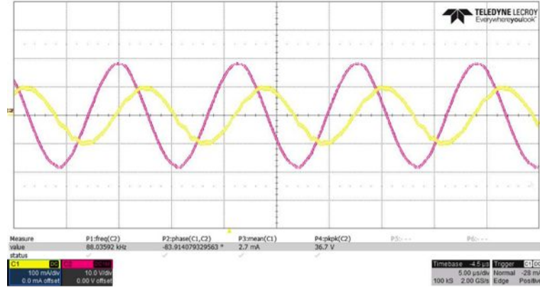
Figure 7.6: Waveforms of the voltage (magenta) 10 V/div and current (yellow) 100 mA/div at the output of the linear power amplifier. Time axis 5 \mu s/div.
