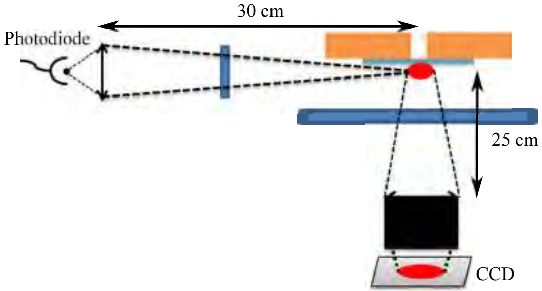
Figure 94: Schematic representation of the detection systems. Another CCD imaging setup identical to the one represented here is directed parallel to the chip surface.
