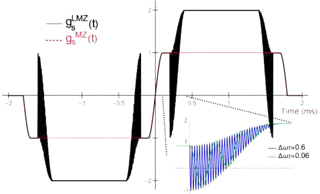
Figure 69: Complete sensitivity function (black) of eq. (104) compared to the three pulse sensitivity function (red, dashed). The interferometer parameters are T = 1 ms, \tau = 100 \mu s and \omega_D = 0 . A comparison of the energy dependent part for two smaller impulsion times \tau = 10 \mu s (blue) and \tau = 1 \mu s (green) is shown on the bottom right.
