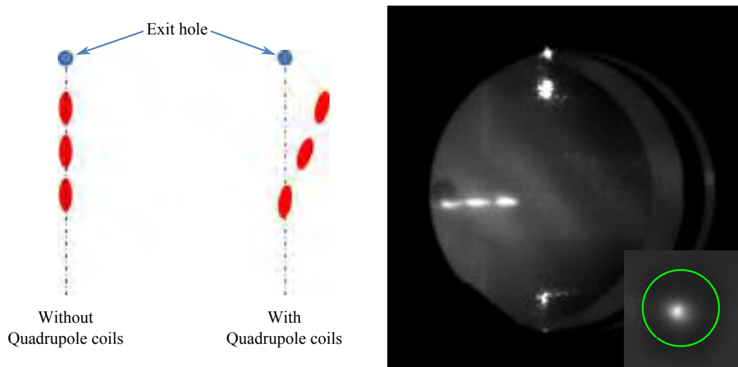
Figure 97: Right hand side: Picture of the 2D MOT clouds taken from the push beam view-port. The camera is slightly out of alignment to show the three cigar shaped regions. The exit hole is the black circle in the background. The vertical bright spots correspond to light scattered by edges inside the chamber. The bottom right inset corresponds to the in-axis view once the three clouds were aligned on the exit hole (emphasized by the green circle). Left hand side: Effect of the quadrupole magnetic field on the 2D MOT prior to magnetic shielding and current imbalance between the 2D MOT coils.
