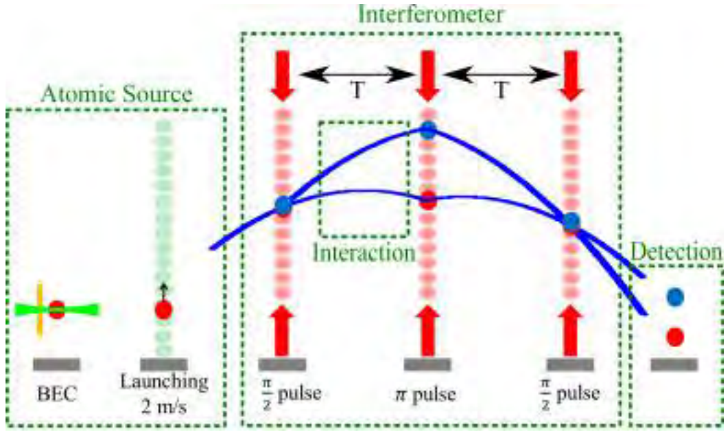
Figure 46: The four (dotted green) parts of our dual isotopes interferometer.
