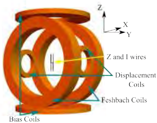
(a) Magnetic coils configuration
