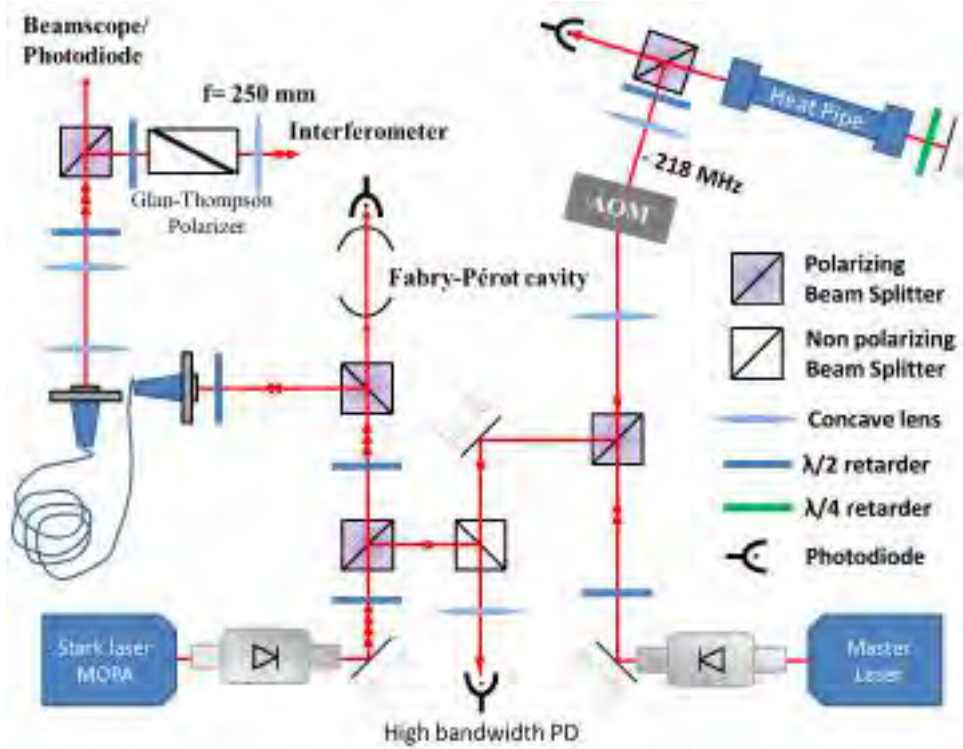
Figure 33: Schematic view of the laser system for phase shifting one arm of the interferometer. A master laser, locked to the blue (218 MHz) of the D1 line with saturated absorption is used as a frequency reference. The Stark laser is locked on a confocal Fabry-Pérot cavity 1 – 4 GHz to the blue of the D1 line. A weak beam of the Stark laser is sent to a high bandwidth photodiode which records the beat note between the two lasers. The main beam is sent with a polarization maintaining fiber to the interferometer breadboard. On this breadboard, the laser beam is shaped, polarization purified with a Glan-Thompson polarizer and focused on one of the interferometric arms. A fraction of the power sent on the atomic beam is also monitored.
