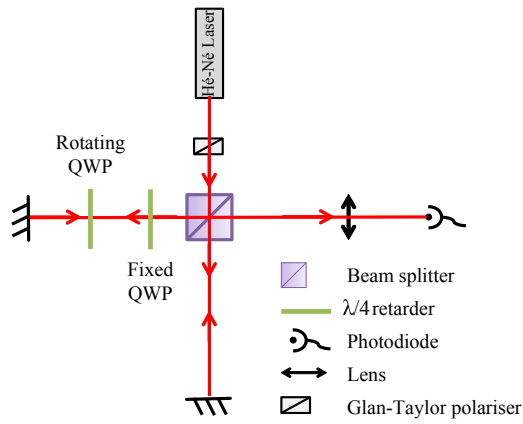
(b) Michelson set-up
