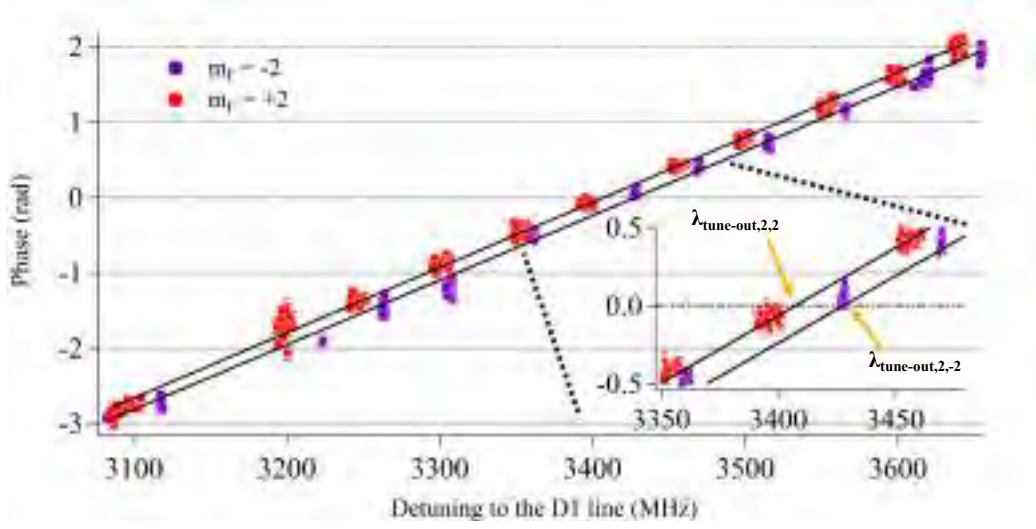
Figure 43: Phase shifts as a function of the laser detuning to the D 1 line. The laser power is fixed at the highest power of 34 mW to increase the phase sensitivity. The shift between the two polarized states 'tune-out' wavelengths is visible and corresponds to 20.5(5) MHz.
