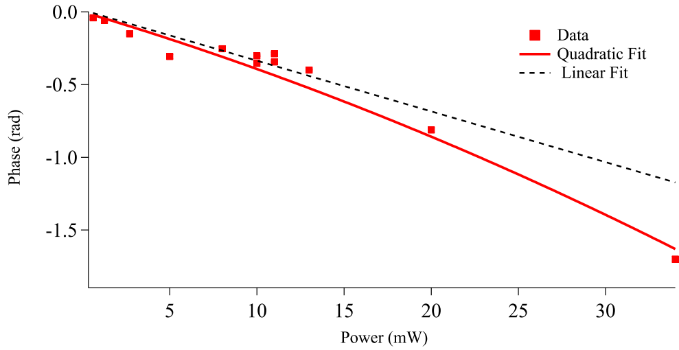
Figure 41: Phase shifts as a function of the laser power at a fixed detuning of 3200 MHz. The red squares are data points and the lines are fits with linear or quadratic power dependence. The deviation from a linear behavior is due to hyperpolarizability components in the Stark shift.
