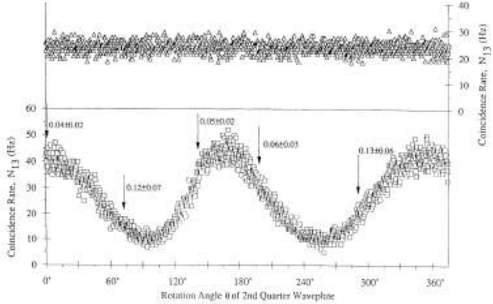
Figure 24: Figure adapted from [154] representing coincident optical interference fringes. The rotation angle of the quarter waveplate scans the Pancharatnam phase. The interference signal top (resp. bottom) corresponds to a broad (resp. narrow) energy filter shows revival of the fringes visibility when the photon distribution is narrow. The arrows indicate the measured triple anticorrelation parameter, ensuring the non-classical state of the detected photons.
