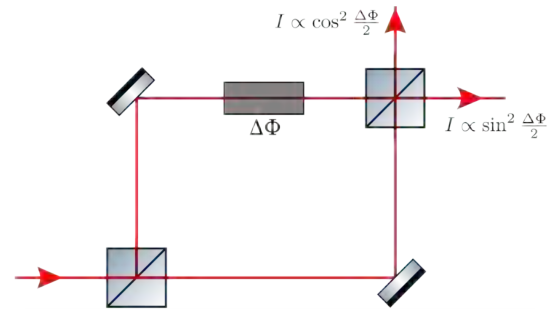
Figure 3 Optical Mach Zehnder interferometer relying on two beam splitters and two mirrors.
