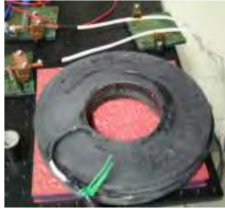
(b) Experimental realization
