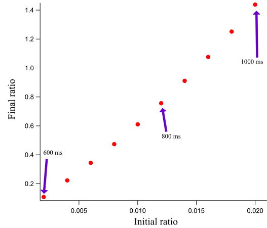
Figure 59 Final atom number ratio N_{85,\text{final}}/N_{87,\text{final}} as a function of the initial atom number ratio N_{85,\text{ini}}/N_{87,\text{ini}} . The evaporation duration for initial ratios of 0.002, 0.012 and 0.02 are represented besides the points.
