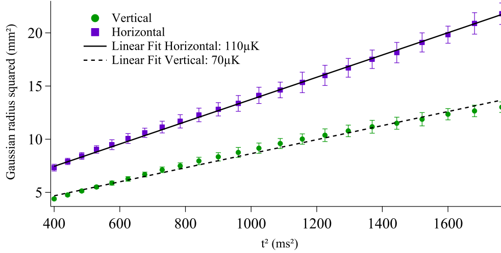
Figure 109: Typical time of flight measurement used for Fig. 108. TOF larger than 20 ms are represented as the density is initially too large for our imaging system. The bi-modal distributions are merged which improves the Gaussian width extraction as can be seen by the more regular behavior of the two orthogonal directions. A discrepancy between the two temperatures remains but almost vanishes when the cloud is completely compressed (see Fig. 108 at \delta_1 = -16\Gamma ).
