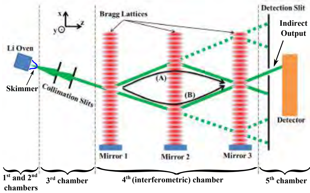
Figure 4: Schematic representation of our Mach-Zehnder lithium interferometer. Four distinct regions separate the lithium source, the collimation slits, the interferometer itself and the detection.
