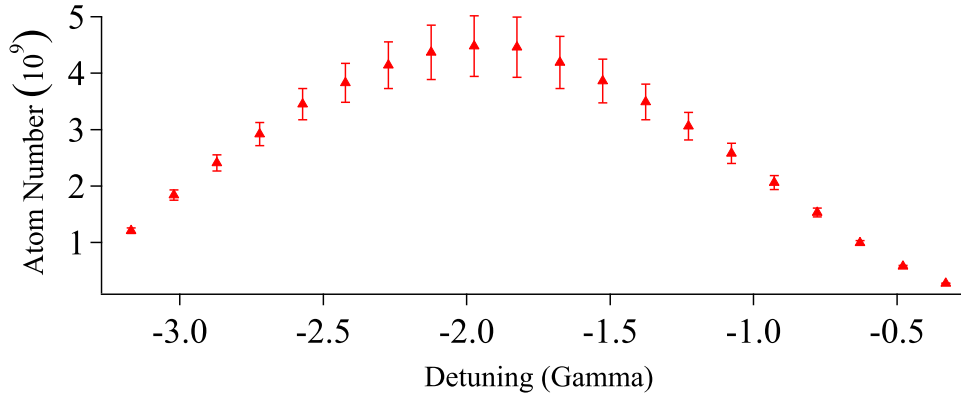
Figure 106: Asymptotic number of loaded atoms as a function of the cooling laser detuning \delta_1 . The maximum around -2\Gamma corresponds to a competition between the radiation pressure and the trapping force.
