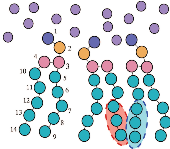
FIG. 1. Example of coarse-grained lipid molecule (DOPC) with bead labels, and two terminal subgroups during a “collision event”.
