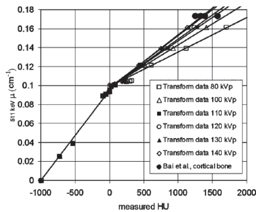
Figure 13: Bilinear scaling to convert CT intensities (HU) into attenuation coefficients ( \text{cm}^{-1} ) for PET energies (lower energies than 80 kVp not in diagram, lines not always on points but uncertainty not estimated). Some manufacturers use different scaling. Source (Carney et al., 2006).
