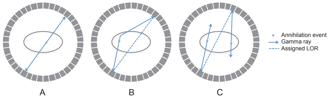
Figure 6: PET detector ring (dark grey) and object to be imaged (oval). Three coincidence types: true coincidence (A), scatter coincidence (B) and random coincidence (C).
