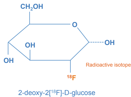
Figure 3: The [ ^{18}\text{F} ]FDG molecule consisting of the chemical compound incorporating the radioactive isotope.
