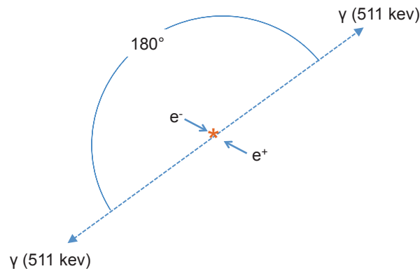
Figure 5: Annihilation reaction.
