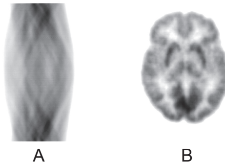
Figure 7: Sinogram (A) and reconstructed brain image (B) corresponding to sinogram. Source: (Fahey, 2002).
