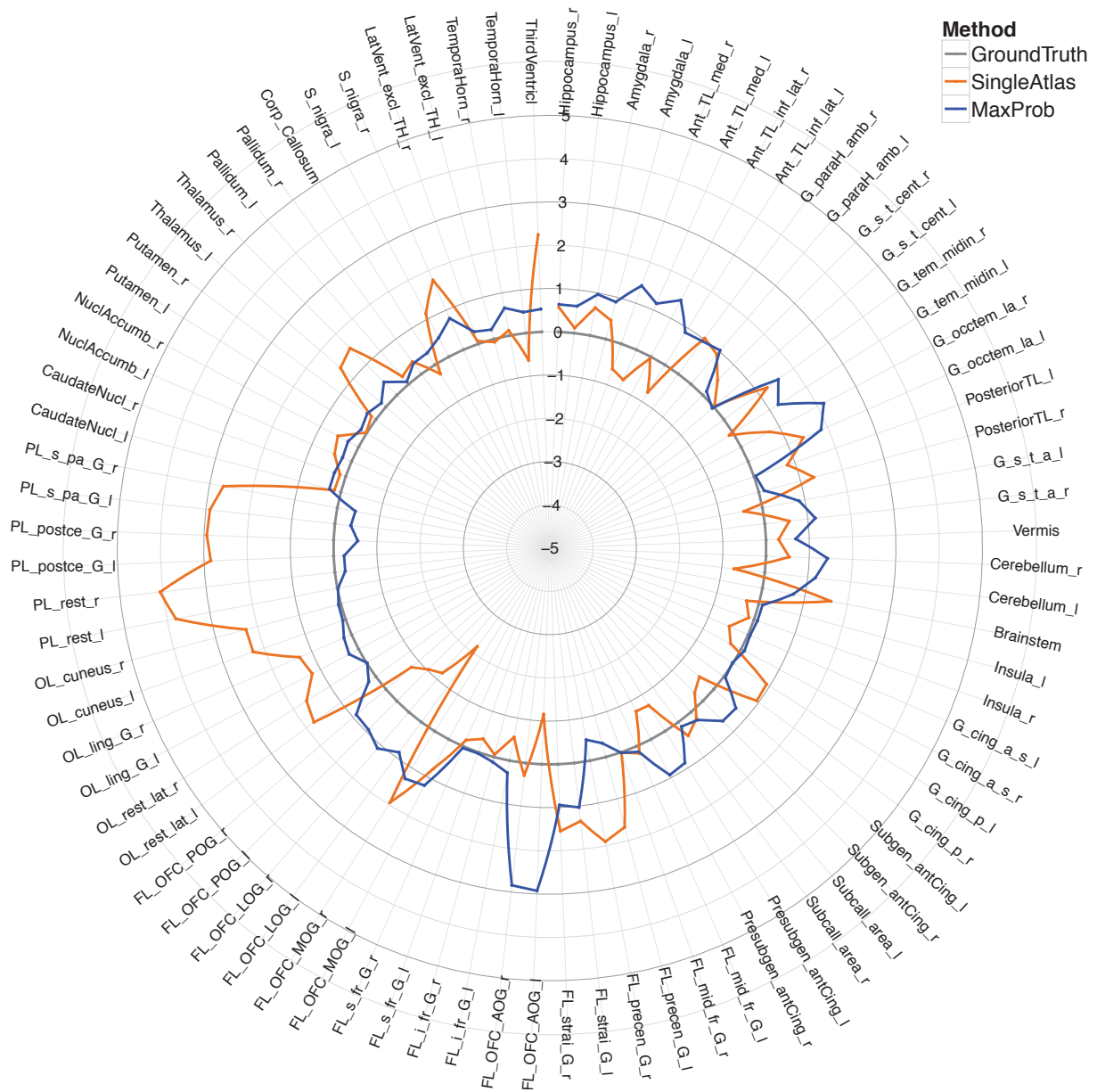
Figure 31: Mean bias for PET [^{18}\text{F}]\text{FDG} , per ROI and per AC method for PET data reconstructed with the filtered back-projection algorithm. Bias (in %) is represented in the radial axis. The regions correspond to the 83-region version of the Hammers_mith atlases ( www.brain-development.org ), with the cerebellar vermis added (see Methods). R, right; I, left; G, gyrus; TL/FL/OL/PL, temporal/frontal/occipital/parietal lobe; OFC, orbitofrontal cortex. For a full list of abbreviations, see Appendix (Table 10). The results obtained with filtered back-projection were very similar to those obtained with the iterative reconstruction algorithm (Figure 27).
