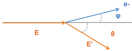
Figure 9: Compton scattering.
