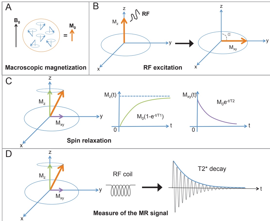
Figure 1: Physical basis of the MR signal. Macroscopic magnetization at equilibrium including precession (A), Radio-frequency applied to disturb the equilibrium (B), Spin relaxation: recover of longitudinal compound and decay of transverse compound (C), Measure of the MR signal (D).
