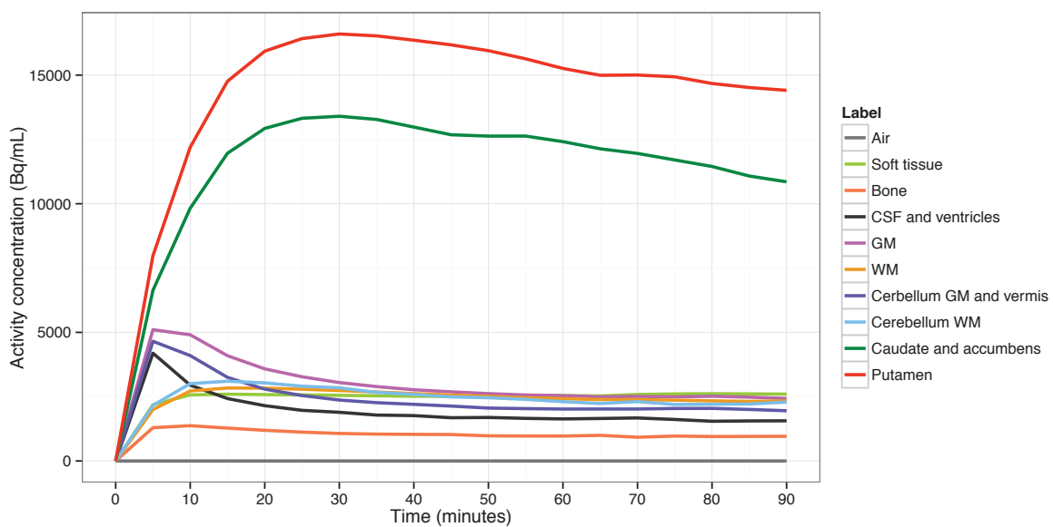
Figure 47: Regional TACs calculated from real PET/CT data and used as input for PET-SORTEO simulations.
