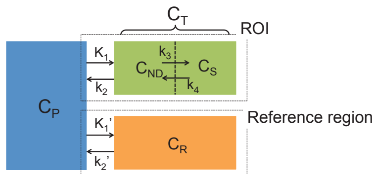
Figure 34: Compartmental model.
