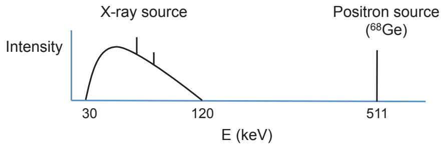
Figure 12: Spectral distributions for x-ray and PET photons (not to scale). X-ray sources produce a polychromatic spectrum. The peaks in the characteristic x-rays represent discrete energies corresponding to the transition of orbital electrons in the target material.
