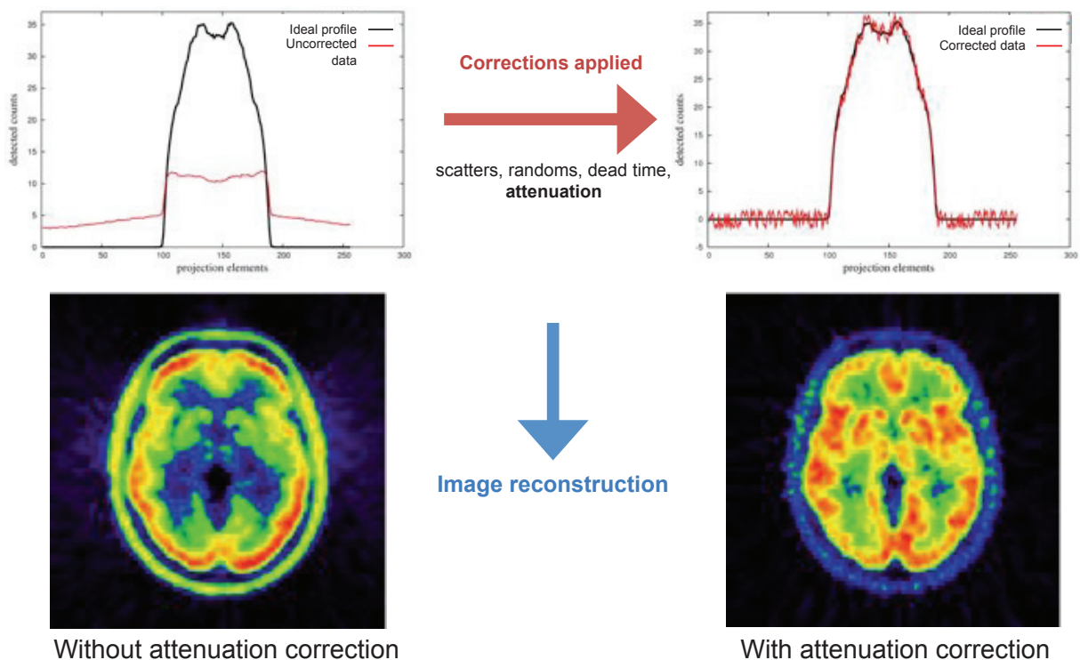
Figure 10: Errors induced in the PET image by the absence of attenuation correction (Source: courtesy from Anthonin Reilhac).
