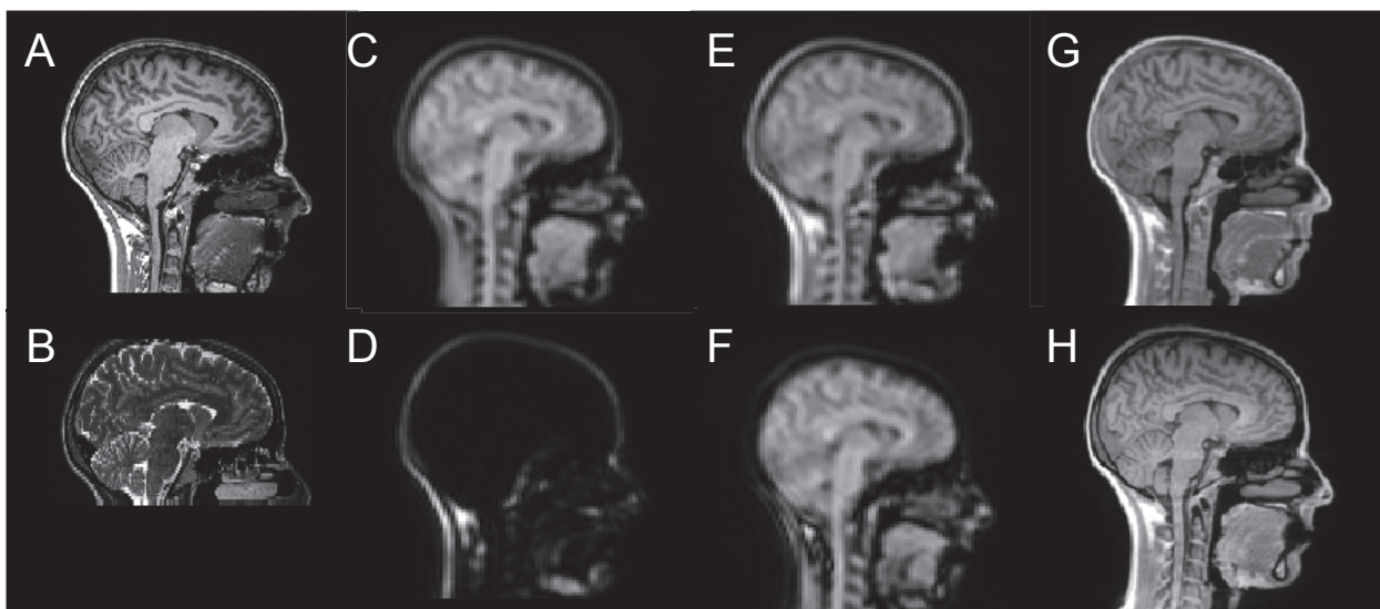
Figure 2: MRI contrasts: T1-weighted (A), T2-weighted (B), Dixon-Water (C), Dixon-Fat (D), Dixon in-phase (E) and Dixon out-of-phase (F), UTE1 (G), UTE2 (H).
