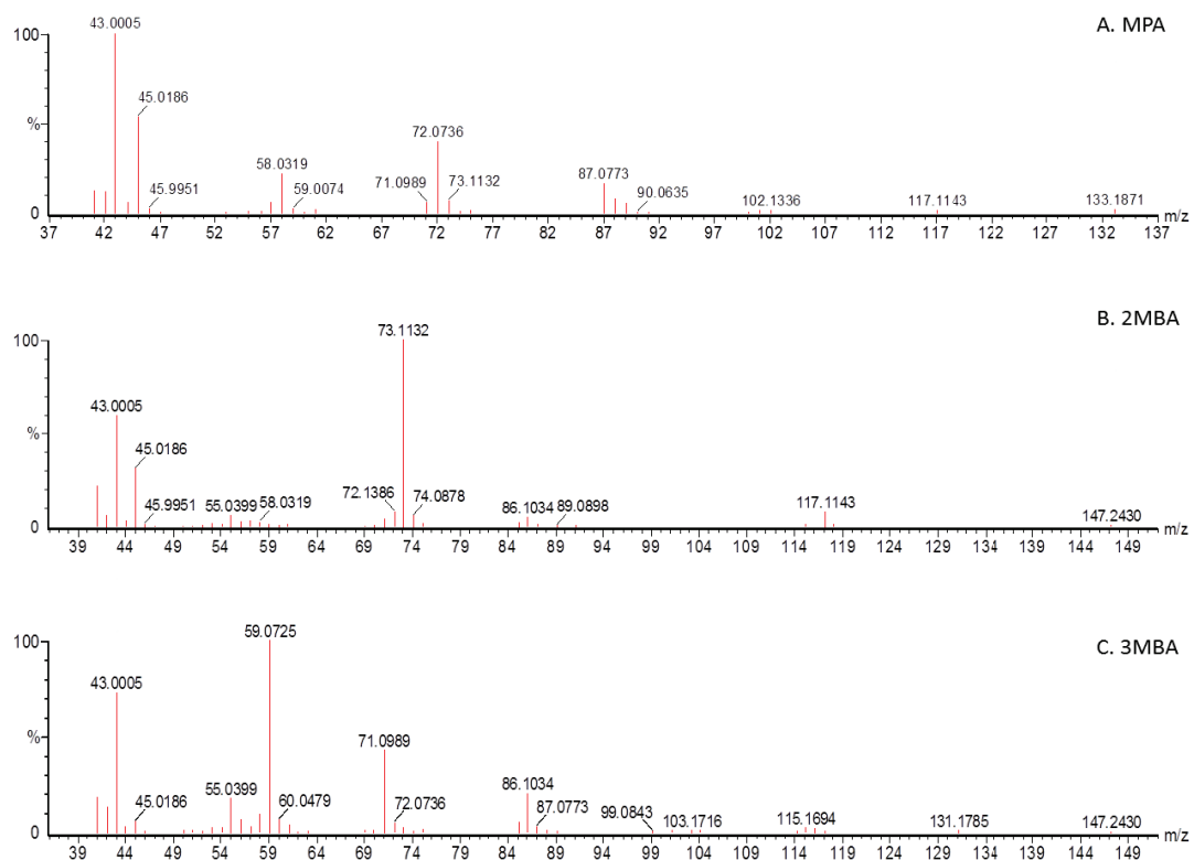
Figure 5: Mass spectra of A) MPA, B) 2MBA and C) 3MBA using the ATD-GC-MS.
