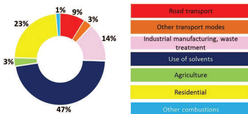
Figure 1.10: Sectors of non-methane VOCs anthropogenic emissions, in 2014, in France metropolitan according to the national inventory report 2016 of the “Centre Interprofessionnel Technique d'Etudes de la Pollution Atmosphérique” (Citepa). 18
