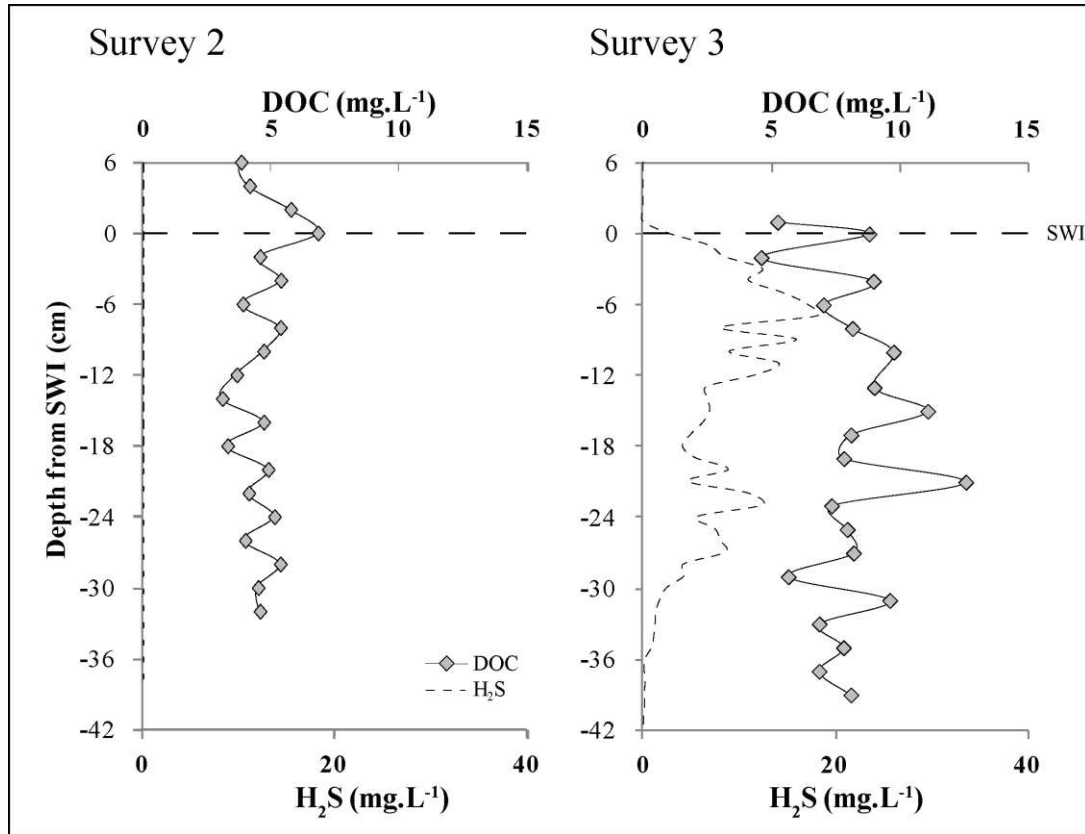
Figure 2 : Dissolved organic carbon (DOC) and sulfide concentrations in the pore water and overlaying water during the Surveys 2 and 3.
