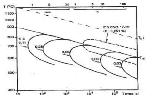
Figure 10: Effect of carbon content on sensitibilization behavior of a 18Cr10Ni steel (AISI 304). T_m is the maximal temperature for carbide existence and T_s is the maximal temperature for the onset of sensitization [20].
