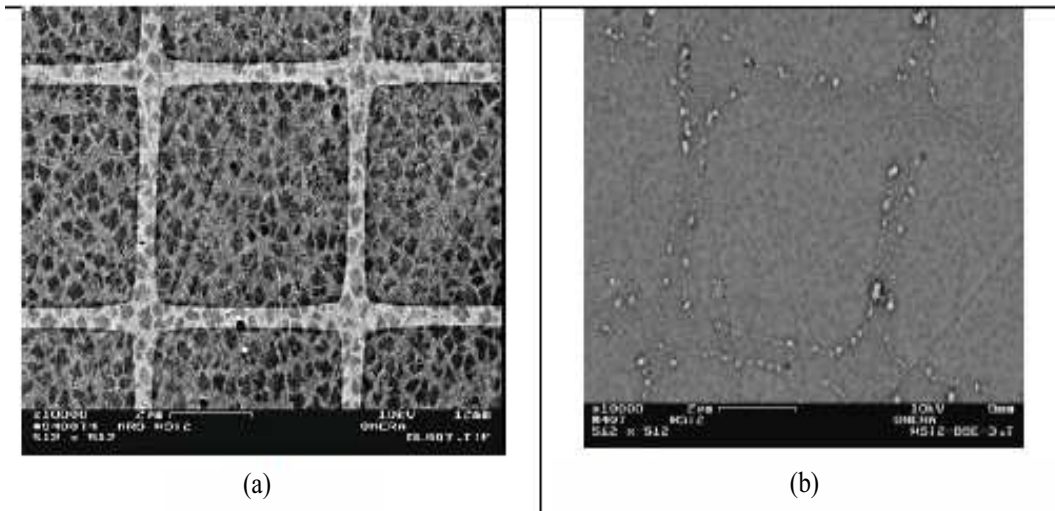
Figure 57: Grid pattern made of WSi_2 (a) after 460h at 750 °C in high vacuum environment with oxygen trappers [56].
