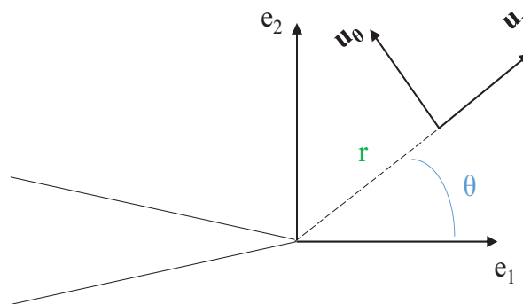
Figure 86: Local coordinate system around the crack tip.
