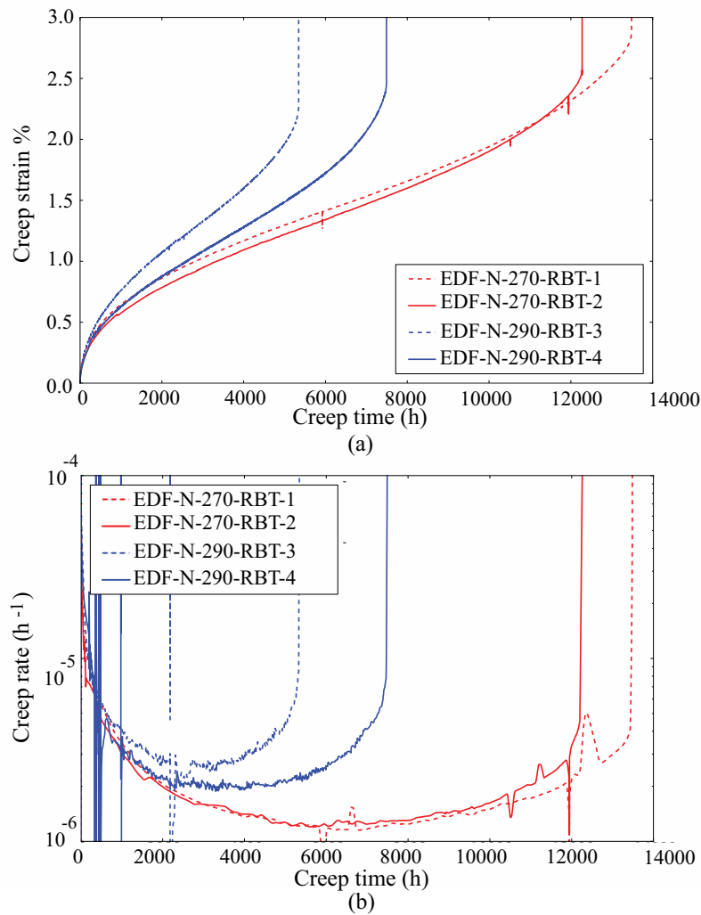
Figure 61: Creep strain as a function of time ( T = 550 °C in air) for EDF-N-270-RBT and EDF-N-290-RBT (a) and corresponding creep strain-rates (b).
