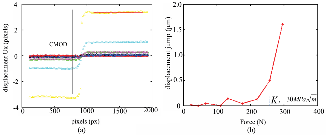
Figure 120: Displacement jumps along the profile (in pixels) (a) and displacement jump ( \mu\text{m} ) (b) considering the loading levels (b) computed between the unloaded and the loaded image for each cycle.
