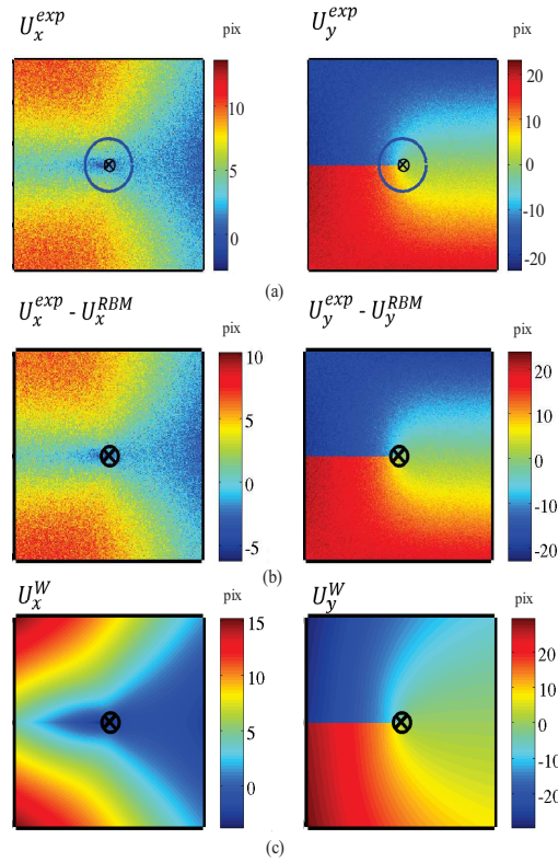
Figure 104: Comparison between the displacement fields for IE-ID ( R_{max} = 128 pixels) and multiple sources of error: u_x^{exp} , u_y^{exp} (a), u_x^{exp} - u_x^{RBM} , u_y^{exp} - u_y^{RBM} (b) u_x^W , u_y^W (c). Notations u_x^{RBM} and u_y^{RBM} stand for the displacement field associated to the rigid body motion (translation and rotation). The cross symbol is used for the estimated values whereas the circle symbol is used for the optimized values. The thick blue circle is used for R_{max} .
