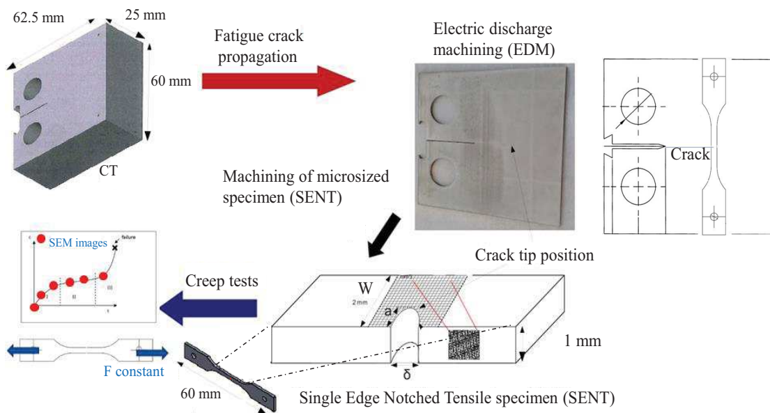
Figure 36: Methodology description for performing creep tests on microsized sample (SENT).
