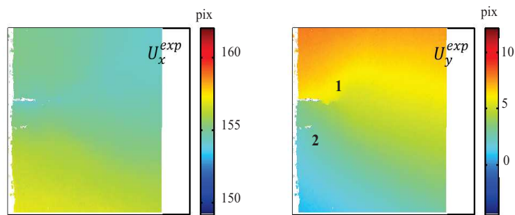
Figure 145: Kinematic fields between Figure 144 a and Figure 144 b. Two discontinuities are visible and are labelled 1, 2.
