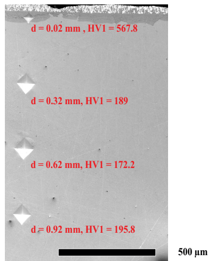
Figure 43: SEM image in BSE mode (Z contrast) of sample after 2,000 h of preconditioning exposure time. The scale bar is 500 \mu\text{m} .
