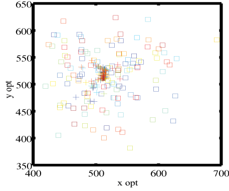
Figure 101: Representation of x^{opt} , y^{opt} for multiple source of errors on the estimated crack parameters for IE-WS R_{max} = 512 pixels. The square symbol is used for the estimated values and the cross symbol is used for the optimized values.
