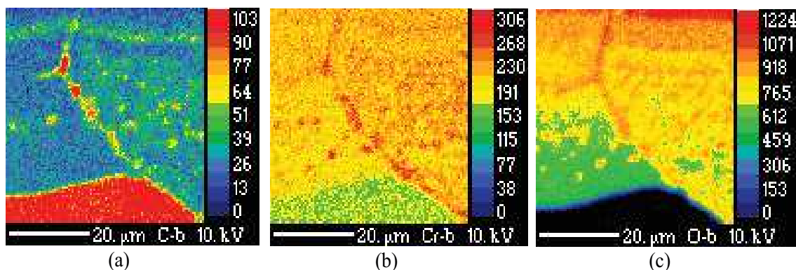
Figure 48: Chemical maps for the same ZOI as in Figure 47 b, Figure 47 c: Carbon elements (a), Chromium elements (b) Oxygen elements (c) using EPMA.
