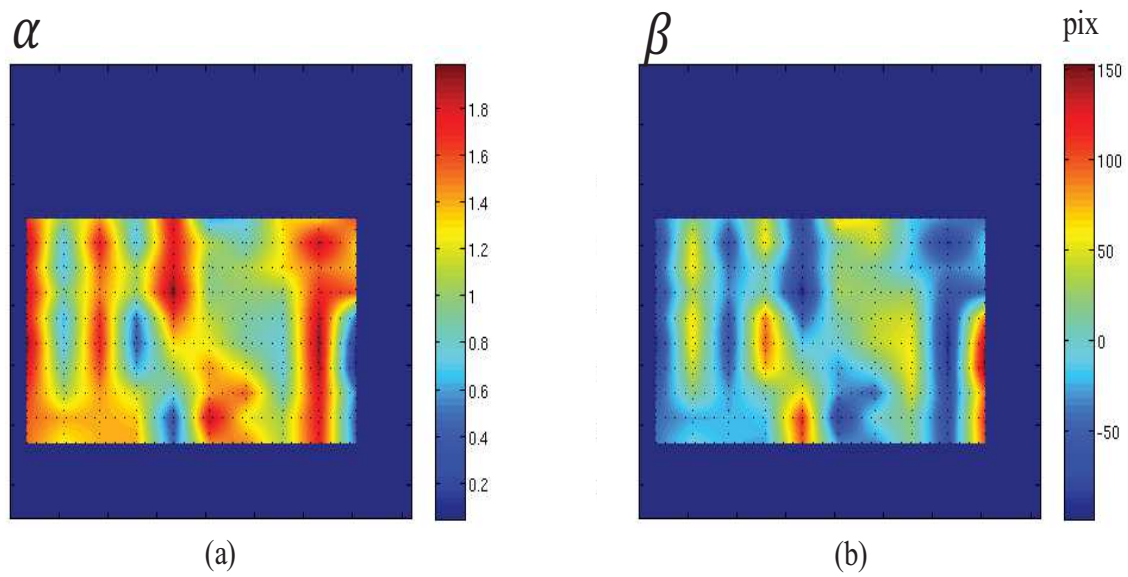
Figure 191: Representation of gain \alpha^e (a) and offset \beta^e (b) for each element e . Mesh of 10 x 10 elements appears using black dashed-lines.
