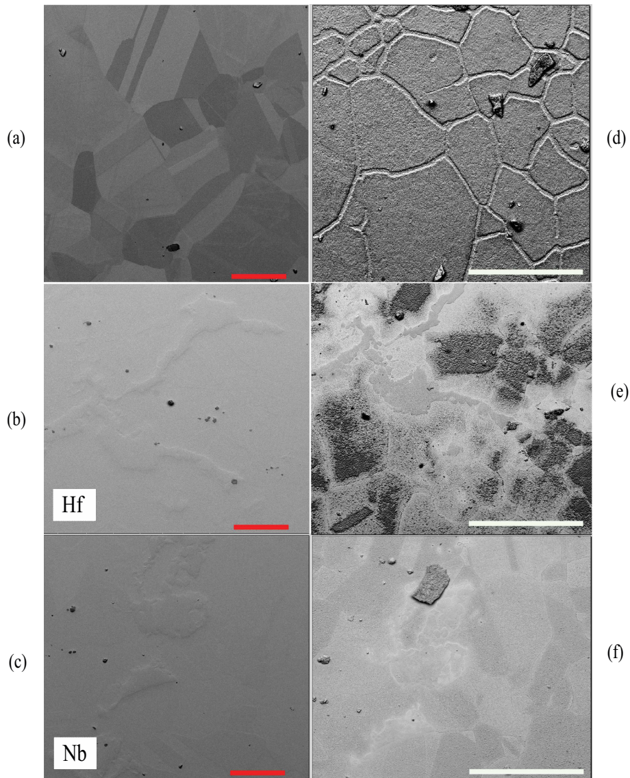
Figure 178: SEM images of 316L sample before and after ten weeks at 550 °C in air oxidation (a, d) after etching with OPS (b, e) covered by hafnium and (c, f) niobium. The red scale bar is 50 \mu\text{m} and the white scale bar is 100 \mu\text{m} .
