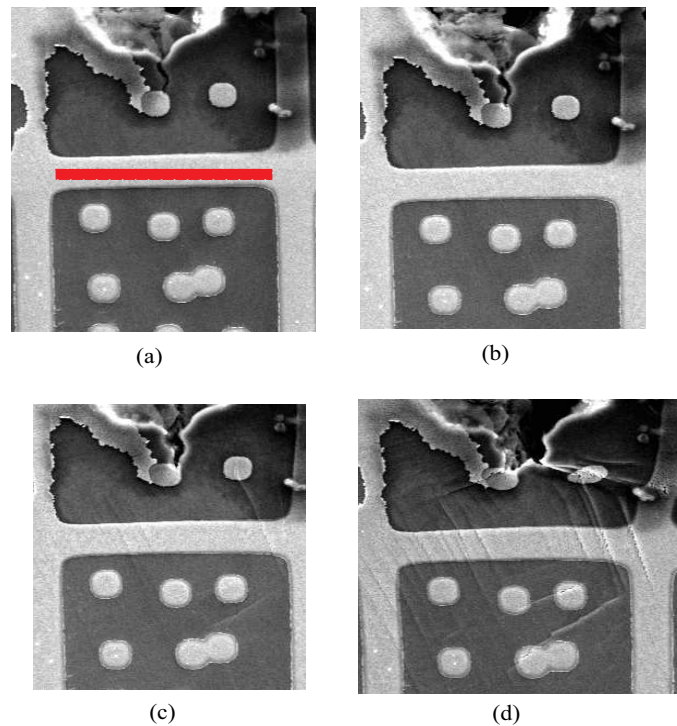
Figure 123: SEM images in SE mode in the crack tip region (a) 44 N, (b) 220 N, (c) 257 N (apparition of slip bands) and (d) 295 N. Magnitude: \times 1411 . The red scale bar is 10 \mu\text{m} .
