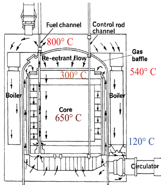
Figure 3: Description of gas flow in AGR [1].
