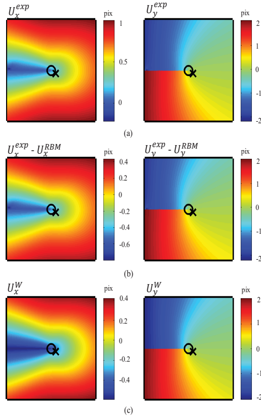
Figure 95: Comparison between the displacement fields for IE-WS ( R_{max} = 512 pixels) and \sigma_{x_0}^{est} , \sigma_{y_0}^{est} = 50 pixels: u_x^{exp}, u_y^{exp} (a), u_x^{exp} - u_x^{RBM}, u_y^{exp} - u_y^{RBM} (b) u_x^W, u_y^W (c). Notations u_x^{RBM} and u_y^{RBM} stand for the displacement field associated to the rigid body motion (translation and rotation). The cross symbol is used for the estimated values whereas the circle symbol is used for the optimized values.
