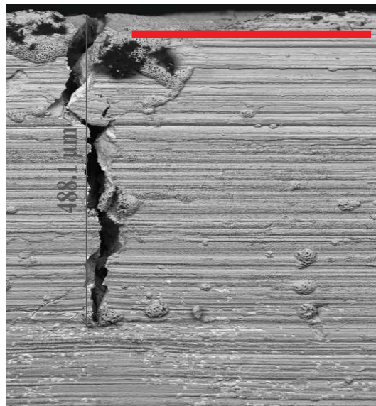
Figure 134: SEM images in BSE mode at the end of the test after unloading in the uncarburized face. The red scale bar is 300 \mu\text{m} .
