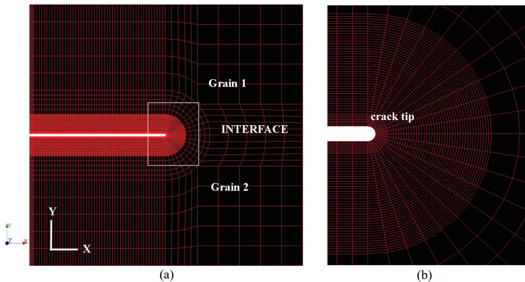
Figure 91: Cracked bicrystal mesh (7850 faces and 23951 nodes).
