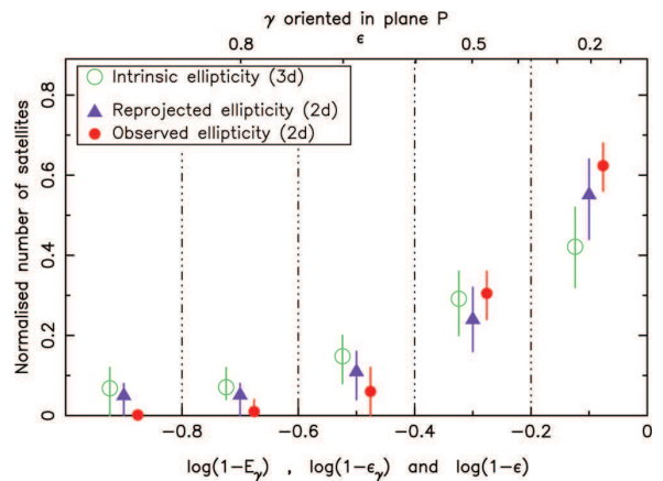
Figure 16. As Fig. 14, but for the \gamma -deprojection method.
