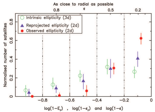
Figure 15. As Fig. 14, but for the radial deprojection method.
