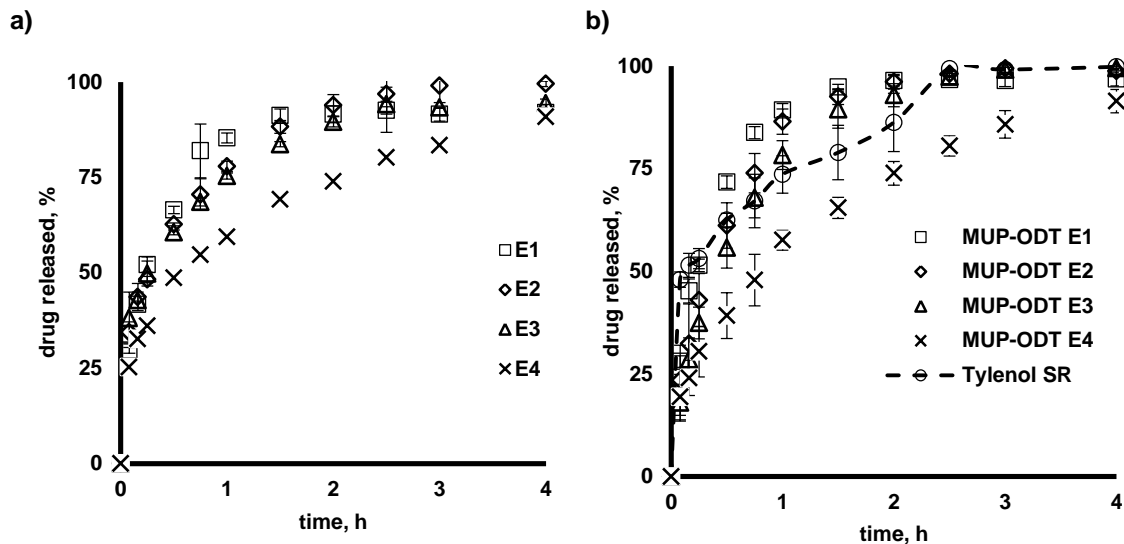
Figure III-29. In-vitro dissolution profile of APAP pellets before compression (a) and after compression (b). Apparatus 2, speed 50 rpm, volume 500 ml, medium SGF pH 1.5.
