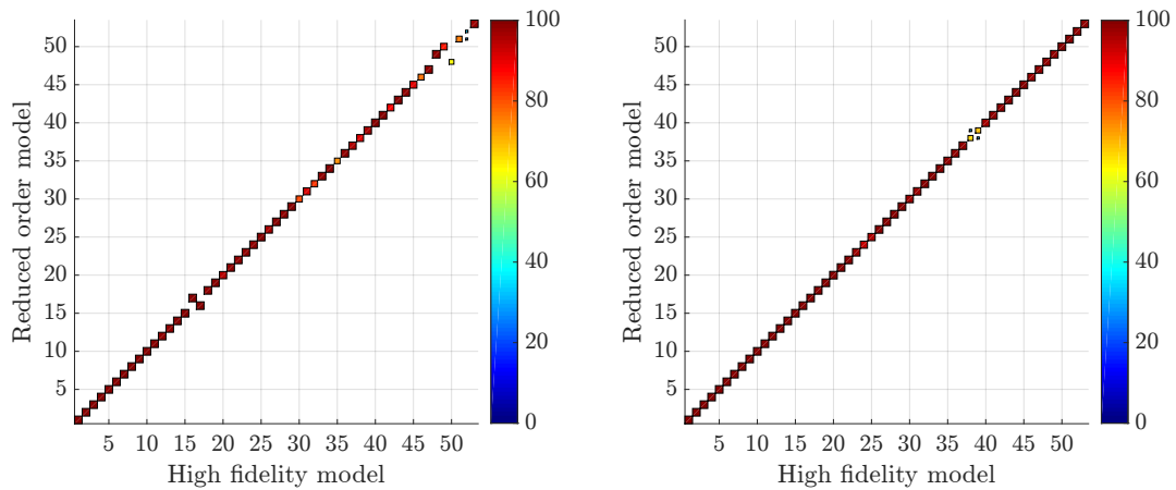
(a) Craig-Bampton method: number of DoF: 1165, MAC average: 94.37% (min.: 32.30%) (b) Proposed method: number of DoF: 185, MAC average: 98.16% (min.: 67.07%)
