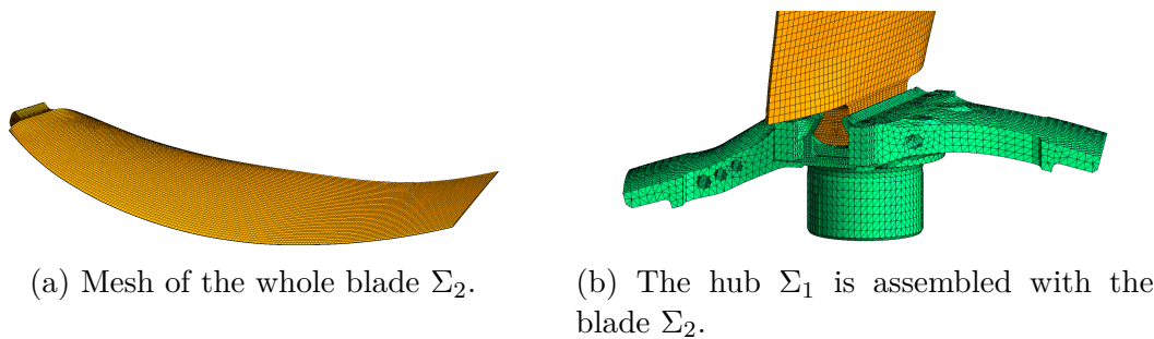
Figure 3.18 – The mesh of the blade \Sigma_2 is composed of 39724 nodes ( n_2 = 119172 DoF) while 24370 nodes ( n_1 = 70716 DoF) are used for the hub mesh \Sigma_1
