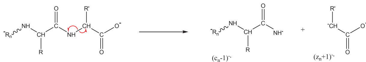
Scheme 2.5 Proposed mechanism for the formation of (c_n-1)^\bullet and (z_n+1)^\bullet fragment ions during UVPD of doubly deprotonated peptide [M-2H]^{2-} .
