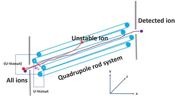
Figure 1.6 Quadrupole mass filter. The ions center and travel in the z-directions while oscillating in the x-y plane. The oscillation is controlled by the DC (U) and RF (V) voltage applied to each pair of rods. Only those ions (purple color) with stable motion at the selected U and V values will pass the quadrupole mass filter and will be detected. Other unstable ions (red) will hit the rod and will be lost.
