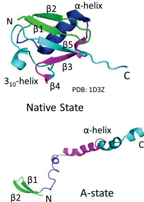
Figure 3.15 Native and A-State of Ubiquitin
