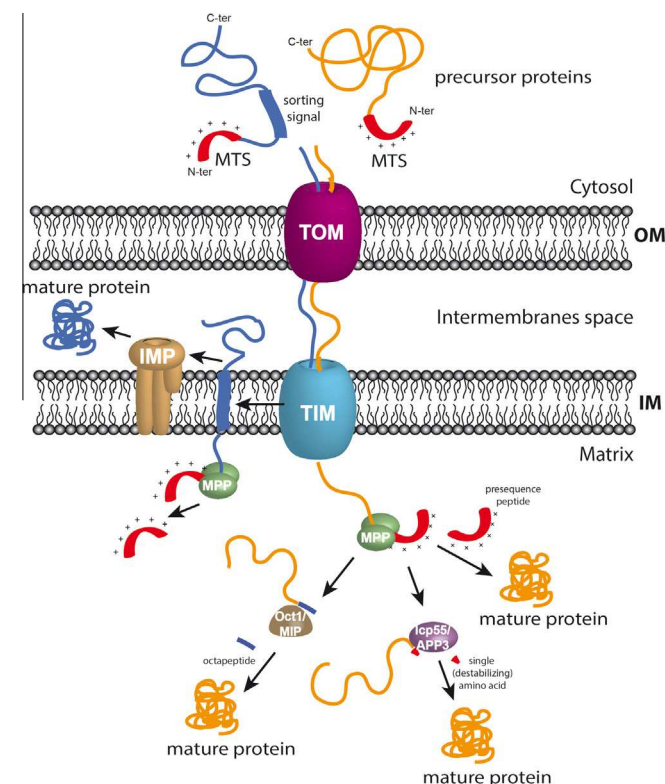
Fig. 1. Schematic overview of mitochondrial processing of precursor proteins with N-terminal targeting sequence (MTS). Mitochondrial precursor proteins are translated on cytosolic ribosomes and transported into mitochondria through the translocase of the outer-membrane (TOM) and the translocase of the inner-membrane (TIM) complexes. The N-terminal MTS is proteolytically removed upon import by several proteases, localized in the mitochondrial matrix and the inner membrane (IM). MPP: mitochondrial processing peptidase; IMP: inner membrane peptidase; Oct1: octapeptidyl aminopeptidase (yeast); MIP: mitochondrial intermediate peptidase; Icp55: intermediate cleaving peptidase 55 (yeast); and AAP3: Aminopeptidase P 3 (human). The illustration is adapted from Ref. [10].
