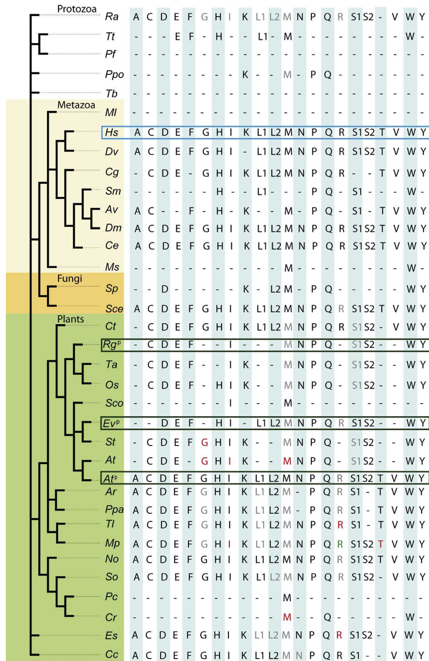
Fig. 2. Transfer RNA genes encoded by mitochondrial genomes of evolutionary divergent organisms. Only a few examples representative of the situation are given. The set of 22 tRNA genes of Homo sapiens was taken as arbitrary reference (blue frame). Amino acids in gray or green indicate that 2 or 3 isoacceptor tRNA genes respectively are mitochondrion-encoded and necessary to decode all codons of the family and ensure mt translation. Amino acids in red indicate that one isoacceptor tRNA is missing to carry out mt translation. Hs , Homo sapiens (J01415); Dv , Didelphis virginiana (Z29573); Dm , Drosophila melanogaster (U37541); Ce , Caenorhabditis elegans (U37541); Sm , Steganacarus magnus (EU935607); Av , Armstrongia vulgaris (EU935607); Cg , Crassostrea gigas (AF177226); Ms , Metridium senile (AF000023); MI , Mnemiopsis leidyi (JF760210); Sc , Saccharomyces cerevisiae (AJ011856); Sp , Spizellomyces punctatus (AF404303; AF404304; AF404305); Ppo , Physarum polycephalum (AB027295); Tt , Tetrahymena thermophila (AB027295); Ra , Reclinomonas americana (AF007261); Tb , Trypanosoma brucei [126]; Pf , Plasmodium falciparum (AJ276845); Cp , Chlamydomonas reinhardtii (AJ276845); Pc , Polytomella capuana (EF645804); Np , Nephrolepis olivacea (AF110138); So , Scenedesmus obliquus (AF040457); Es , Ectocarpus siliculosus (FP885846); Cc , Chondrus crispus (Z47547); Ppa , Physcometrella patens (AB251495); Mp , Marchantia polymorpha (M68929); Ar , Anomodon rugelii (JF973314); Tl , Trebulia lacunosa (JF973315); Ct , Cycas taitungensis (AP009381); At , Arabidopsis thaliana (Y08501); St , Solanum tuberosum (L. Maréchal-Drouard, personal communication); Sco , Silene conica [127]; Ta , Triticum aestivum (AP008982); Os , Oryza sativa (BA000029). The tRNA genes encoded by Rg p ( Rhizanthella gardneri , NC 014874), Ev p ( Epifagus virginiana , NC 014874) and At p ( Neurospora crassa , NC 009322) plastidial genomes are framed in green.
