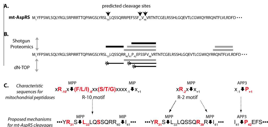
Fig. 3. N-termini for human mitochondrial aspartyl-tRNA synthetase. A. N-terminal sequence of the human mt-AspRS precursor. Cleavage sites, predicted in silico (MitoFates [32] for L_{33} ; Predotar [30] and MitoProt [31] for F_{47} ; based on multiple sequence alignment for V_{48} [3]) are shown with black arrowheads. B. Peptides identified experimentally, by the shotgun Proteomics approach on mt-AspRS enriched sample (above the sequence), and by the doublet N-terminal oriented Proteomics (below the sequence). Tryptic peptides are in gray, semi-tryptic peptides in black, and TMPP-modified peptides in black with asterisks. C. Sequence motifs for peptidases implicated in MTS processing. Upper part: characteristic sequences of R-10 motif, known to be cleaved by mitochondrial processing peptidase (MPP) and mitochondrial intermediate peptidase (MIP); of R-2 motif, cleaved by the MPP (reviewed in [11,35]); and of sequence cleaved by the Aminopeptidase P APP3 [14,39]. Lower part: inspection of mt-AspRS sequence and possible cleavages in agreement with N-terminal peptides experimentally validated.
