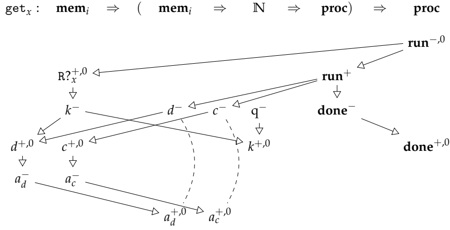
FIGURE 5. An alternative interpretation of \text{get}_x performing more reorderings
