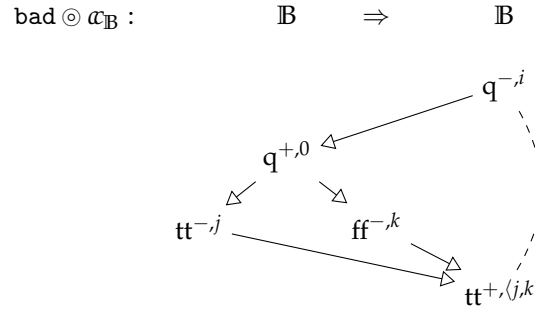
FIGURE 3. The strategy bad
